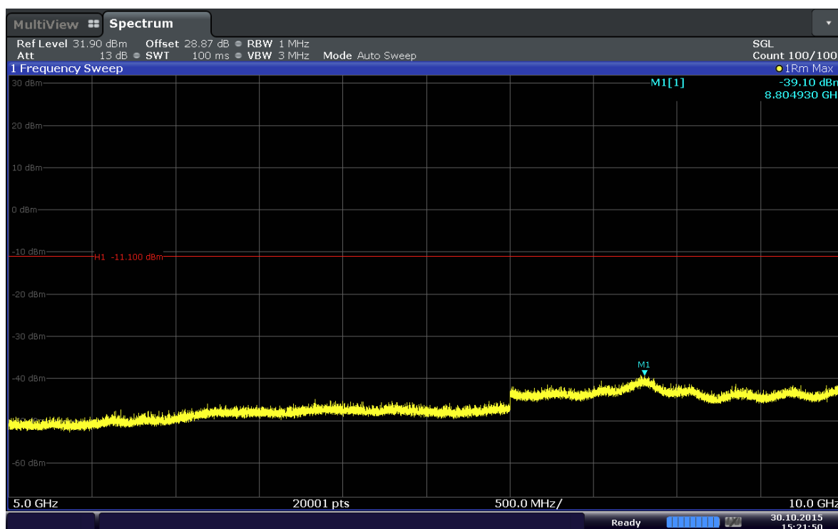
Plot 6-22. Conducted Spurious Plot (Band 5–5.0MHz–QPSK–RB Size 1–RB Offset 0– Ch.20425)
