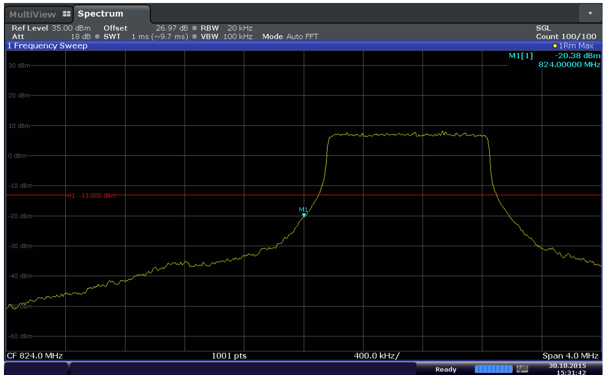
Plot 6-33. Lower Band Edge Plot (Band5 – 1.4MHz – QPSK – RB Size 6)
