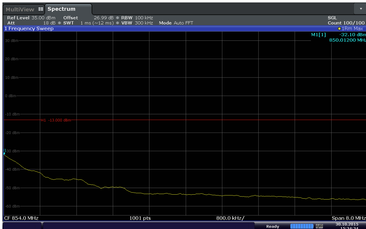
Plot 6-36. Extended Upper Band Edge Plot (Band5 – 1.4MHz – QPSK – RB Size 6)
