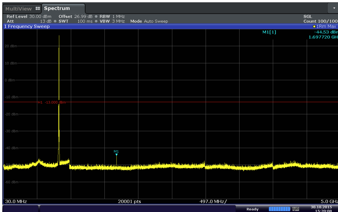
Plot 6-19. Conducted Spurious Plot (Band 5–3.0MHz–QPSK–RB Size 1–RB Offset 14– Ch.20635)
