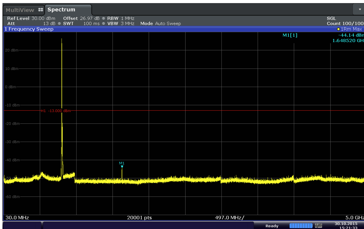
Plot 6-21. Conducted Spurious Plot (Band 5–5.0MHz–QPSK–RB Size 1–RB Offset 0– Ch.20425)
