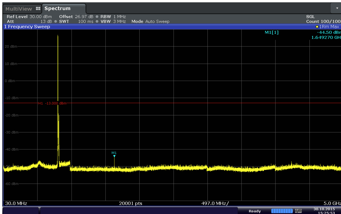
Plot 6-27. Conducted Spurious Plot (Band 5–10.0MHz–QPSK–RB Size 1–RB Offset 0– Ch.20450)
