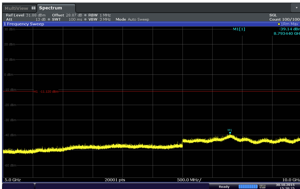
Plot 6-20. Conducted Spurious Plot (Band 5–3.0MHz–QPSK–RB Size 1–RB Offset 14– Ch.20635)
