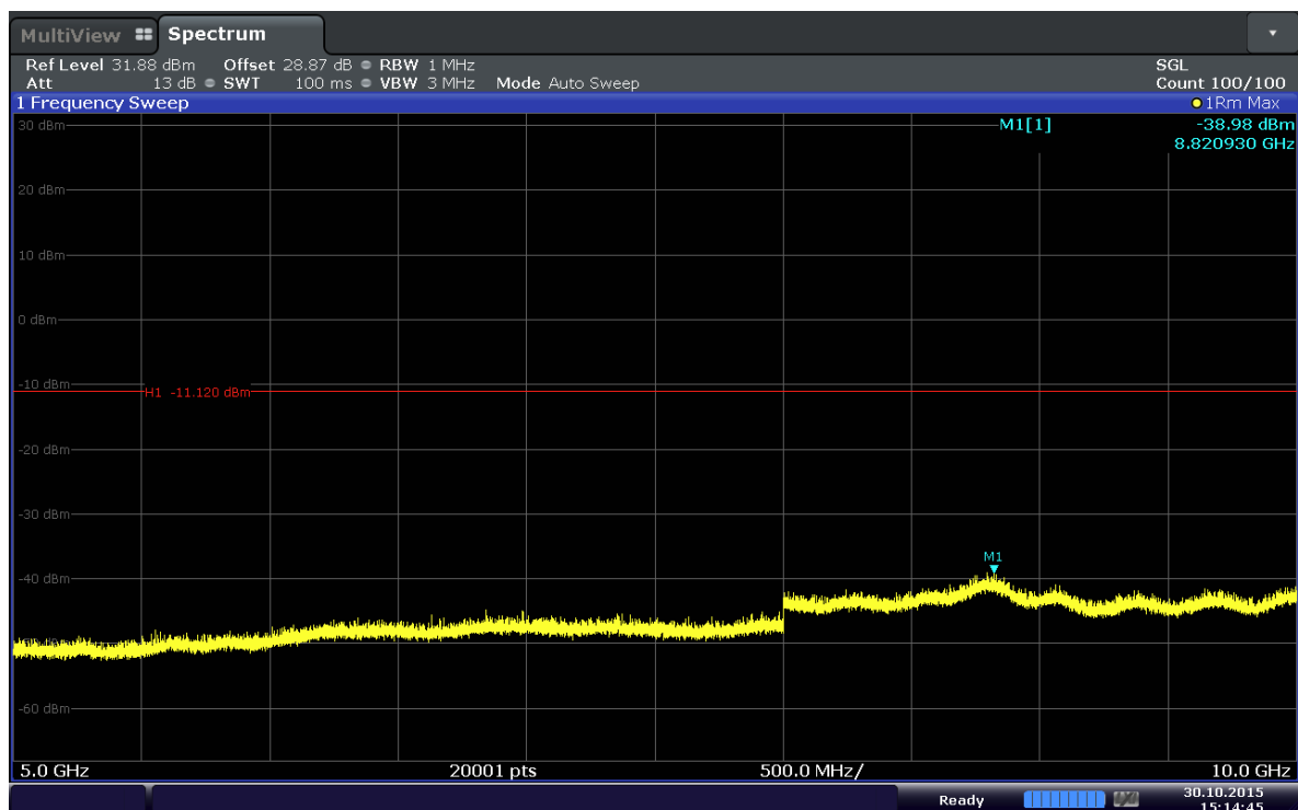
Plot 6-12. Conducted Spurious Plot (Band 5–1.4MHz–QPSK–RB Size 1–RB Offset 2–Ch.20525)
