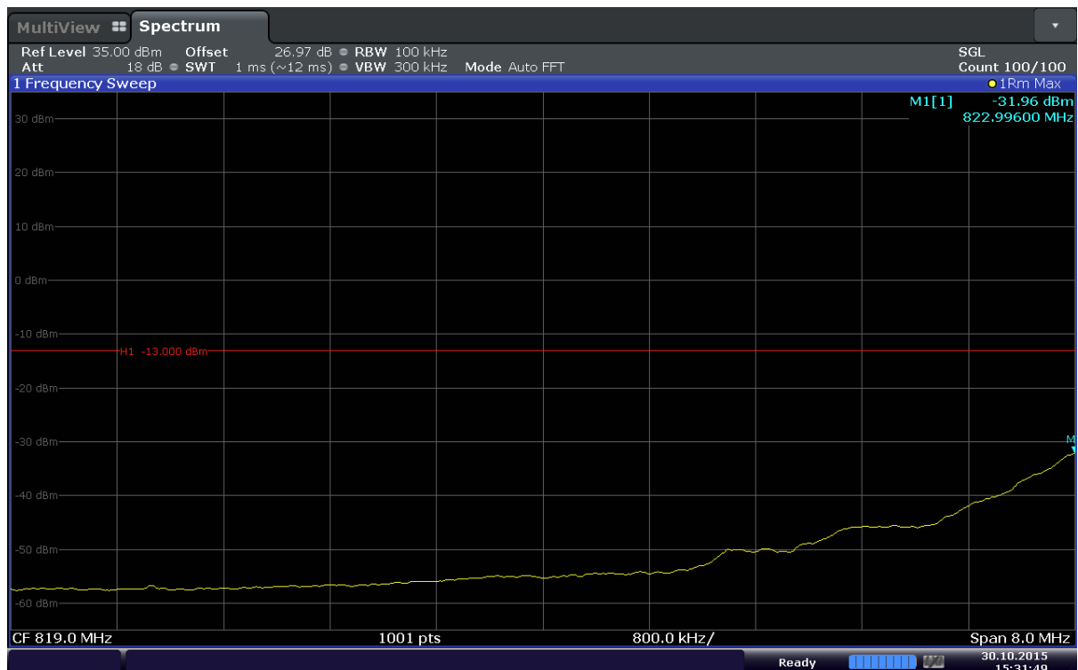
Plot 6-34. Extended Lower Band Edge Plot (Band5 – 1.4MHz – QPSK – RB Size 6)
