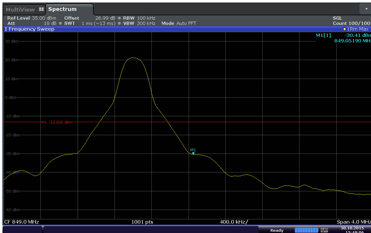
Plot 6-48. Upper Band Edge Plot (Band 5 – 10.0MHz – QPSK – RB Size 1 – RB Offset 49)
