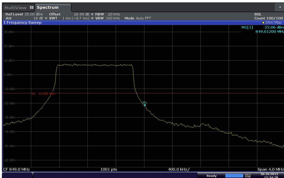
Plot 6-35. Upper Band Edge Plot (Band5 – 1.4MHz – QPSK – RB Size 6)
