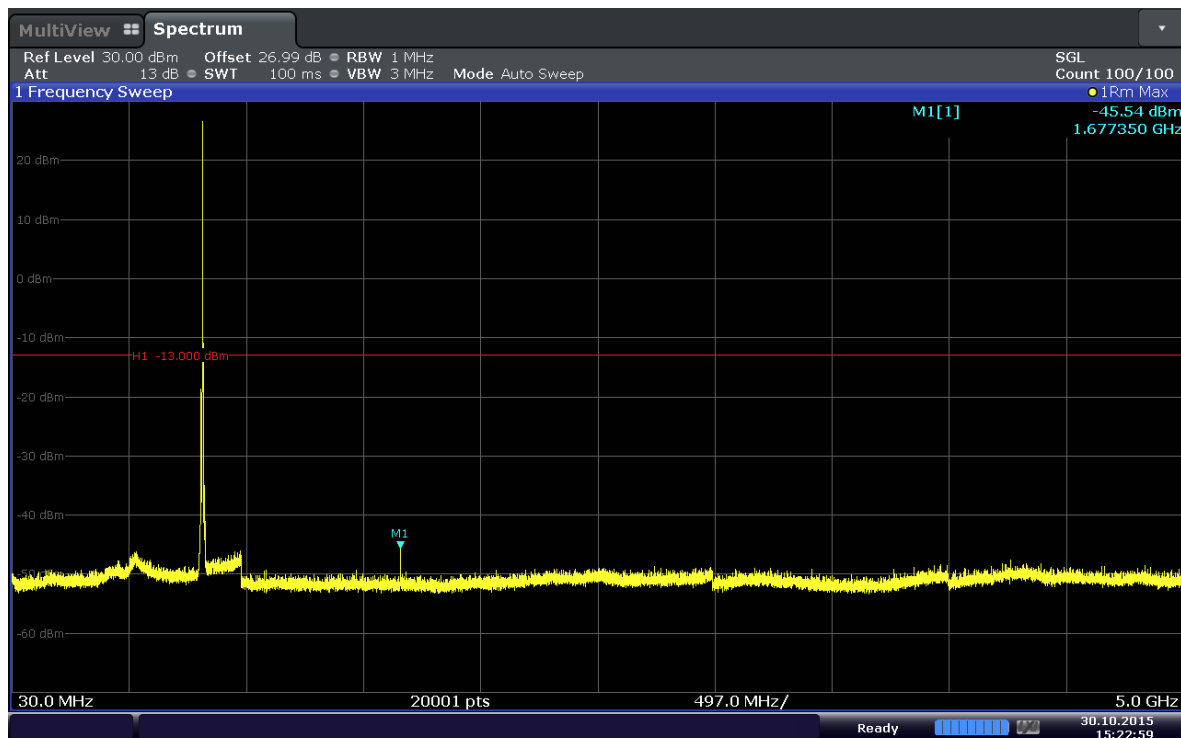
Plot 6-23. Conducted Spurious Plot (Band 5–5.0MHz–QPSK–RB Size 1–RB Offset 24– Ch.20525)
