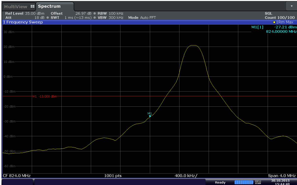
Plot 6-46. Lower Band Edge Plot (Band 5 – 10.0MHz – QPSK – RB Size 1 – RB Offset 0)
