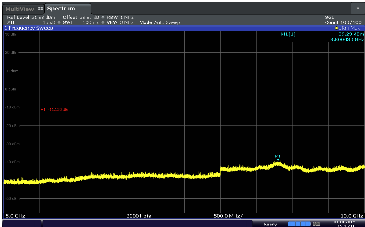
Plot 6-14. Conducted Spurious Plot (Band 5–1.4MHz–QPSK–RB Size 1–RB Offset 0– Ch.20643)
