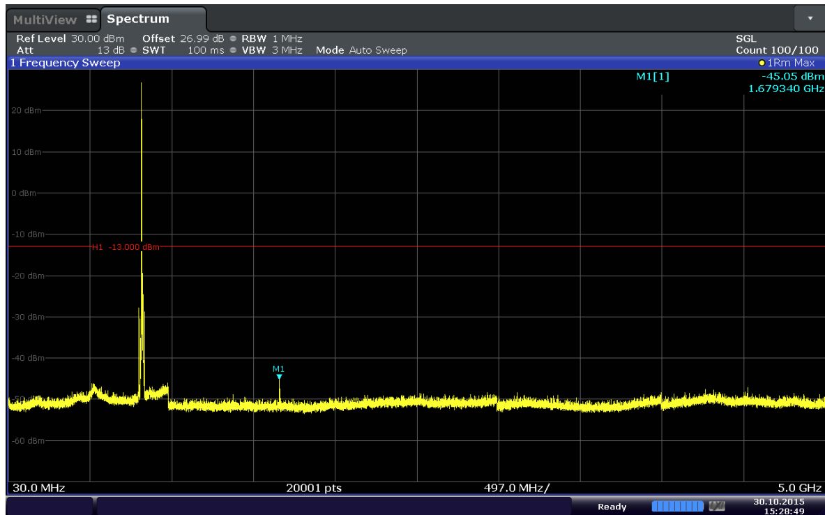
Plot 6-31. Conducted Spurious Plot (Band 5–10.0MHz–QPSK–RB Size 1–RB Offset 0– Ch.20600)
