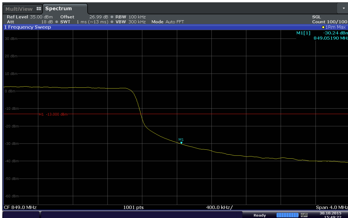
Plot 6-47. Upper Band Edge Plot (Band 5 – 10.0MHz – QPSK – RB Size 50)
