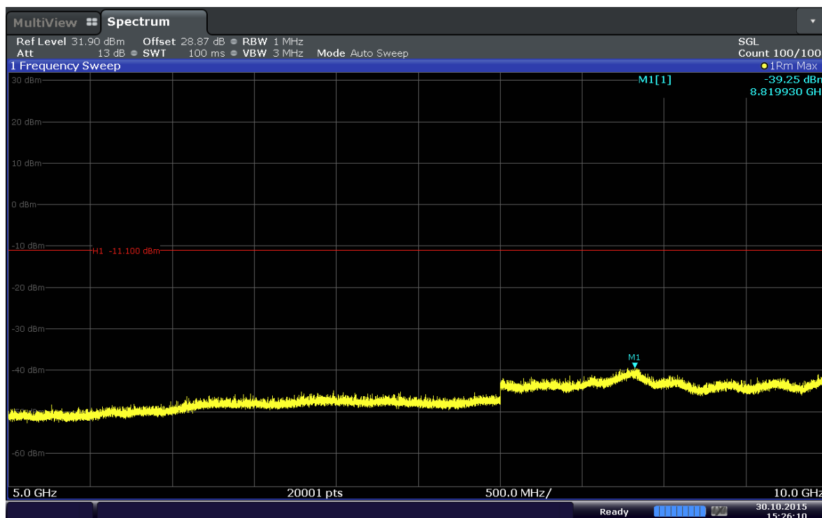
Plot 6-28. Conducted Spurious Plot (Band 5–10.0MHz–QPSK–RB Size 1–RB Offset 0– Ch.20450)
