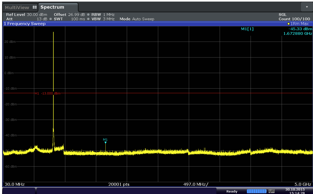
Plot 6-11. Conducted Spurious Plot (Band 5–1.4MHz–QPSK–RB Size 1–RB Offset 2–Ch.20525)
