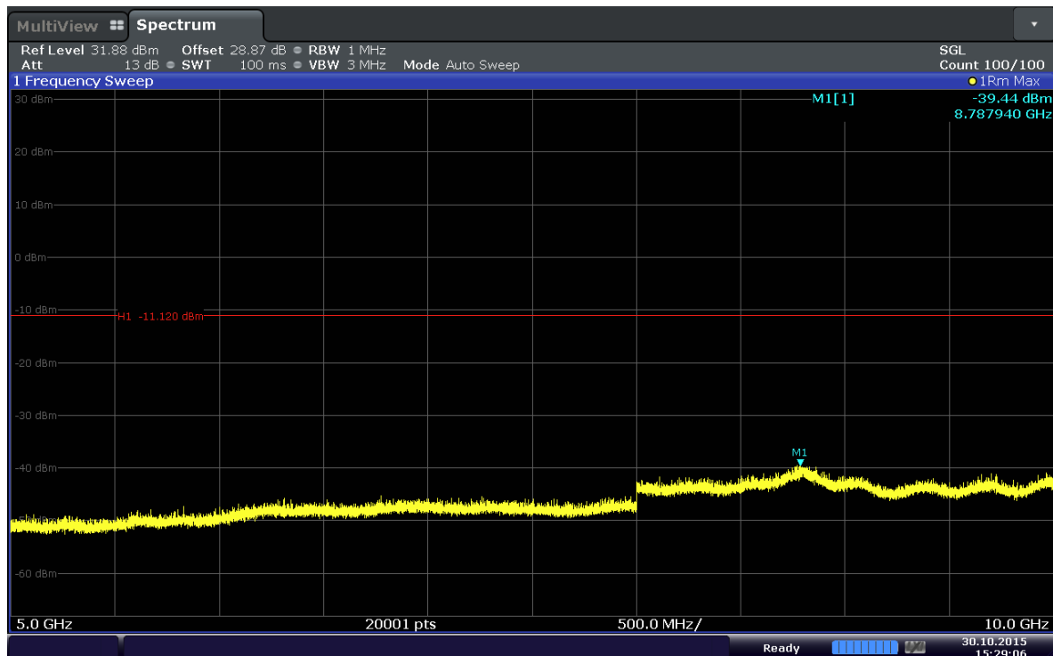
Plot 6-32. Conducted Spurious Plot (Band 5–10.0MHz–QPSK–RB Size 1–RB Offset 0– Ch.20600)
