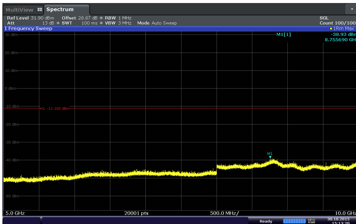
Plot 6-9. Conducted Spurious Plot (Band 5–1.4MHz–QPSK–RB Size 1–RB Offset 2–Ch.20407)
