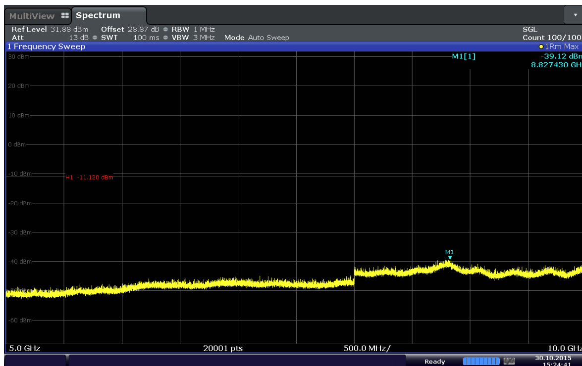
Plot 6-26. Conducted Spurious Plot (Band 5–5.0MHz–QPSK–RB Size 1–RB Offset 0– Ch.20625)
