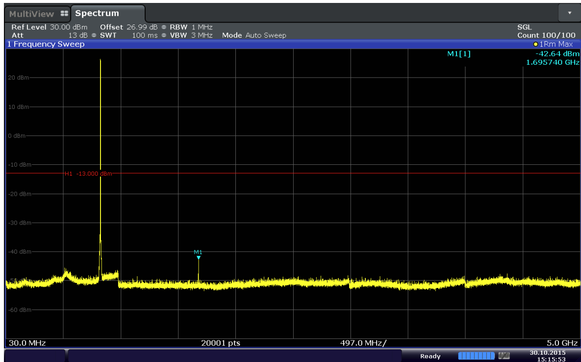
Plot 6-13. Conducted Spurious Plot (Band 5–1.4MHz–QPSK–RB Size 1–RB Offset 0– Ch.20643)
