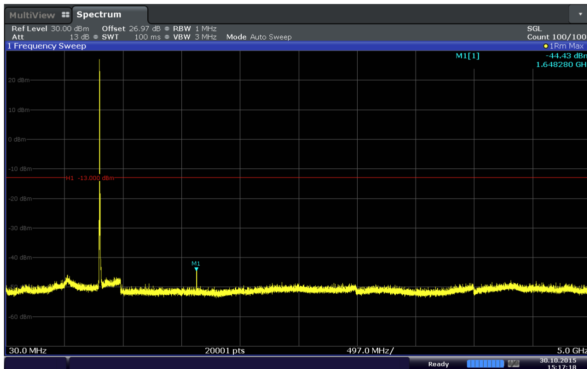
Plot 6-15. Conducted Spurious Plot (Band 5–3.0MHz–QPSK–RB Size 1–RB Offset 0– Ch.20415)
