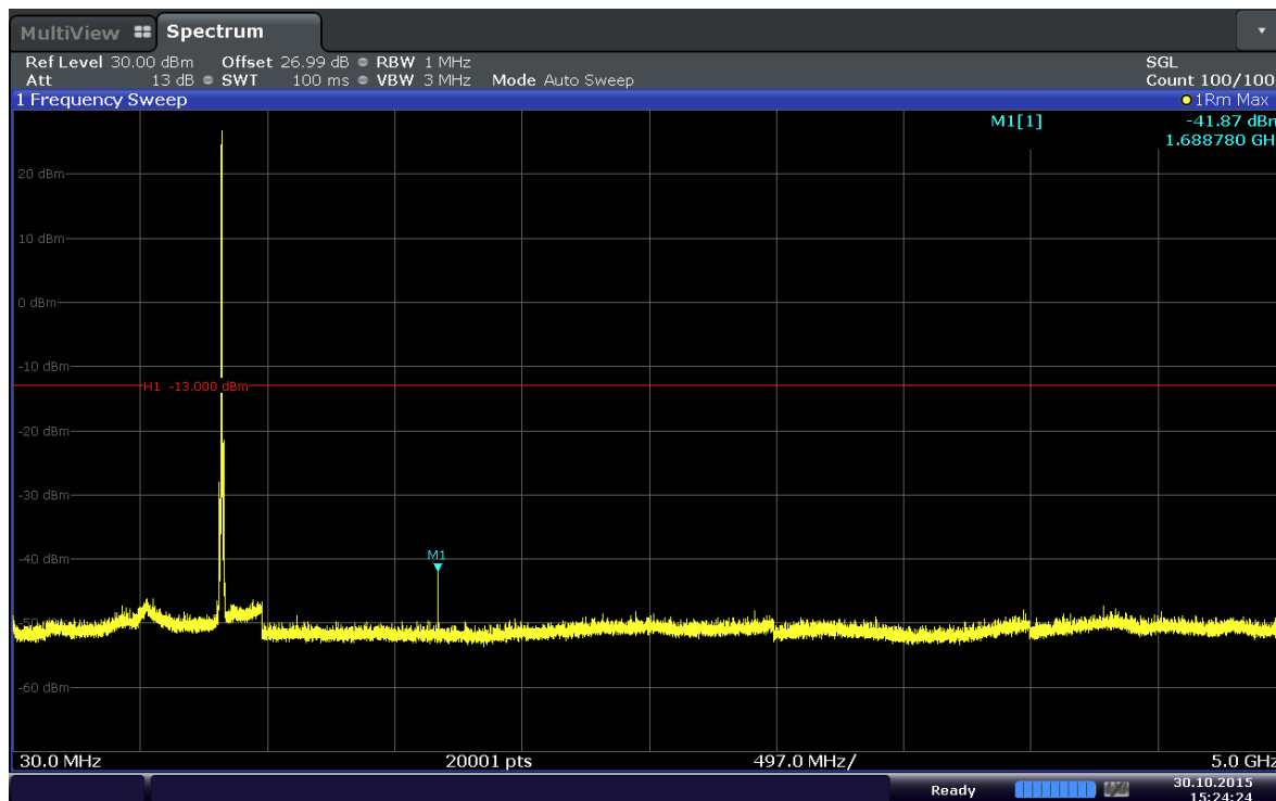
Plot 6-25. Conducted Spurious Plot (Band 5–5.0MHz–QPSK–RB Size 1–RB Offset 0– Ch.20625)
