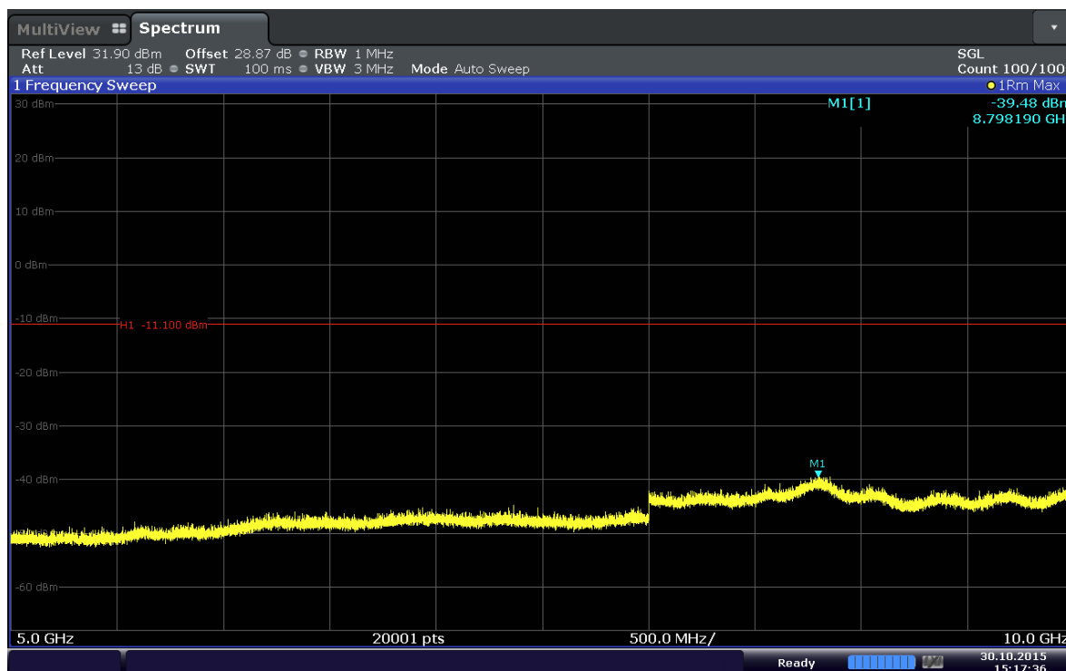
Plot 6-16. Conducted Spurious Plot (Band 5–3.0MHz–QPSK–RB Size 1–RB Offset 0– Ch.20415)
