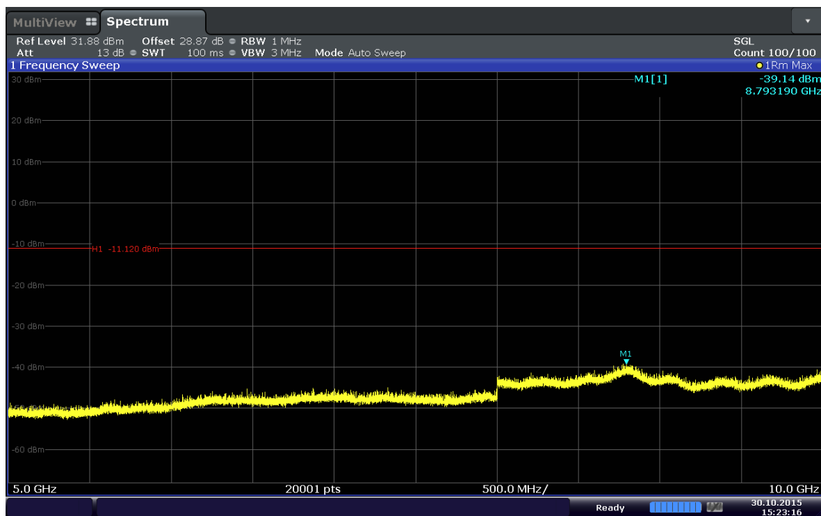
Plot 6-24. Conducted Spurious Plot (Band 5–5.0MHz–QPSK–RB Size 1–RB Offset 24– Ch.20525)
