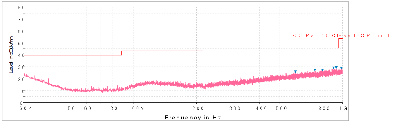
Plot 7-52. Radiated Spurious Plot below 1GHz (Pol. H)
