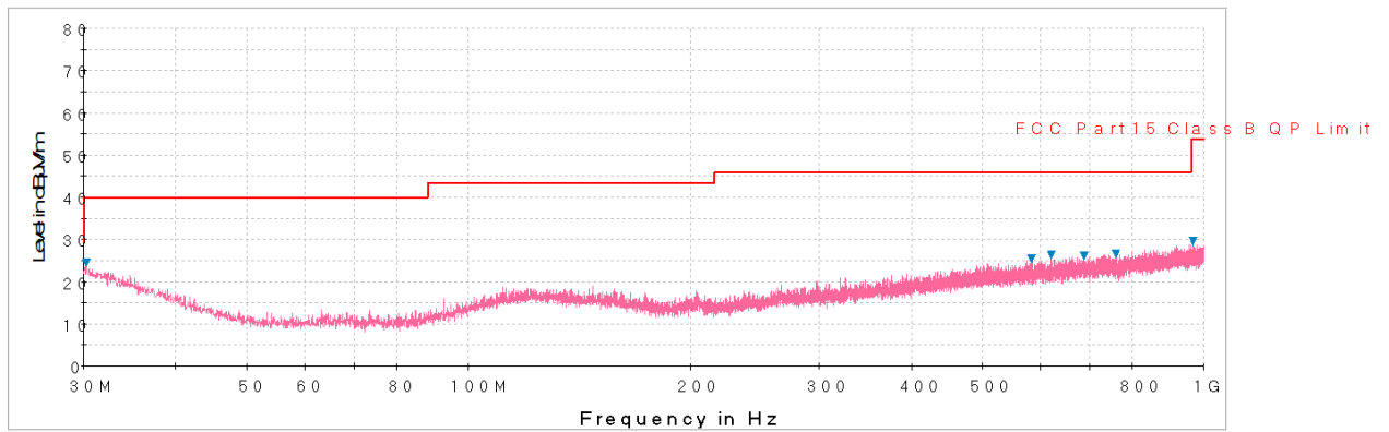
Plot 7-53. Radiated Spurious Plot below 1GHz (Pol. V)
