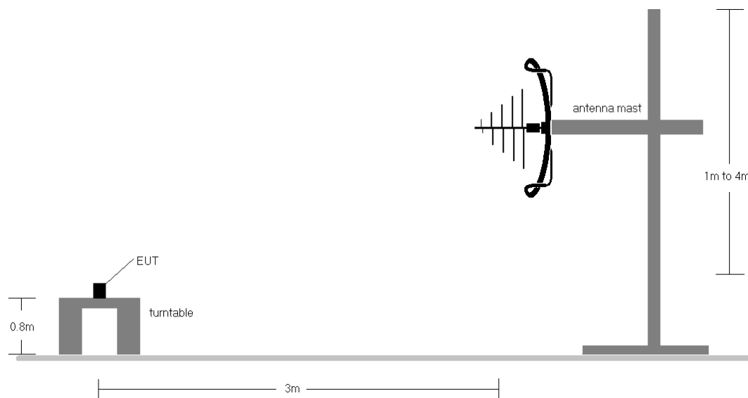
Figure 8-5. Radiated Test Setup
