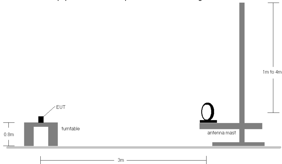
Figure 8-4. Radiated Test Setup
