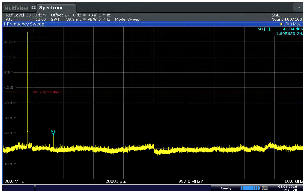
Plot 6-11. Conducted Spurious Plot (Band 5–1.4MHz–QPSK–RB Size 1–RB Offset 0– Ch.20643)
