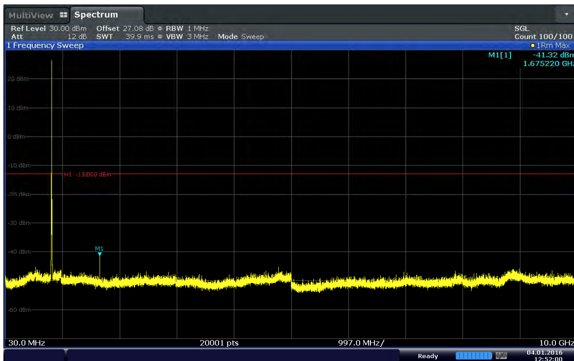
Plot 6-13. Conducted Spurious Plot (Band 5–3.0MHz–QPSK–RB Size 1–RB Offset 14– Ch.20525)
