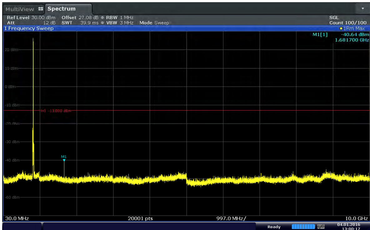
Plot 6-19. Conducted Spurious Plot (Band 5–10.0MHz–QPSK–RB Size 1–RB Offset 49– Ch.20525)
