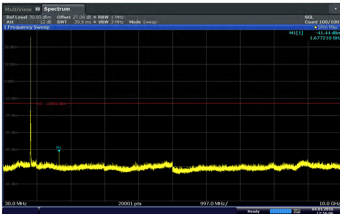
Plot 6-16. Conducted Spurious Plot (Band 5–5.0MHz–QPSK–RB Size 1–RB Offset 24– Ch.20525)
