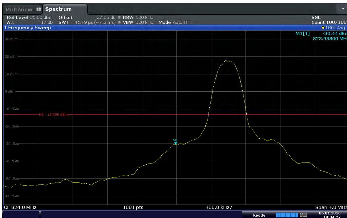
Plot 6-34. Lower Band Edge Plot (Band 5 – 10.0MHz – QPSK – RB Size 1 – RB Offset 0)
