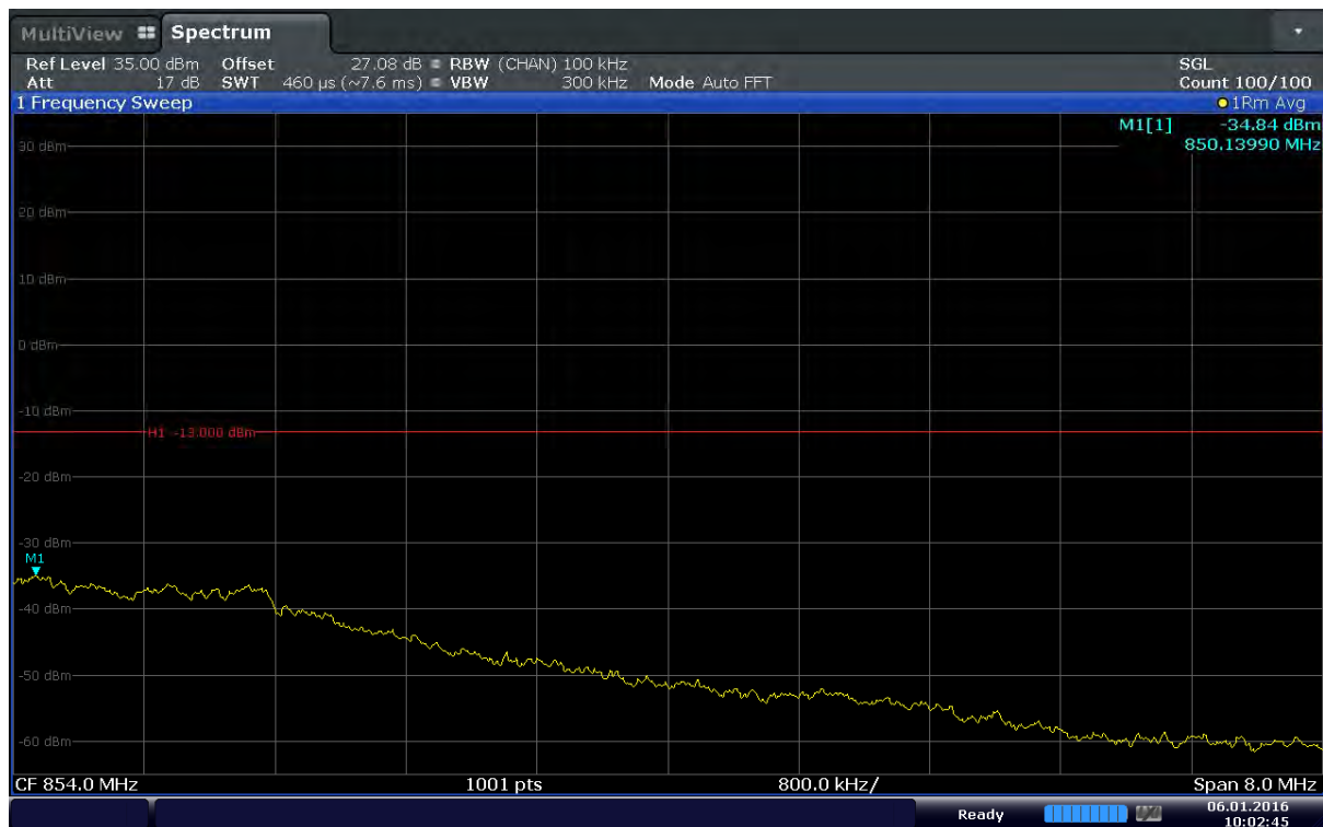
Plot 6-28. Extended Upper Band Edge Plot (Band 5 – 3.0MHz – QPSK – RB Size 15)
