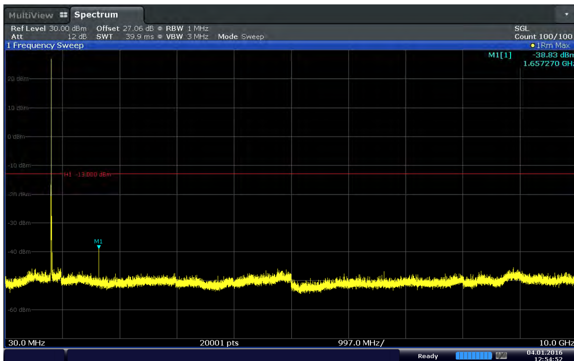
Plot 6-15. Conducted Spurious Plot (Band 5–5.0MHz–QPSK–RB Size 1–RB Offset 24– Ch.20425)
