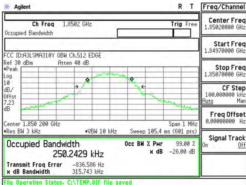
Plot 6-4. Occupied Bandwidth Plot (EDGE1900 Mode - Ch.512)
