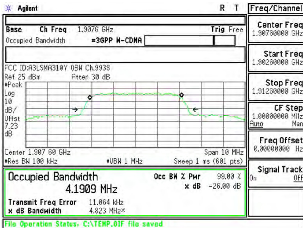
Plot 6-6. Occupied Bandwidth Plot (PCS WCDMA Mode - Ch.9538(DL9938))
