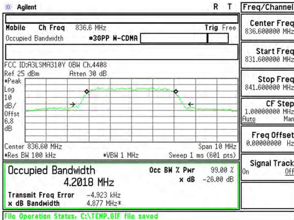
Plot 6-5. Occupied Bandwidth Plot (Cellular WCDMA Mode - Ch.4183(DL4408))
