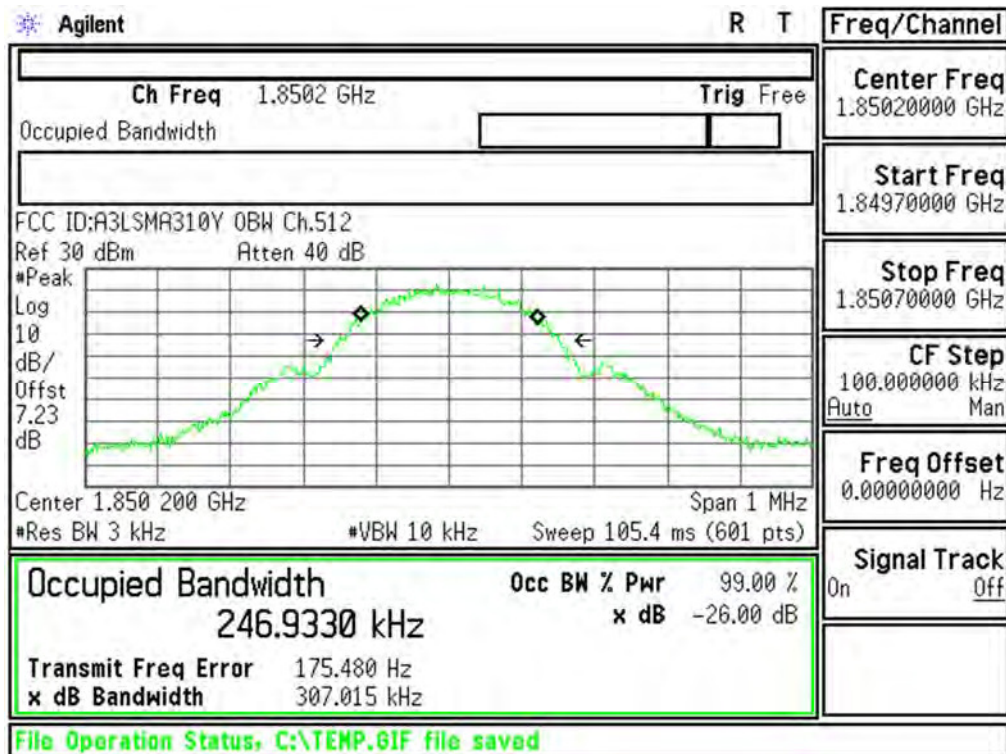
Plot 6-3. Occupied Bandwidth Plot (PCS GSM Mode - Ch.512)
