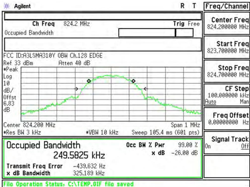
Plot 6-2. Occupied Bandwidth Plot (EDGE850 Mode - Ch.128)
