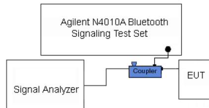
Figure 7-7. Test Instrument & Measurement Setup
