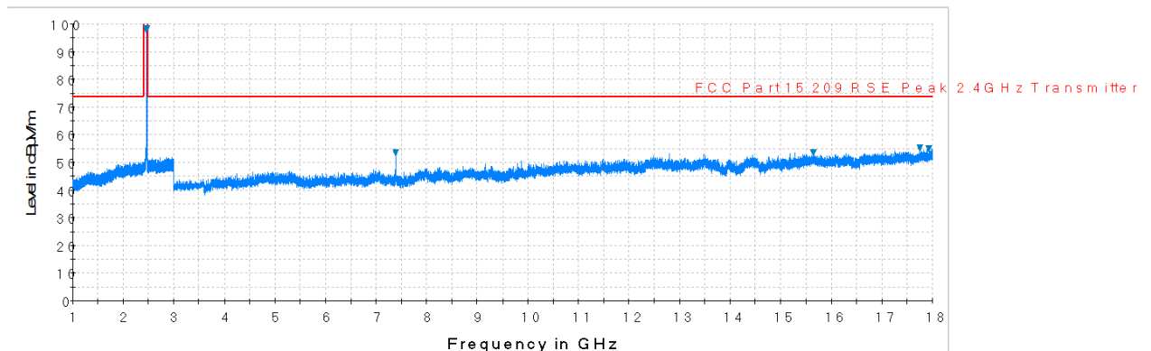
Plot 7-36. Radiated Spurious Plot above 1GHz (802.11b – Ch. 11, Ant. Pol. V)
