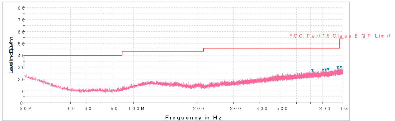
Plot 7-41. Radiated Spurious Plot below 1GHz (Pol. H)
