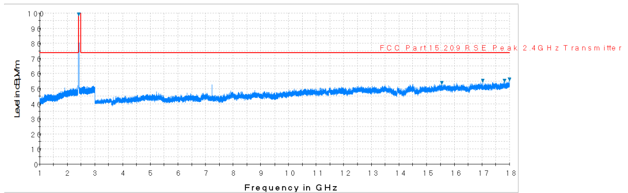
Plot 7-32. Radiated Spurious Plot above 1GHz (802.11b – Ch. 1, Ant. Pol. V)
