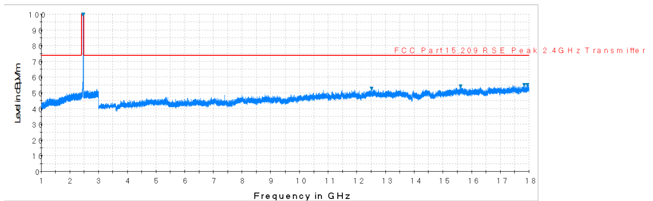
Plot 7-35. Radiated Spurious Plot above 1GHz (802.11b – Ch. 11, Ant. Pol. H)
