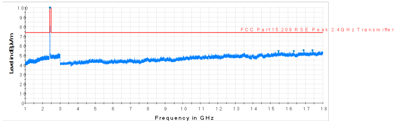
Plot 7-31. Radiated Spurious Plot above 1GHz (802.11b – Ch. 1, Ant. Pol. H)
