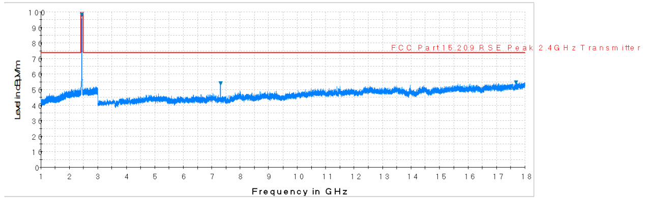
Plot 7-34. Radiated Spurious Plot above 1GHz (802.11b – Ch. 6, Ant. Pol. V)
