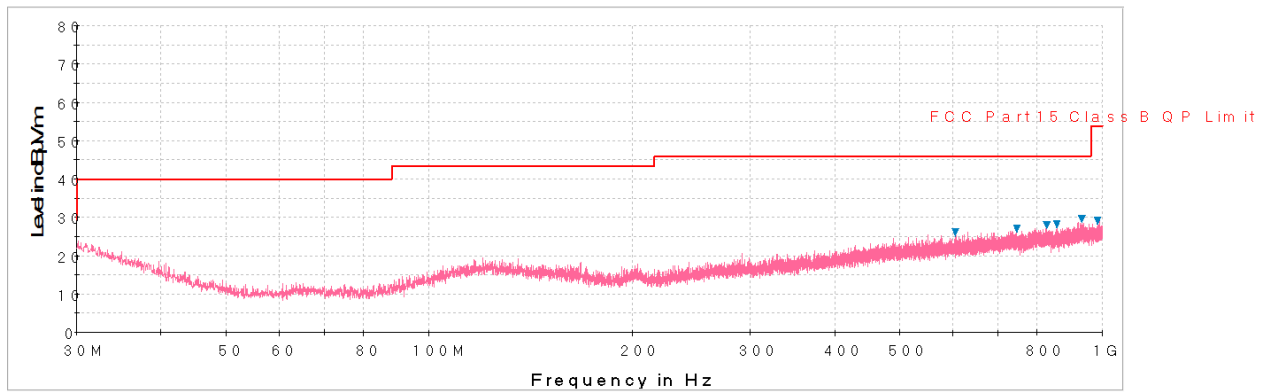
Plot 7-42. Radiated Spurious Plot below 1GHz (Pol. V)
