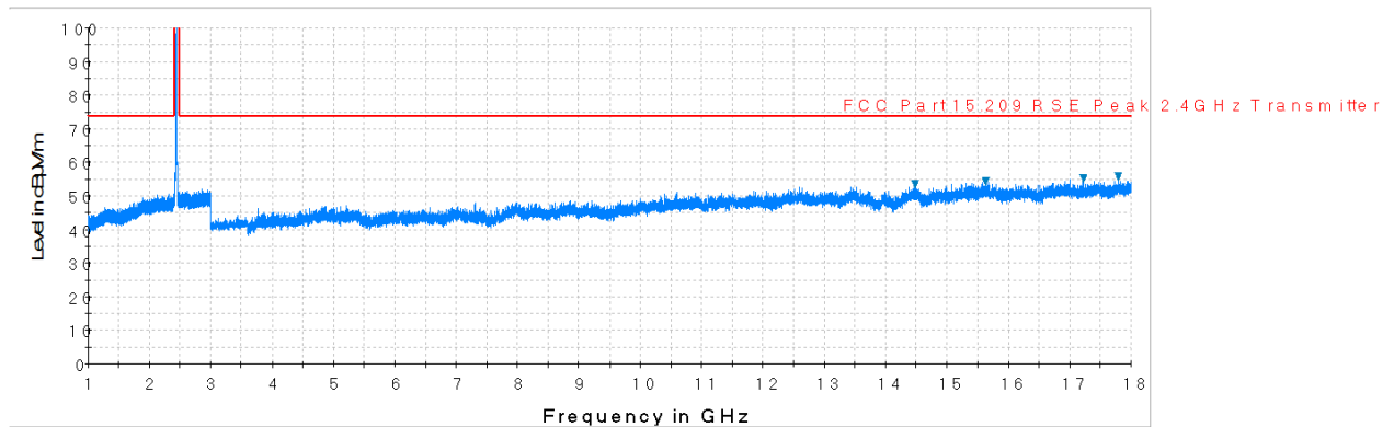
Plot 7-33. Radiated Spurious Plot above 1GHz (802.11b – Ch. 6, Ant. Pol. H)
