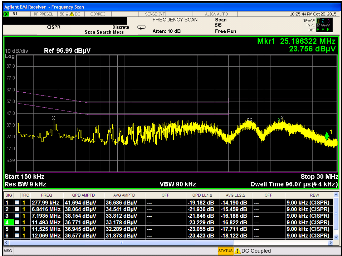
Plot 7-44. Line Conducted Plot with 802.11b (N)
