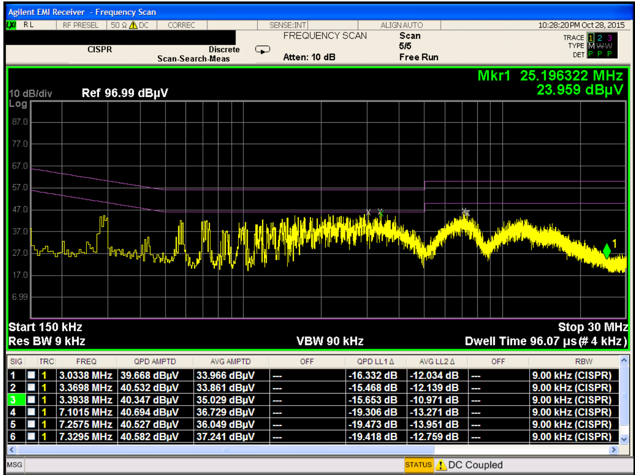
Plot 7-43. Line Conducted Plot with 802.11b (L1)
