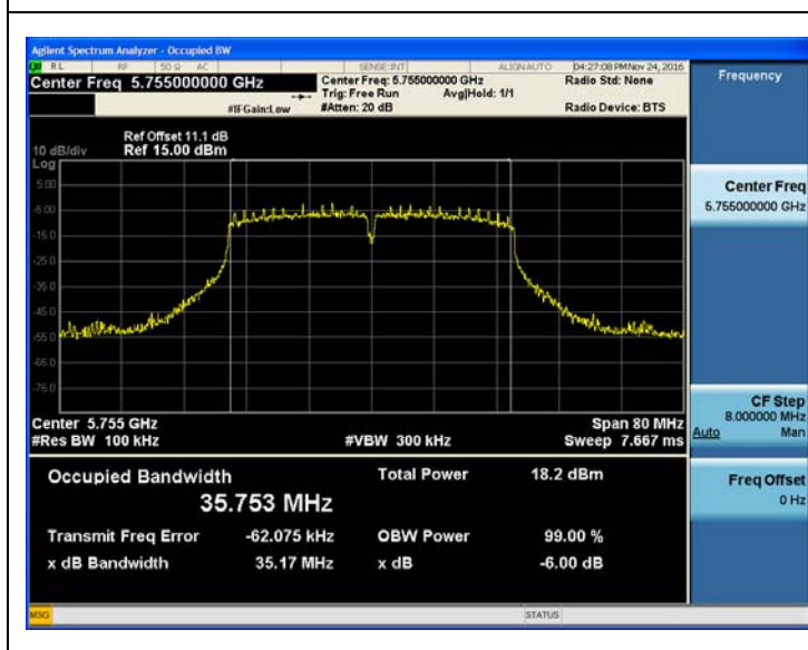
802.11n_HT40 UNII 3 BAND 6dB Bandwidth(CH.151)
