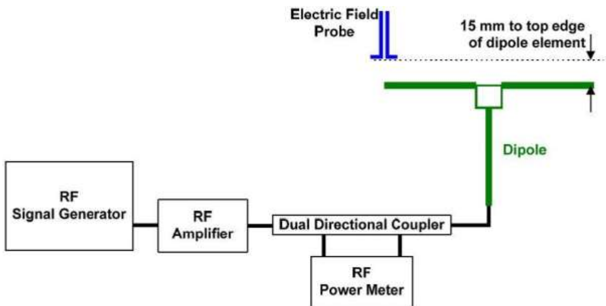
Setup diagram
