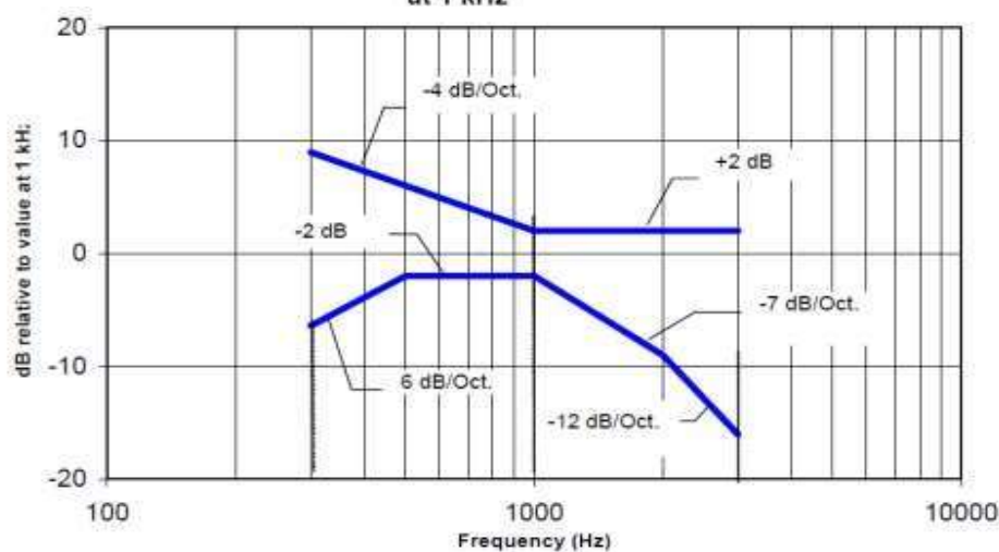
Figure 8.1—Magnetic field frequency response for WDs with field strength \leq -15 dB (A/m) at 1 kHz
