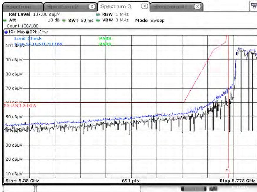
Peak Result (802.11ac_VHT40, Ch.151, X-H)
