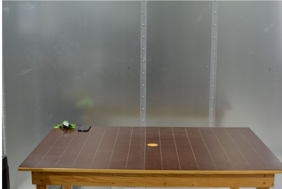
Figure 7. Test Setup – ACLC– <30MHz
