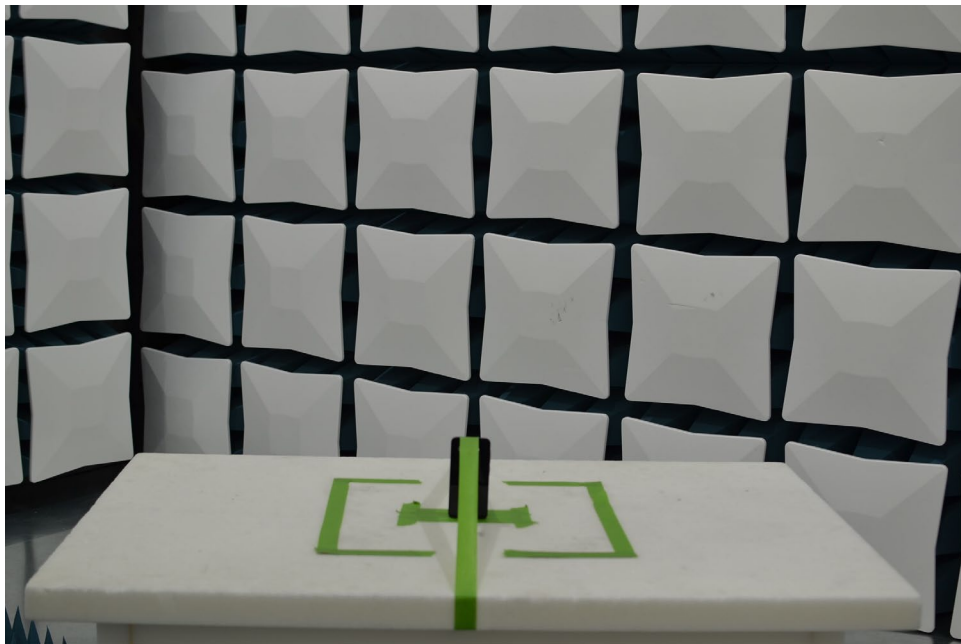
Figure 6. Test Setup – Z Position – 30MHz-1GHz
