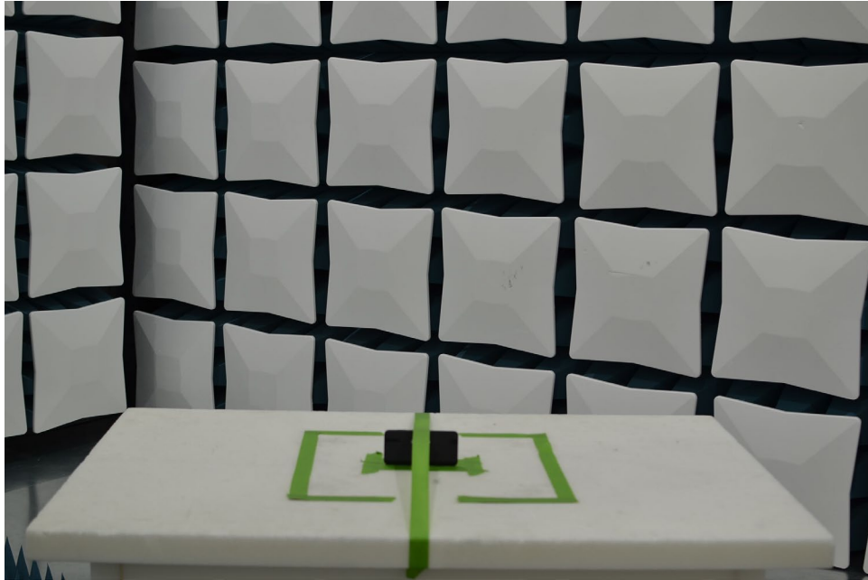
Figure 5. Test Setup – Y Position – 30MHz-1GHz
