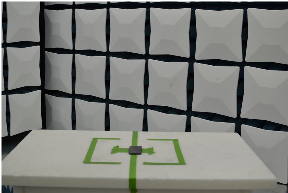
Figure 4. Test Setup – X Position – 30MHz-1GHz
