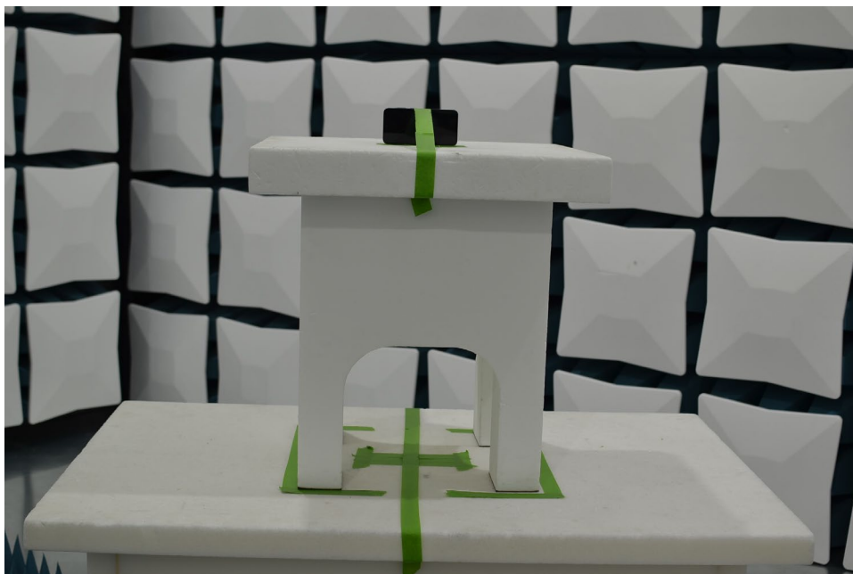
Figure 2. Test Setup – Y Position – 1GHz-18GHz
