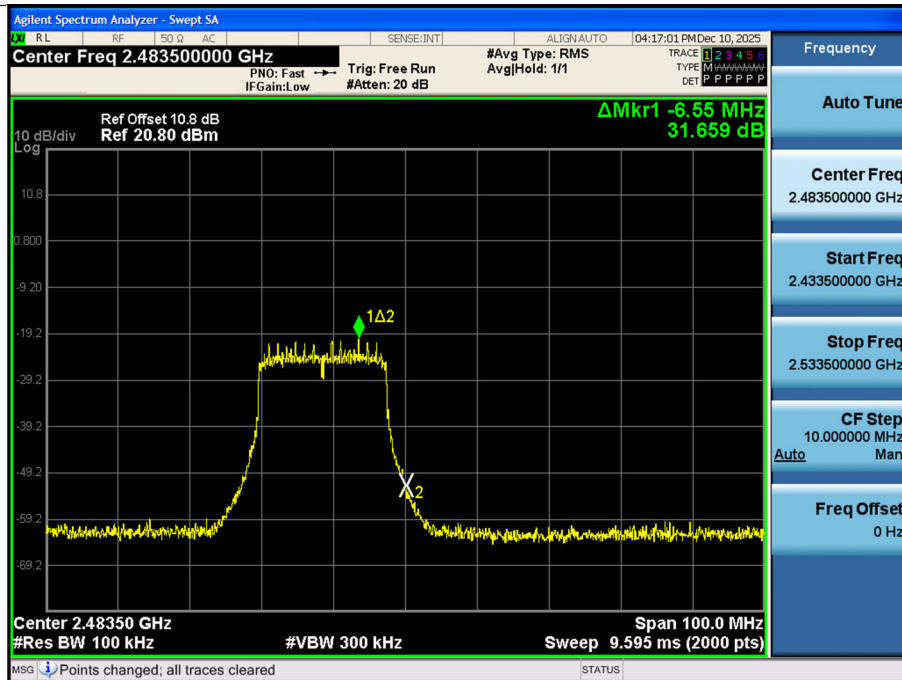
[ANT. 2] 802.11n(HT20)- CH 13
