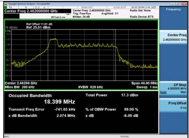
BW20M Ch.11(2462 MHz) RU 0
