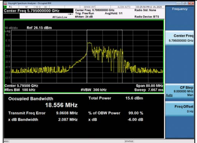
Bandwidth 40M Ch.159, 26 Tones RU 9
