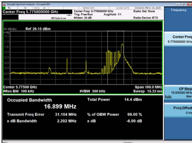
Bandwidth 80M Ch.155, 26 Tones RU 36
