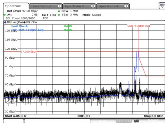
Average result (802.11ax(HE80) Ch.171, 106T RU 60)
