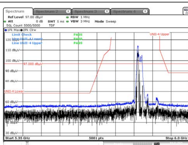
Peak result (802.11ax(HE40) Ch.167, 52T RU 37)
