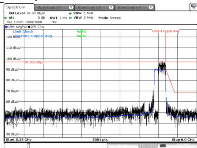
Average result (802.11ax(HE80) Ch.171, 484T RU 66)
