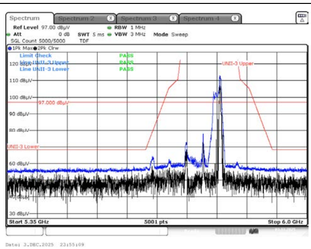
Peak result (802.11ax(HE80) Ch.155, 52T RU 52)
