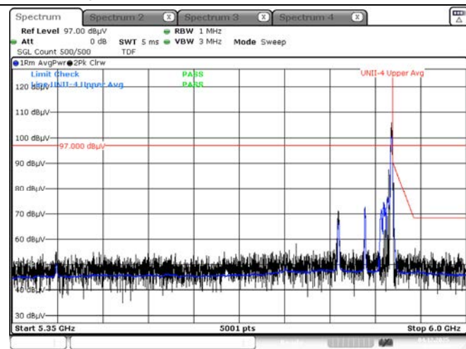
Average result (802.11ax(HE80) Ch.171, 26T RU 36)
