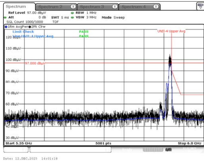
Average result (802.11ax(HE40) Ch.175, 484T RU 65)
