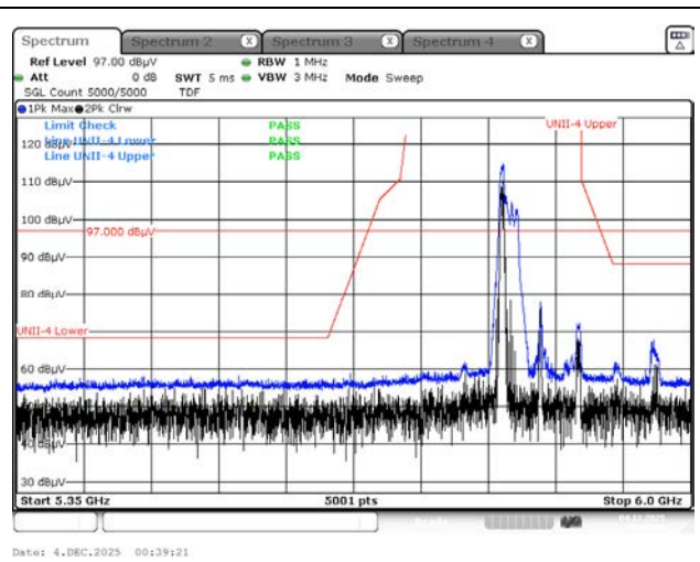
Peak result (802.11ax(HE80) Ch.171, 52T RU 37)
