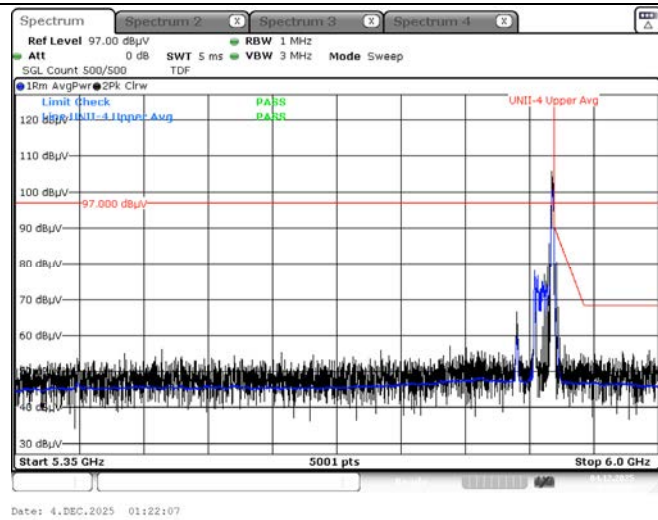
Average result (802.11ax(HE40) Ch.175, 106T RU 56)
