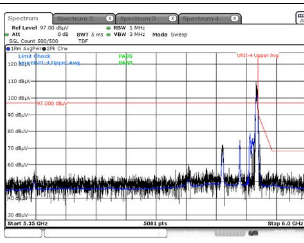
Average result (802.11ax(HE80) Ch.171, 52T RU 52)
