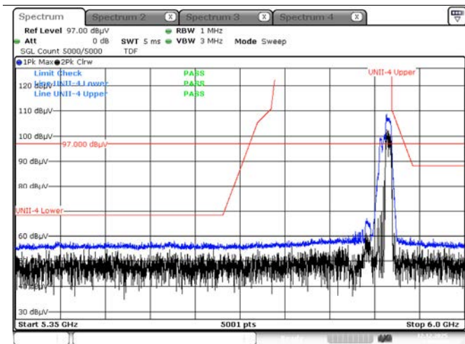
Peak result (802.11ax(HE40) Ch.175, 106T RU 56)
