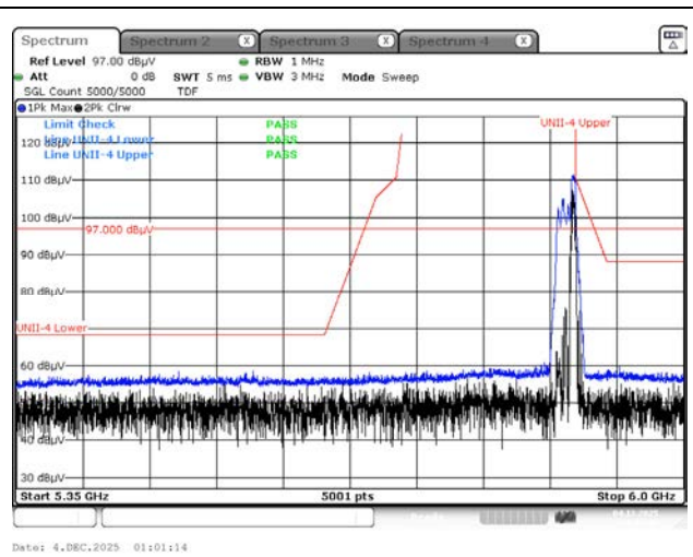
Peak result (802.11ax(HE20) Ch.177, 52T RU 40)
