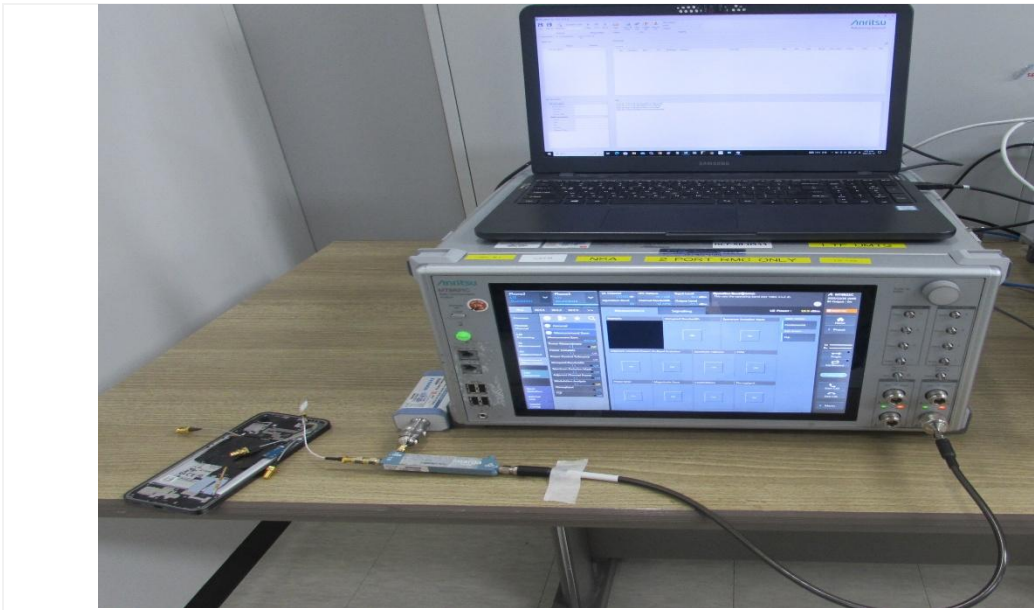
Test setup photo-1 TC01,05,09,10
