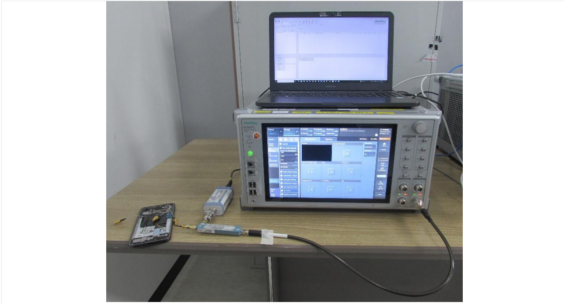
Test setup photo-3 TC03,04,07,08
