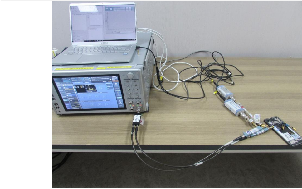
Test setup photo-7 TC15
