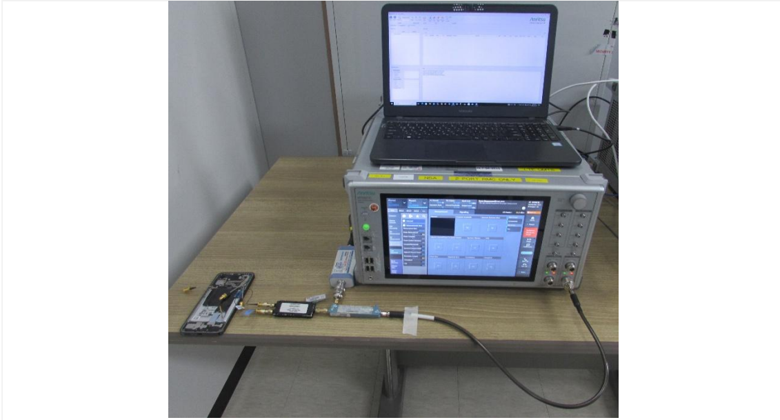
Test setup photo-5 TC12
