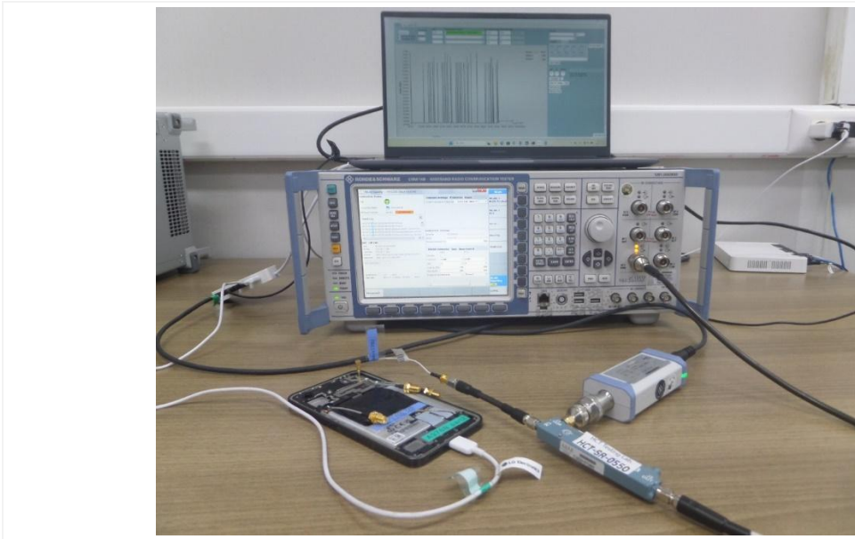
Test setup photo-9 W_TC02
