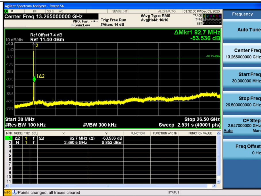
Spurious Emissions (30 MHz - 26.50 GHz) 8DPSK Ch. 78
