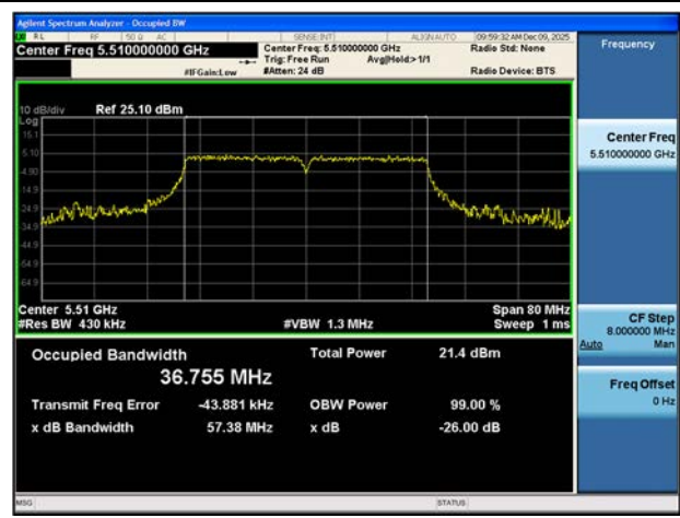
Bandwidth 40M, 802.11n(HT40) Ch.102
