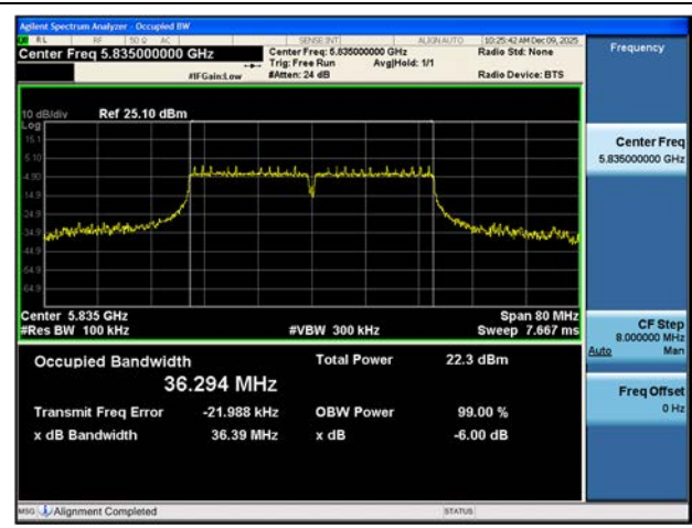
Bandwidth 40M, 802.11n(HT40) Ch.167
