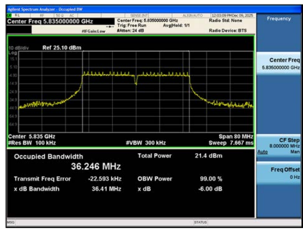
Bandwidth 40M, 802.11n(HT40) Ch.167
