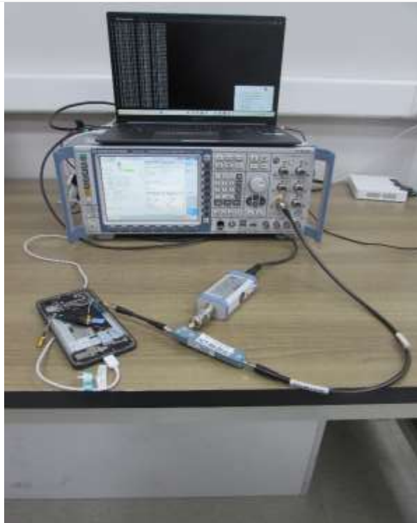
Test setup photo-7 W_TC01
