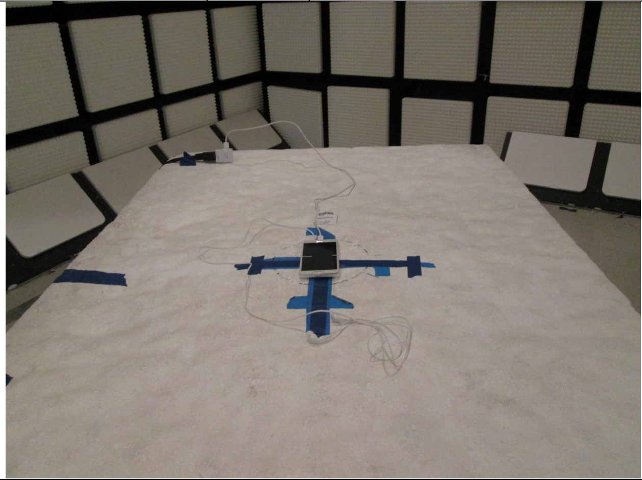
RADIATED FRONT=PHOTO (BELOW 1 GHz)
