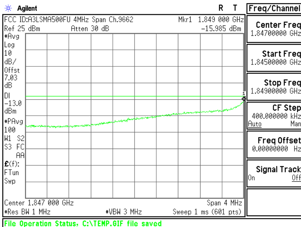
Plot 6-56. 4MHz Span Plot (PCS WCDMA Mode - Ch.9262(DL9662))
