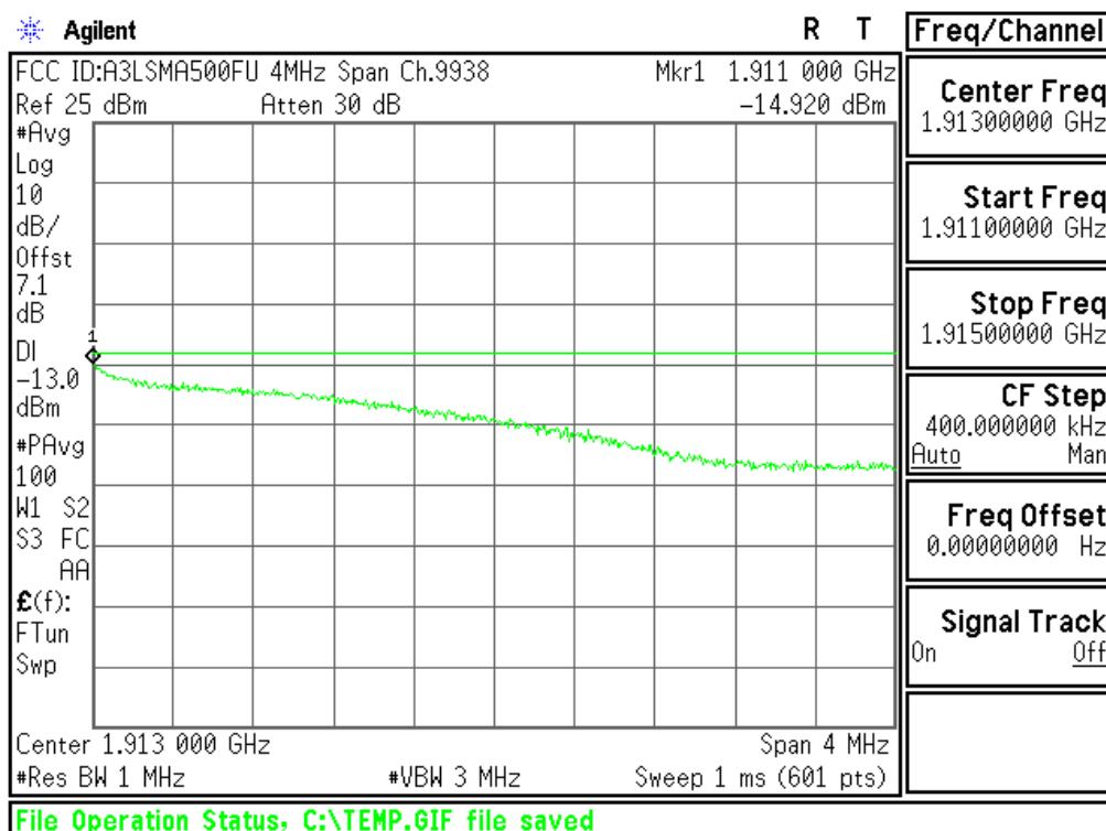
Plot 6-58. 4MHz Span Plot (PCS WCDMA Mode - Ch.9538(DL9938))
