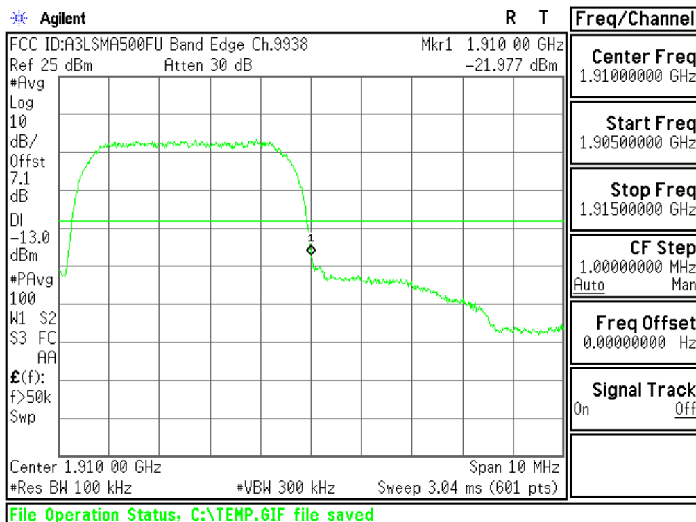
Plot 6-57. Band Edge Plot (PCS WCDMA Mode - Ch.9538(DL9938))
