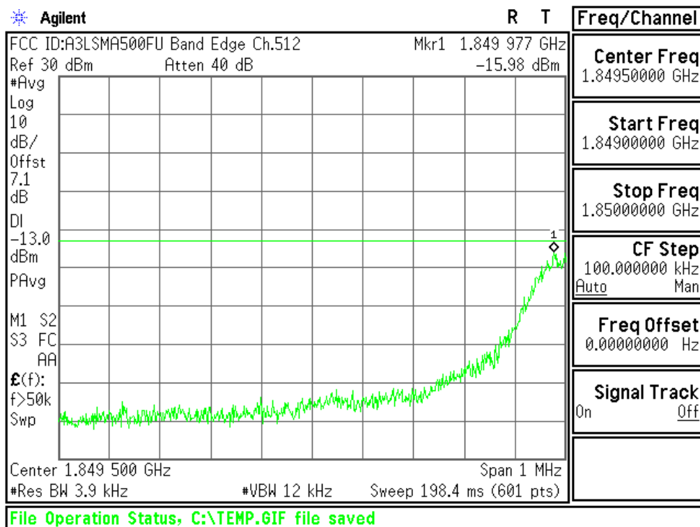
Plot 6-48. Band Edge Plot (PCS GSM Mode – Ch.512)
