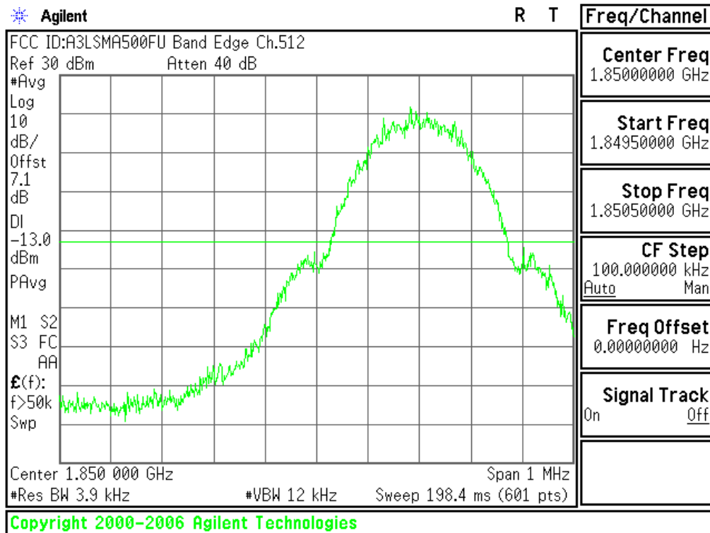
Plot 6-47. Band Edge Plot (PCS GSM Mode – Ch.512)
