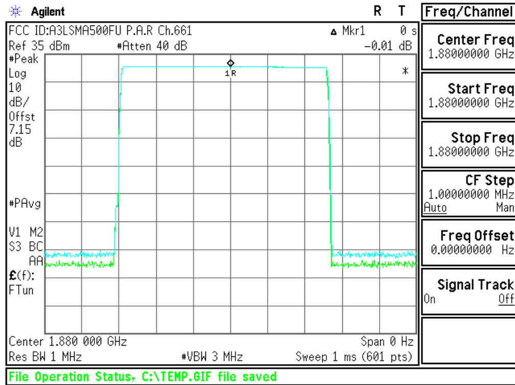
Plot 6-59. Peak-Average Ratio Plot (PCS GSM Mode - Ch.661)
