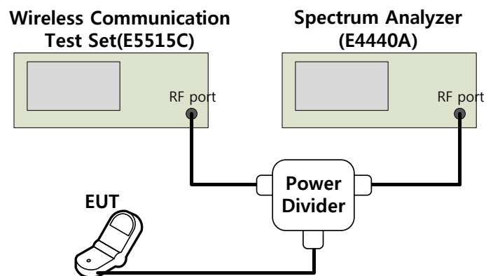
Figure 6-5. Test Instruments & Measurement Setup
