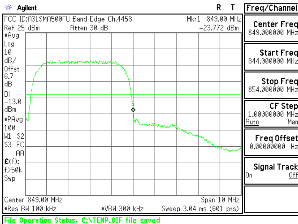
Plot 6-53. Band Edge Plot (Cellular WCDMA Mode - Ch.4233(DL4458))
