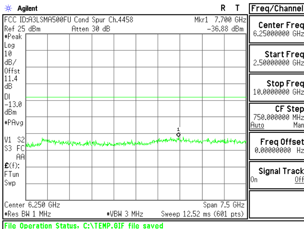
Plot 6-30. Conducted Spurious Plot (Cellular WCDMA Mode - Ch.4233(DL4458))
