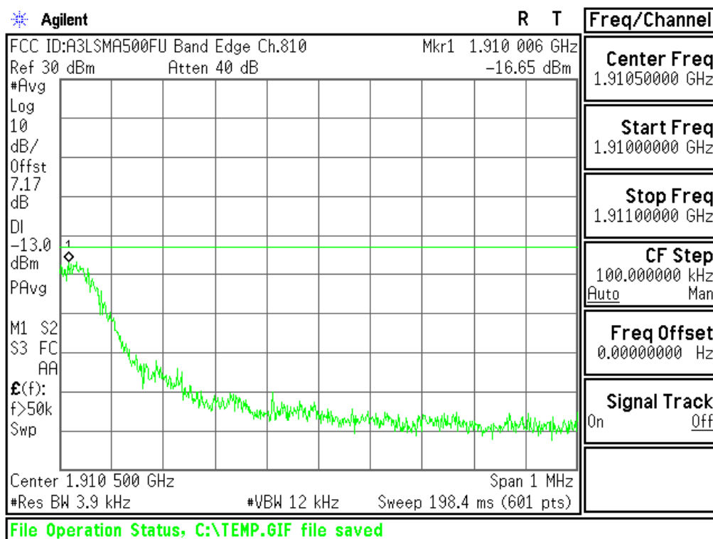
Plot 6-50. Band Edge Plot (PCS GSM Mode – Ch.810)
