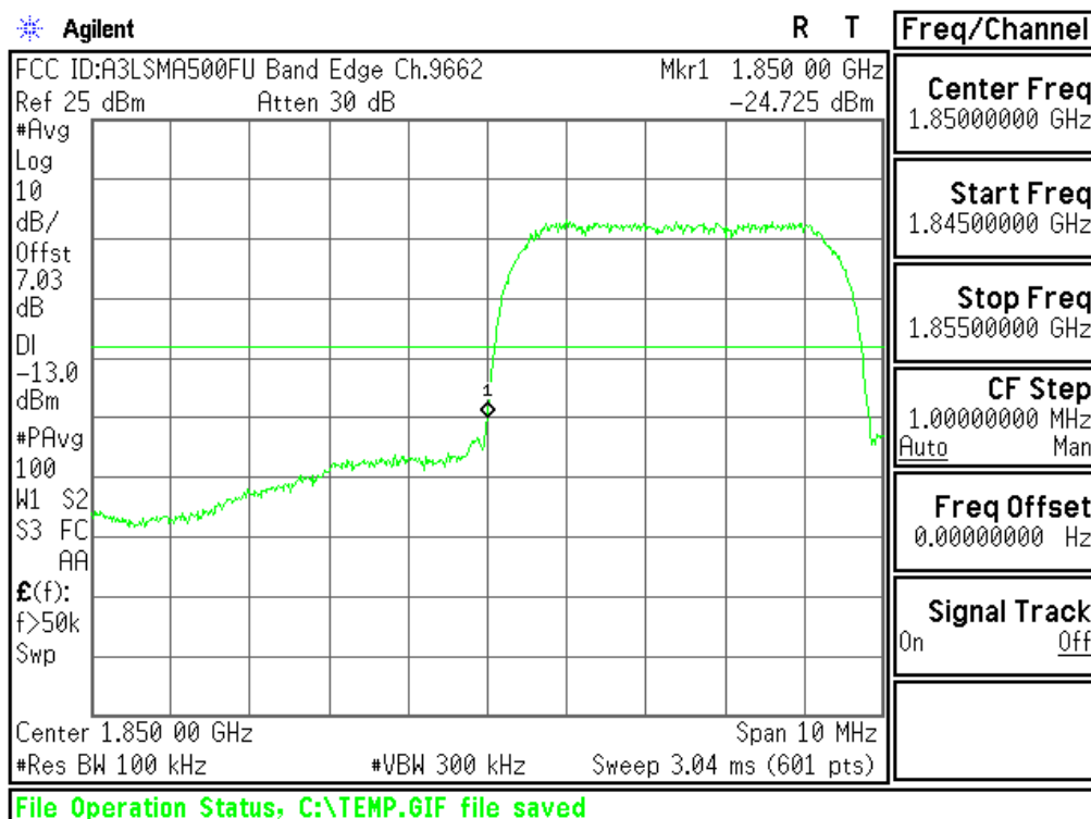
Plot 6-55. Band Edge Plot (PCS WCDMA Mode - Ch.9262(DL9662))
