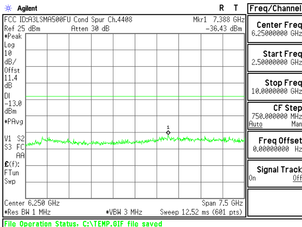
Plot 6-26. Conducted Spurious Plot (Cellular WCDMA Mode - Ch.4183(DL4408))
