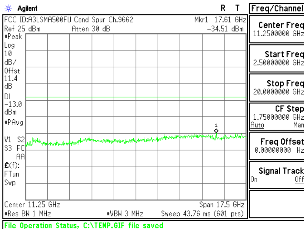
Plot 6-34. Conducted Spurious Plot (PCS WCDMA Mode - Ch.9262(DL9662))
