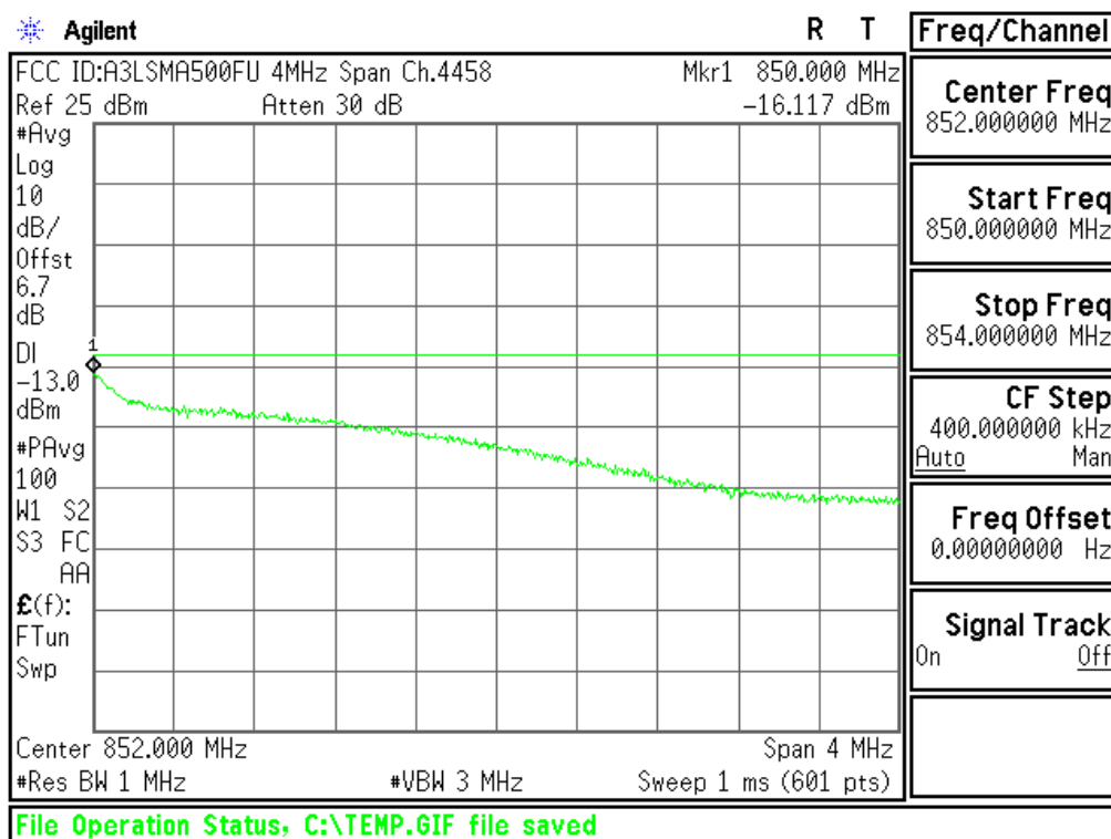
Plot 6-54. 4MHz Span Plot (Cellular WCDMA Mode - Ch.4233(DL4458))
