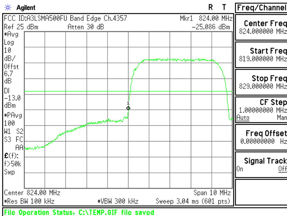
Plot 6-51. Band Edge Plot (Cellular WCDMA Mode - Ch.4132(DL4357))
