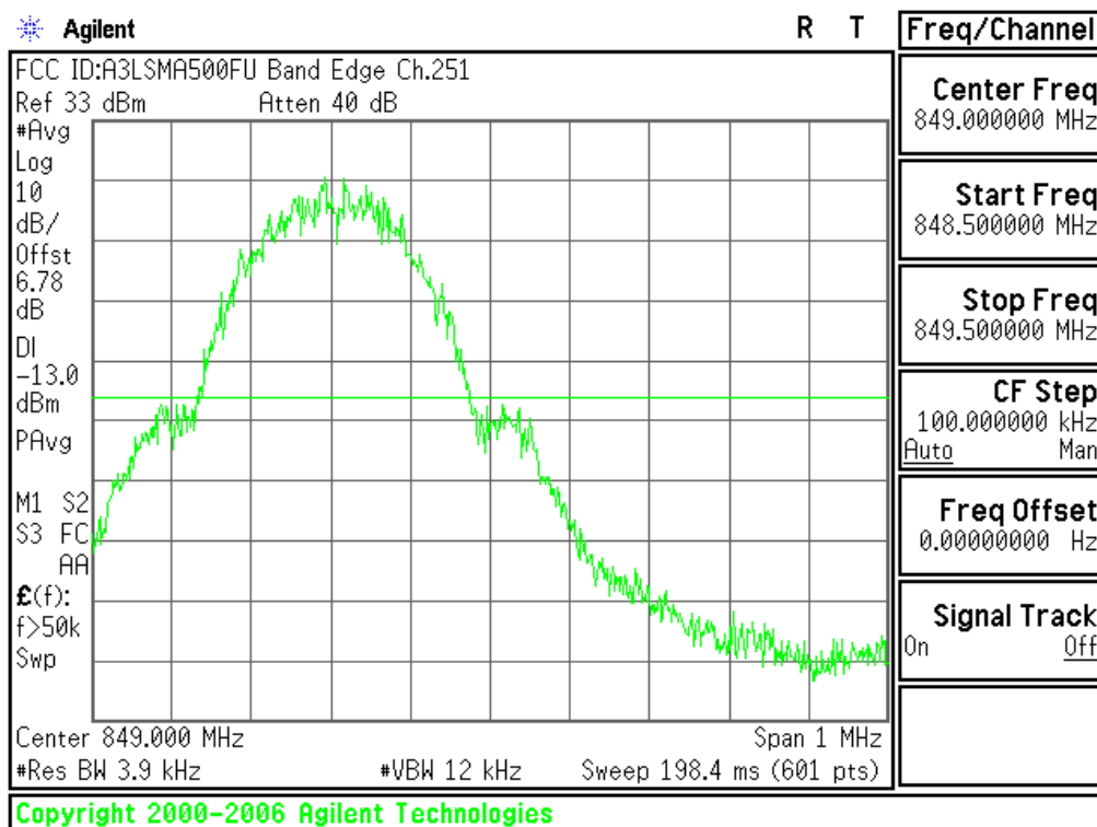
Plot 6-45. Band Edge Plot (Cellular GSM Mode – Ch.251)
