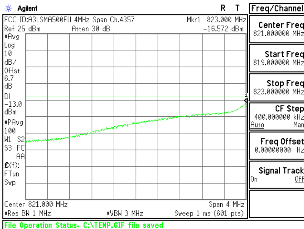
Plot 6-52. 4MHz Span Plot (Cellular WCDMA Mode - Ch.4132(DL4357))
