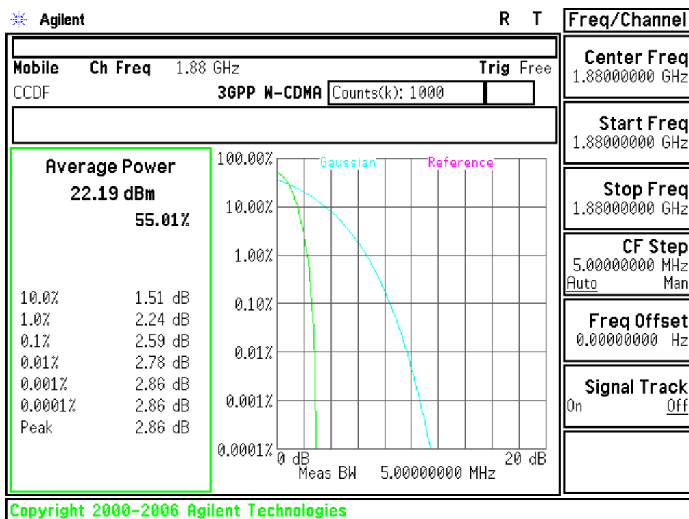
Plot 6-61. Peak-Average Ratio Plot (PCS WCDMA Mode - Ch.9400(DL9800))
