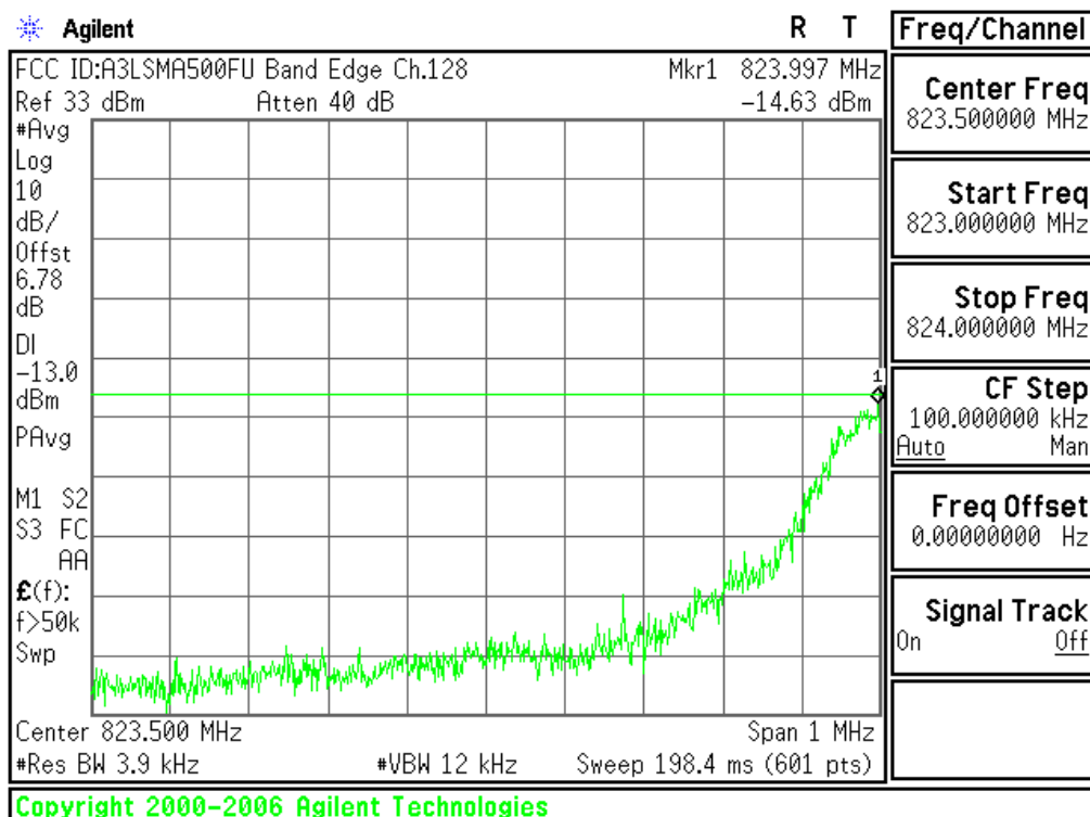
Plot 6-44. Band Edge Plot (Cellular GSM Mode – Ch.128)
