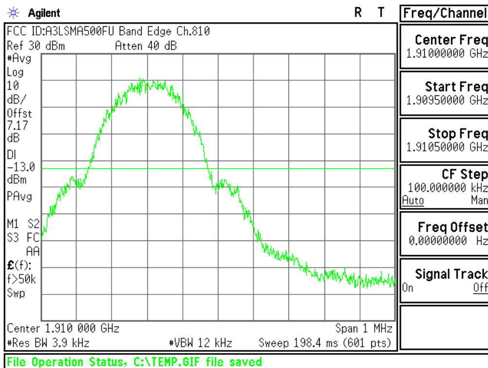
Plot 6-49. Band Edge Plot (PCS GSM Mode – Ch.810)
