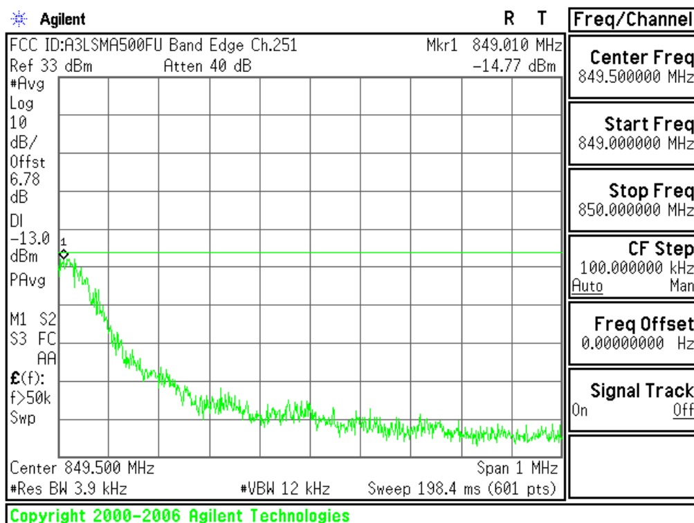
Plot 6-46. Band Edge Plot (Cellular GSM Mode – Ch.251)
