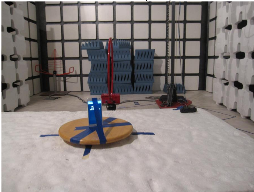
RADIATED EMISSIONS BELOW 30MHz (BACK)
