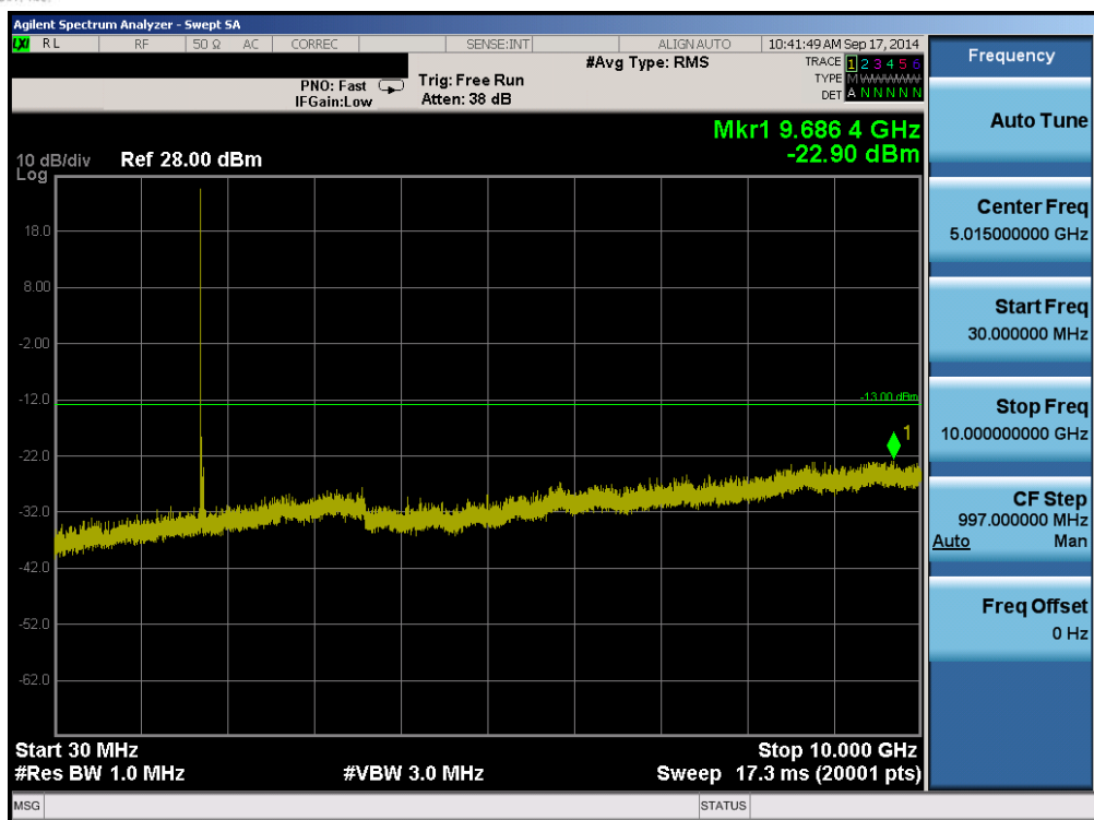
Plot 6-49. Conducted Spurious Plot (Band 4 – 3.0MHz QPSK – RB Size 1, RB Offset 0 – Low Channel)
