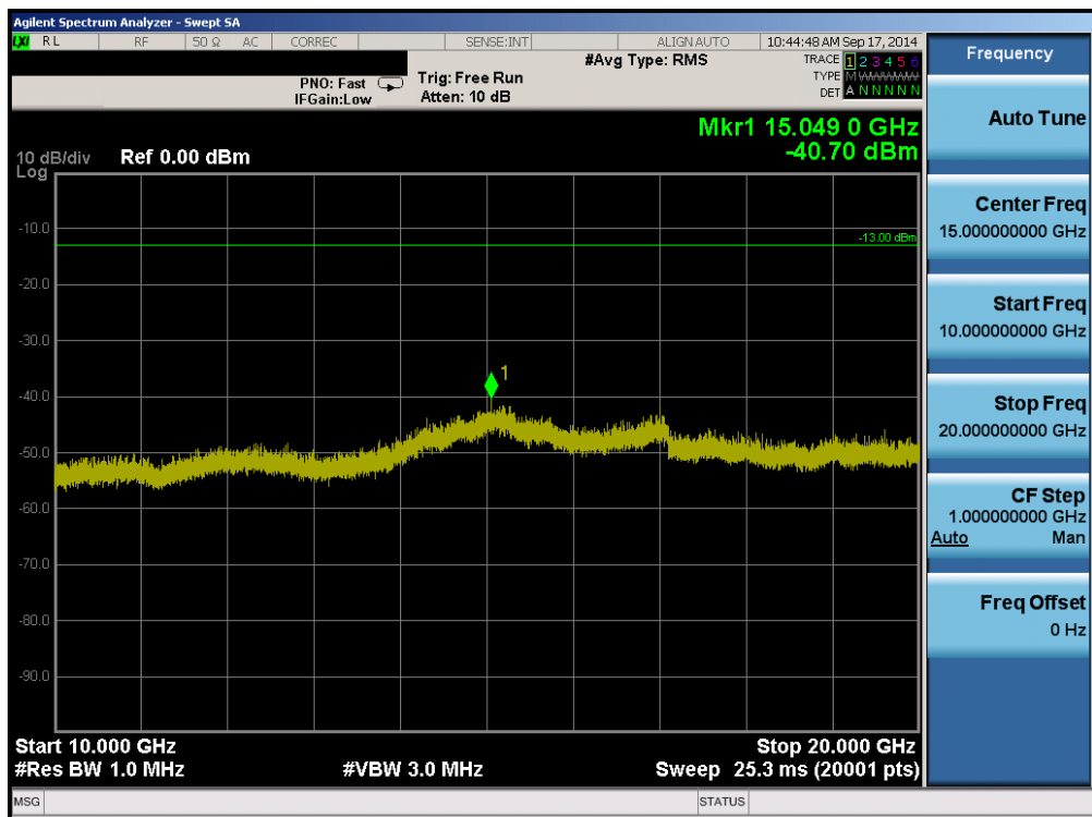
Plot 6-54. Conducted Spurious Plot (Band 4 – 3.0MHz QPSK – RB Size 1, RB Offset 0 – High Channel)
