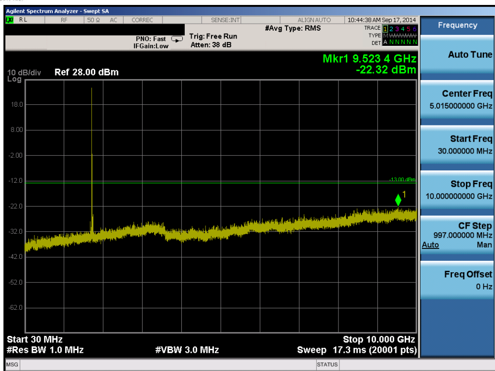
Plot 6-53. Conducted Spurious Plot (Band 4 – 3.0MHz QPSK – RB Size 1, RB Offset 0 – High Channel)
