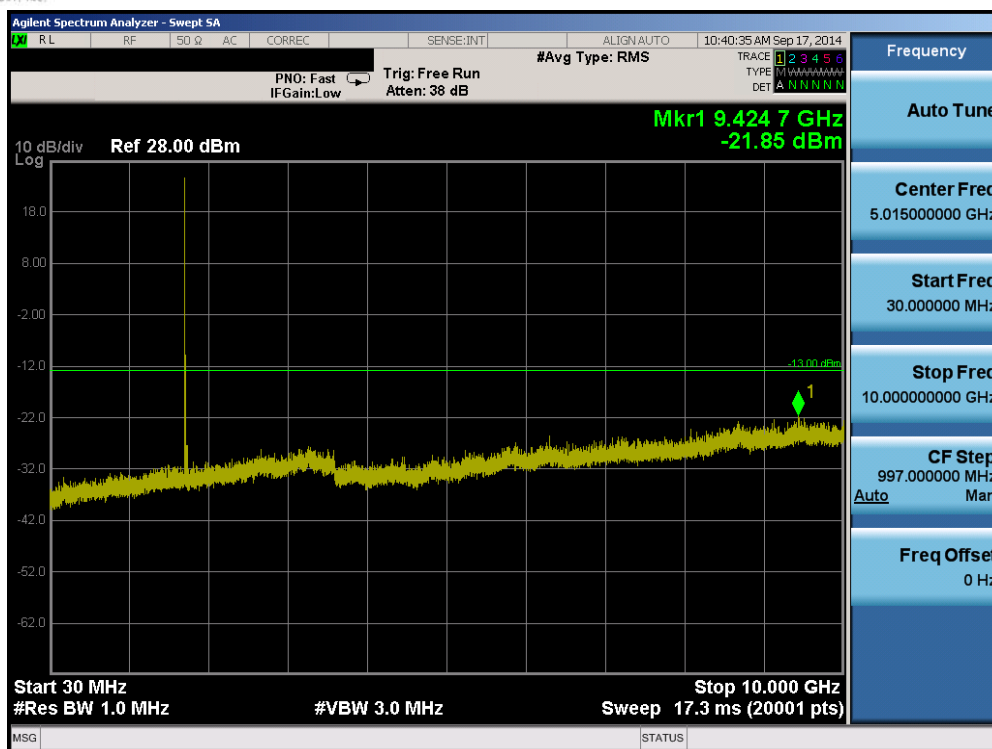
Plot 6-51. Conducted Spurious Plot (Band 4 – 3.0MHz QPSK – RB Size 1, RB Offset 0 – Mid Channel)
