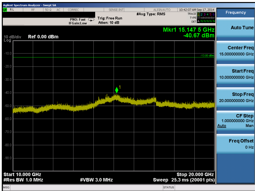
Plot 6-50. Conducted Spurious Plot (Band 4 – 3.0MHz QPSK – RB Size 1, RB Offset 0 – Low Channel)
