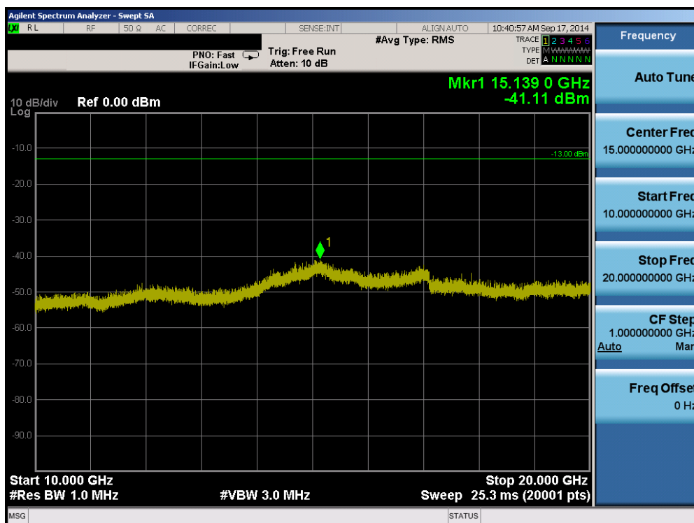
Plot 6-52. Conducted Spurious Plot (Band 4 – 3.0MHz QPSK – RB Size 1, RB Offset 0 – Mid Channel)
