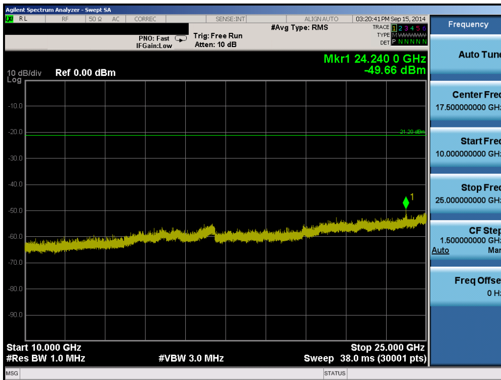
Plot 6-48. Conducted Spurious Plot (802.11b – Ch. 1)
