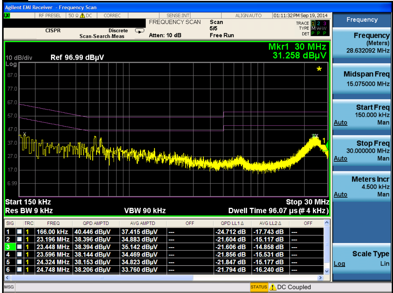
Plot 6-64. Line Conducted Plot with 802.11b (N)
