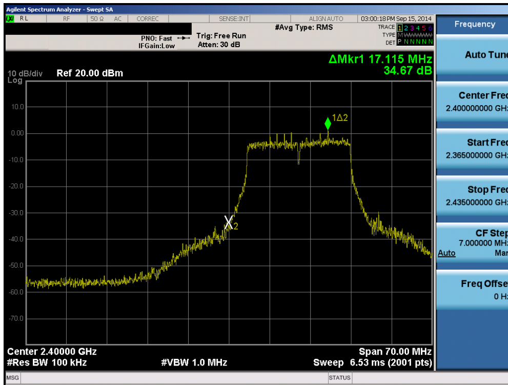
Plot 6-39. Band Edge Plot (802.11n (2.4GHz) – Ch. 1)
