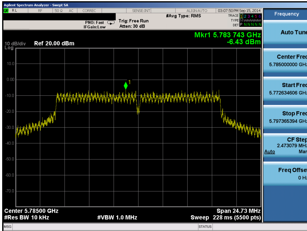
Plot 6-28. Power Spectral Density Plot (802.11a – Ch. 157)
