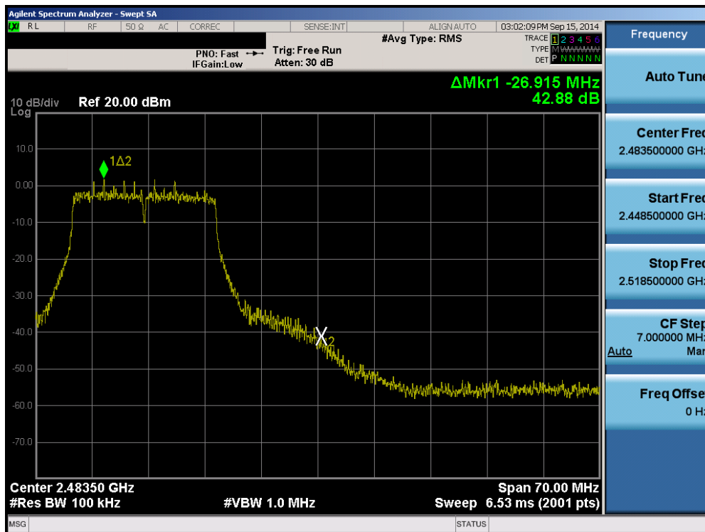
Plot 6-40. Band Edge Plot (802.11n (2.4GHz) – Ch. 11)
