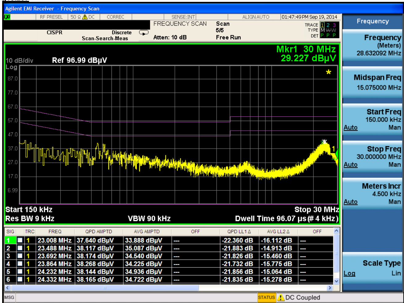
Plot 6-66. Line Conducted Plot with 802.11a (N)
