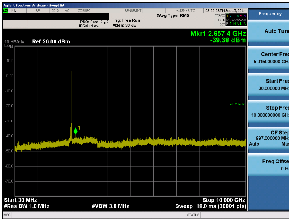
Plot 6-51. Conducted Spurious Plot (802.11b – Ch. 11)
