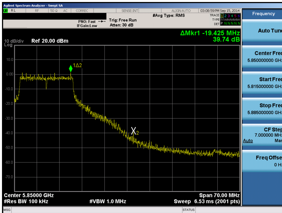
Plot 6-42. Band Edge Plot (802.11a – Ch. 165)
