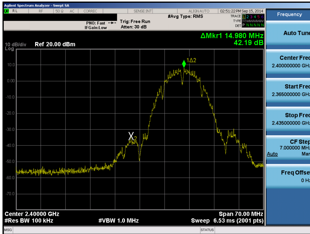
Plot 6-35. Band Edge Plot (802.11b – Ch. 1)
