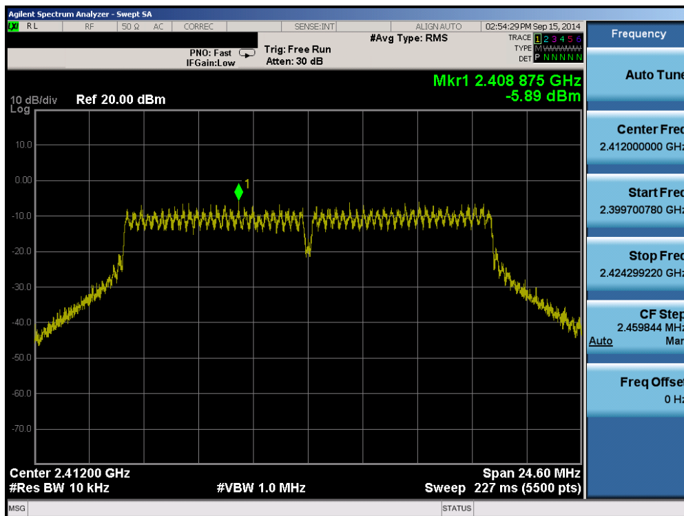
Plot 6-21. Power Spectral Density Plot (802.11g – Ch. 1)
