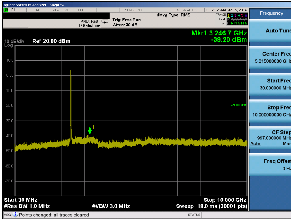
Plot 6-49. Conducted Spurious Plot (802.11b – Ch. 6)
