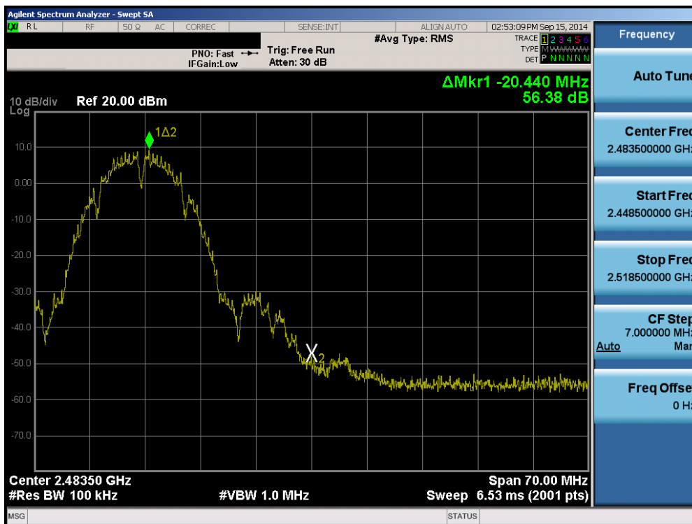
Plot 6-36. Band Edge Plot (802.11b – Ch. 11)
