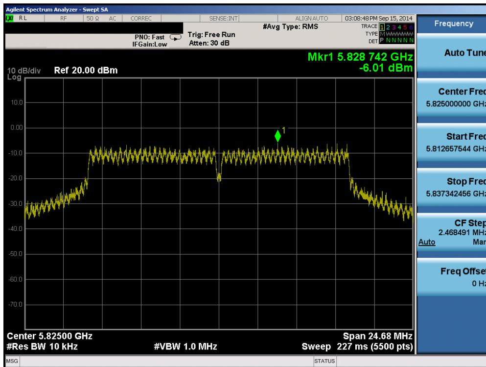
Plot 6-29. Power Spectral Density Plot (802.11a – Ch. 165)
