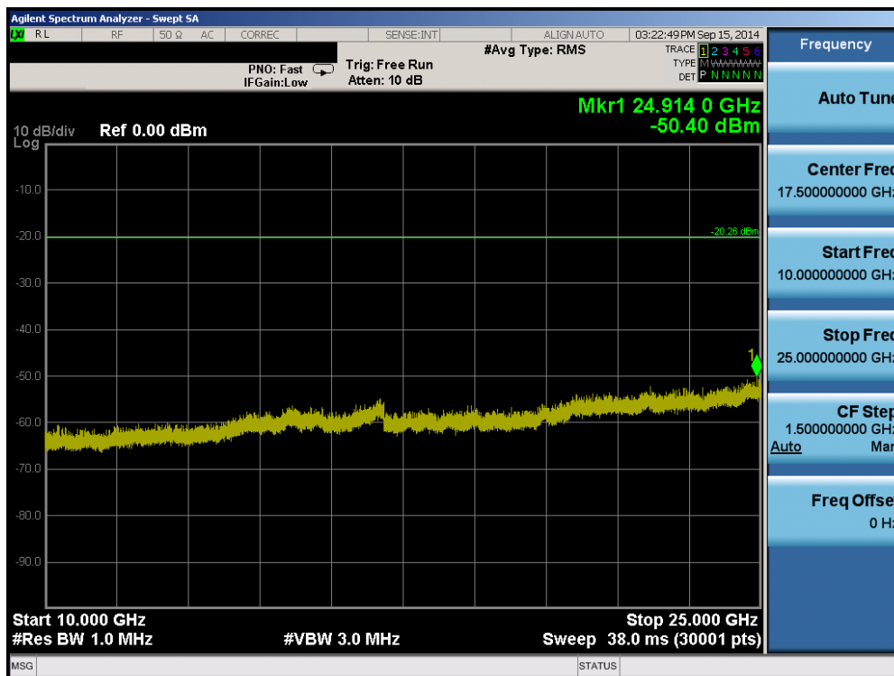
Plot 6-52. Conducted Spurious Plot (802.11b – Ch. 11)
