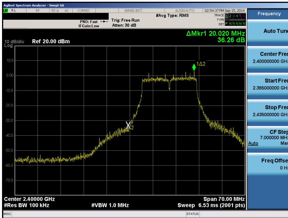
Plot 6-37. Band Edge Plot (802.11g– Ch. 1)
