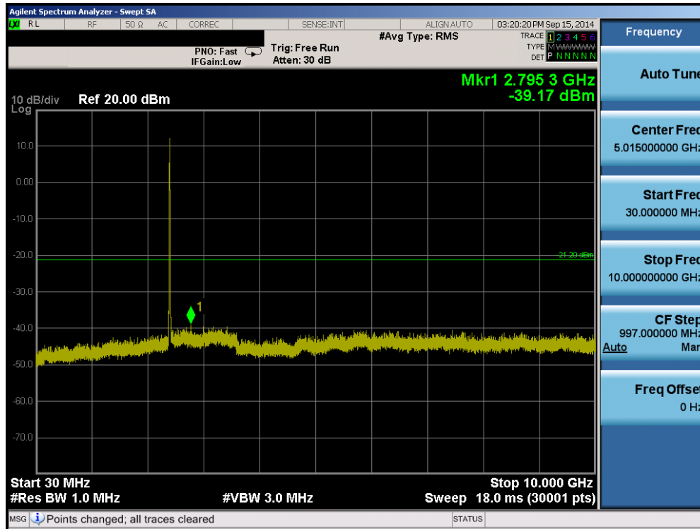
Plot 6-47. Conducted Spurious Plot (802.11b – Ch. 1)
