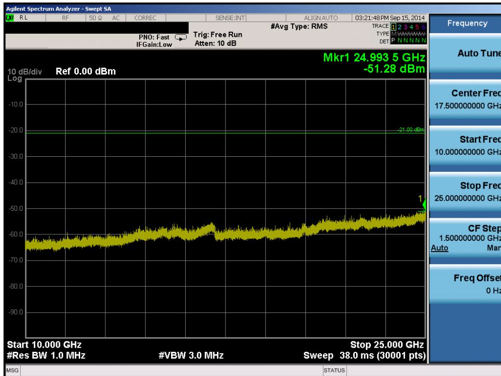
Plot 6-50. Conducted Spurious Plot (802.11b – Ch. 6)
