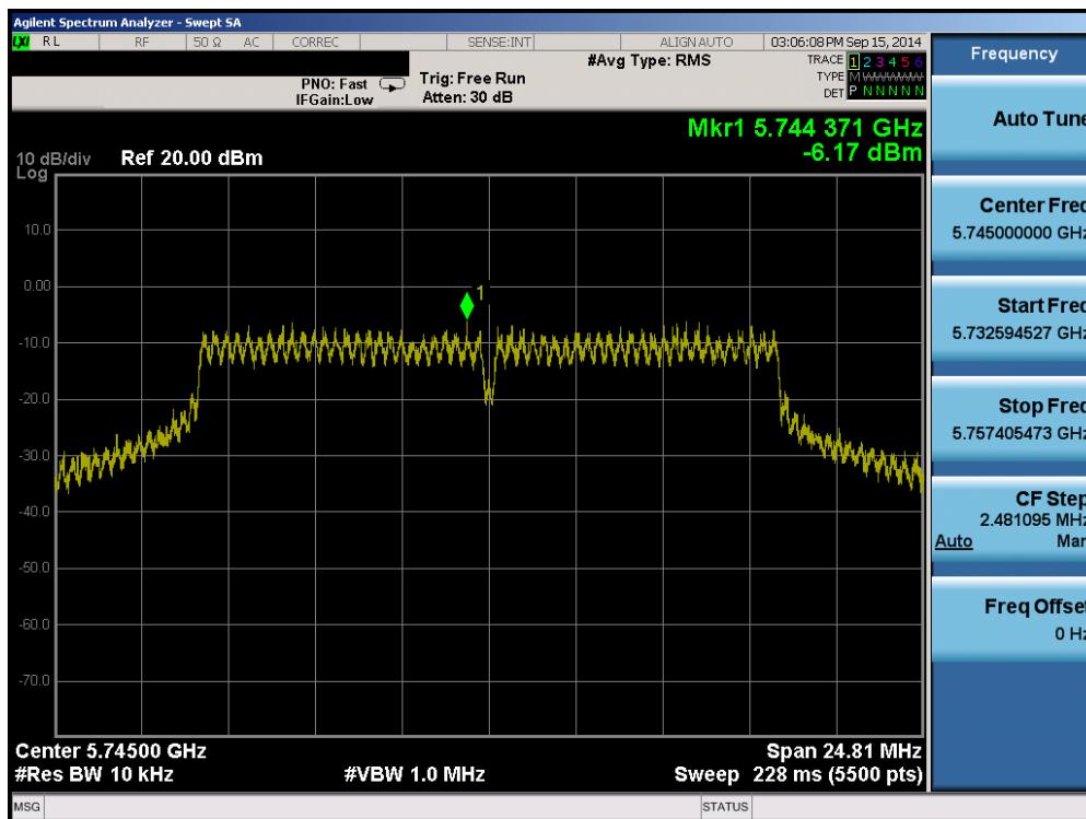
Plot 6-27. Power Spectral Density Plot (802.11a – Ch. 149)
