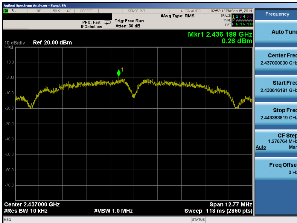
Plot 6-19. Power Spectral Density Plot (802.11b – Ch. 6)
