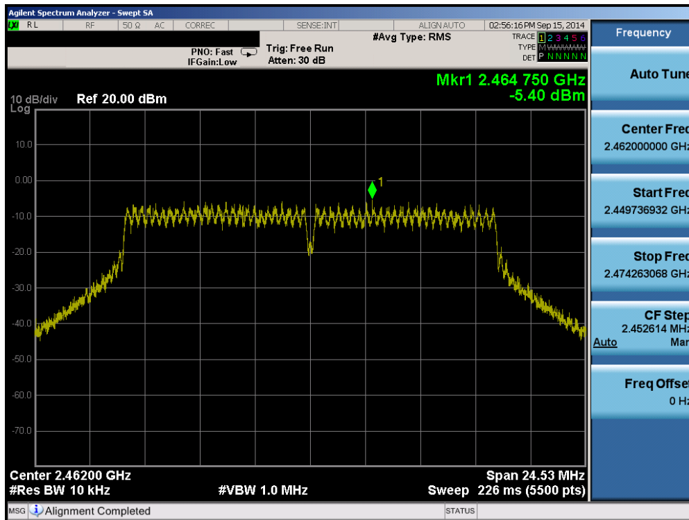
Plot 6-23. Power Spectral Density Plot (802.11g – Ch. 11)
