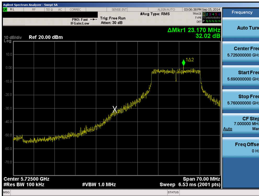
Plot 6-41. Band Edge Plot (802.11a – Ch. 149)
