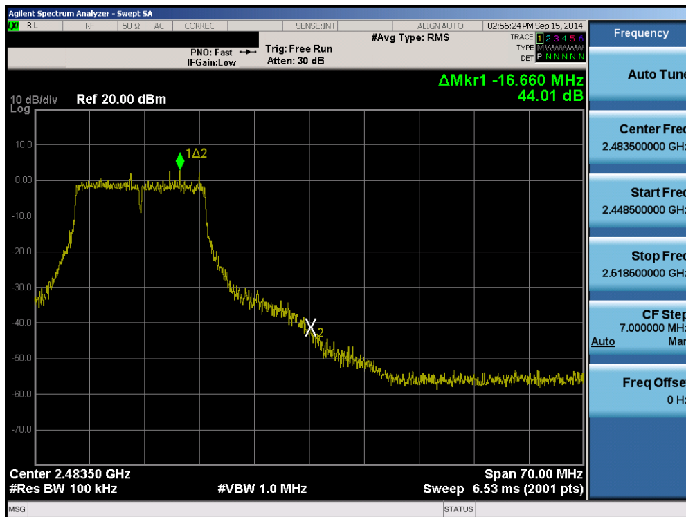
Plot 6-38. Band Edge Plot (802.11g – Ch. 11)
