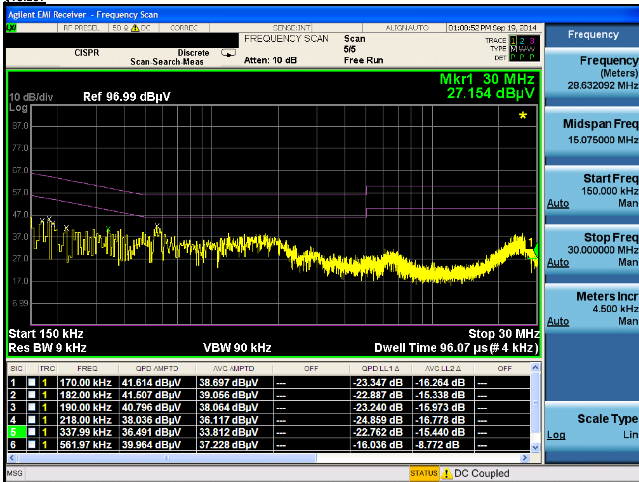
Plot 6-63. Line Conducted Plot with 802.11b (L1)
