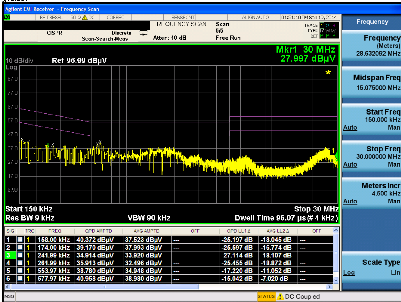
Plot 6-65. Line Conducted Plot with 802.11a (L1)
