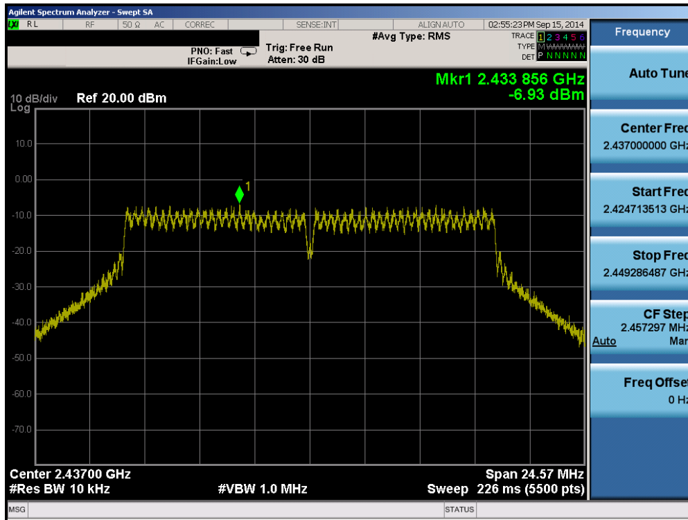
Plot 6-22. Power Spectral Density Plot (802.11g – Ch. 6)
