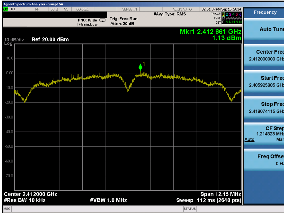
Plot 6-18. Power Spectral Density Plot (802.11b – Ch. 1)
