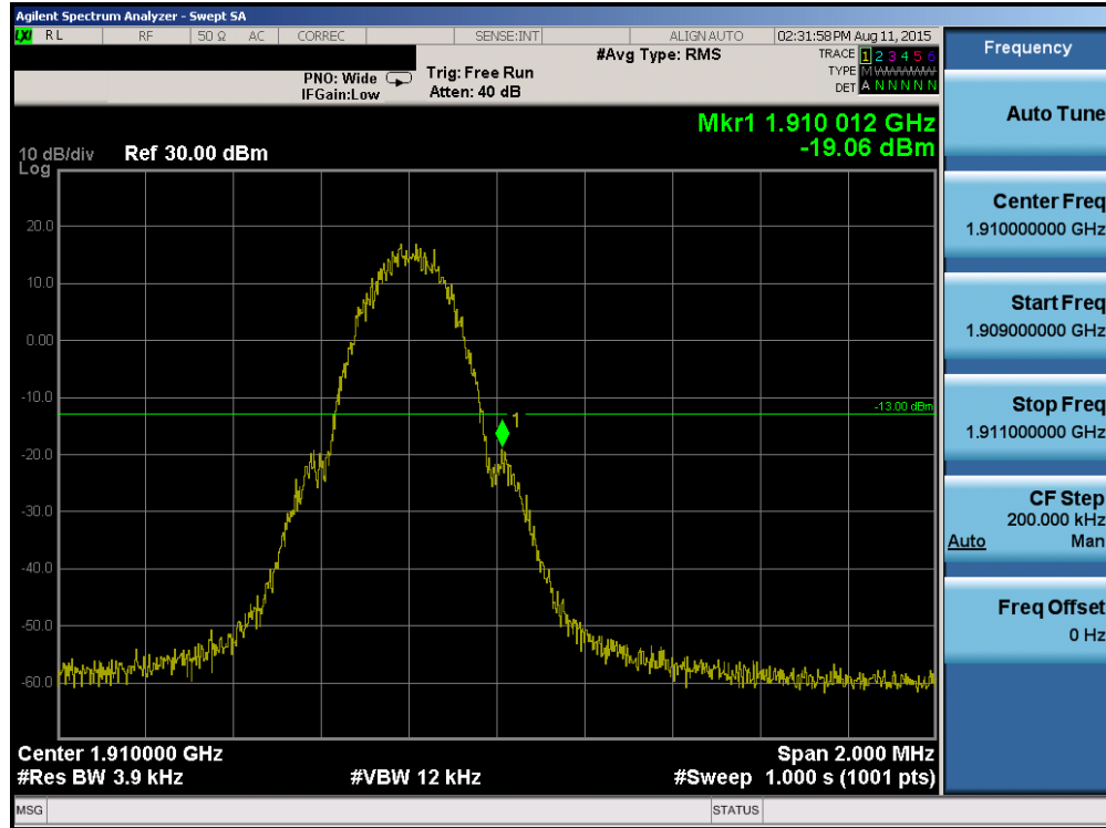
Plot 7-47. Band Edge Plot (PCS GSM Mode – Ch. 810)
