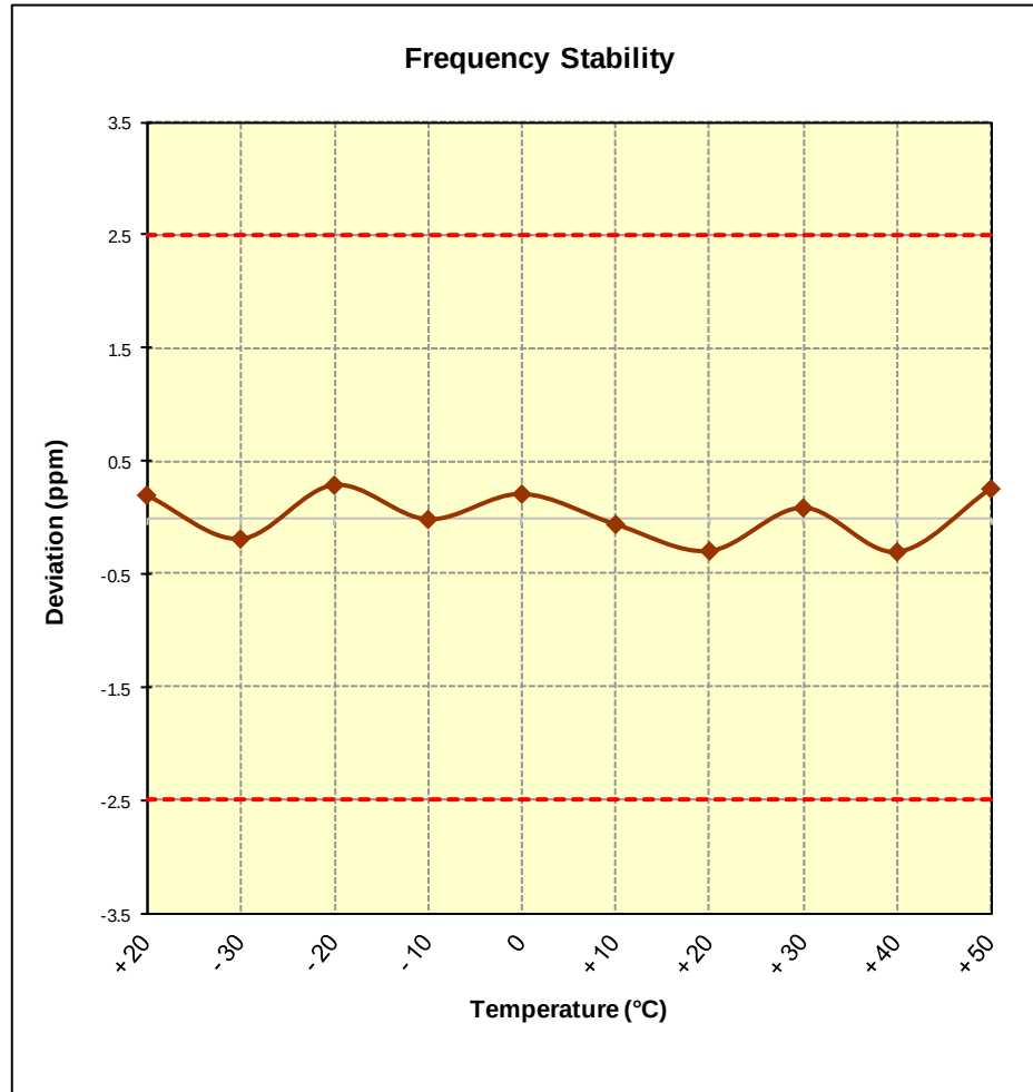
Figure 7-7. Frequency Stability Graph (Cellular GSM Mode – Ch. 190)
