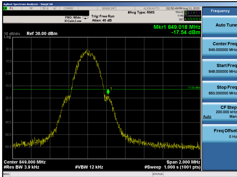
Plot 7-44. Band Edge Plot (Cellular GSM Mode – Ch. 251)
