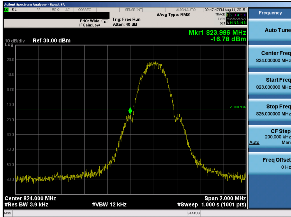
Plot 7-43. Band Edge Plot (Cellular GSM Mode – Ch. 128)
