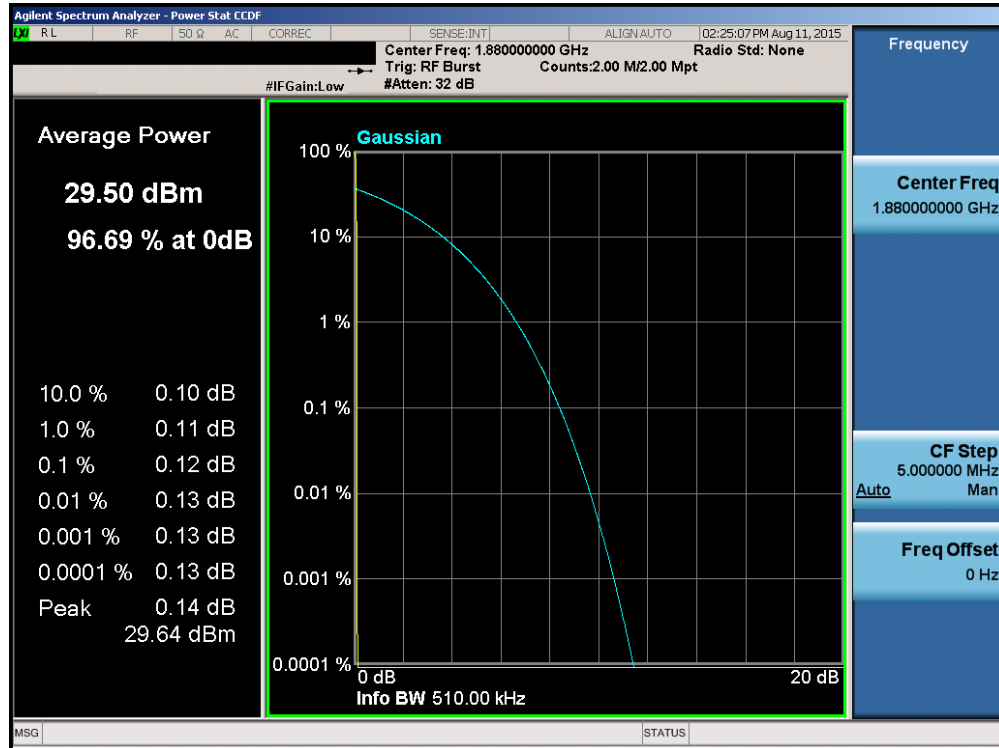
Plot 7-55. Peak-Average Ratio Plot (PCS GSM Mode – Ch. 661)
