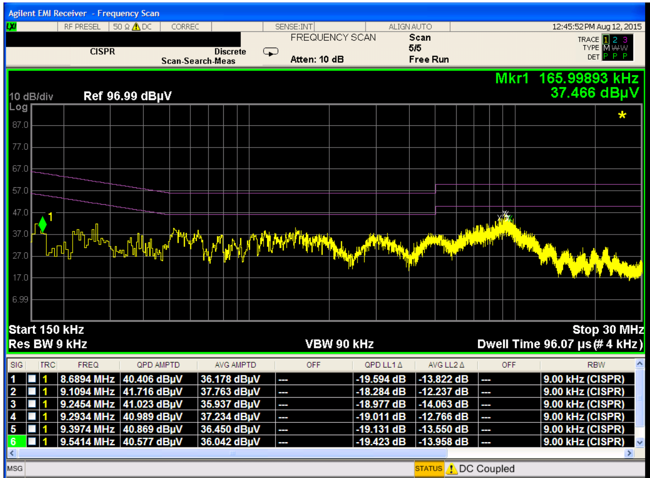
Plot 7-7. Line-Conducted Test Plot (N)
