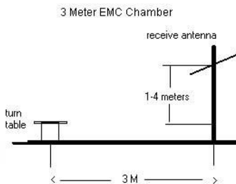
Figure 7-6. Test Instrument & Measurement Setup
