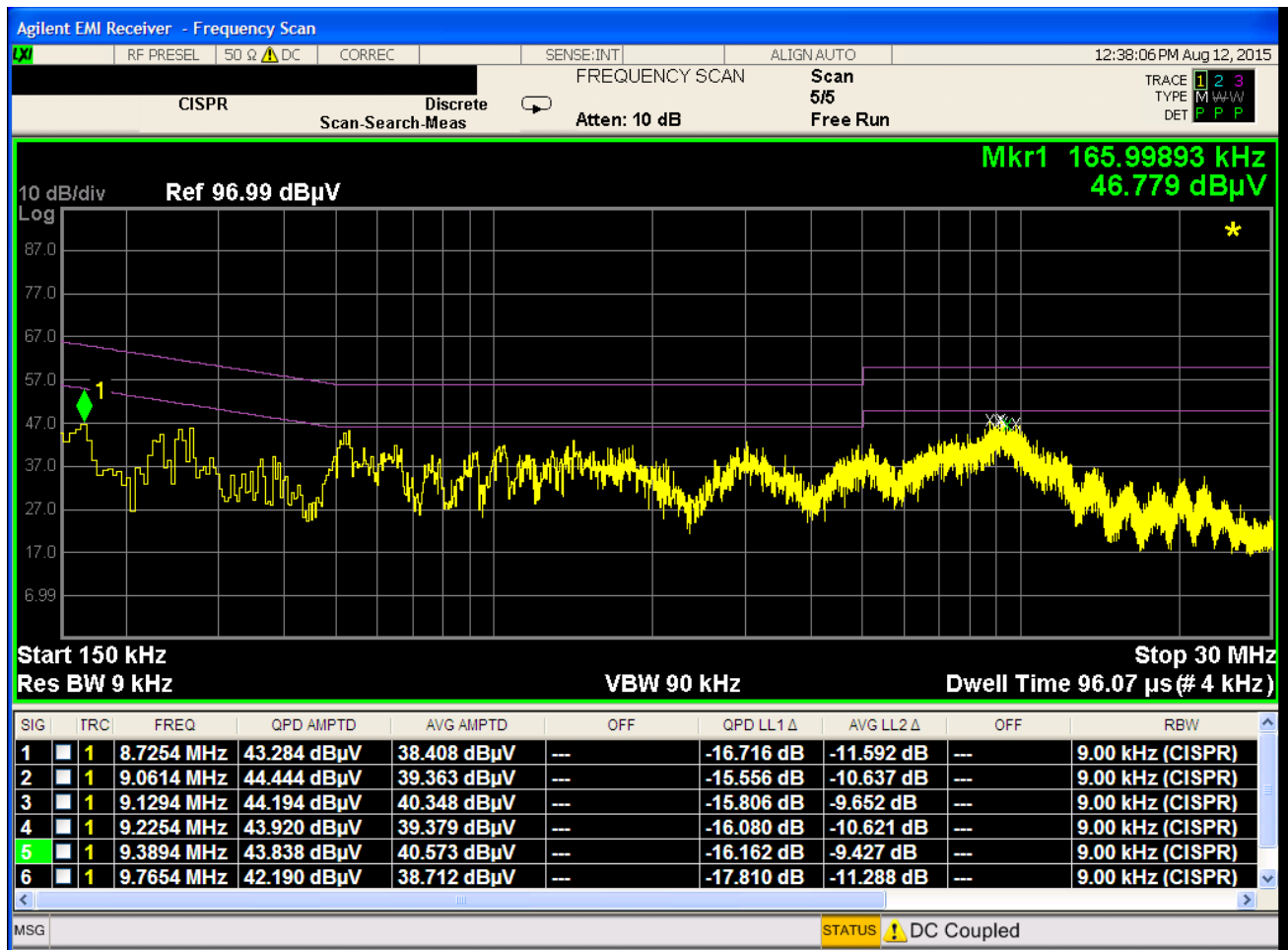
Plot 7-54. Line-Conducted Test Plot (L1)
