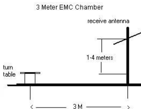
Figure 7-8. Test Instrument & Measurement Setup
