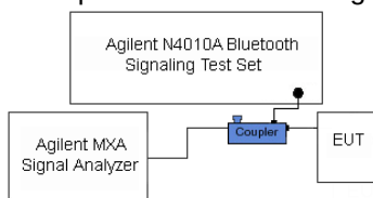
Figure 7-1. Test Instrument & Measurement Setup
