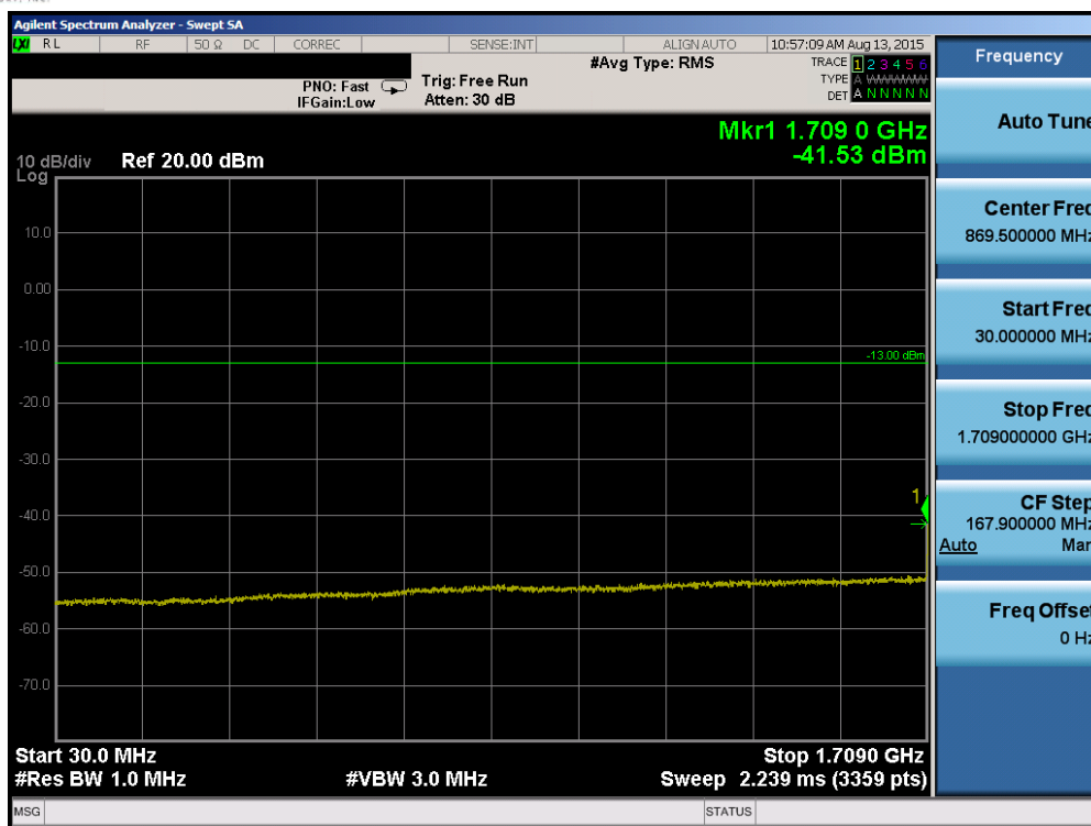
Plot 7-55. Conducted Spurious Plot (Band 4 – 5.0MHz QPSK – RB Size 1, RB Offset 0 – Low Channel)
