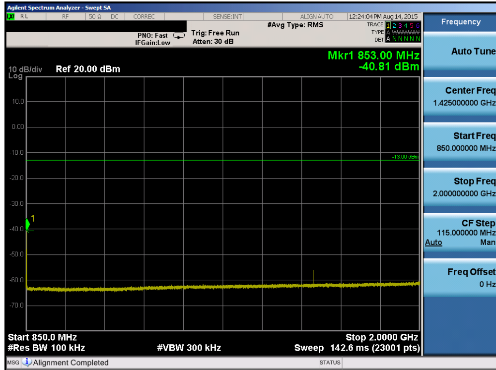
Plot 7-53. Conducted Spurious Plot (Band 5 – 5.0MHz QPSK – RB Size 1, RB Offset 0 – High Channel)
