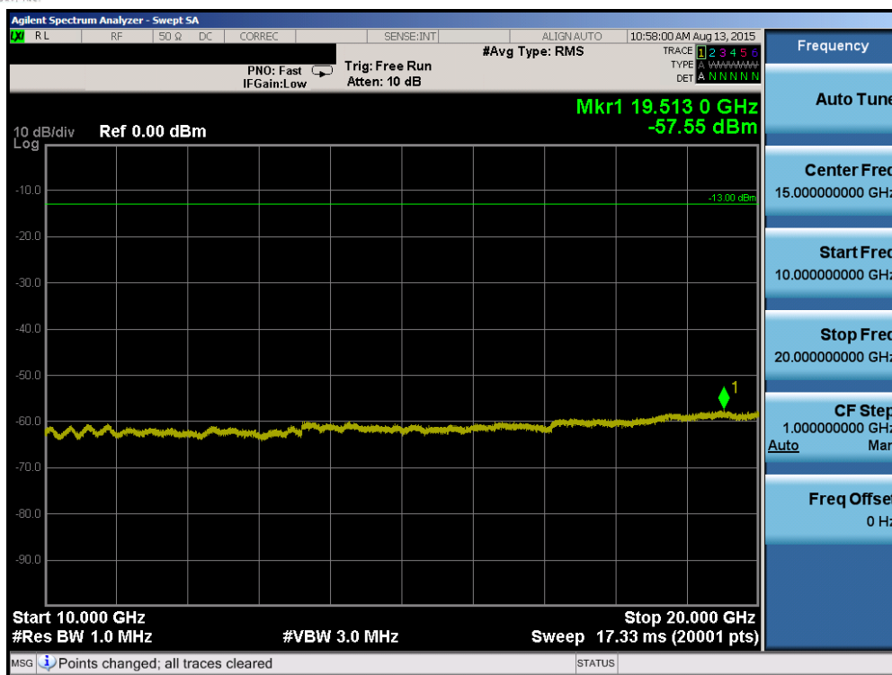
Plot 7-57. Conducted Spurious Plot (Band 4 – 5.0MHz QPSK – RB Size 1, RB Offset 0 – Low Channel)
