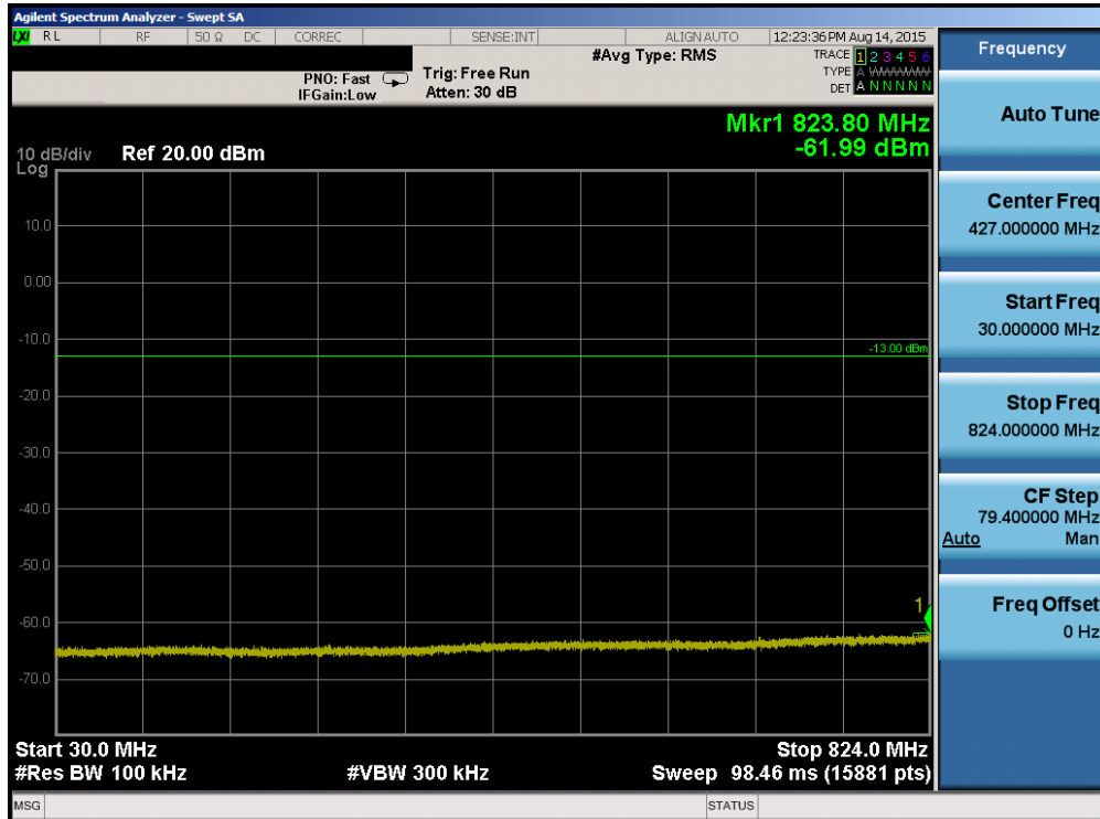
Plot 7-52. Conducted Spurious Plot (Band 5 – 5.0MHz QPSK – RB Size 1, RB Offset 0 – High Channel)
