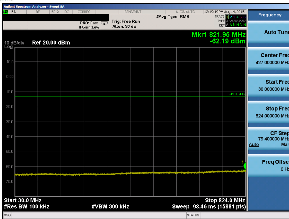
Plot 7-49. Conducted Spurious Plot (Band 5 – 5.0MHz QPSK – RB Size 1, RB Offset 0 – Mid Channel)
