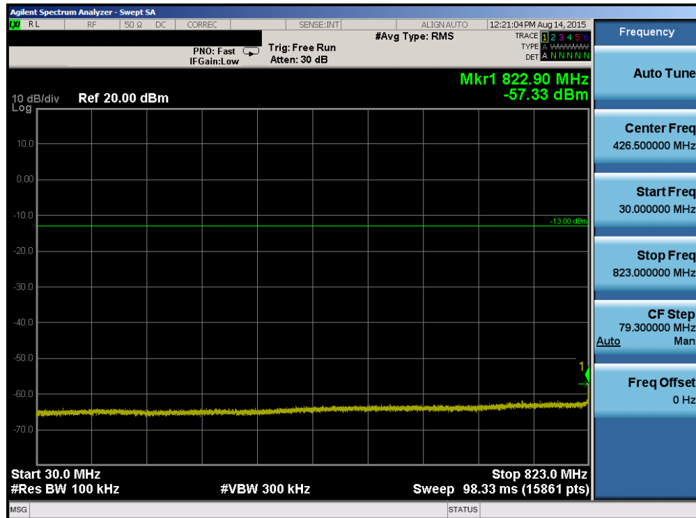
Plot 7-46. Conducted Spurious Plot (Band 5 – 5.0MHz QPSK – RB Size 1, RB Offset 0 – Low Channel)
