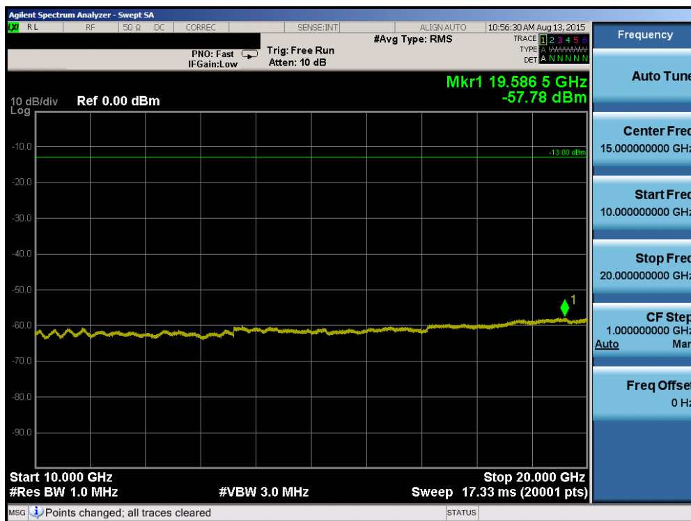
Plot 7-60. Conducted Spurious Plot (Band 4 – 5.0MHz QPSK – RB Size 1, RB Offset 0 – Mid Channel)
