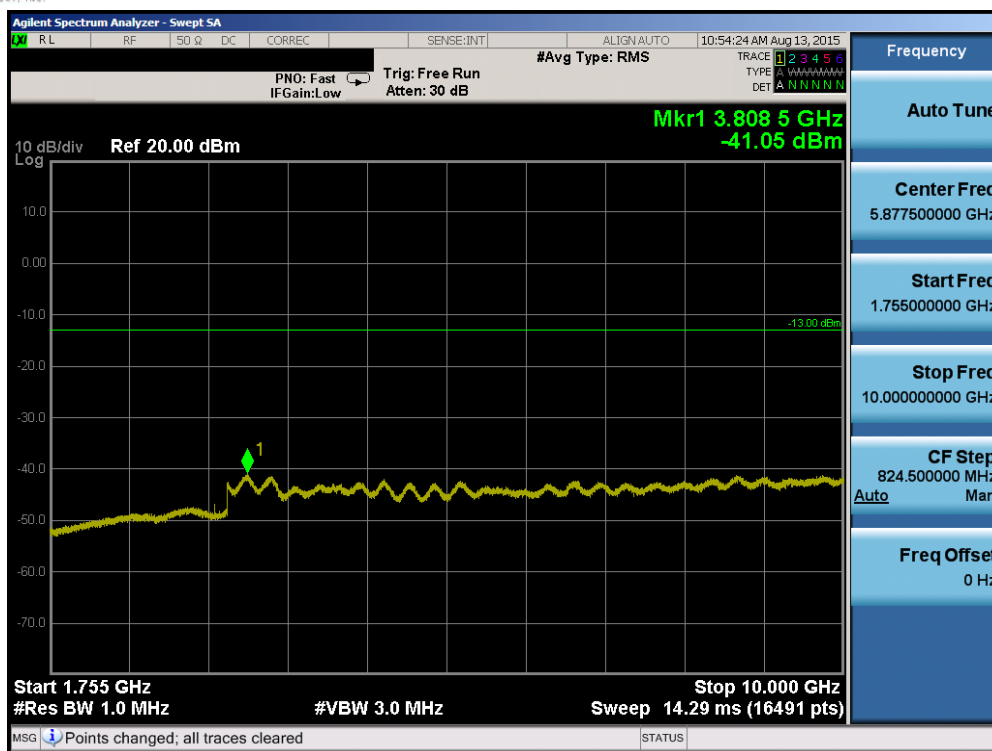
Plot 7-59. Conducted Spurious Plot (Band 4 – 5.0MHz QPSK – RB Size 1, RB Offset 0 – Mid Channel)
