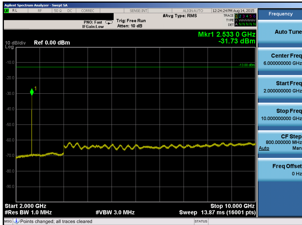
Plot 7-54. Conducted Spurious Plot (Band 5 – 5.0MHz QPSK – RB Size 1, RB Offset 0 – High Channel)
