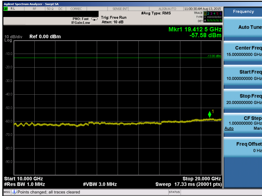
Plot 7-63. Conducted Spurious Plot (Band 4 – 5.0MHz QPSK – RB Size 1, RB Offset 0 – High Channel)
