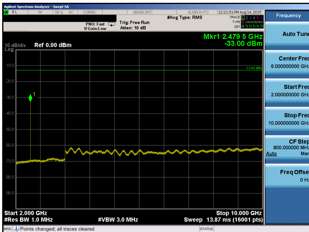
Plot 7-48. Conducted Spurious Plot (Band 5 – 5.0MHz QPSK – RB Size 1, RB Offset 0 – Low Channel)
