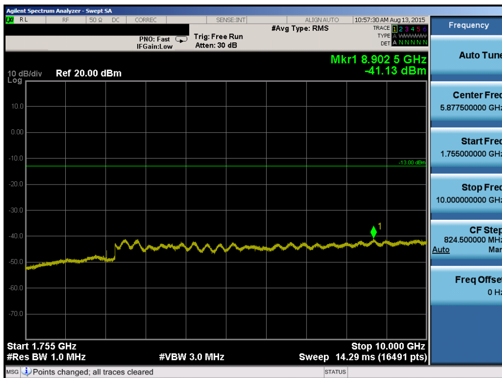
Plot 7-56. Conducted Spurious Plot (Band 4 – 5.0MHz QPSK – RB Size 1, RB Offset 0 – Low Channel)
