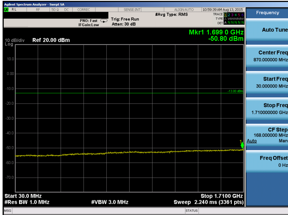
Plot 7-61. Conducted Spurious Plot (Band 4 – 5.0MHz QPSK – RB Size 1, RB Offset 0 – High Channel)
