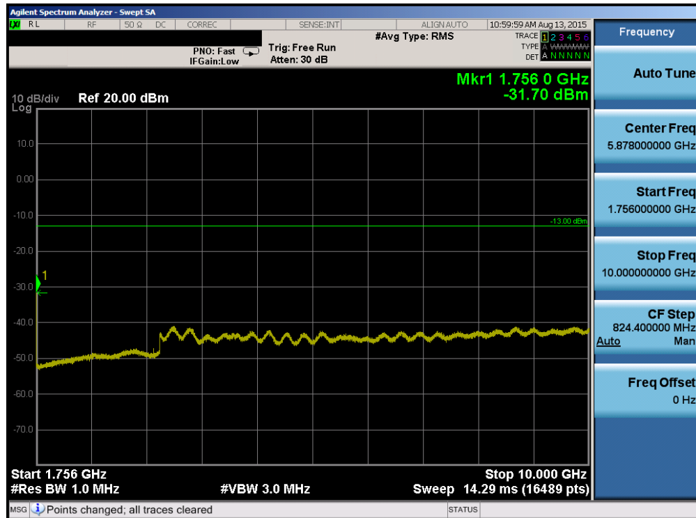
Plot 7-62. Conducted Spurious Plot (Band 4 – 5.0MHz QPSK – RB Size 1, RB Offset 0 – High Channel)
