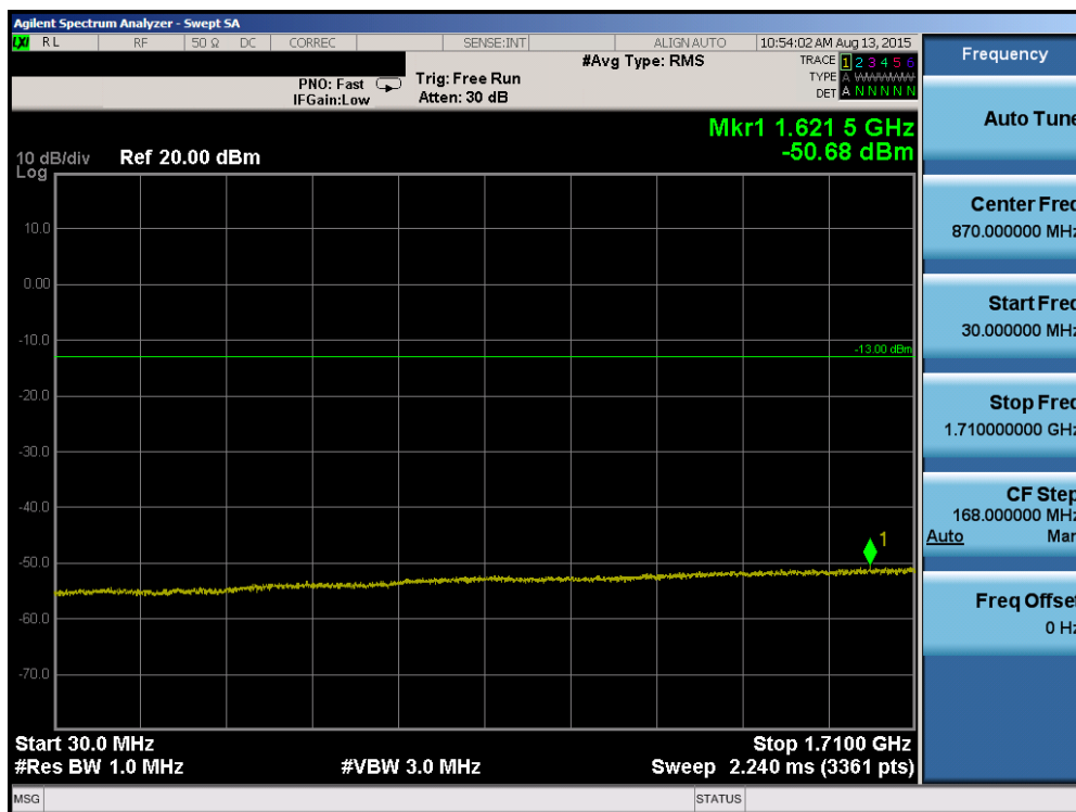
Plot 7-58. Conducted Spurious Plot (Band 4 – 5.0MHz QPSK – RB Size 1, RB Offset 0 – Mid Channel)
