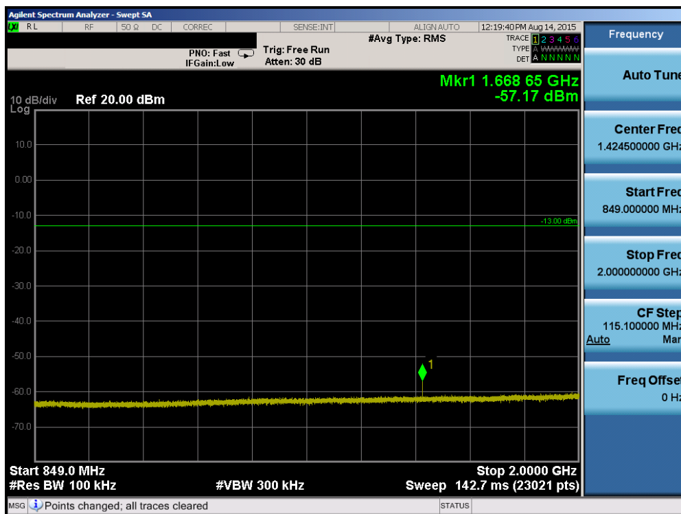
Plot 7-50. Conducted Spurious Plot (Band 5 – 5.0MHz QPSK – RB Size 1, RB Offset 0 – Mid Channel)
