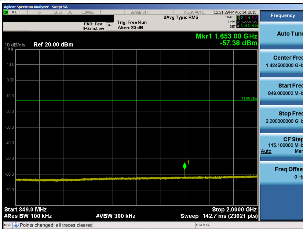
Plot 7-47. Conducted Spurious Plot (Band 5 – 5.0MHz QPSK – RB Size 1, RB Offset 0 – Low Channel)
