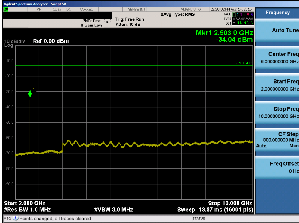
Plot 7-51. Conducted Spurious Plot (Band 5 – 5.0MHz QPSK – RB Size 1, RB Offset 0 – Mid Channel)
