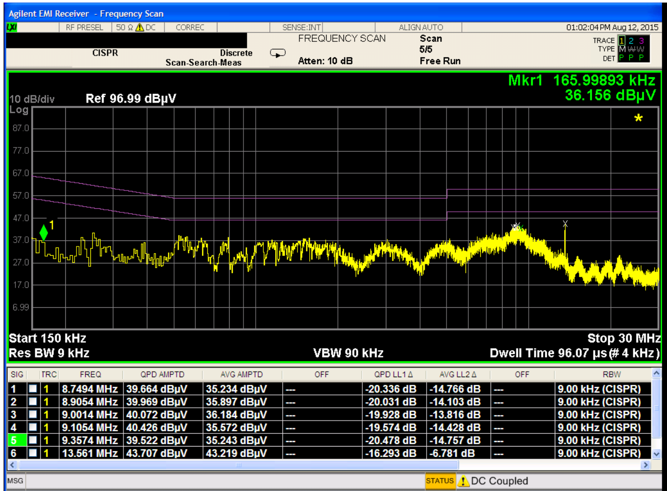
Plot 8-2. Line-Conducted Test Plot (N)
