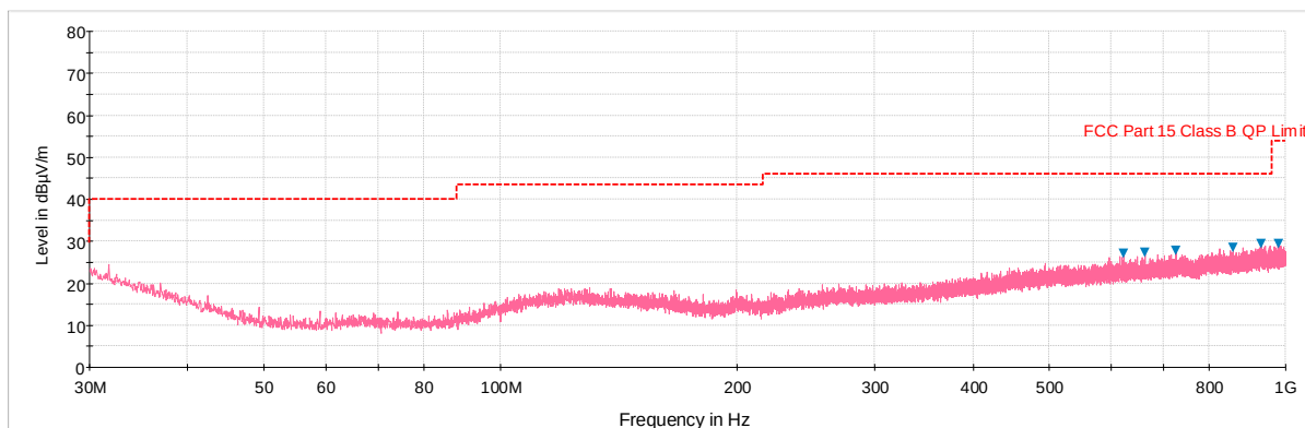
Plot 7-92. Radiated Spurious Plot below 1GHz (802.11a – U3 Ch. 157, Ant. Pol. V)
