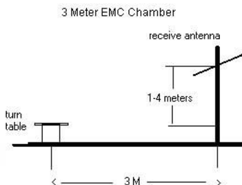
Figure 7-5. Test Instrument & Measurement Setup
