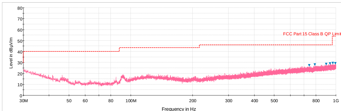
Plot 7-91. Radiated Spurious Plot below 1GHz (802.11a – U3 Ch. 157, Ant. Pol. H)
