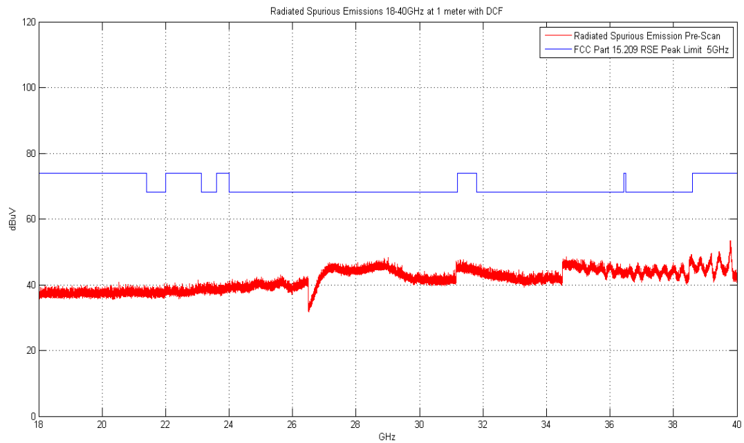
Plot 7-76. Radiated Spurious Plot above 18GHz (802.11a – Ant. Pol. V)
