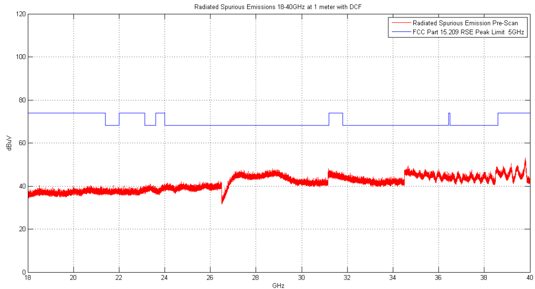
Plot 7-75. Radiated Spurious Plot above 18GHz (802.11a – Ant. Pol. H)
