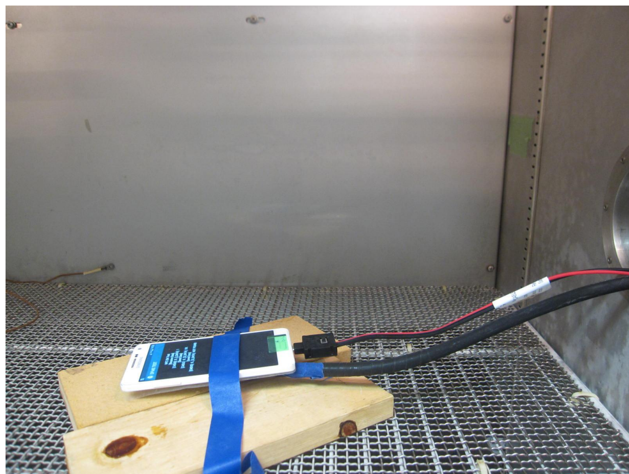
TEMPERATURE CHAMBER ENVIRONMENT
