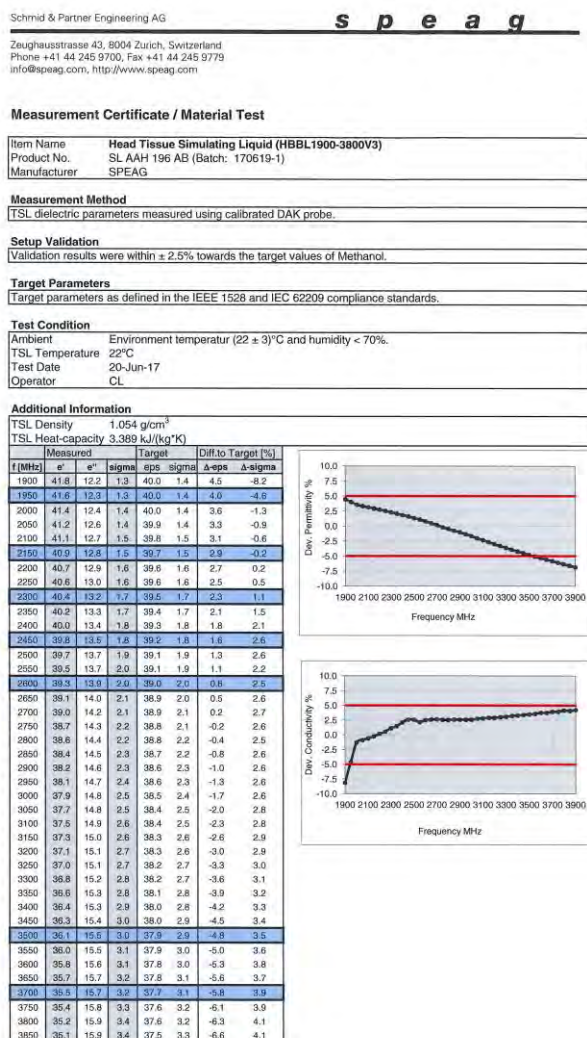
Figure D-5 2.45-2.6 GHz Head Tissue Equivalent Matter
