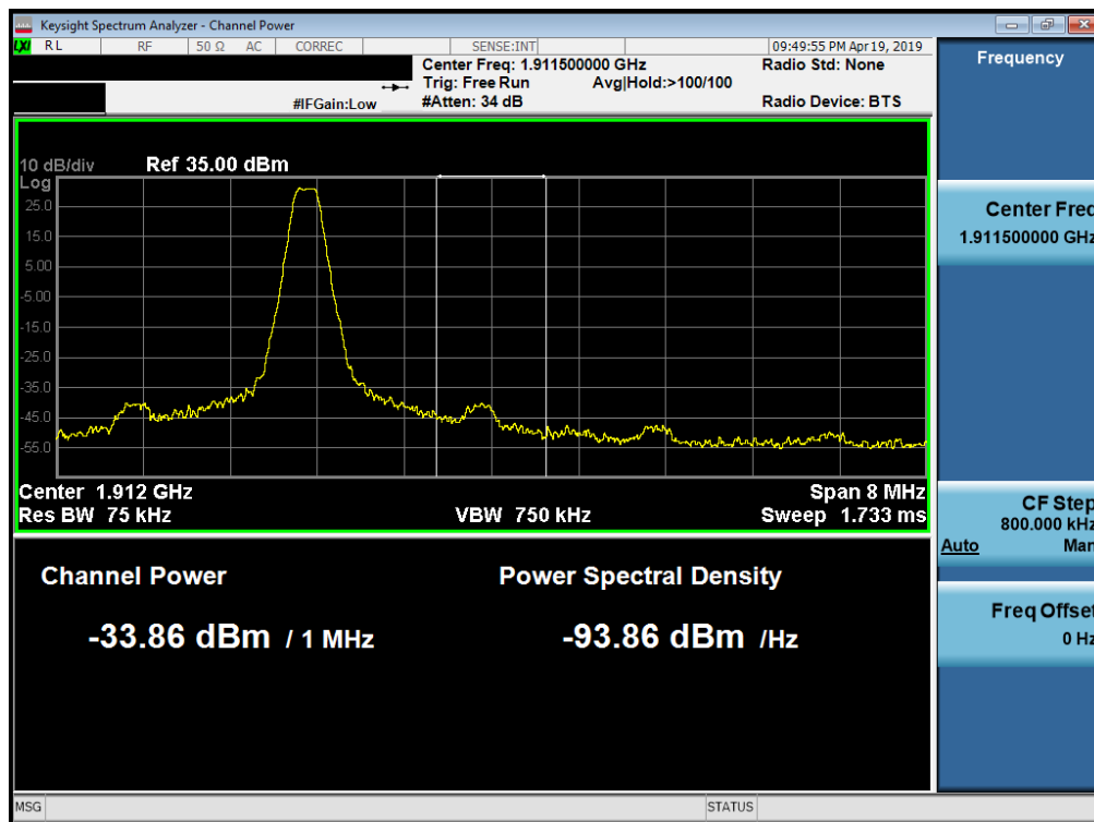
Plot 7-78. Band Edge Plot (PCS GPRS Mode – High Channel)
