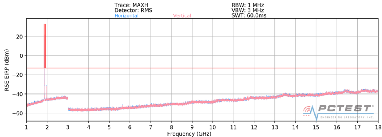
Plot 7-108. Radiated Spurious Plot above 1GHz (PCS GPRS Mode)
