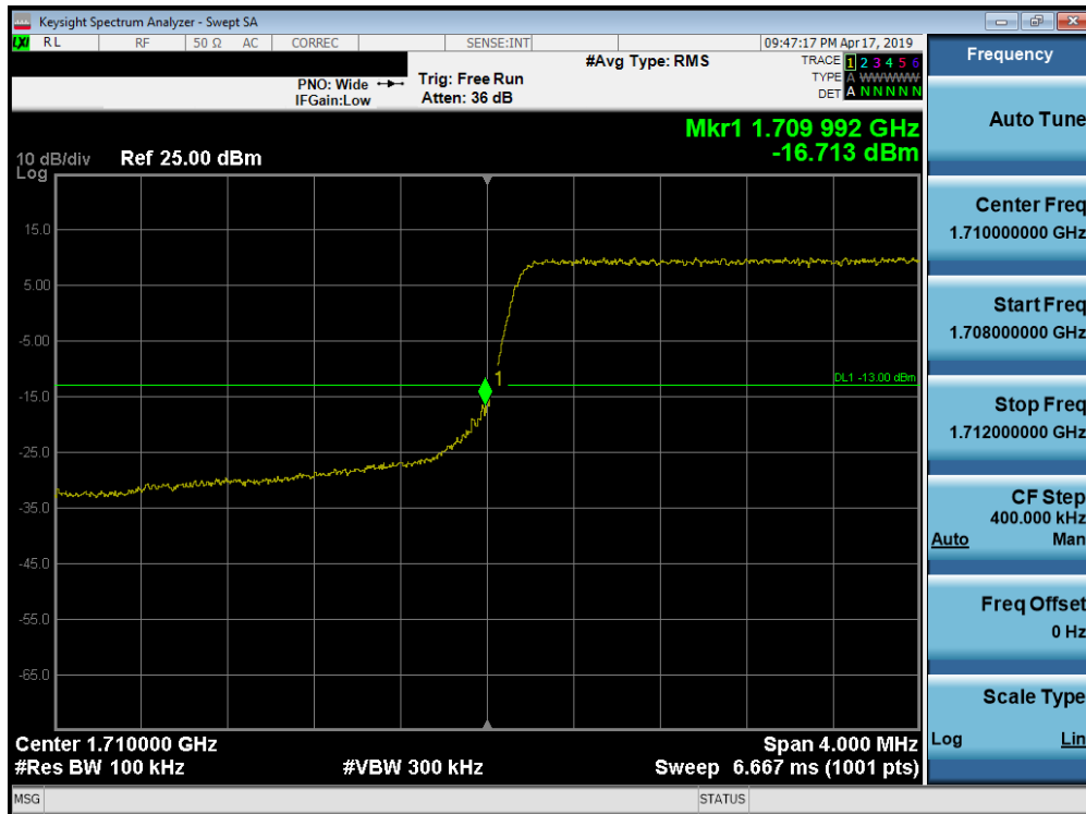
Plot 7-235. Lower Band Edge Plot (Band 66/4 - 3.0MHz QPSK - Full RB Configuration)
