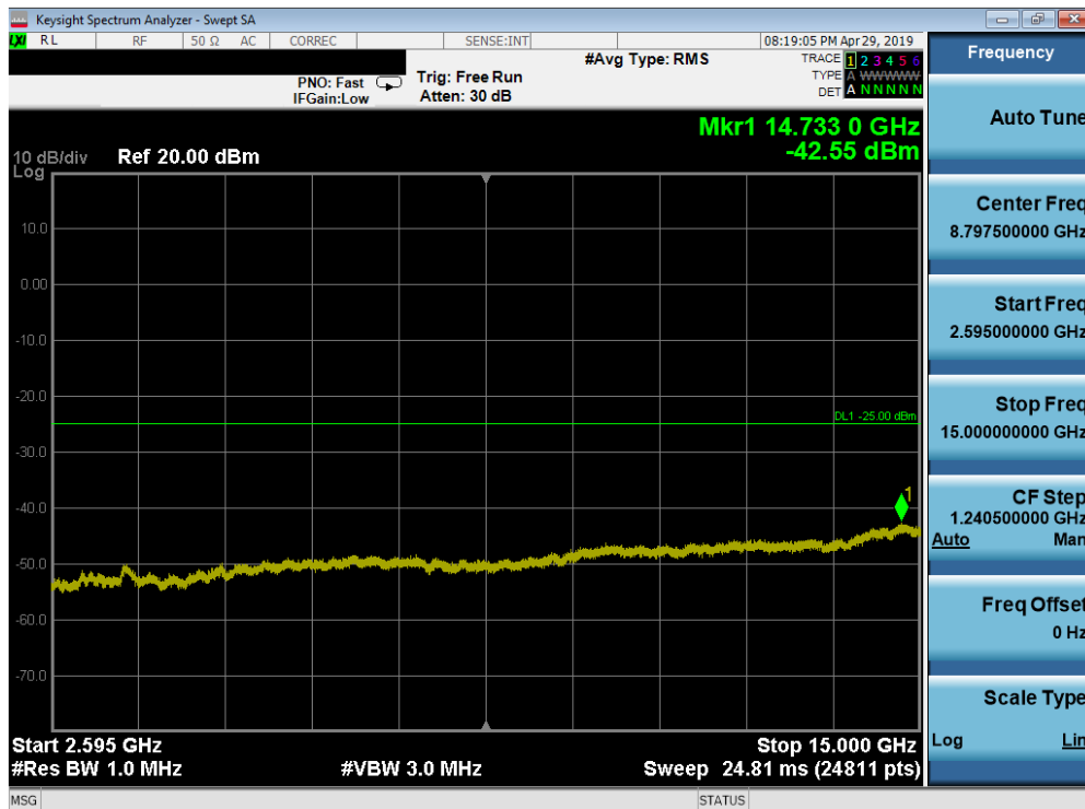
Plot 7-173. Conducted Spurious Plot (Band 7 - 20.0MHz QPSK - RB Size 1, RB Offset 0 - High Channel)
