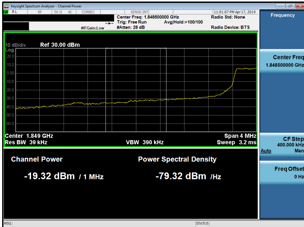
Plot 7-272. Lower Extended Band Edge Plot (Band 25/2 - 3.0MHz QPSK - Full RB Configuration)
