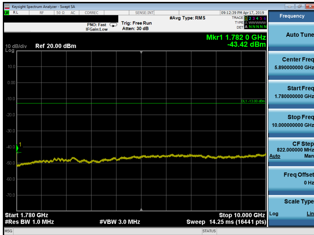
Plot 7-149. Conducted Spurious Plot (Band 66/4 - 20.0MHz QPSK - RB Size 1, RB Offset 0 - Low Channel)
