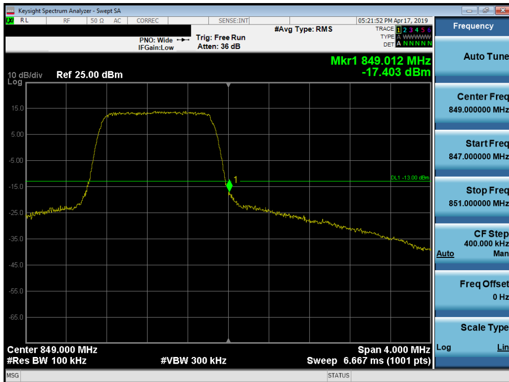
Plot 7-220. Upper Band Edge Plot (Band 26/5 - 1.4MHz QPSK - Full RB Configuration)
