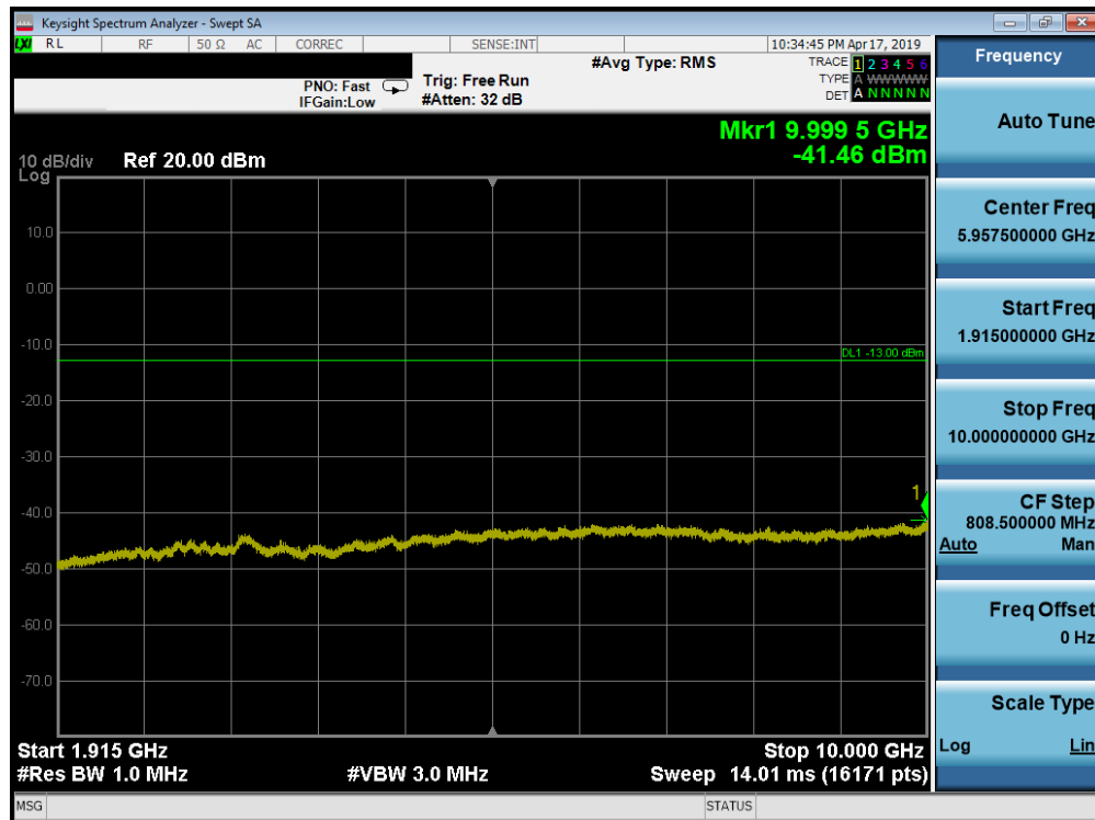
Plot 7-158. Conducted Spurious Plot (Band 25/2 - 20.0MHz QPSK - RB Size 1, RB Offset 0 - Low Channel)
