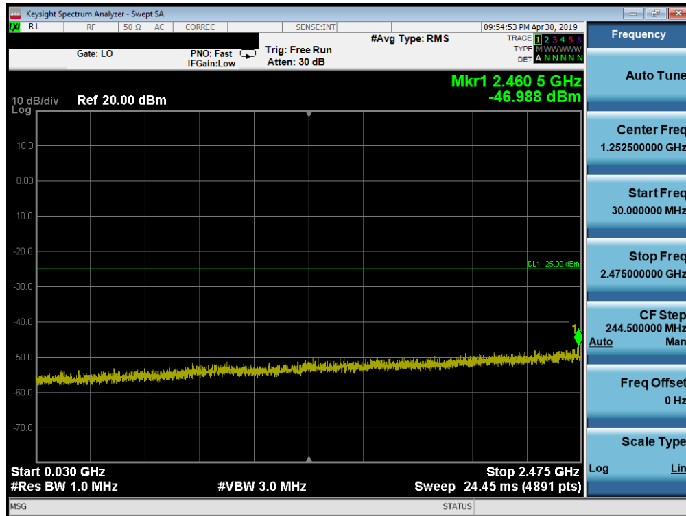
Plot 7-175. Conducted Spurious Plot (Band 41 PC2 - 20.0MHz QPSK - RB Size 1, RB Offset 0 - Low Channel)
