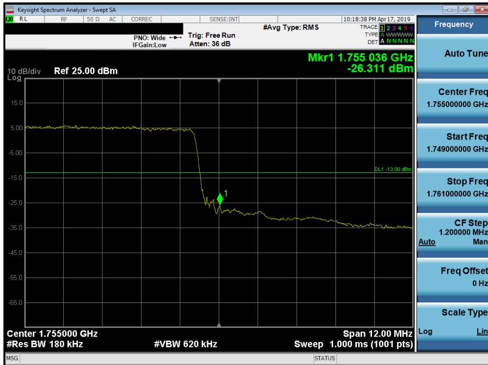
Plot 7-255. Upper Band Edge Plot (Band 4 - 15.0MHz QPSK - Full RB Configuration)
