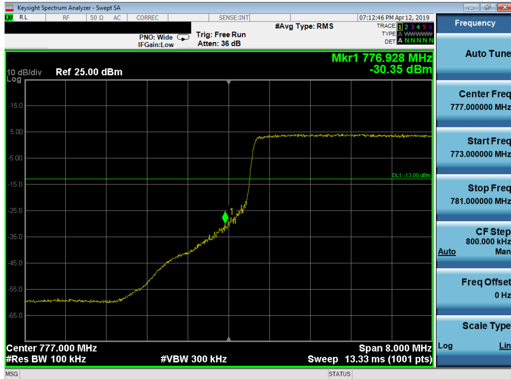
Plot 7-215. Lower Band Edge Plot (Band 13 - 10.0MHz QPSK - Full RB Configuration)
