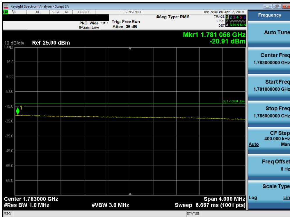
Plot 7-264. Upper Extended Band Edge Plot (Band 66 - 20.0MHz QPSK - Full RB Configuration)
