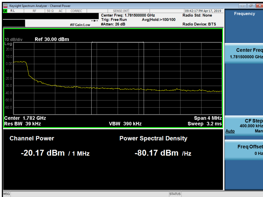
Plot 7-246. Upper Extended Band Edge Plot (Band 66 - 5.0MHz QPSK - Full RB Configuration)
