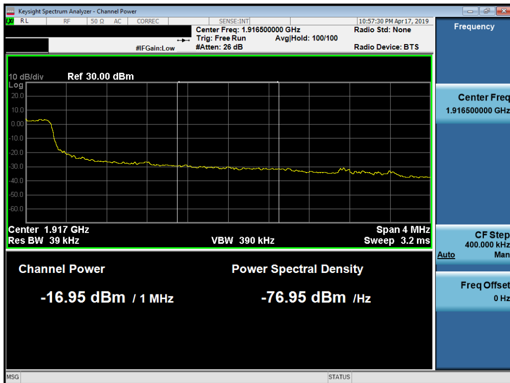
Plot 7-282. Upper Extended Band Edge Plot (Band 25 - 5.0MHz QPSK - Full RB Configuration)
