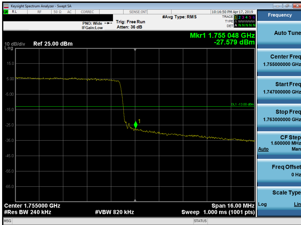
Plot 7-261. Upper Band Edge Plot (Band 4 - 20.0MHz QPSK - Full RB Configuration)
