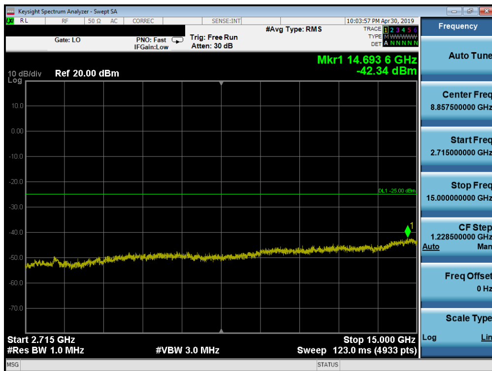
Plot 7-191. Conducted Spurious Plot (Band 41 PC2 - 20.0MHz QPSK - RB Size 1, RB Offset 0 - High Channel)
