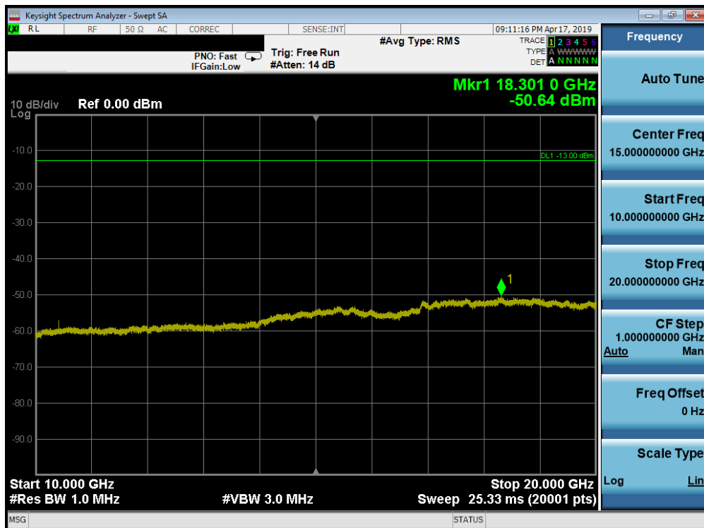
Plot 7-153. Conducted Spurious Plot (Band 66/4 - 20.0MHz QPSK - RB Size 1, RB Offset 0 - Mid Channel)
