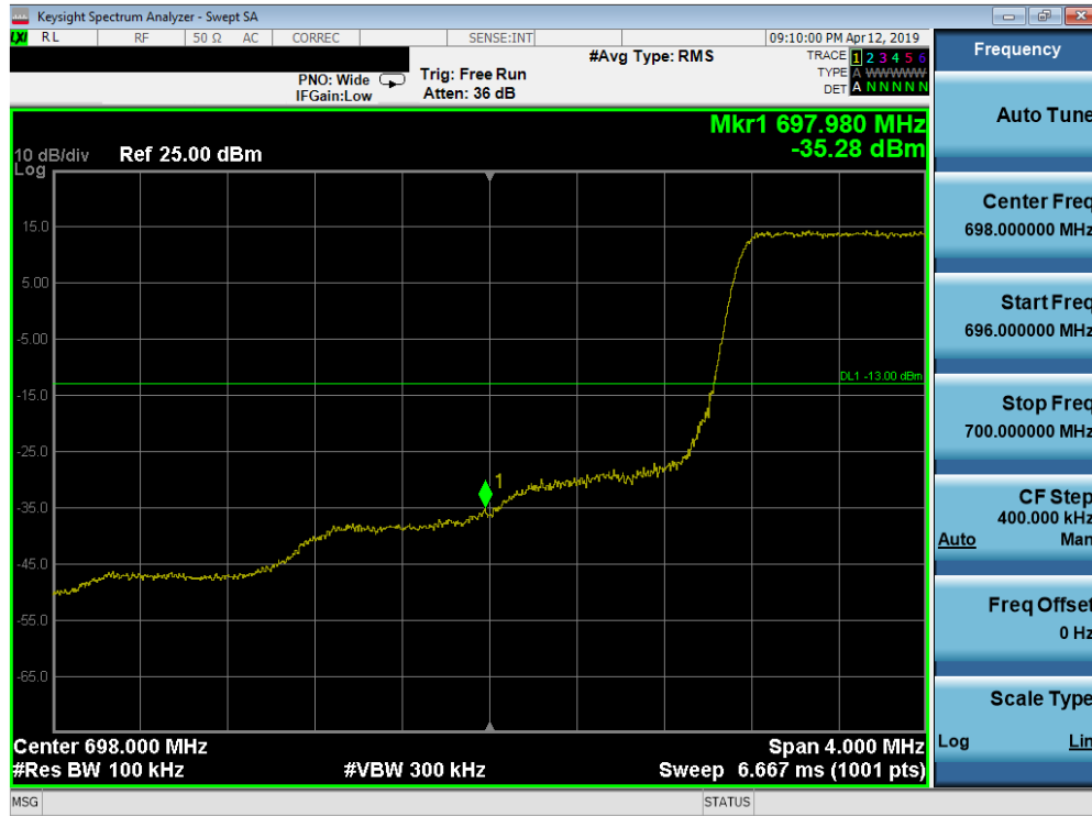
Plot 7-201. Lower Band Edge Plot (Band 12 - 1.4MHz QPSK - Full RB Configuration)
