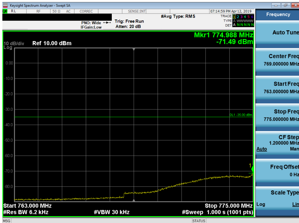
Plot 7-216. Lower Emission Mask Plot (Band 13 - 10.0MHz QPSK - Full RB Configuration)
