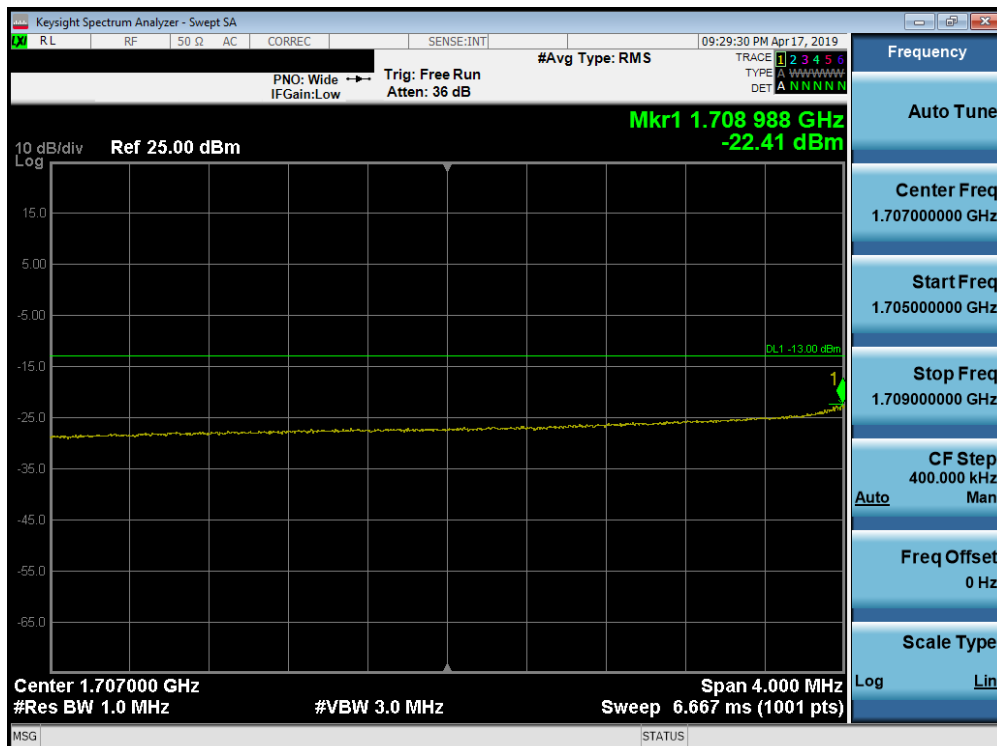
Plot 7-248. Lower Extended Band Edge Plot (Band 66/4 - 10.0MHz QPSK - Full RB Configuration)
