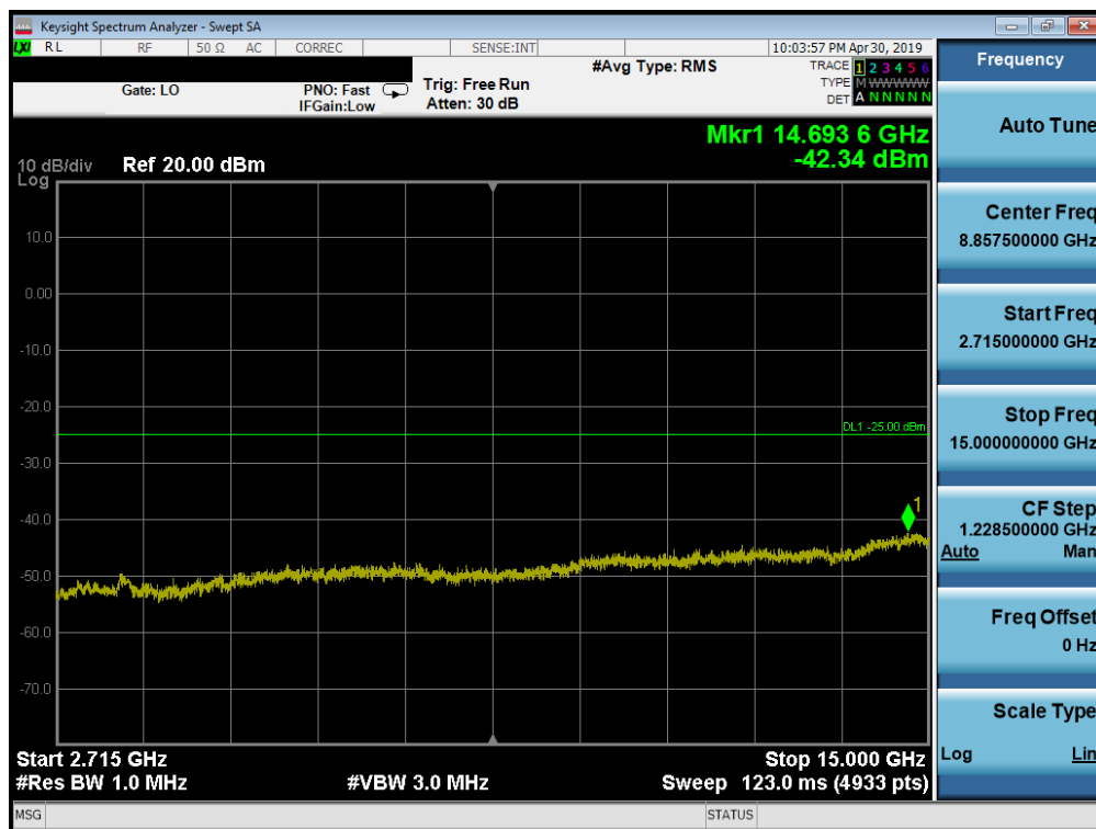
Plot 7-182. Conducted Spurious Plot (Band 41 PC2 - 20.0MHz QPSK - RB Size 1, RB Offset 0 - High Channel)
