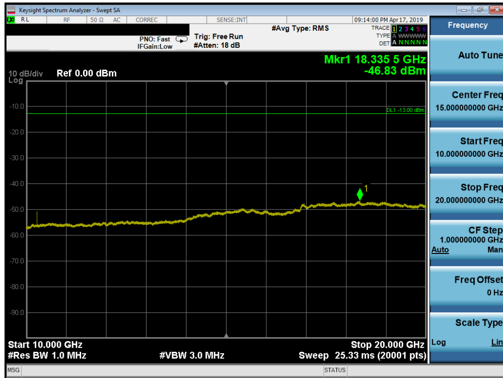
Plot 7-150. Conducted Spurious Plot (Band 66/4 - 20.0MHz QPSK - RB Size 1, RB Offset 0 - Low Channel)
