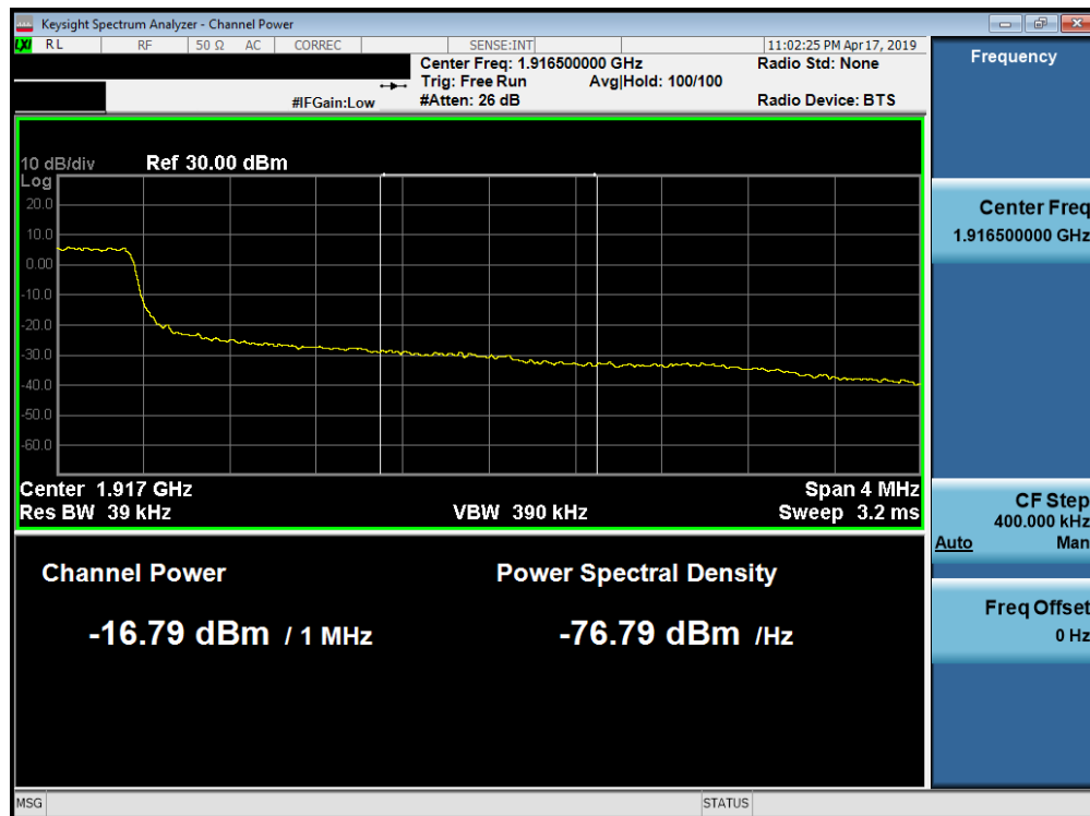
Plot 7-276. Upper Extended Band Edge Plot (Band 25 - 3.0MHz QPSK - Full RB Configuration)
