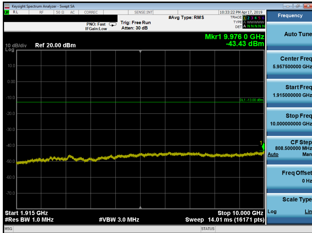
Plot 7-161. Conducted Spurious Plot (Band 25/2 - 20.0MHz QPSK - RB Size 1, RB Offset 0 - Mid Channel)
