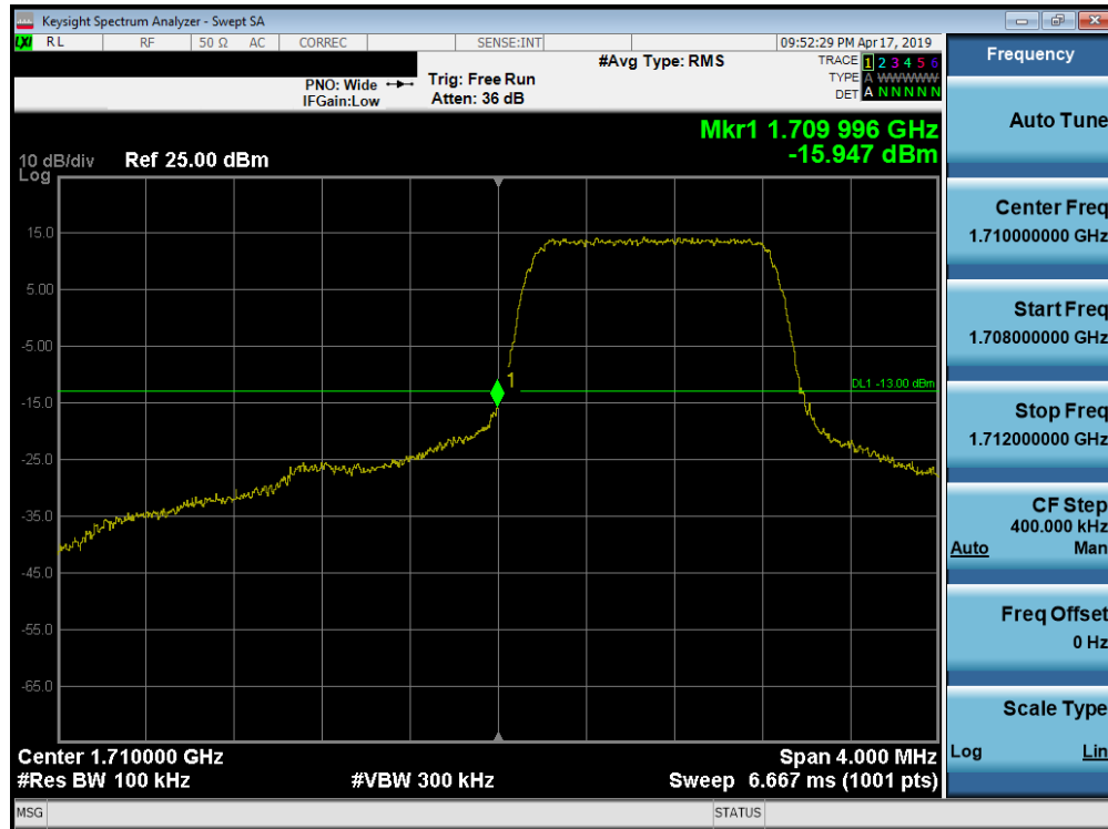
Plot 7-229. Lower Band Edge Plot (Band 66/4 - 1.4MHz QPSK - Full RB Configuration)
