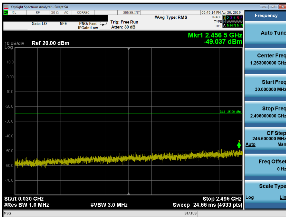
Plot 7-178. Conducted Spurious Plot (Band 41 PC2 - 20.0MHz QPSK - RB Size 1, RB Offset 0 - Mid Channel)
