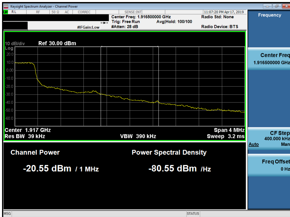
Plot 7-270. Upper Extended Band Edge Plot (Band 25 - 1.4MHz QPSK - Full RB Configuration)
