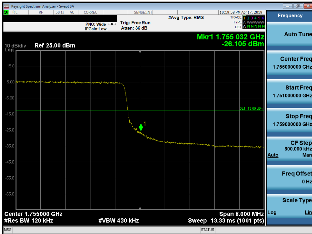
Plot 7-249. Upper Band Edge Plot (Band 4 - 10.0MHz QPSK - Full RB Configuration)
