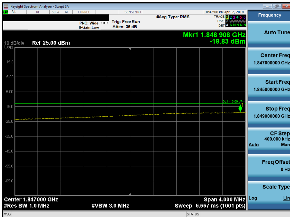
Plot 7-290. Lower Extended Band Edge Plot (Band 25/2 - 15.0MHz QPSK - Full RB Configuration)
