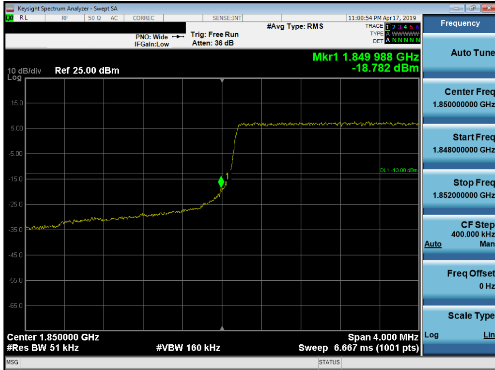
Plot 7-271. Lower Band Edge Plot (Band 25/2 - 3.0MHz QPSK - Full RB Configuration)
