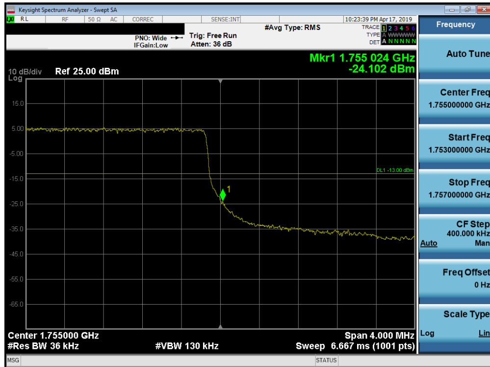
Plot 7-237. Upper Band Edge Plot (Band 4 - 3.0MHz QPSK - Full RB Configuration)
