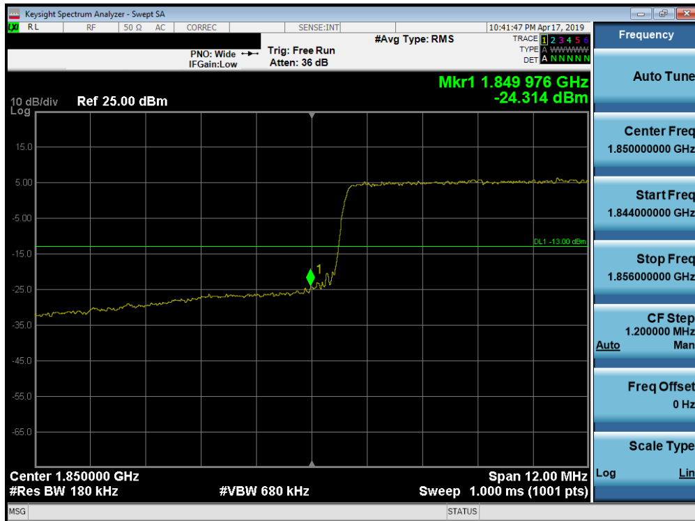
Plot 7-289. Lower Band Edge Plot (Band 25/2 - 15.0MHz QPSK - Full RB Configuration)
