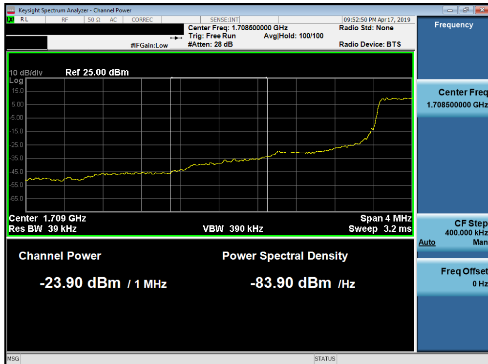
Plot 7-230. Lower Extended Band Edge Plot (Band 66/4 - 1.4MHz QPSK - Full RB Configuration)
