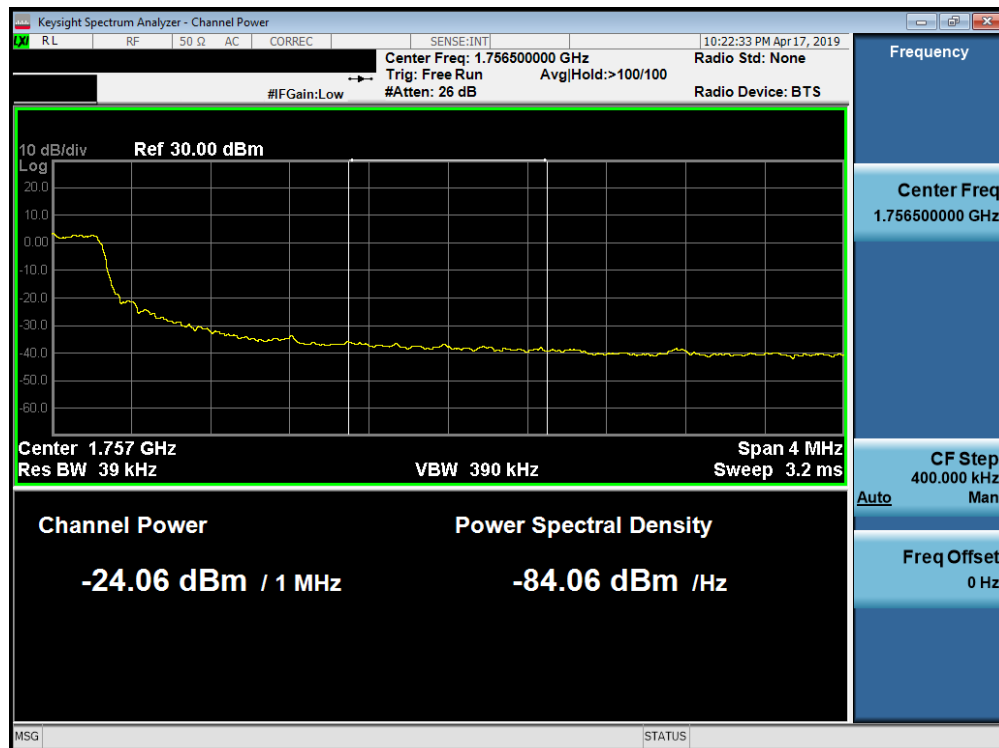
Plot 7-244. Upper Extended Band Edge Plot (Band 4 - 5.0MHz QPSK - Full RB Configuration)
