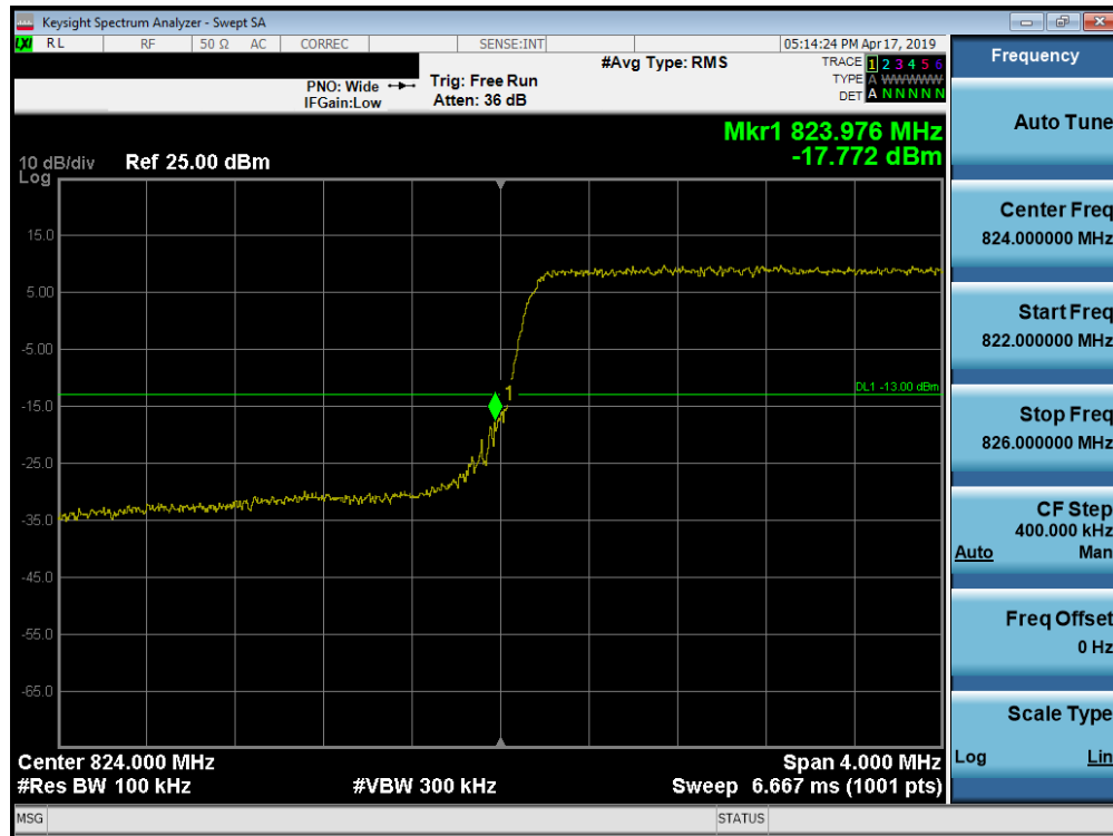
Plot 7-221. Lower Band Edge Plot (Band 26/5 - 3.0MHz QPSK - Full RB Configuration)
