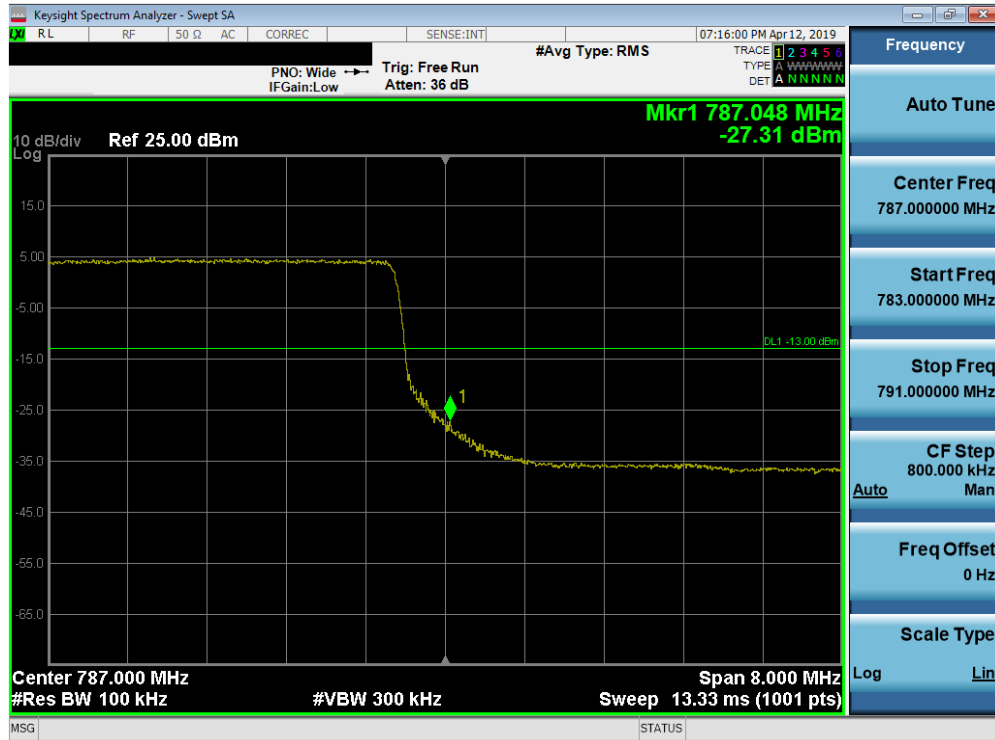
Plot 7-217. Upper Band Edge Plot (Band 13 - 10.0MHz QPSK - Full RB Configuration)
