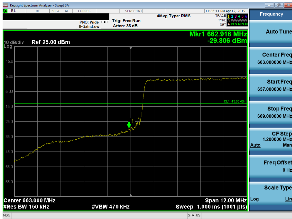
Plot 7-197. Lower Band Edge Plot (Band 71 - 15.0MHz QPSK - Full RB Configuration)
