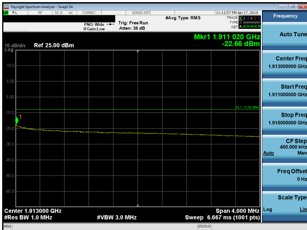
Plot 7-286. Upper Extended Band Edge Plot (Band 2 - 10.0MHz QPSK - Full RB Configuration)
