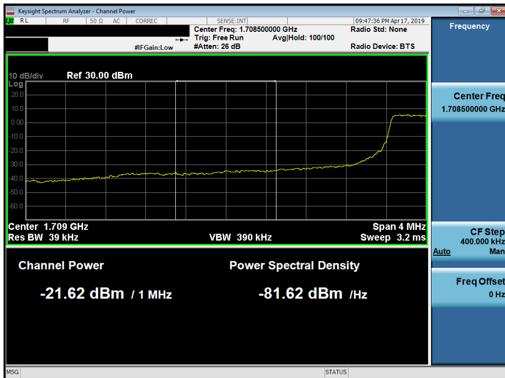
Plot 7-236. Lower Extended Band Edge Plot (Band 66/4 - 3.0MHz QPSK - Full RB Configuration)
