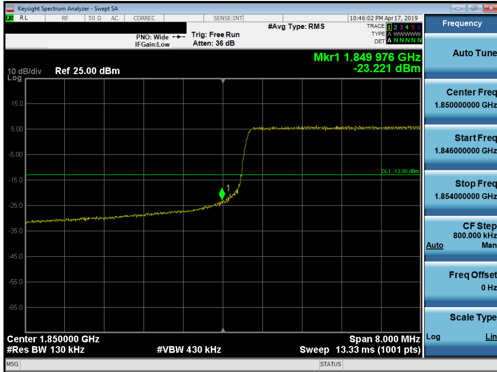
Plot 7-283. Lower Band Edge Plot (Band 25/2 - 10.0MHz QPSK - Full RB Configuration)
