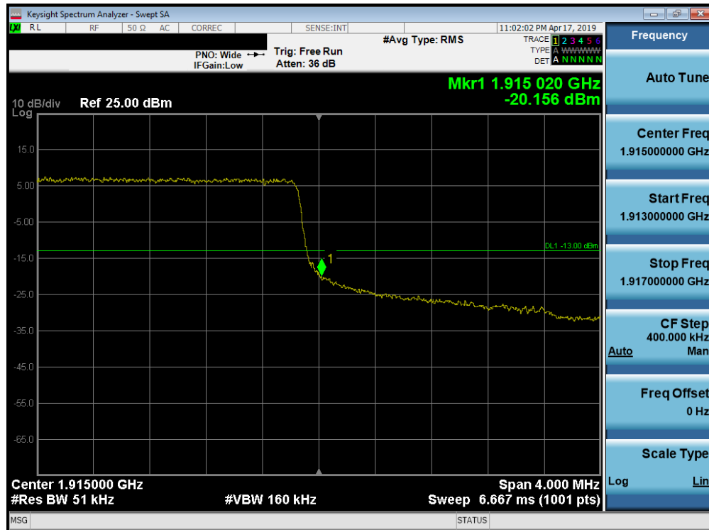
Plot 7-275. Upper Band Edge Plot (Band 25 - 3.0MHz QPSK - Full RB Configuration)
