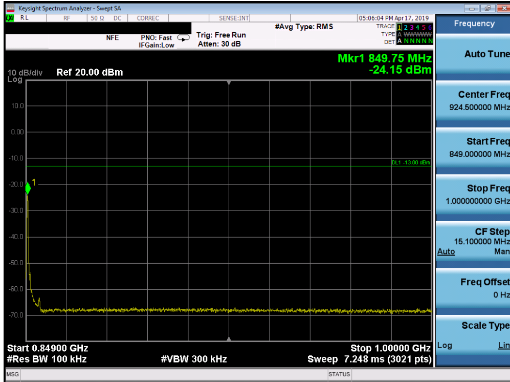
Plot 7-143. Conducted Spurious Plot (Band 26/5 - 10.0MHz QPSK - RB Size 1, RB Offset 0 - Mid Channel)
