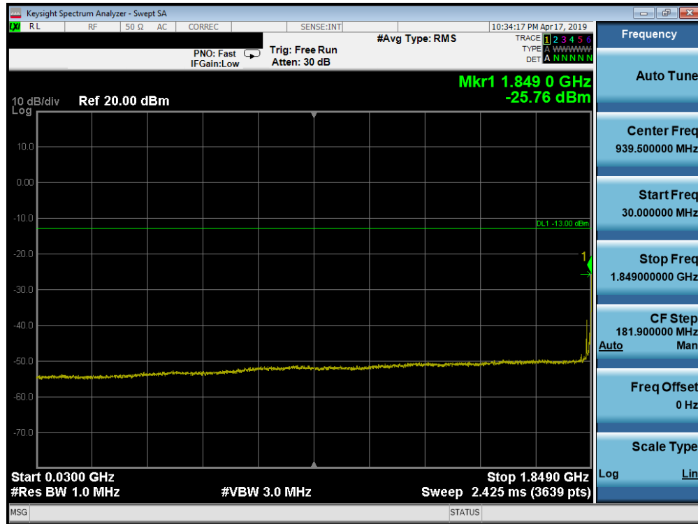
Plot 7-157. Conducted Spurious Plot (Band 25/2 - 20.0MHz QPSK - RB Size 1, RB Offset 0 - Low Channel)
