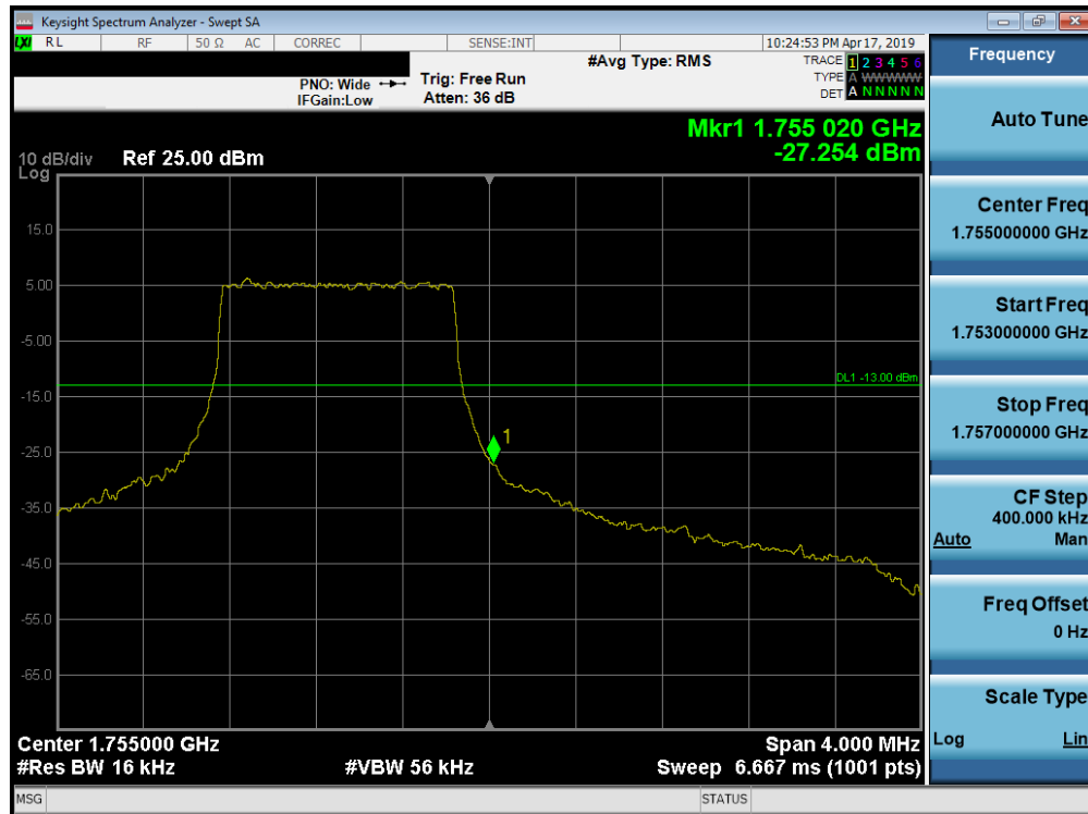
Plot 7-231. Upper Band Edge Plot (Band 4 - 1.4MHz QPSK - Full RB Configuration)
