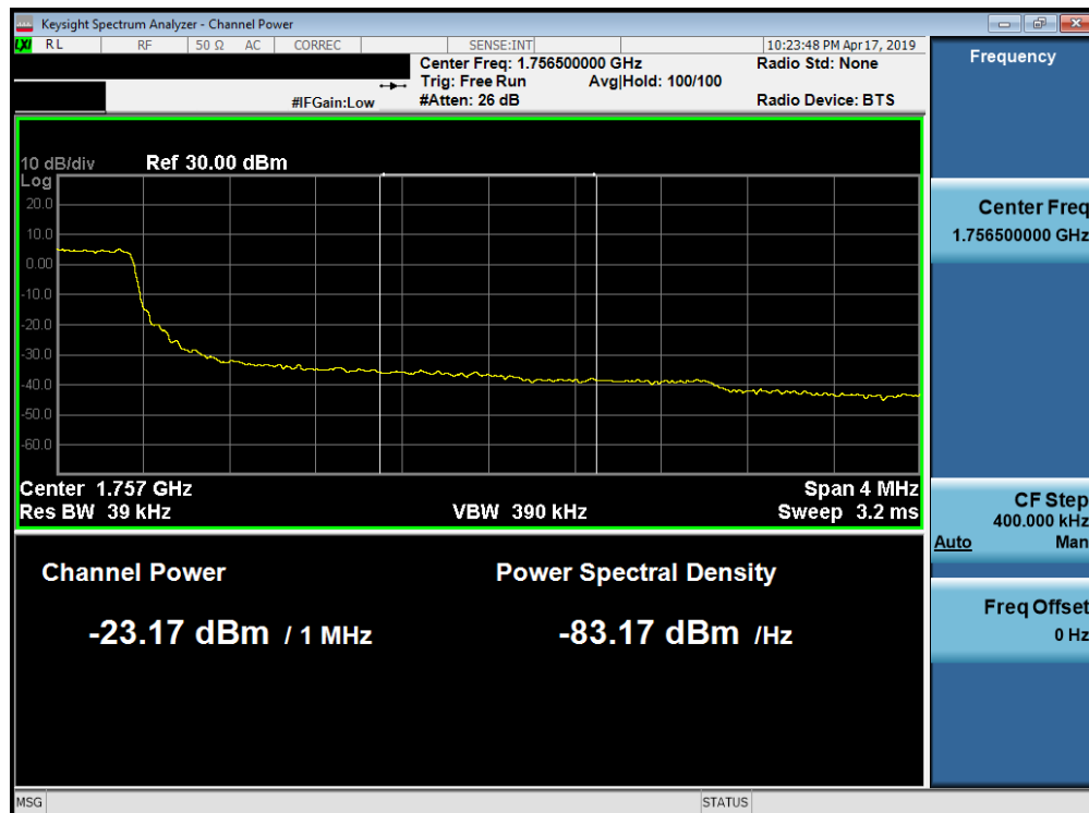
Plot 7-238. Upper Extended Band Edge Plot (Band 4 - 3.0MHz QPSK - Full RB Configuration)
