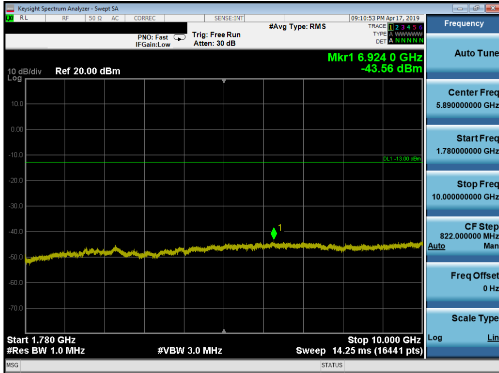
Plot 7-152. Conducted Spurious Plot (Band 66/4 - 20.0MHz QPSK - RB Size 1, RB Offset 0 - Mid Channel)
