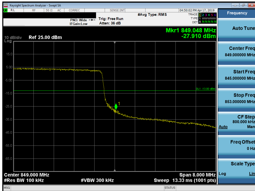
Plot 7-226. Upper Band Edge Plot (Band 26/5 - 10.0MHz QPSK - Full RB Configuration)
