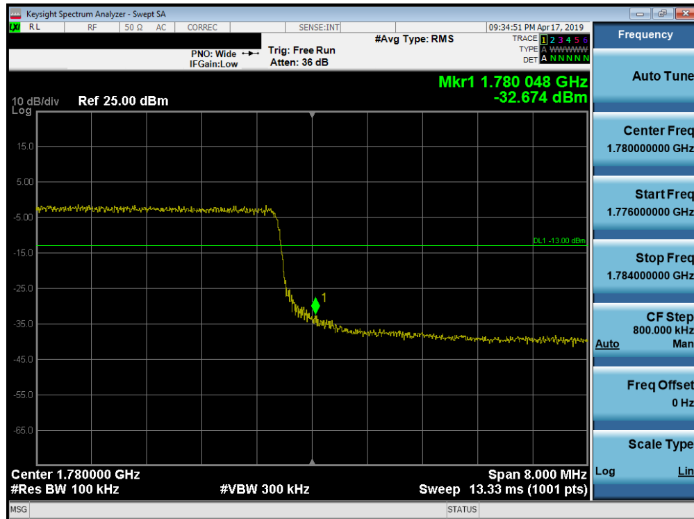
Plot 7-251. Upper Band Edge Plot (Band 66 - 10.0MHz QPSK - Full RB Configuration)
