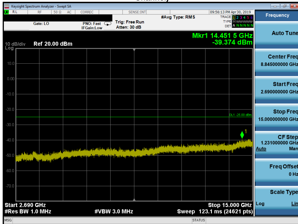
Plot 7-176. Conducted Spurious Plot (Band 41 PC2 - 20.0MHz QPSK - RB Size 1, RB Offset 0 - Low Channel)
