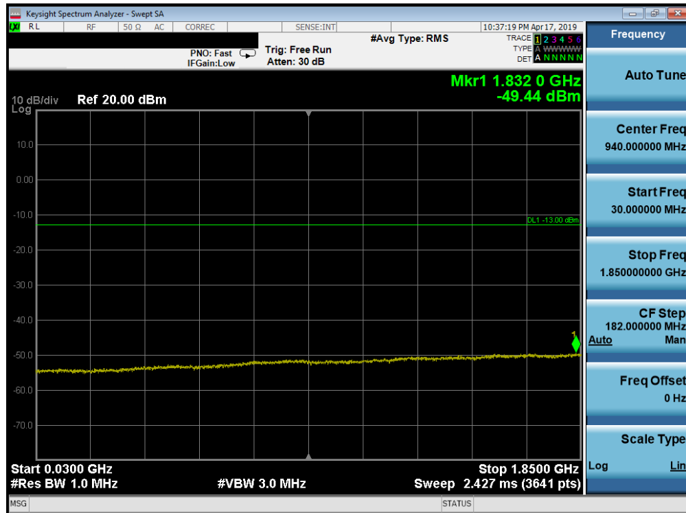
Plot 7-163. Conducted Spurious Plot (Band 25/2 - 20.0MHz QPSK - RB Size 1, RB Offset 0 - High Channel)
