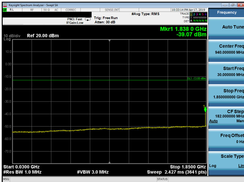
Plot 7-160. Conducted Spurious Plot (Band 25/2 - 20.0MHz QPSK - RB Size 1, RB Offset 0 - Mid Channel)
