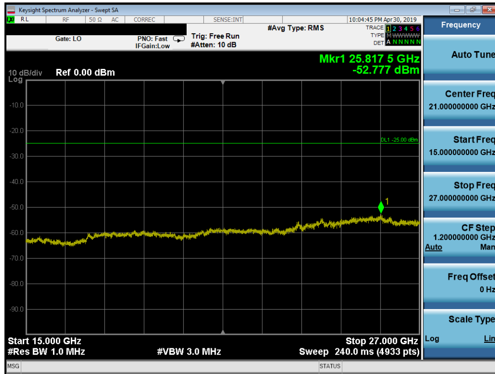
Plot 7-183. Conducted Spurious Plot (Band 41 PC2 - 20.0MHz QPSK - RB Size 1, RB Offset 0 - High Channel)
