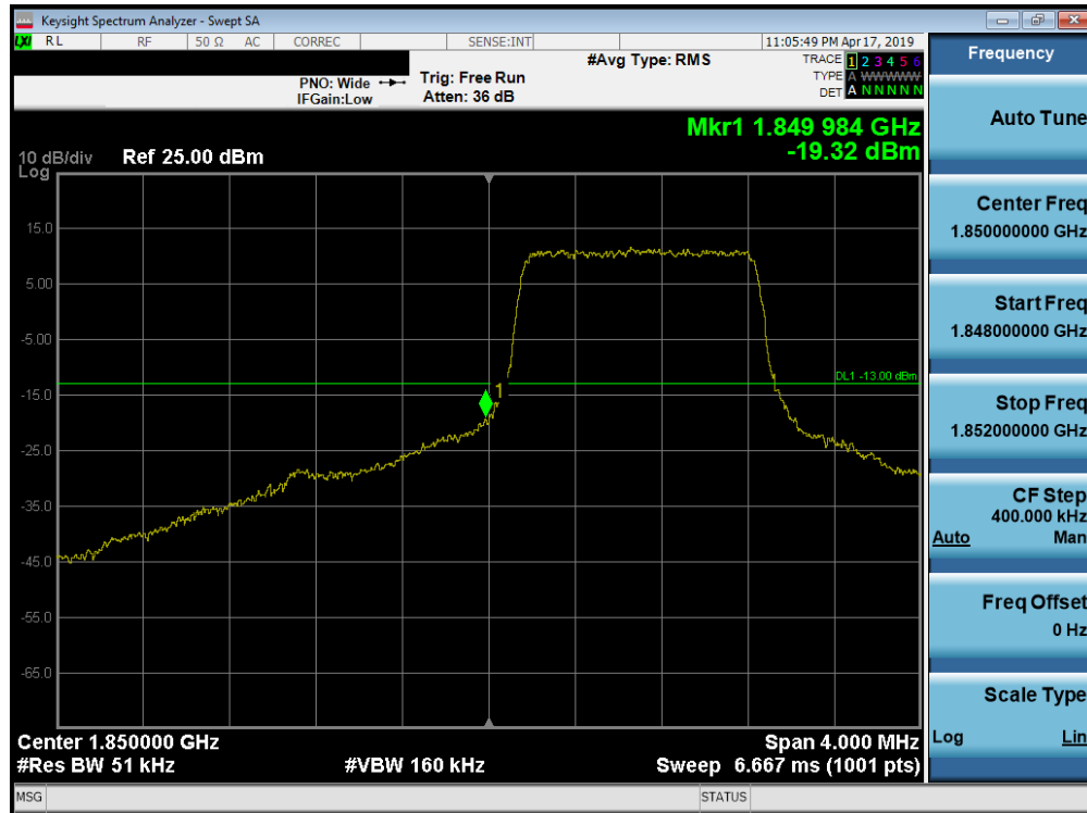
Plot 7-265. Lower Band Edge Plot (Band 25/2 - 1.4MHz QPSK - Full RB Configuration)
