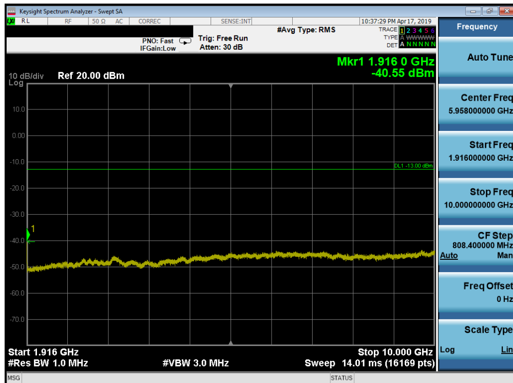
Plot 7-164. Conducted Spurious Plot (Band 25/2 - 20.0MHz QPSK - RB Size 1, RB Offset 0 - High Channel)
