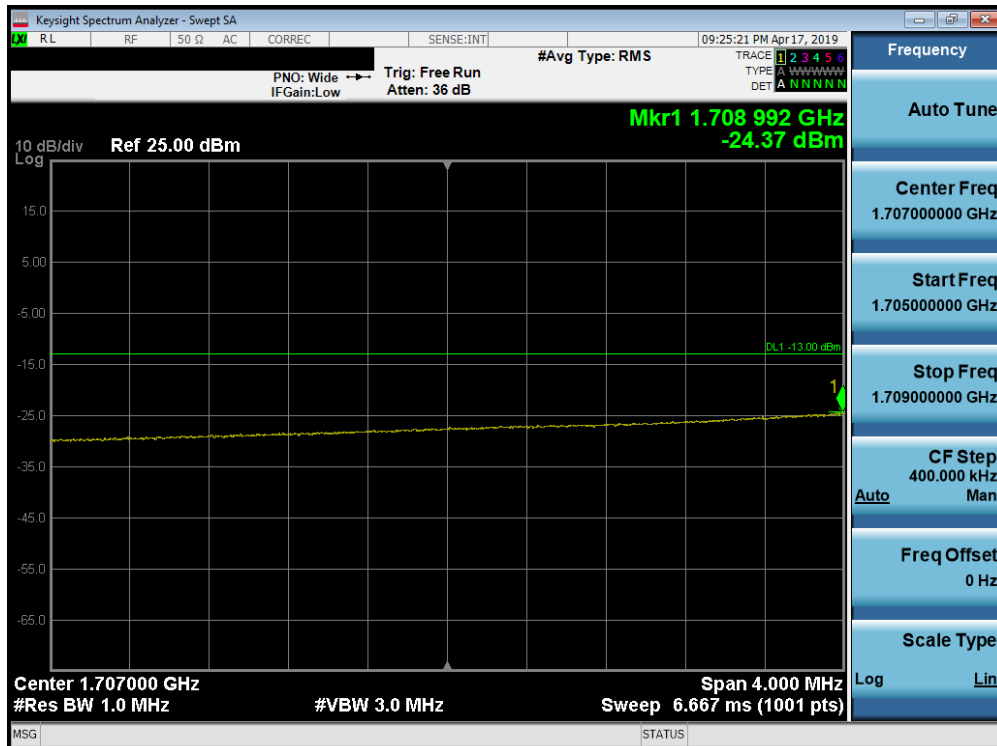
Plot 7-254. Lower Extended Band Edge Plot (Band 66/4 - 15.0MHz QPSK - Full RB Configuration)
