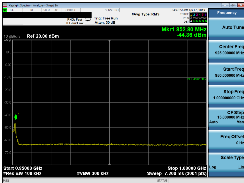
Plot 7-146. Conducted Spurious Plot (Band 26/5 - 10.0MHz QPSK - RB Size 1, RB Offset 0 - High Channel)
