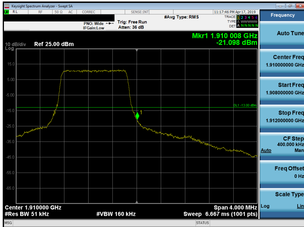
Plot 7-267. Upper Band Edge Plot (Band 2 - 1.4MHz QPSK - Full RB Configuration)
