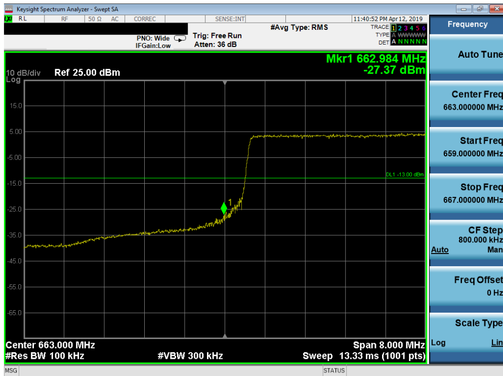
Plot 7-195. Lower Band Edge Plot (Band 71 - 10.0MHz QPSK - Full RB Configuration)
