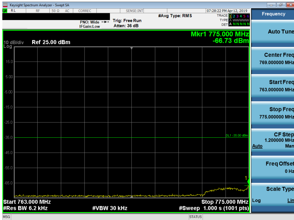
Plot 7-212. Lower Emission Mask Plot (Band 13 - 5.0MHz QPSK - Full RB Configuration)
