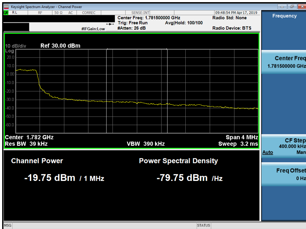
Plot 7-240. Upper Extended Band Edge Plot (Band 66 - 3.0MHz QPSK - Full RB Configuration)
