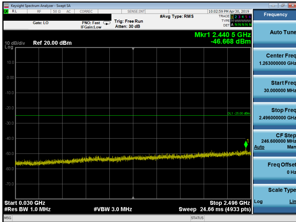
Plot 7-190. Conducted Spurious Plot (Band 41 PC2- 20.0MHz QPSK - RB Size 1, RB Offset 0 - High Channel)
