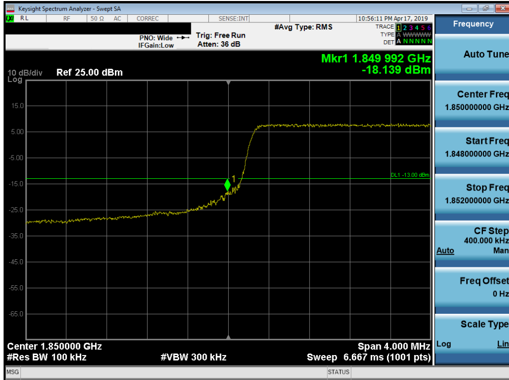
Plot 7-277. Lower Band Edge Plot (Band 25/2 - 5.0MHz QPSK - Full RB Configuration)
