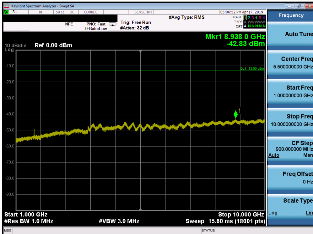
Plot 7-144. Conducted Spurious Plot (Band 26/5 - 10.0MHz QPSK - RB Size 1, RB Offset 0 - Mid Channel)
