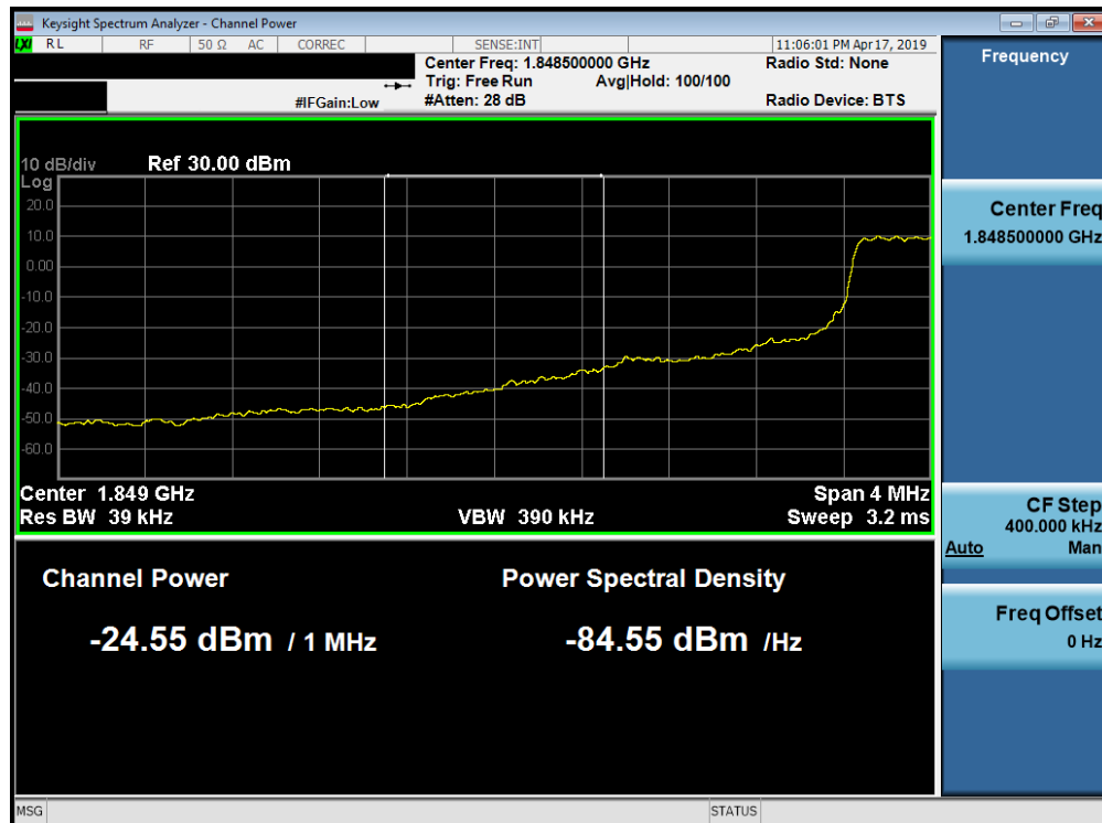
Plot 7-266. Lower Extended Band Edge Plot (Band 25/2 - 1.4MHz QPSK - Full RB Configuration)
