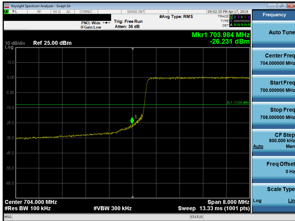
Plot 7-209. Lower Band Edge Plot (Band 17 - 10.0MHz QPSK - Full RB Configuration)
