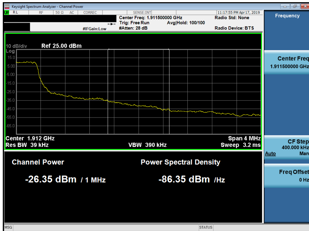
Plot 7-268. Upper Extended Band Edge Plot (Band 2 - 1.4MHz QPSK - Full RB Configuration)
