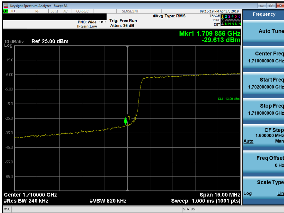
Plot 7-259. Lower Band Edge Plot (Band 66/4 - 20.0MHz QPSK - Full RB Configuration)
