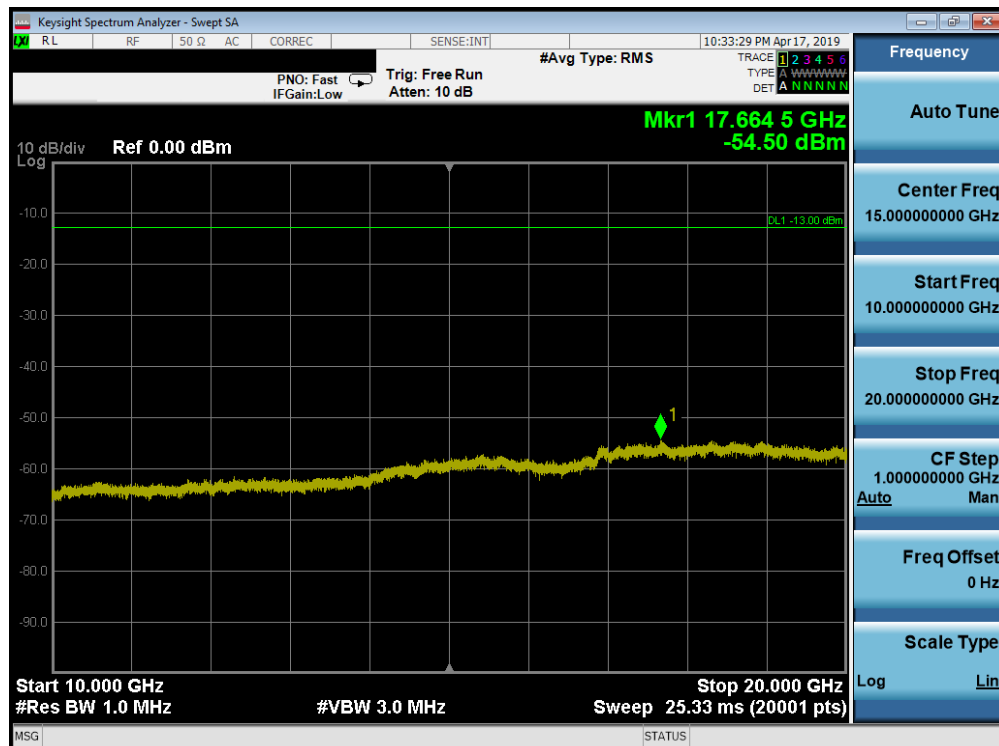
Plot 7-162. Conducted Spurious Plot (Band 25/2 - 20.0MHz QPSK - RB Size 1, RB Offset 0 - Mid Channel)
