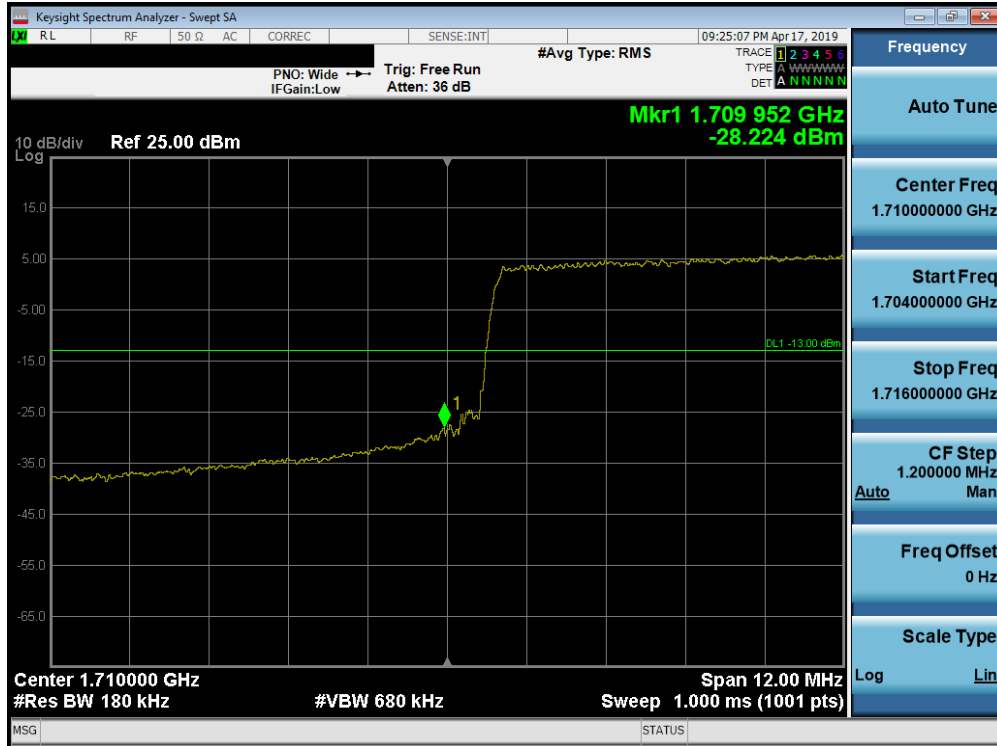
Plot 7-253. Lower Band Edge Plot (Band 66/4 - 15.0MHz QPSK - Full RB Configuration)
