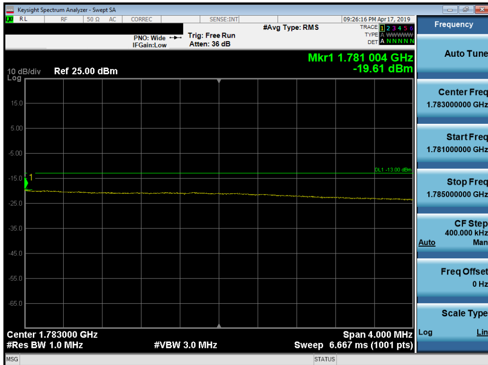
Plot 7-258. Upper Extended Band Edge Plot (Band 66 - 15.0MHz QPSK - Full RB Configuration)
