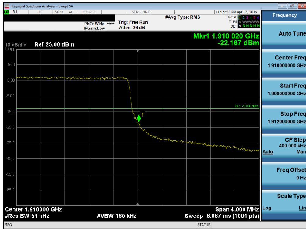
Plot 7-273. Upper Band Edge Plot (Band 2 - 3.0MHz QPSK - Full RB Configuration)
