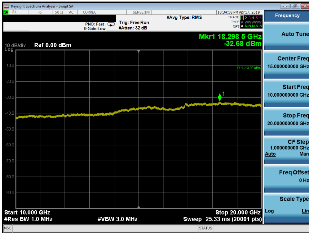
Plot 7-159. Conducted Spurious Plot (Band 25/2 - 20.0MHz QPSK - RB Size 1, RB Offset 0 - Low Channel)
