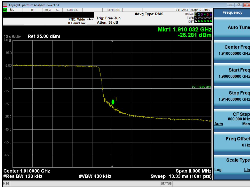
Plot 7-285. Upper Band Edge Plot (Band 2 - 10.0MHz QPSK - Full RB Configuration)
