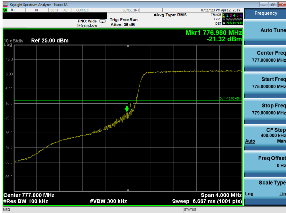
Plot 7-211. Lower Band Edge Plot (Band 13 - 5.0MHz QPSK - Full RB Configuration)
