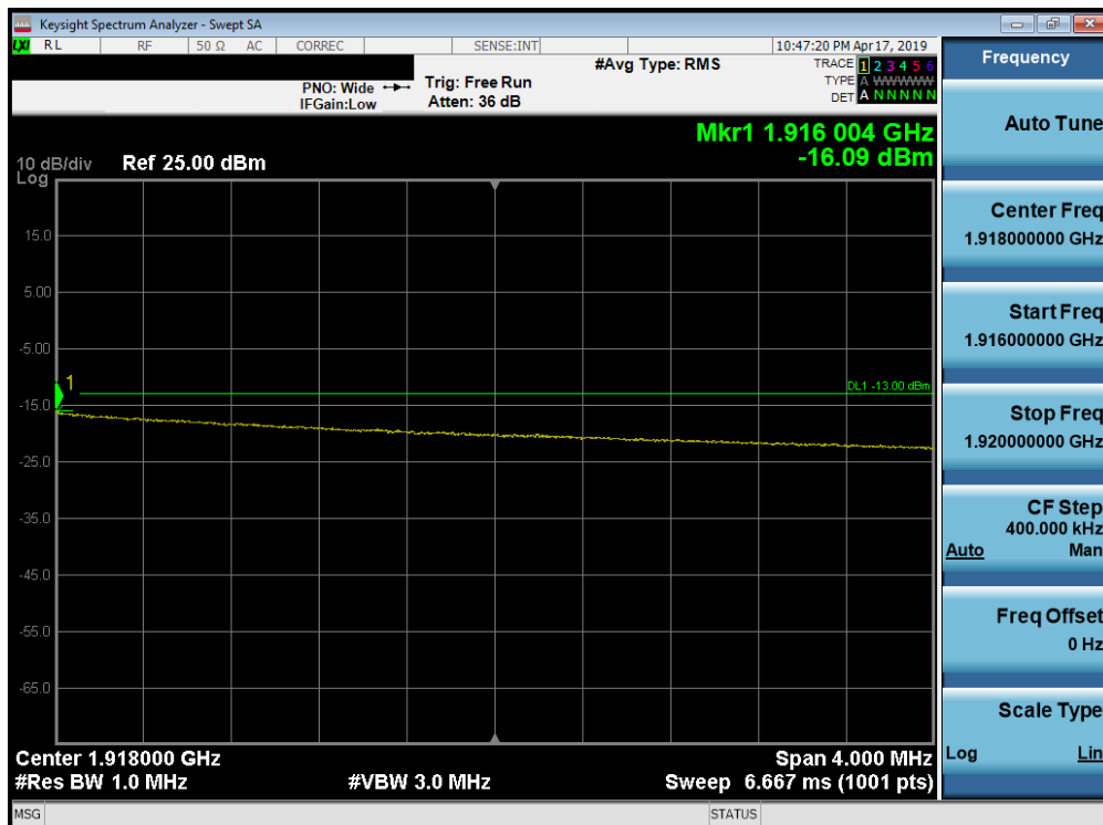
Plot 7-288. Upper Extended Band Edge Plot (Band 25 - 10.0MHz QPSK - Full RB Configuration)
