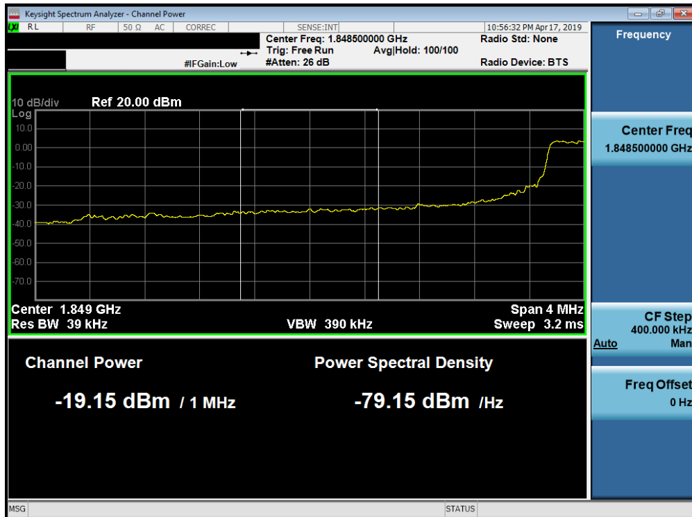
Plot 7-278. Lower Extended Band Edge Plot (Band 25/2 - 5.0MHz QPSK - Full RB Configuration)
