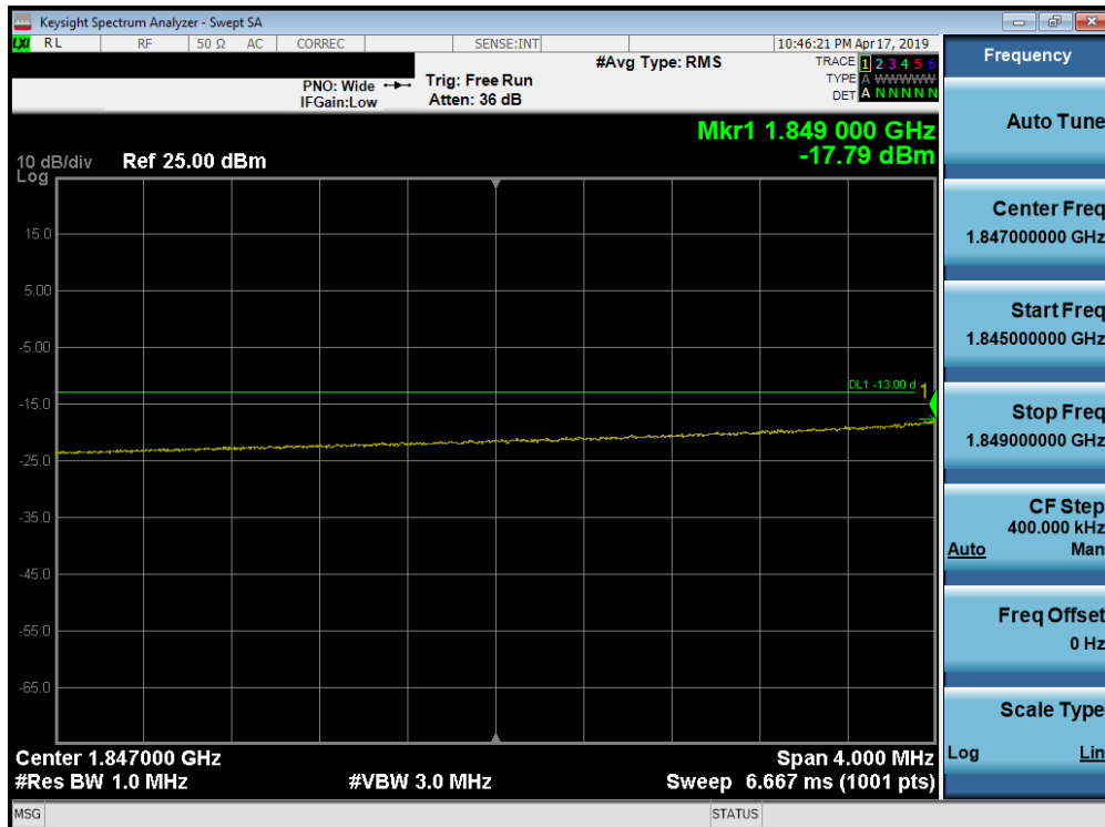
Plot 7-284. Lower Extended Band Edge Plot (Band 25/2 - 10.0MHz QPSK - Full RB Configuration)
