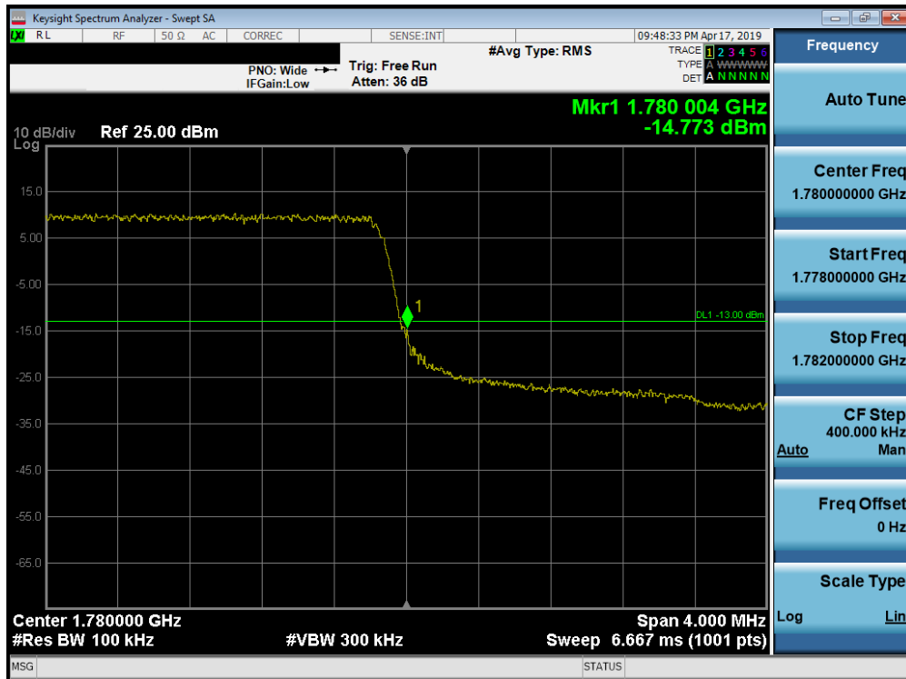
Plot 7-239. Upper Band Edge Plot (Band 66 - 3.0MHz QPSK - Full RB Configuration)
