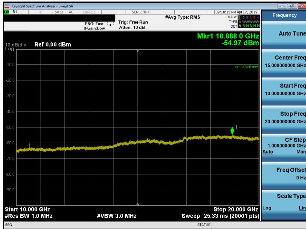
Plot 7-156. Conducted Spurious Plot (Band 66/4 - 20.0MHz QPSK - RB Size 1, RB Offset 0 - High Channel)
