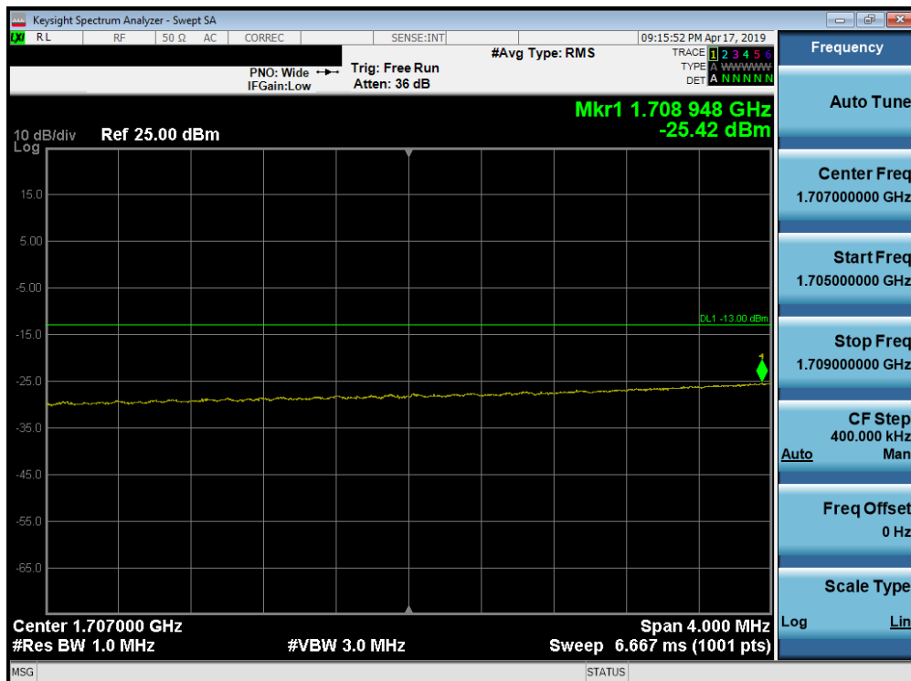
Plot 7-260. Lower Extended Band Edge Plot (Band 66/4 - 20.0MHz QPSK - Full RB Configuration)
