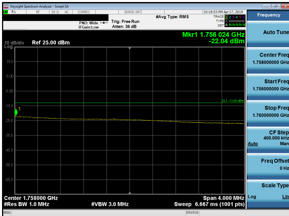
Plot 7-256. Upper Extended Band Edge Plot (Band 4 - 15.0MHz QPSK - Full RB Configuration)
