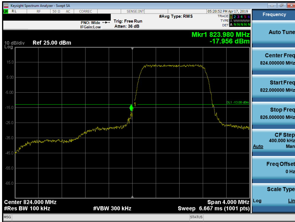
Plot 7-219. Lower Band Edge Plot (Band 26/5 - 1.4MHz QPSK - Full RB Configuration)
