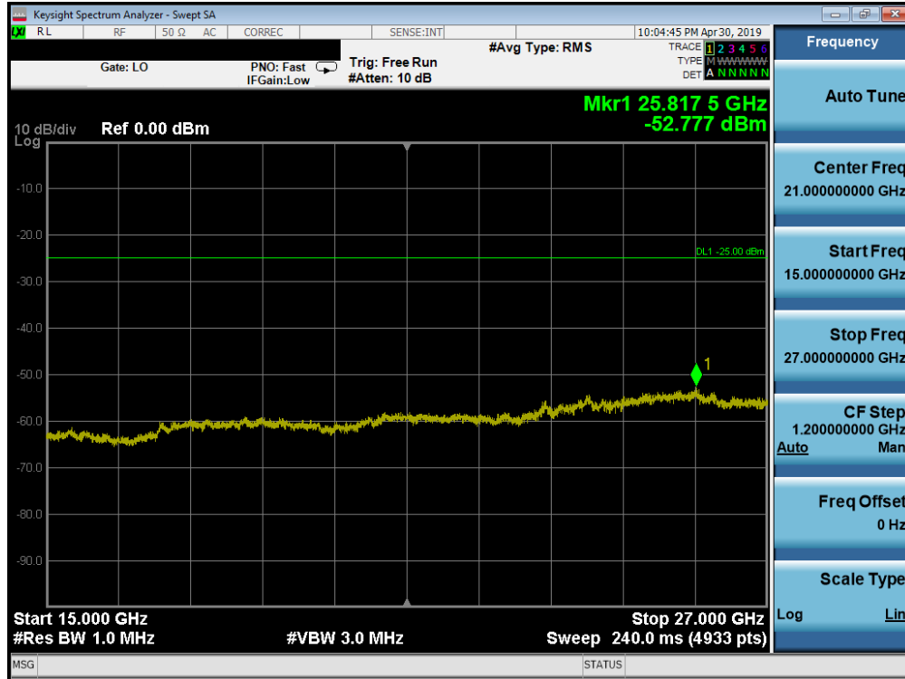
Plot 7-192. Conducted Spurious Plot (Band 41 PC2 - 20.0MHz QPSK - RB Size 1, RB Offset 0 - High Channel)
