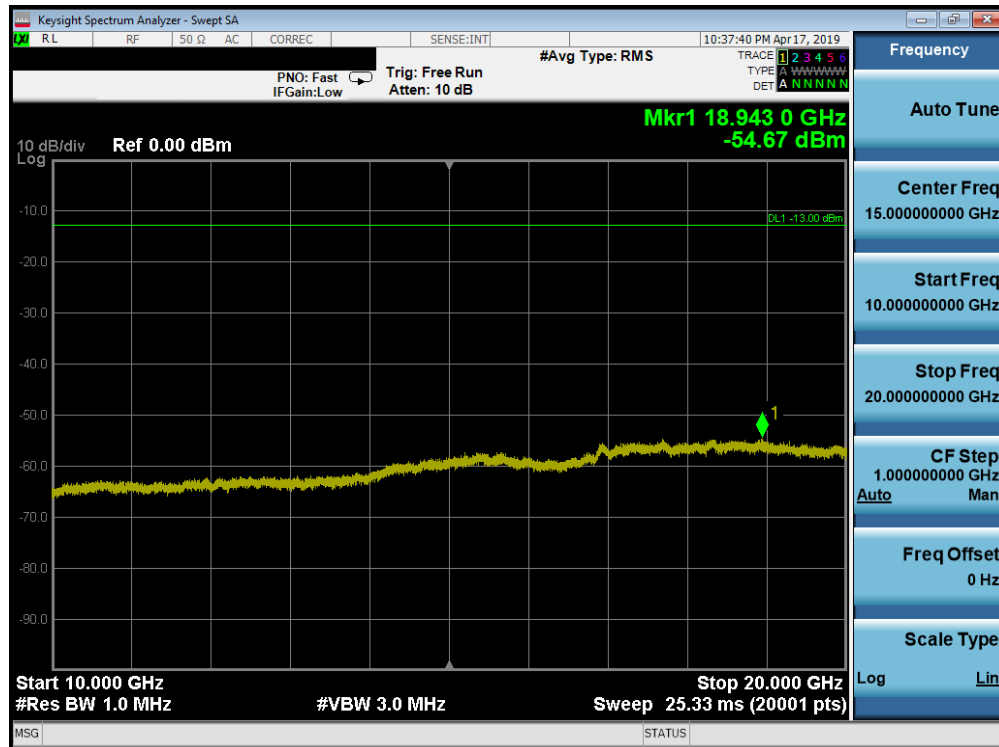
Plot 7-165. Conducted Spurious Plot (Band 25/2 - 20.0MHz QPSK - RB Size 1, RB Offset 0 - High Channel)
