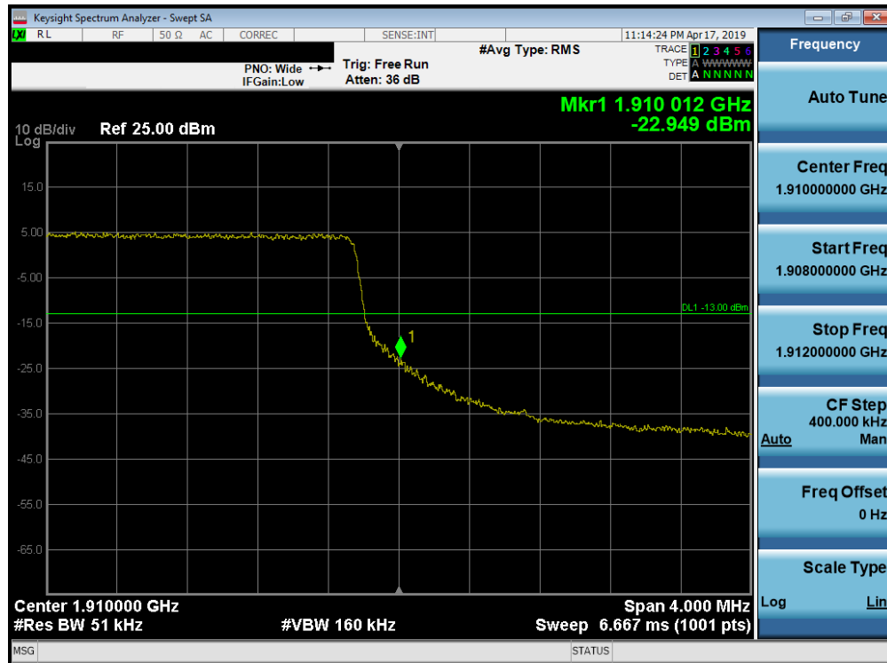
Plot 7-279. Upper Band Edge Plot (Band 2 - 5.0MHz QPSK - Full RB Configuration)
