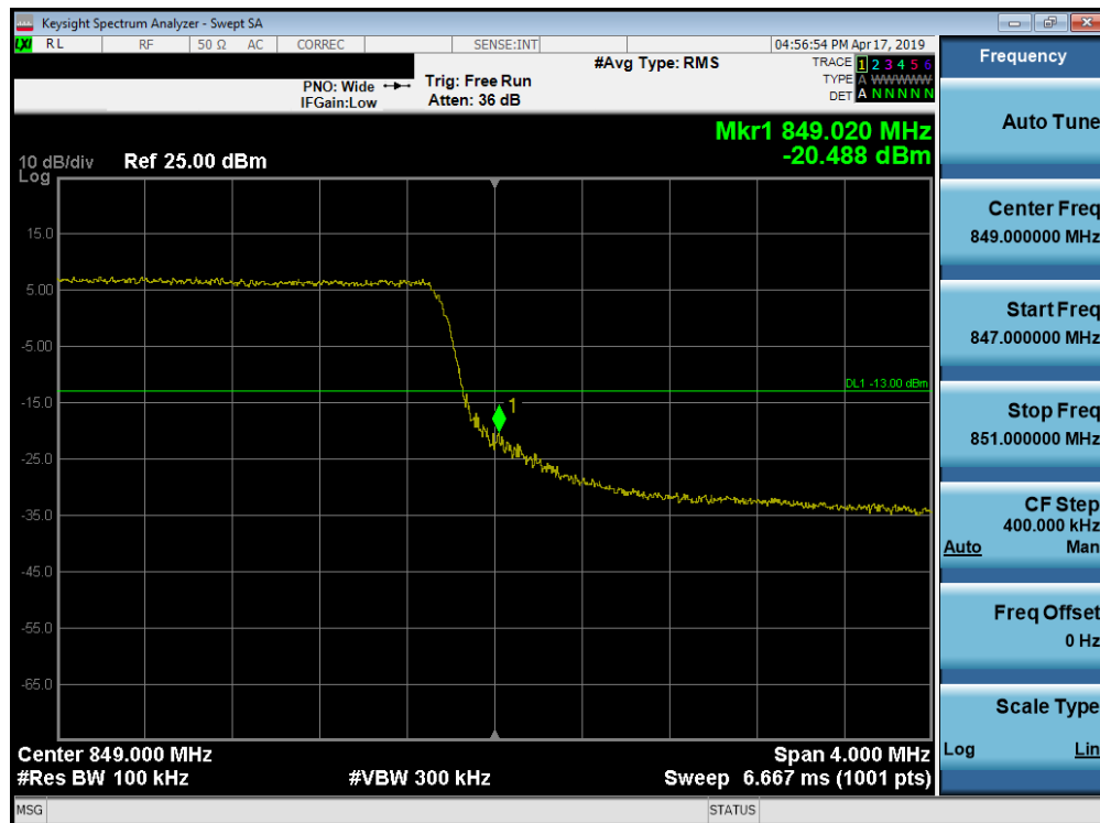
Plot 7-224. Upper Band Edge Plot (Band 26/5 - 5.0MHz QPSK - Full RB Configuration)
