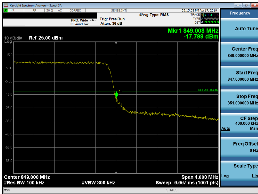
Plot 7-222. Upper Band Edge Plot (Band 26/5 - 3.0MHz QPSK - Full RB Configuration)
