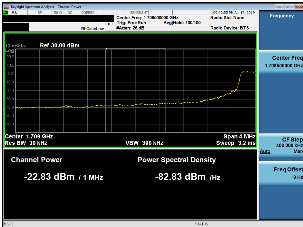
Plot 7-242. Lower Extended Band Edge Plot (Band 66/4 - 5.0MHz QPSK - Full RB Configuration)
