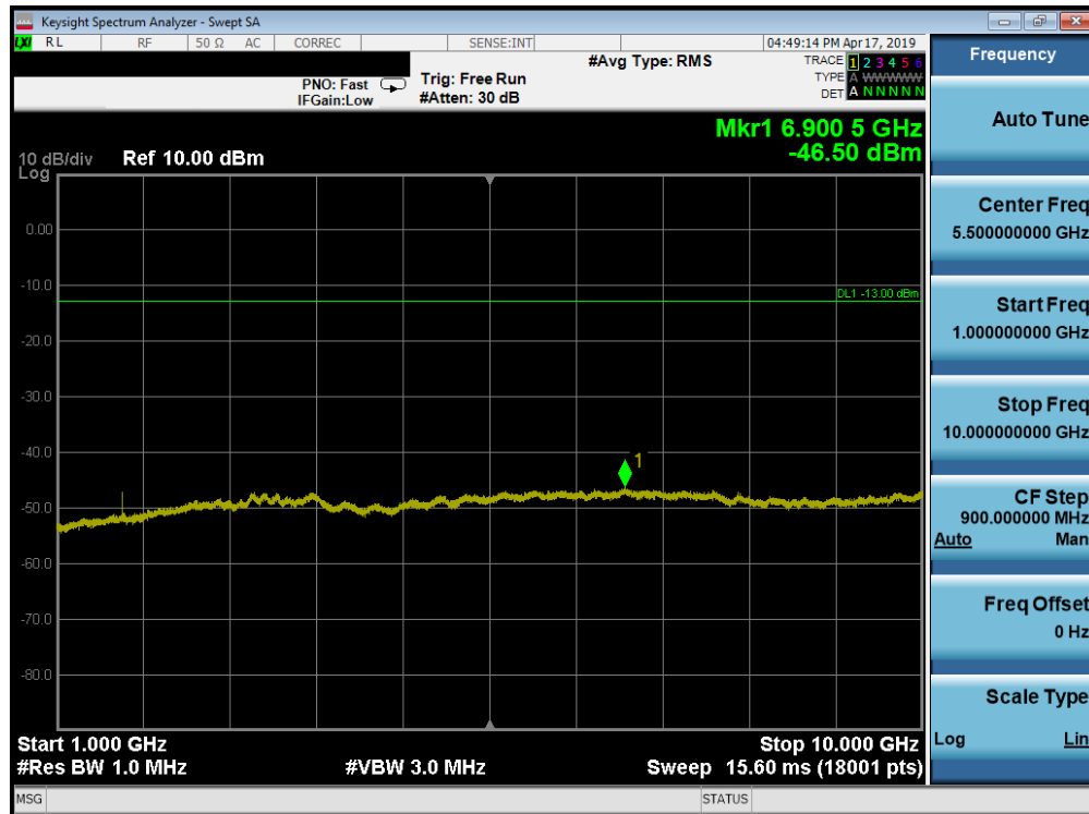
Plot 7-147. Conducted Spurious Plot (Band 26/5 - 10.0MHz QPSK - RB Size 1, RB Offset 0 - High Channel)
