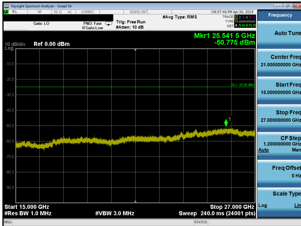
Plot 7-177. Conducted Spurious Plot (Band 41 PC2 - 20.0MHz QPSK - RB Size 1, RB Offset 0 - Low Channel)
