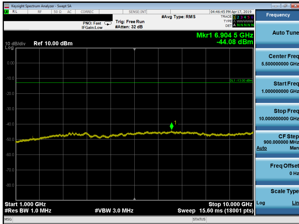
Plot 7-141. Conducted Spurious Plot (Band 26/5 - 10.0MHz QPSK - RB Size 1, RB Offset 0 - Low Channel)
