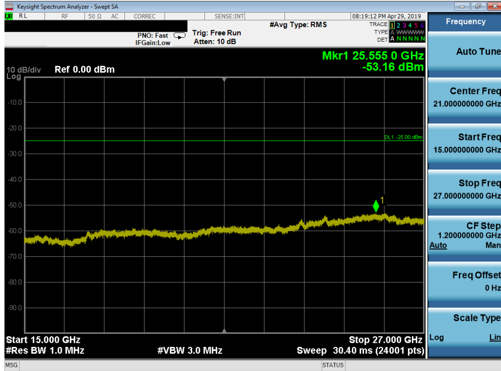
Plot 7-174. Conducted Spurious Plot (Band 7 - 20.0MHz QPSK - RB Size 1, RB Offset 0 - High Channel)
