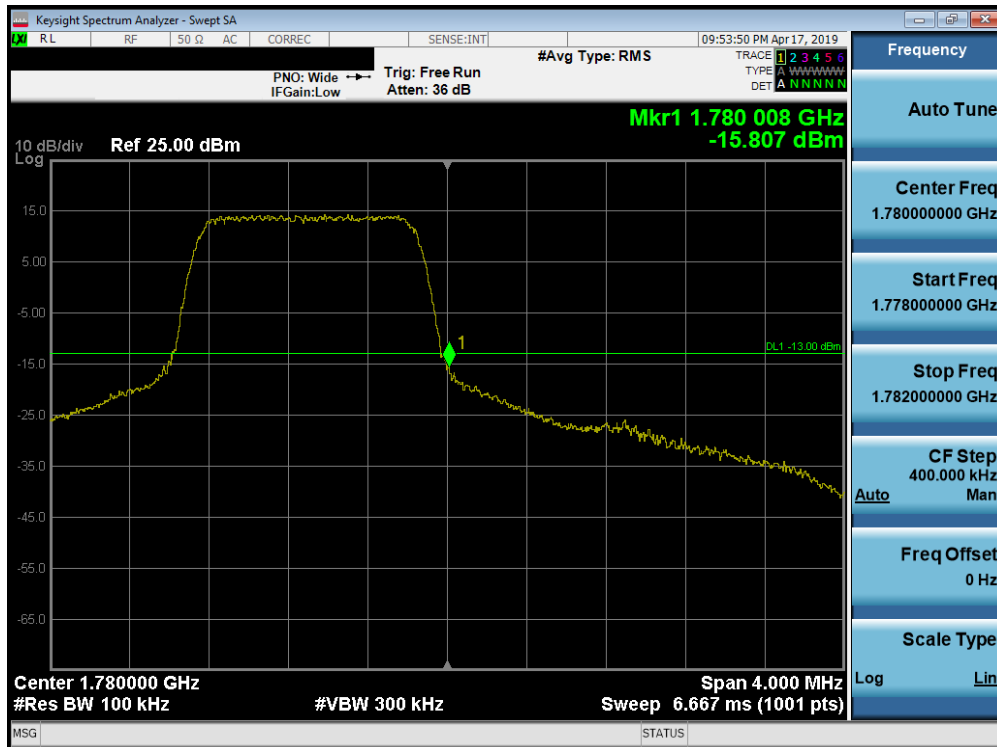
Plot 7-233. Upper Band Edge Plot (Band 66 - 1.4MHz QPSK - Full RB Configuration)
