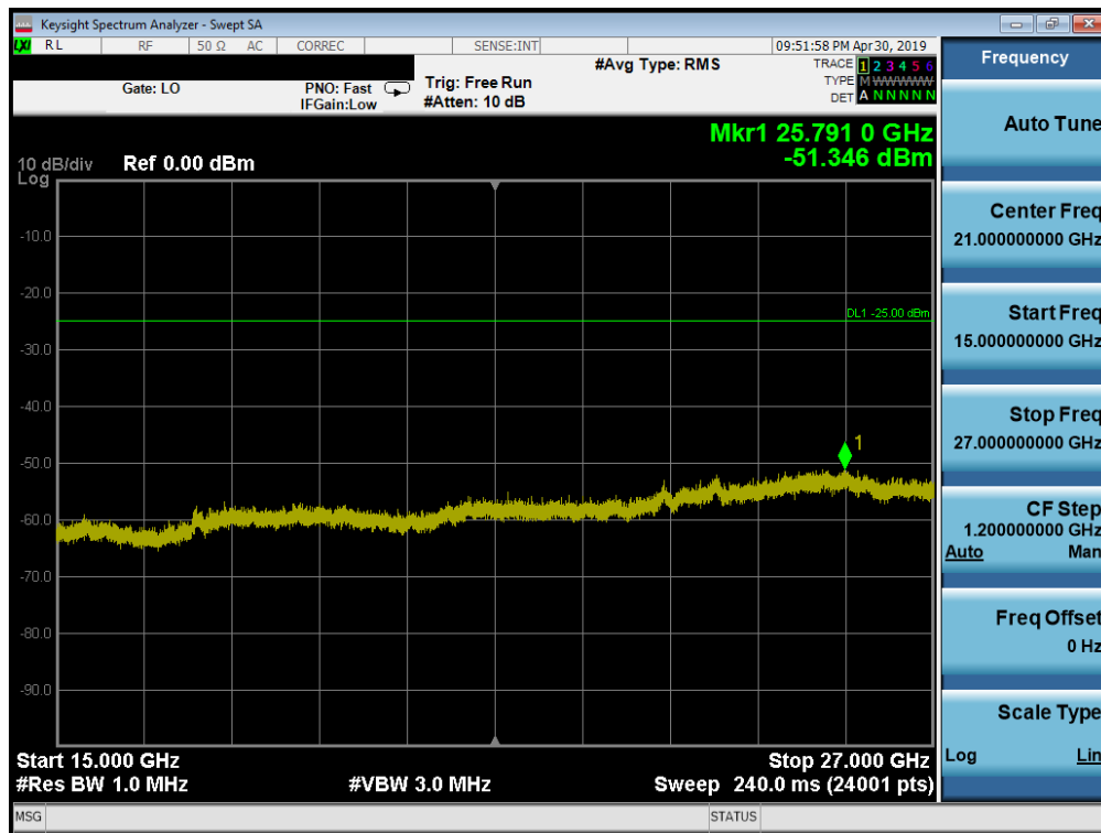
Plot 7-180. Conducted Spurious Plot (Band 41 PC2 - 20.0MHz QPSK - RB Size 1, RB Offset 0 - Mid Channel)
