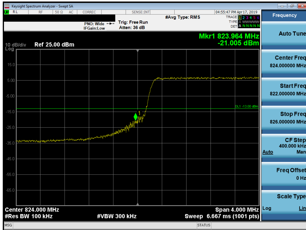
Plot 7-223. Lower Band Edge Plot (Band 26/5 - 5.0MHz QPSK - Full RB Configuration)
