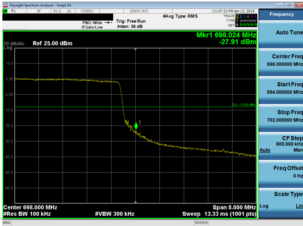
Plot 7-196. Upper Band Edge Plot (Band 71 - 10.0MHz QPSK - Full RB Configuration)
