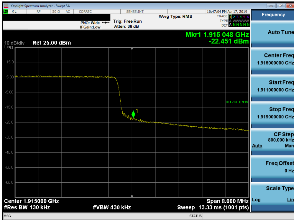
Plot 7-287. Upper Band Edge Plot (Band 25 - 10.0MHz QPSK - Full RB Configuration)
