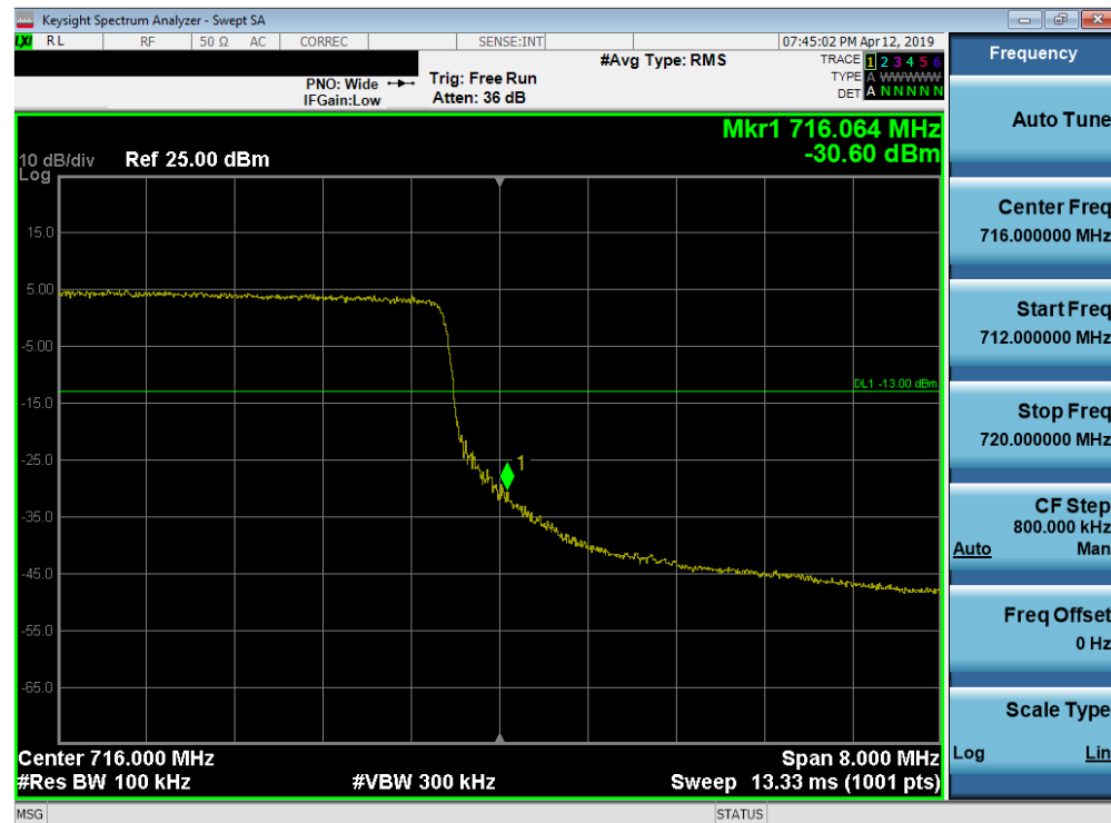
Plot 7-210. Upper Band Edge Plot (Band 12/17 - 10.0MHz QPSK - Full RB Configuration)
