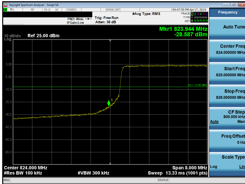
Plot 7-225. Lower Band Edge Plot (Band 26/5 - 10.0MHz QPSK - Full RB Configuration)
