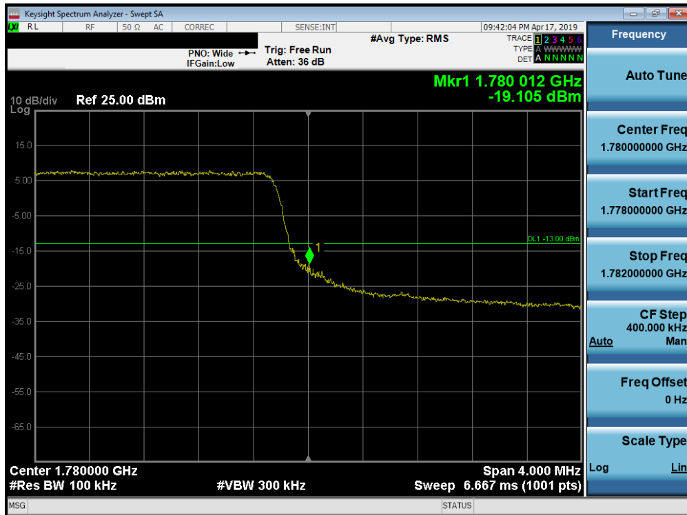
Plot 7-245. Upper Band Edge Plot (Band 66 - 5.0MHz QPSK - Full RB Configuration)
