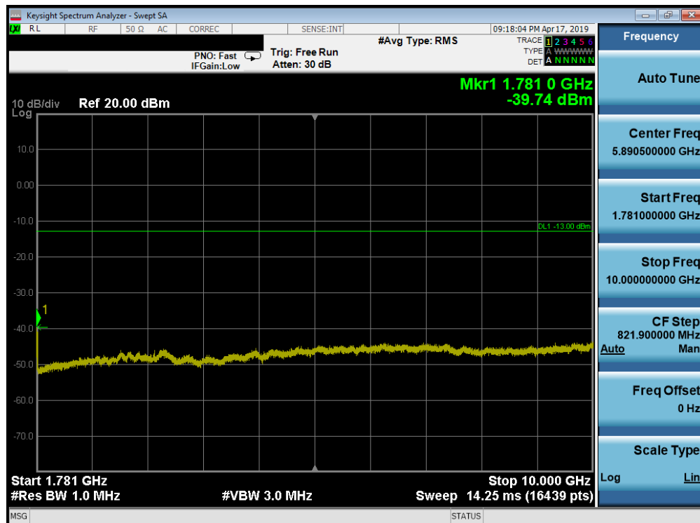
Plot 7-155. Conducted Spurious Plot (Band 66/4 - 20.0MHz QPSK - RB Size 1, RB Offset 0 - High Channel)
