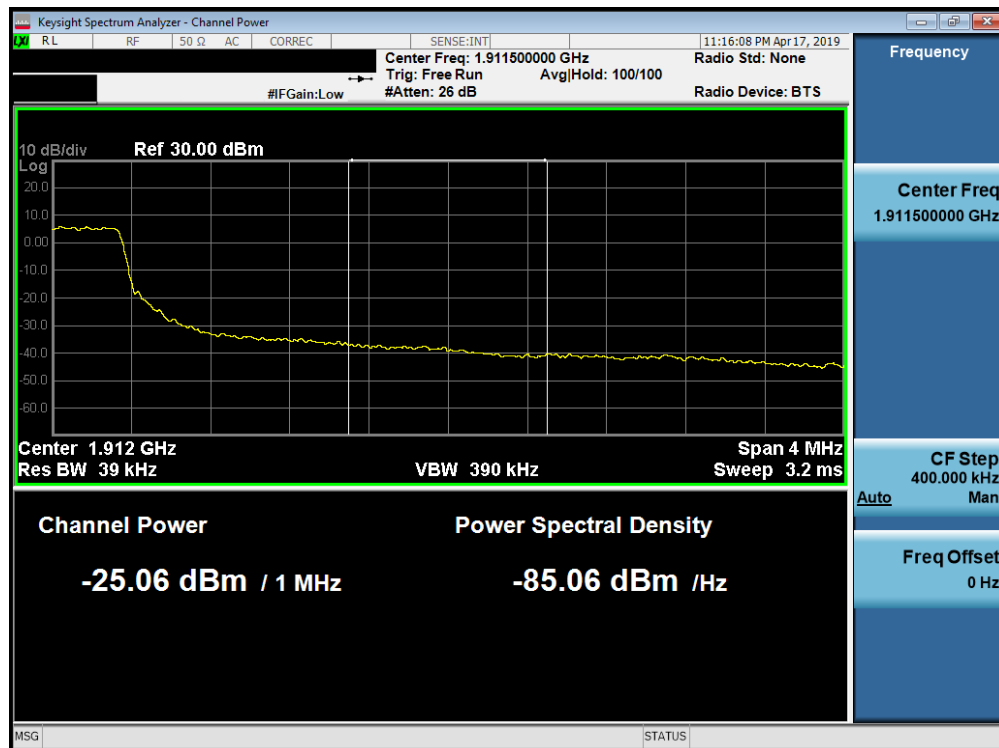
Plot 7-274. Upper Extended Band Edge Plot (Band 2 - 3.0MHz QPSK - Full RB Configuration)
