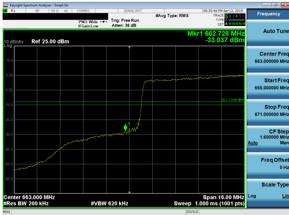
Plot 7-199. Lower Band Edge Plot (Band 71 - 20.0MHz QPSK - Full RB Configuration)
