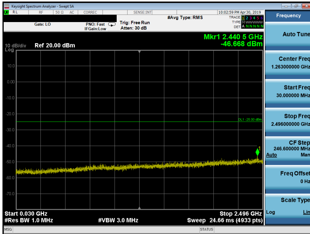
Plot 7-181. Conducted Spurious Plot (Band 41 PC2 - 20.0MHz QPSK - RB Size 1, RB Offset 0 - High Channel)
