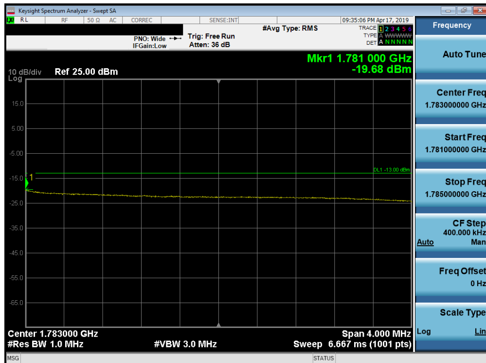
Plot 7-252. Upper Extended Band Edge Plot (Band 66 - 10.0MHz QPSK - Full RB Configuration)
