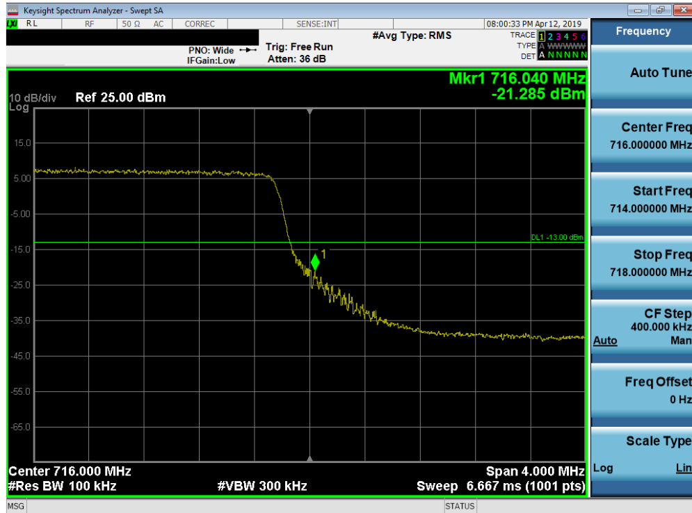
Plot 7-207. Upper Band Edge Plot (Band 12/17 - 5.0MHz QPSK - Full RB Configuration)
