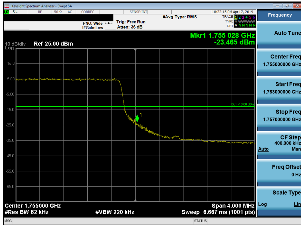
Plot 7-243. Upper Band Edge Plot (Band 4 - 5.0MHz QPSK - Full RB Configuration)
