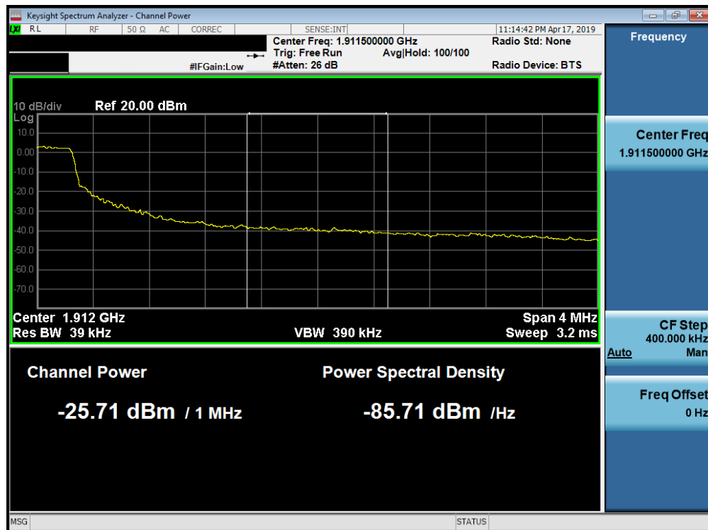
Plot 7-280. Upper Extended Band Edge Plot (Band 2 - 5.0MHz QPSK - Full RB Configuration)
