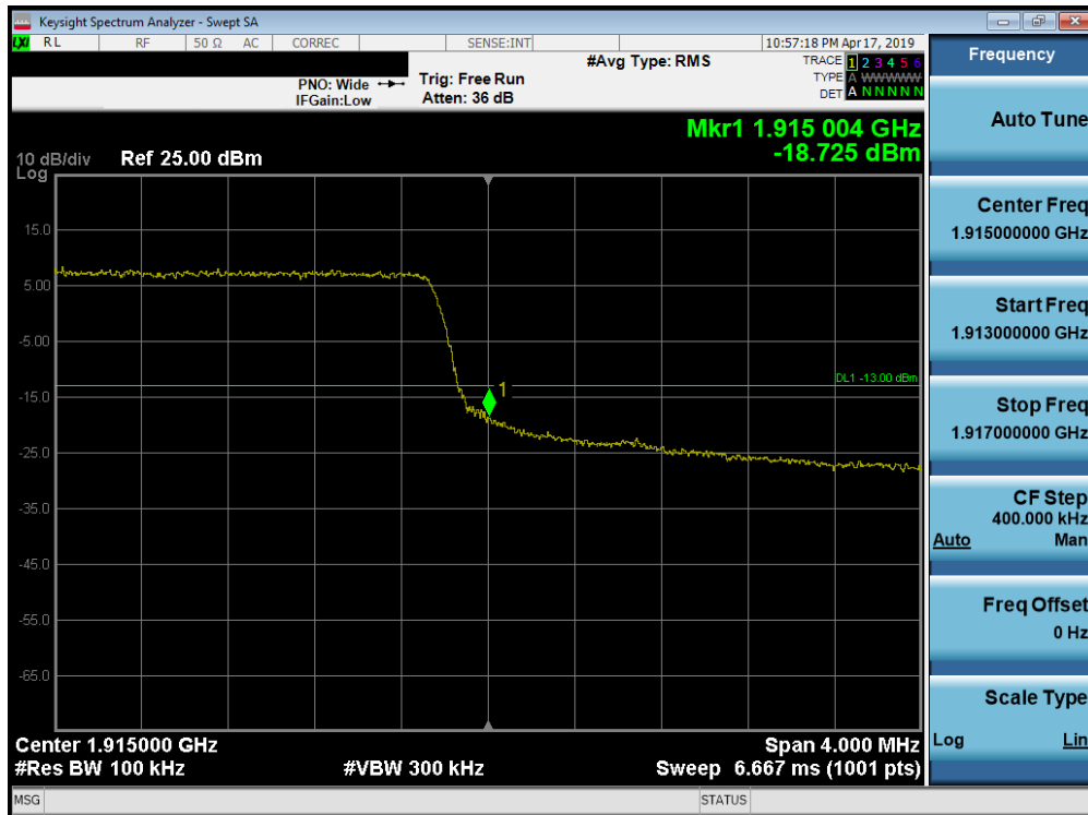
Plot 7-281. Upper Band Edge Plot (Band 25 - 5.0MHz QPSK - Full RB Configuration)
