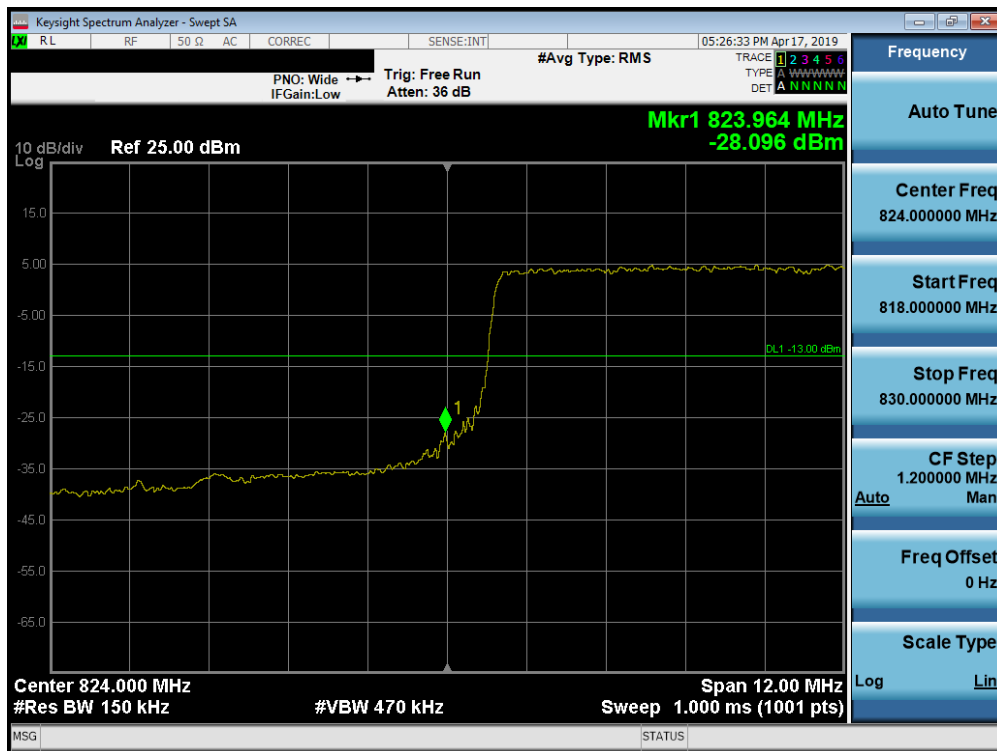
Plot 7-227. Lower Band Edge Plot (Band 26 - 15.0MHz QPSK - Full RB Configuration)
