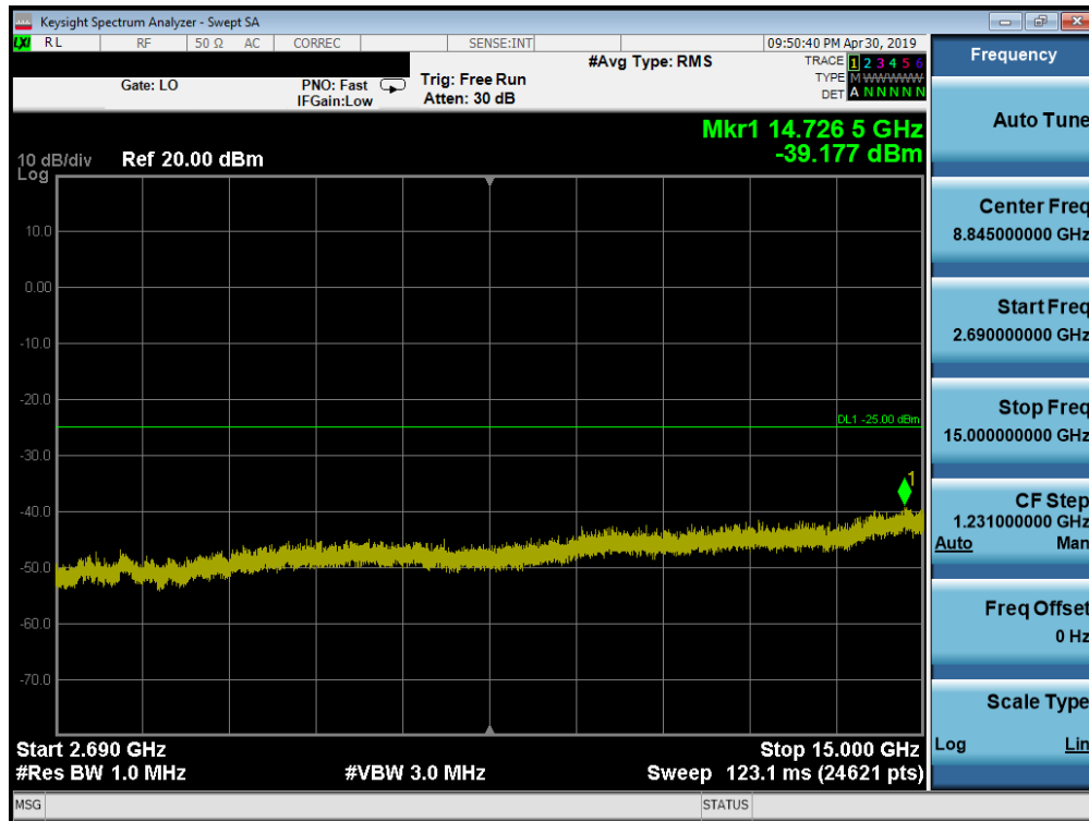
Plot 7-179. Conducted Spurious Plot (Band 41 PC2 - 20.0MHz QPSK - RB Size 1, RB Offset 0 - Mid Channel)
