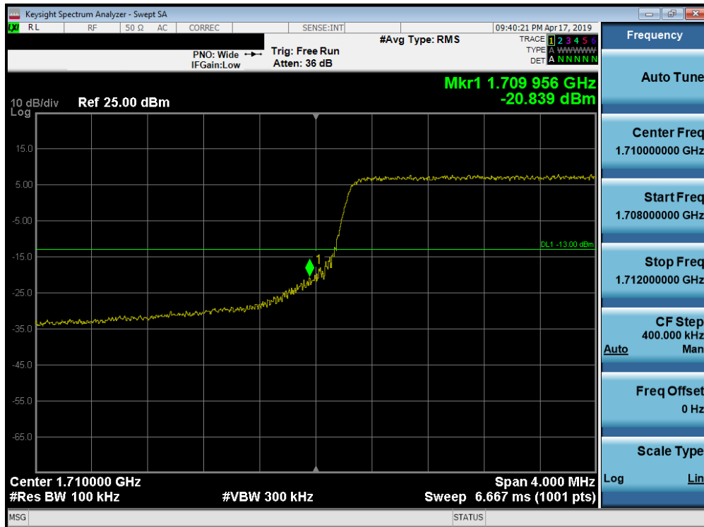
Plot 7-241. Lower Band Edge Plot (Band 66/4 - 5.0MHz QPSK - Full RB Configuration)
