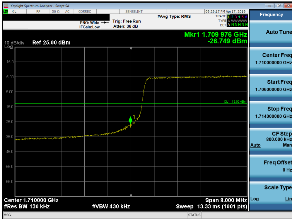
Plot 7-247. Lower Band Edge Plot (Band 66/4 - 10.0MHz QPSK - Full RB Configuration)
