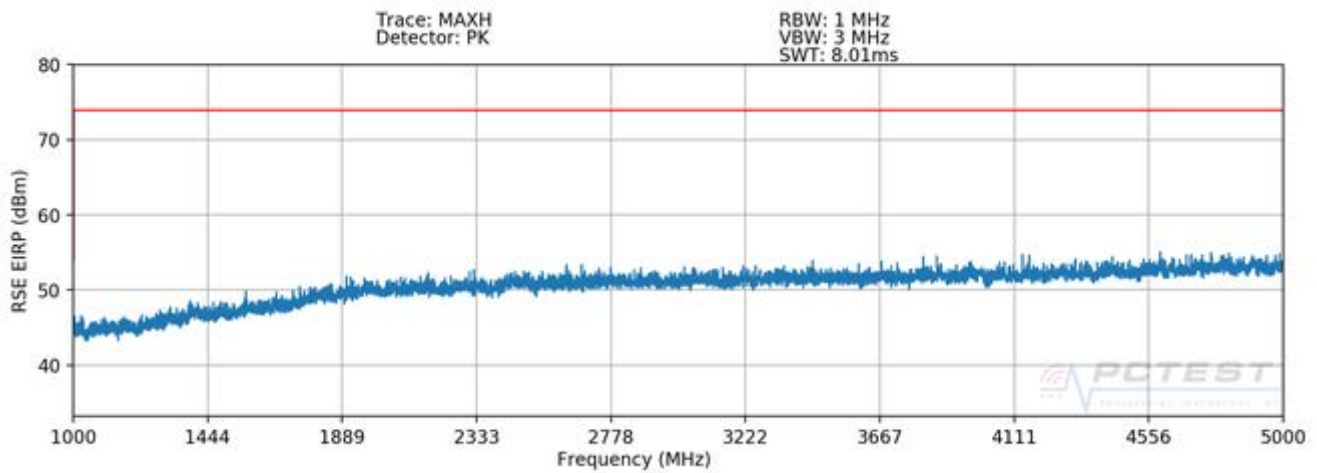
Plot 7-2. Radiated Spurious Plot above 1GHz (H)
