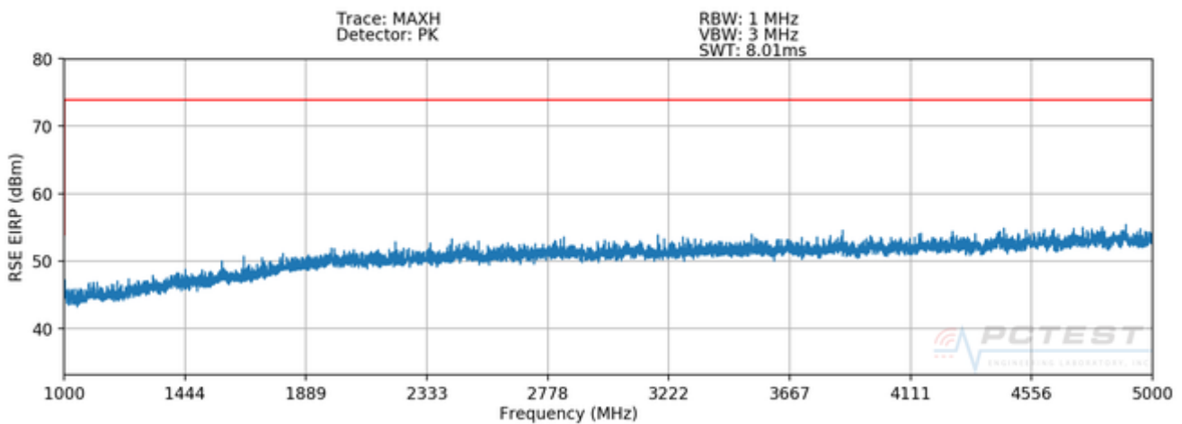
Plot 7-3. Radiated Spurious Plot above 1GHz (V)
