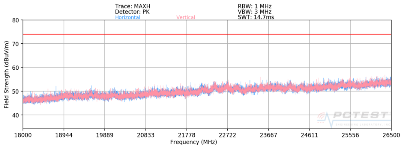
Plot 7-83. Radiated Spurious Plot 18GHz - 26.5GHz (802.11a)
