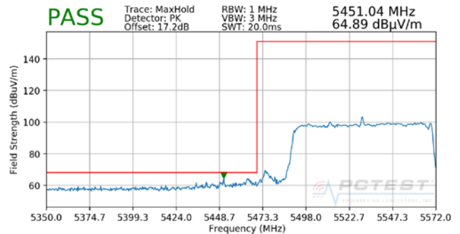
Plot 7-104. Radiated Lower Band Edge Plot (Peak – UNII Band 2C)
