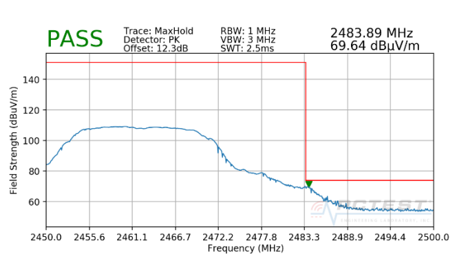
Plot 7-44. Radiated Restricted Upper Band Edge Measurement (Peak)
