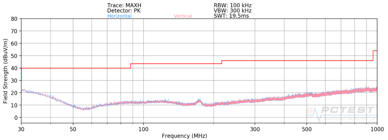
Plot 7-49. Radiated Spurious Plot below 1GHz
