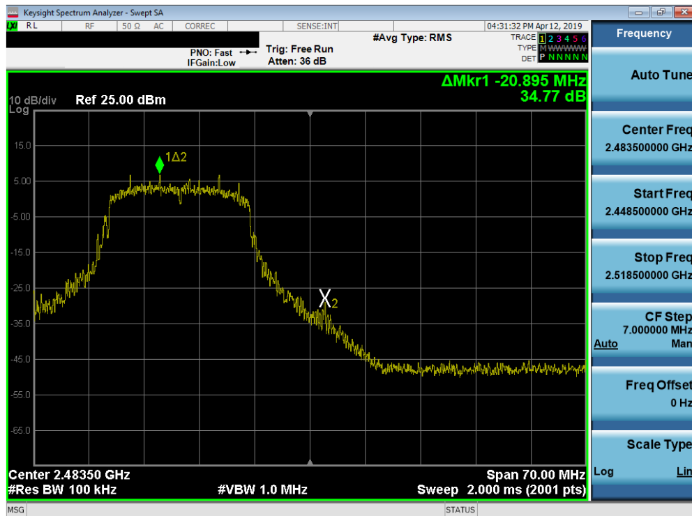
Plot 7-30. Band Edge Plot (802.11n – Ch. 13)
