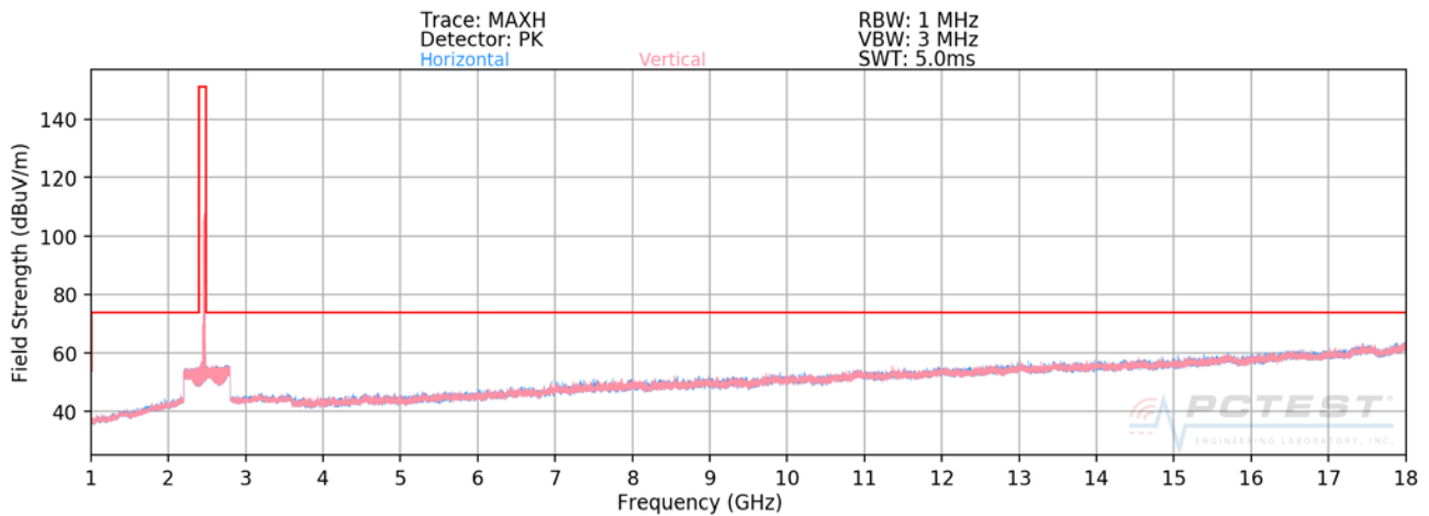
Plot 7-39. Radiated Spurious Plot above 1GHz (802.11b – Ch. 11)
