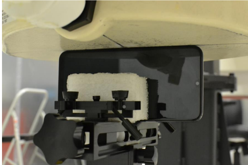
SAR Test Setup Photo 19 – Left Side at 0 mm
