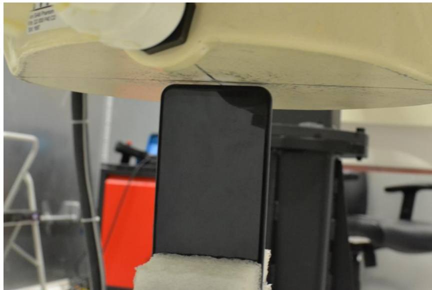
SAR Test Setup Photo 14 – Bottom Side at 2 mm
