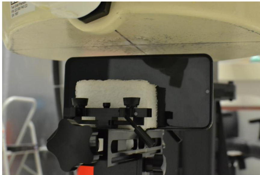
SAR Test Setup Photo 18 – Left Side at 10 mm
