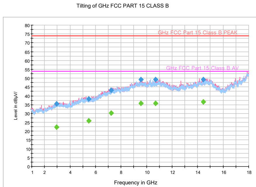
Figure 4: Radiated Emission, Receiver mode (LTE B5 Low CH Idle)
