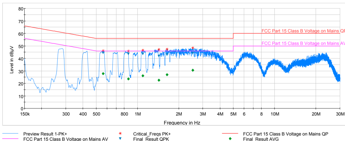
Plot 7-6. Line-Conducted Test Plot (L1)
