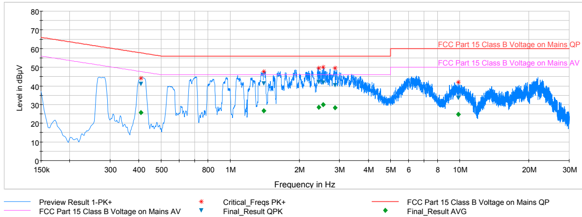
Plot 7-7. Line-Conducted Test Plot (N)
