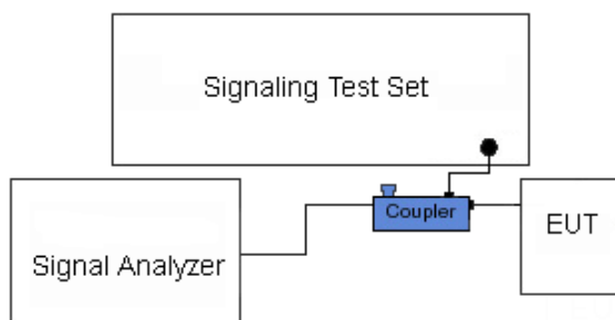
Figure 7-5. Test Instrument & Measurement Setup
