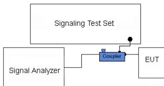
Figure 7-4. Test Instrument & Measurement Setup
