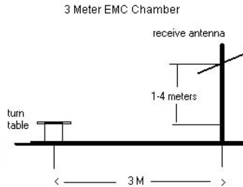
Figure 7-8. Test Instrument & Measurement Setup
