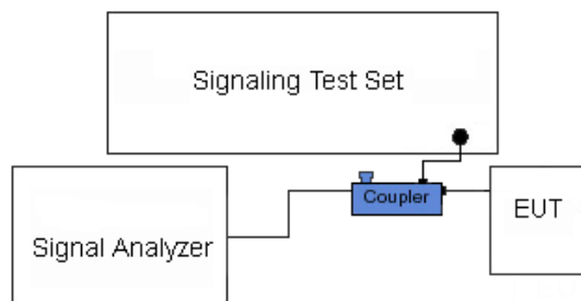
Figure 7-7. Test Instrument & Measurement Setup
