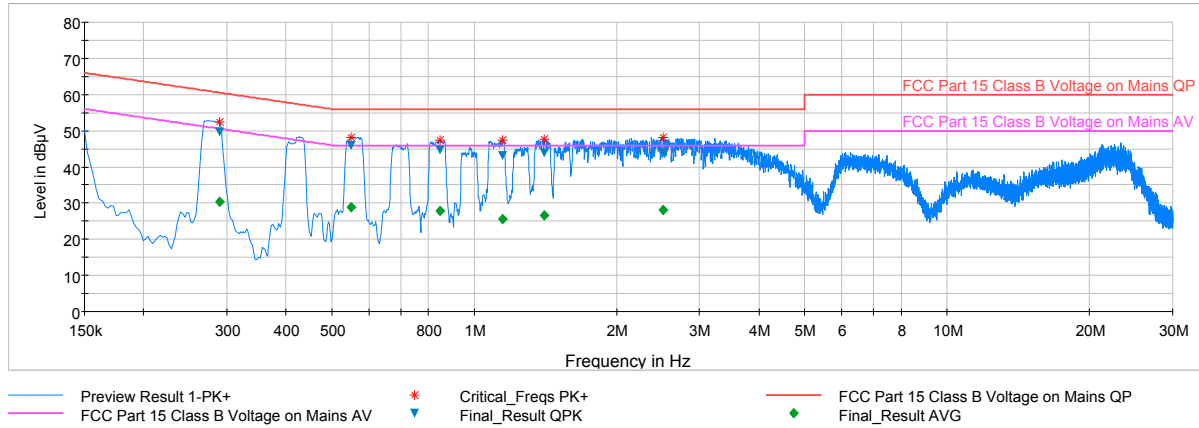
Plot 7-54. Line-Conducted Test Plot (L1)
