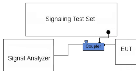
Figure 7-6. Test Instrument & Measurement Setup
