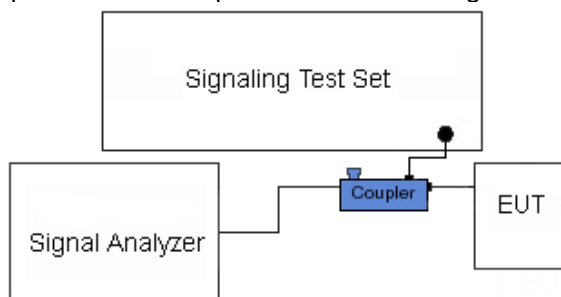
Figure 7-1. Test Instrument & Measurement Setup
