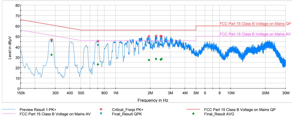
Plot 7-55. Line-Conducted Test Plot (N)
