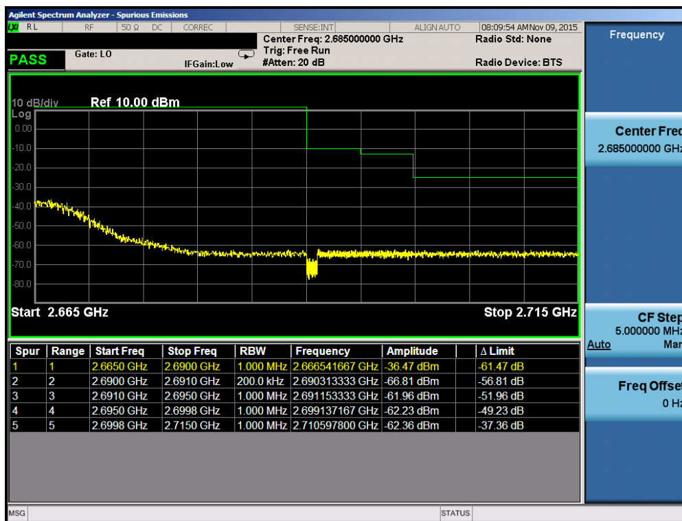
Plot 7-21. Upper ACP Plot (Band 41 – 10.0MHz QPSK – RB Size 50)
