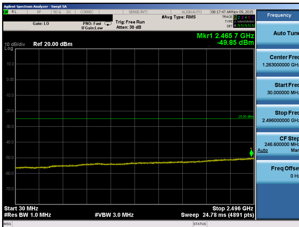
Plot 7-12. Conducted Spurious Plot (Band 41 – 20.0MHz QPSK – RB Size 1, RB Offset 0 – Mid Channel)
