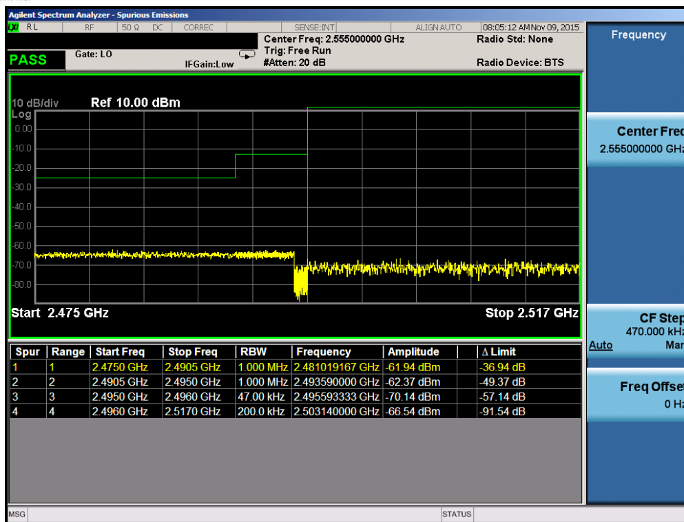
Plot 7-18. Lower ACP Plot (Band 41 – 5.0MHz QPSK – RB Size 25)
