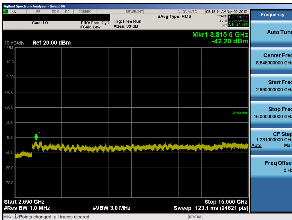
Plot 7-10. Conducted Spurious Plot (Band 41 – 20.0MHz QPSK – RB Size 1, RB Offset 0 – Low Channel)
