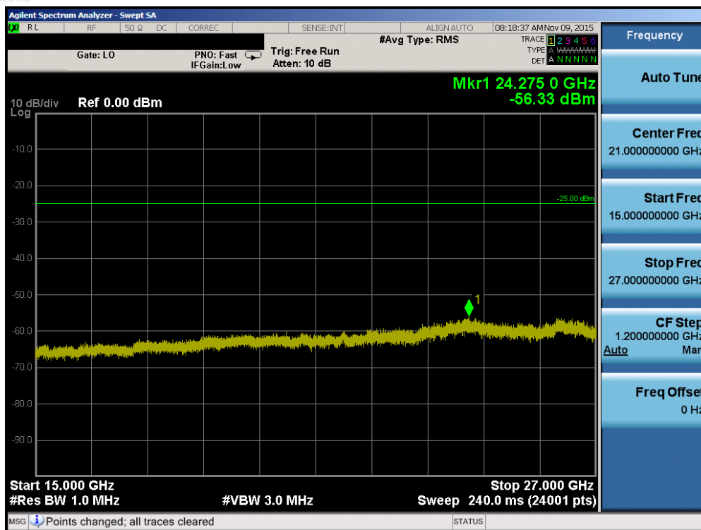
Plot 7-11. Conducted Spurious Plot (Band 41 – 20.0MHz QPSK – RB Size 1, RB Offset 0 – Low Channel)
