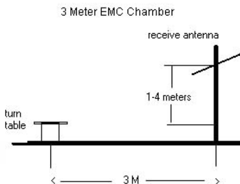
Figure 7-4. Test Instrument & Measurement Setup
