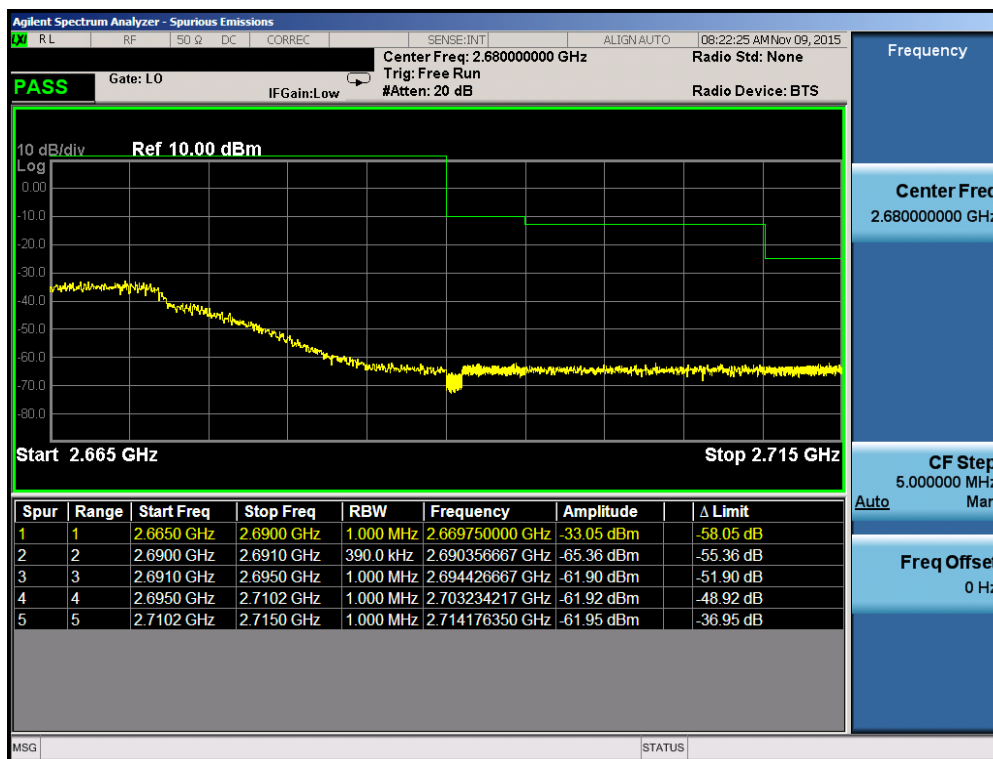
Plot 7-25. Upper ACP Plot (Band 41 – 20.0MHz QPSK – RB Size 100)
