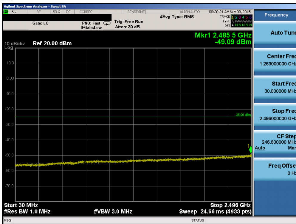
Plot 7-15. Conducted Spurious Plot (Band 41 – 20.0MHz QPSK – RB Size 1, RB Offset 0 – High Channel)
