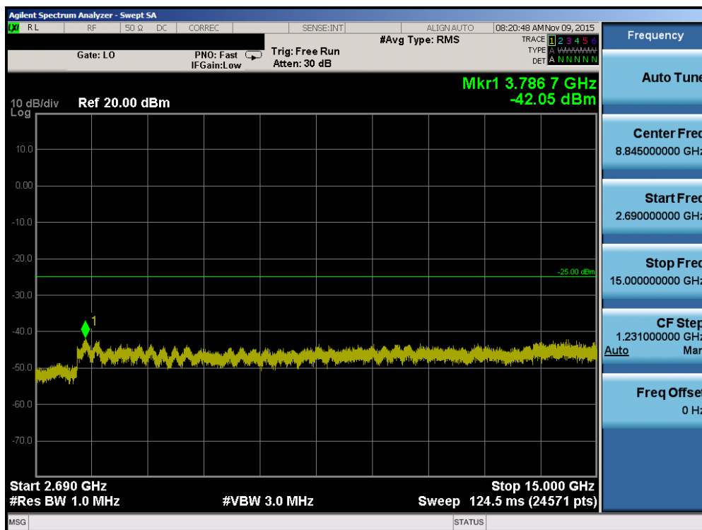
Plot 7-16. Conducted Spurious Plot (Band 41 – 20.0MHz QPSK – RB Size 1, RB Offset 0 – High Channel)
