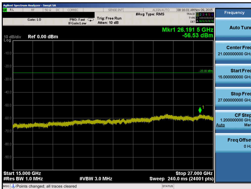
Plot 7-14. Conducted Spurious Plot (Band 41 – 20.0MHz QPSK – RB Size 1, RB Offset 0 – Mid Channel)
