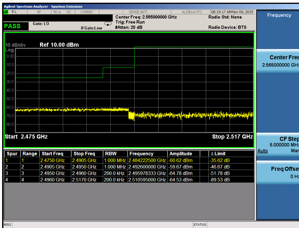
Plot 7-24. Lower ACP Plot (Band 41 – 20.0MHz QPSK – RB Size 100)
