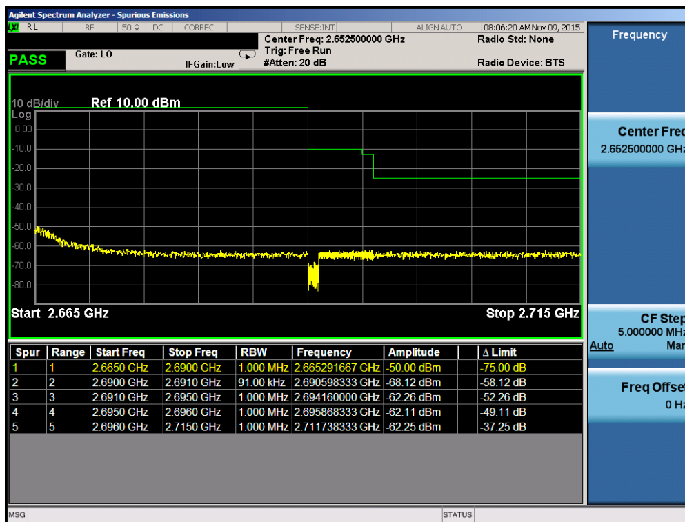
Plot 7-19. Upper ACP Plot (Band 41 – 5.0MHz QPSK – RB Size 25)
