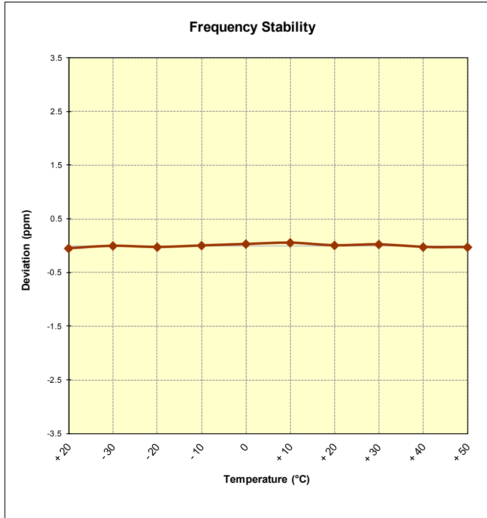
Figure 7-6. Frequency Stability Graph (Band 41)
