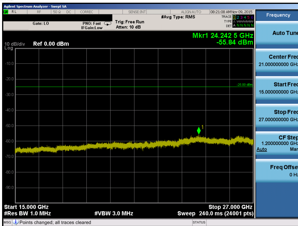
Plot 7-17. Conducted Spurious Plot (Band 41 – 20.0MHz QPSK – RB Size 1, RB Offset 0 – High Channel)
