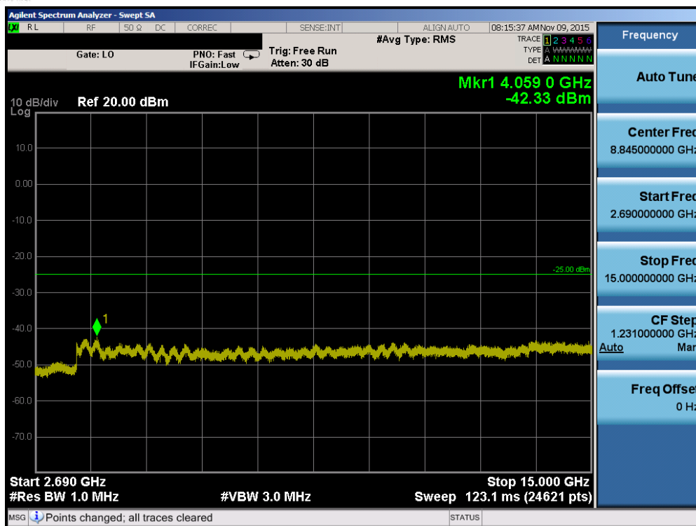
Plot 7-13. Conducted Spurious Plot (Band 41 – 20.0MHz QPSK – RB Size 1, RB Offset 0 – Mid Channel)
