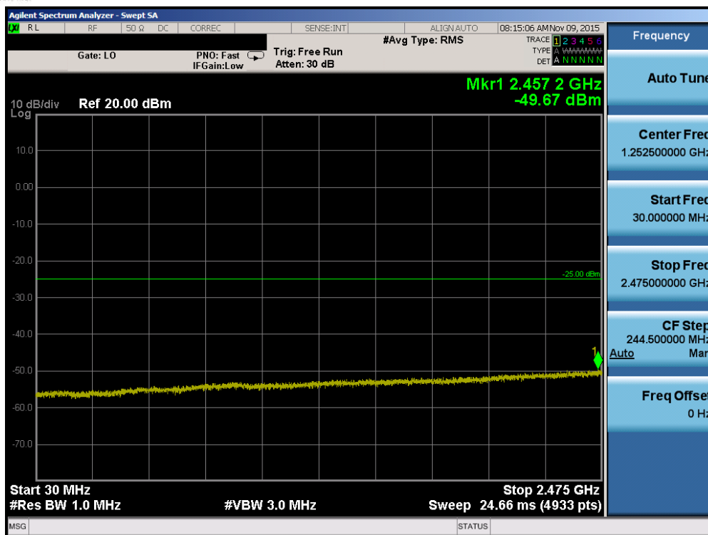
Plot 7-9. Conducted Spurious Plot (Band 41 – 20.0MHz QPSK – RB Size 1, RB Offset 0– Low Channel)
