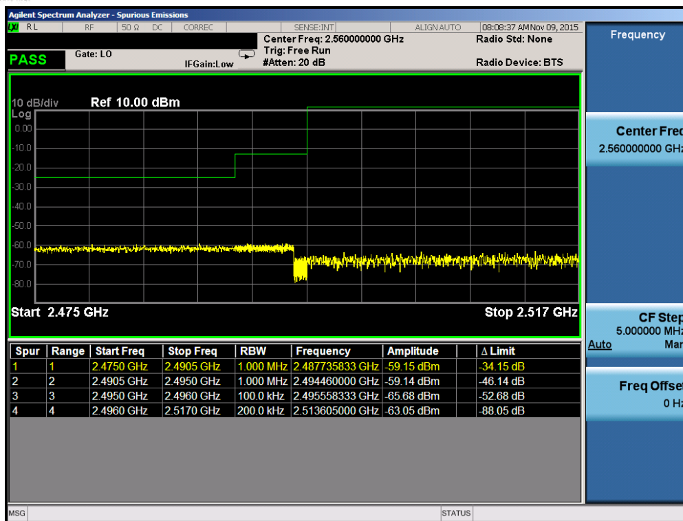
Plot 7-20. Lower ACP Plot (Band 41 – 10.0MHz QPSK – RB Size 50)
