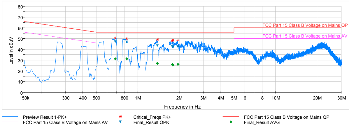
Plot 7-102. Line Conducted Plot with 802.11a UNII Band 3 (N)
