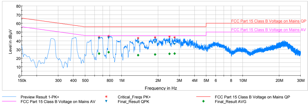
Plot 7-101. Line Conducted Plot with 802.11a UNII Band 3 (L1)
