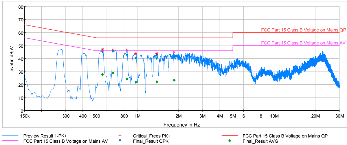
Plot 7-97. Line Conducted Plot with 802.11a UNII Band 2A (L1)
