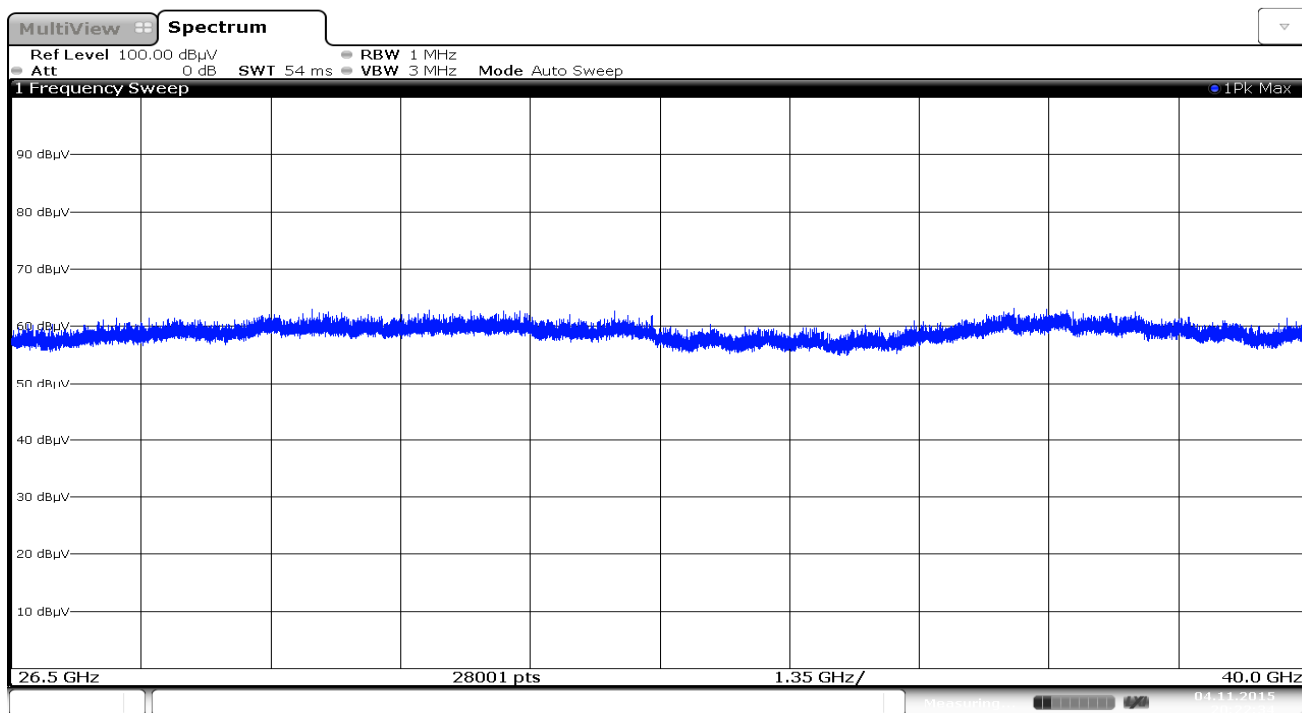
Plot 7-78. Radiated Spurious Plot above 18GHz (802.11a – Ant. Pol. V)
