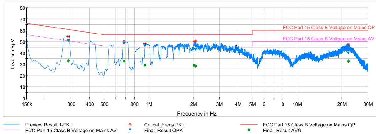
Plot 7-100. Line Conducted Plot with 802.11a UNII Band 2C (N)
