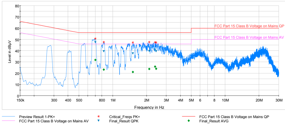
Plot 7-98. Line Conducted Plot with 802.11a UNII Band 2A (N)
