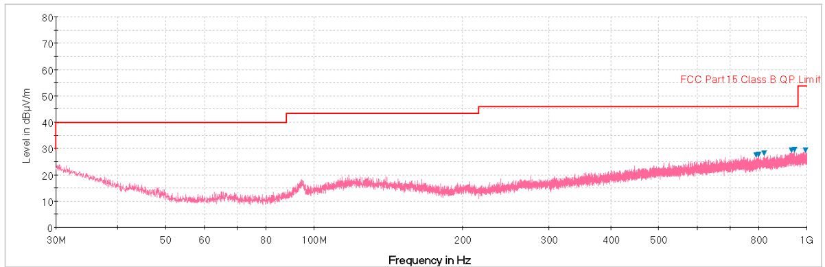
Plot 7-94. Radiated Spurious Plot below 1GHz (802.11a – U3 Ch. 157, Ant. Pol. V)
