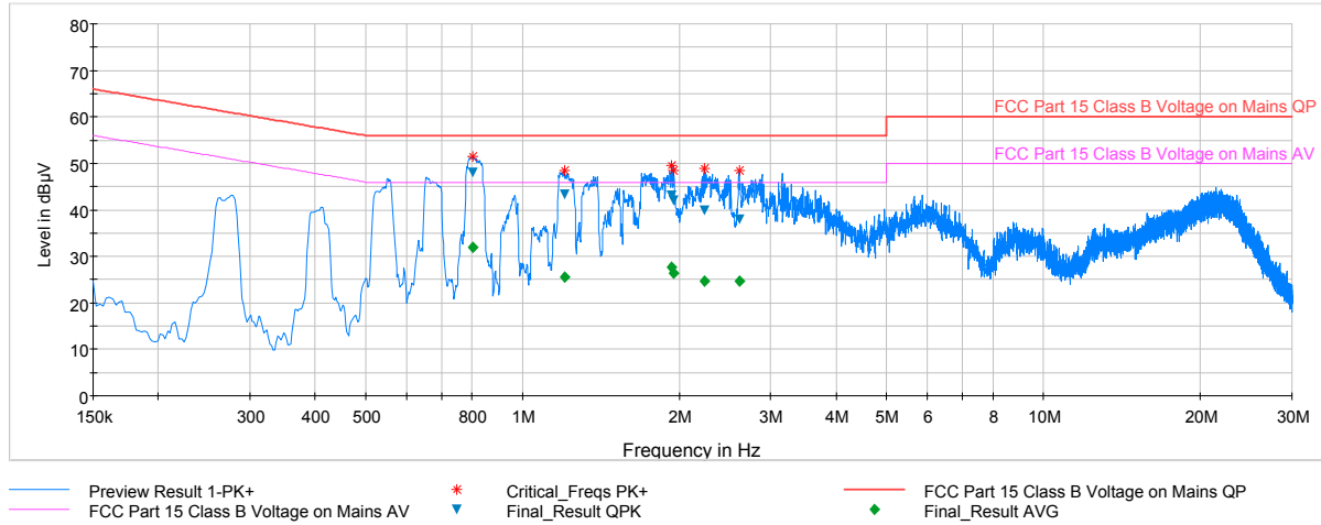
Plot 7-96. Line Conducted Plot with 802.11a UNII Band 1 (N)
