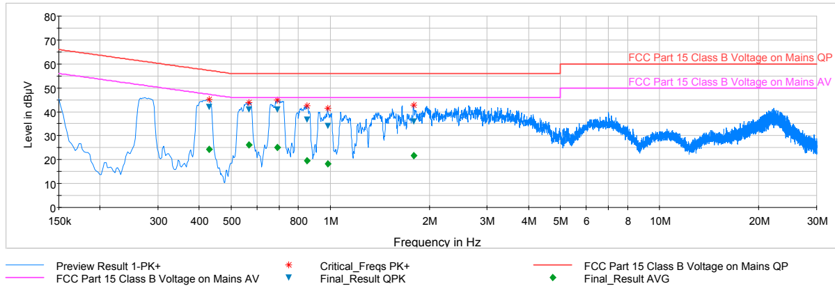
Plot 7-99. Line Conducted Plot with 802.11a UNII Band 2C (L1)
