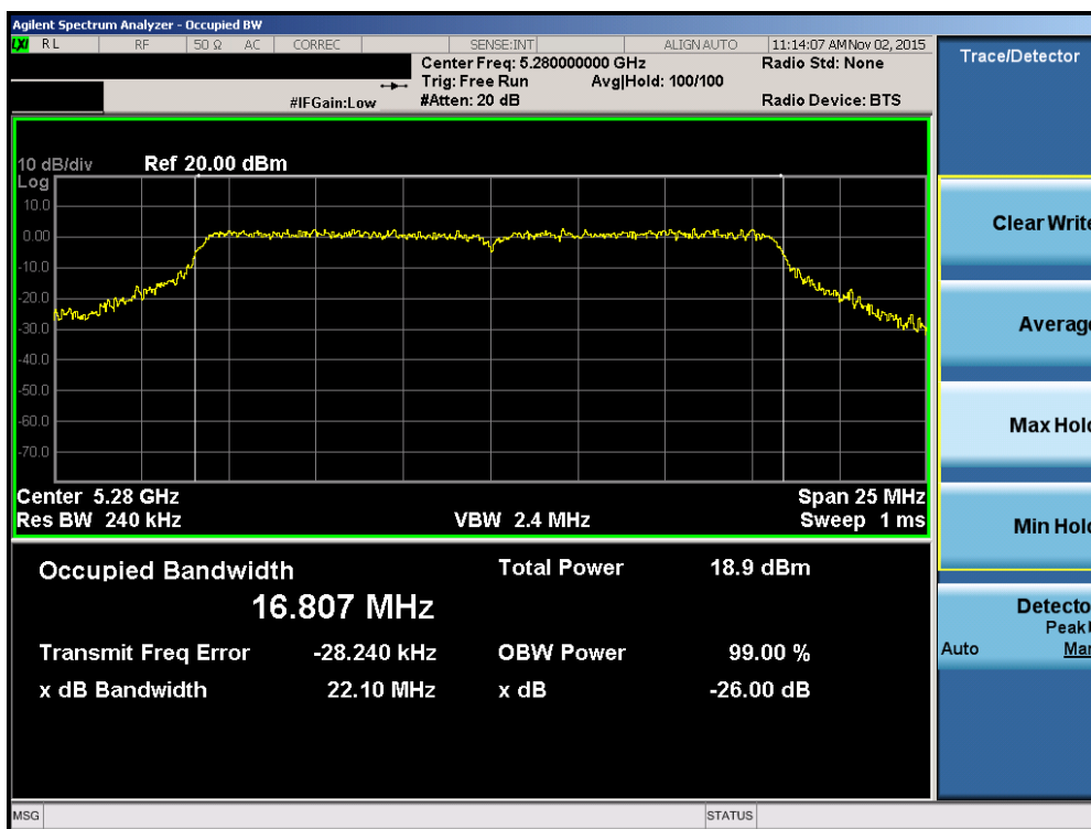
Plot 7-10. 26dB Bandwidth Plot (802.11a (UNII Band 2A) – Ch. 56)
