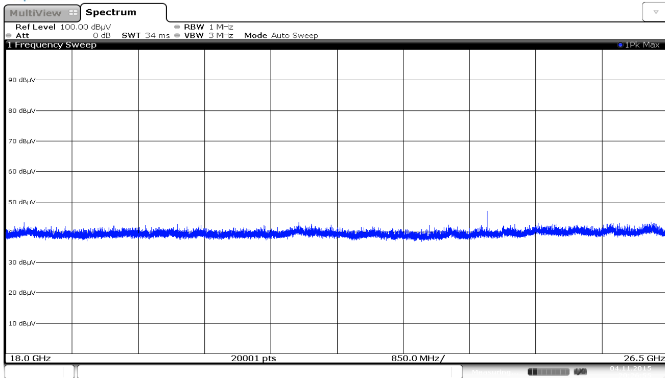
Plot 7-77. Radiated Spurious Plot above 18GHz (802.11a – Ant. Pol. V)
