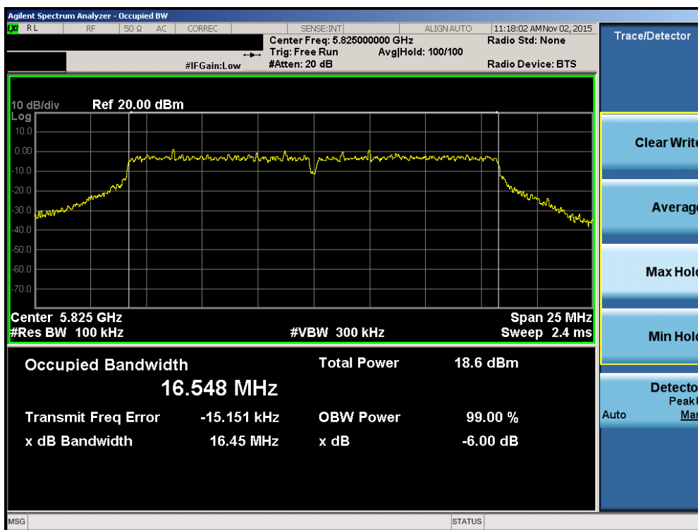
Plot 7-28. 6dB Bandwidth Plot (802.11a (UNII Band 3) – Ch. 165)
