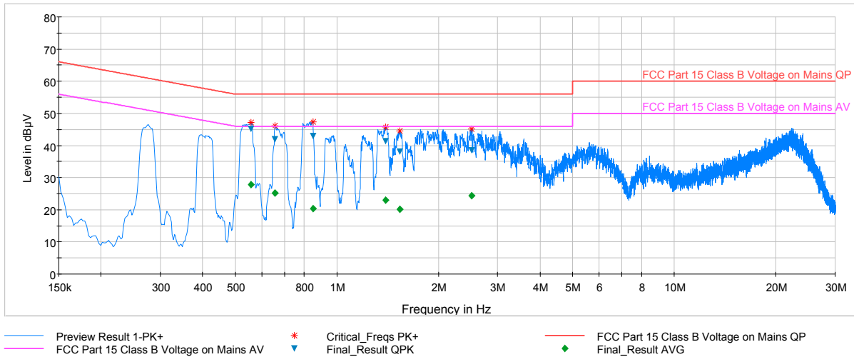
Plot 7-95. Line Conducted Plot with 802.11a UNII Band 1 (L1)
