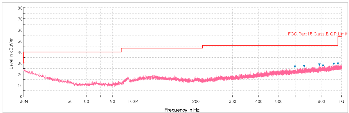
Plot 7-44. Radiated Spurious Plot below 1GHz (Pol. V)
