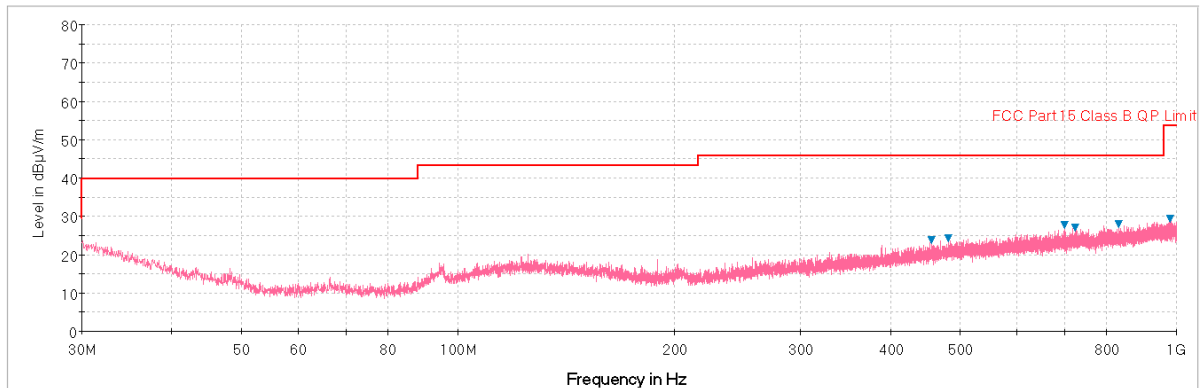
Plot 7-43. Radiated Spurious Plot below 1GHz (Pol. H)
