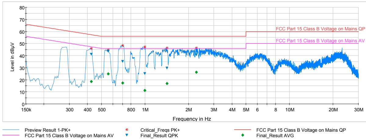
Plot 7-45. Line Conducted Plot with 802.11b (L1)
