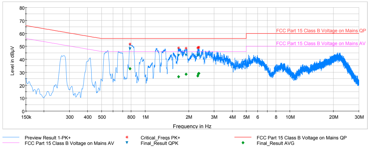
Plot 7-46. Line Conducted Plot with 802.11b (N)
