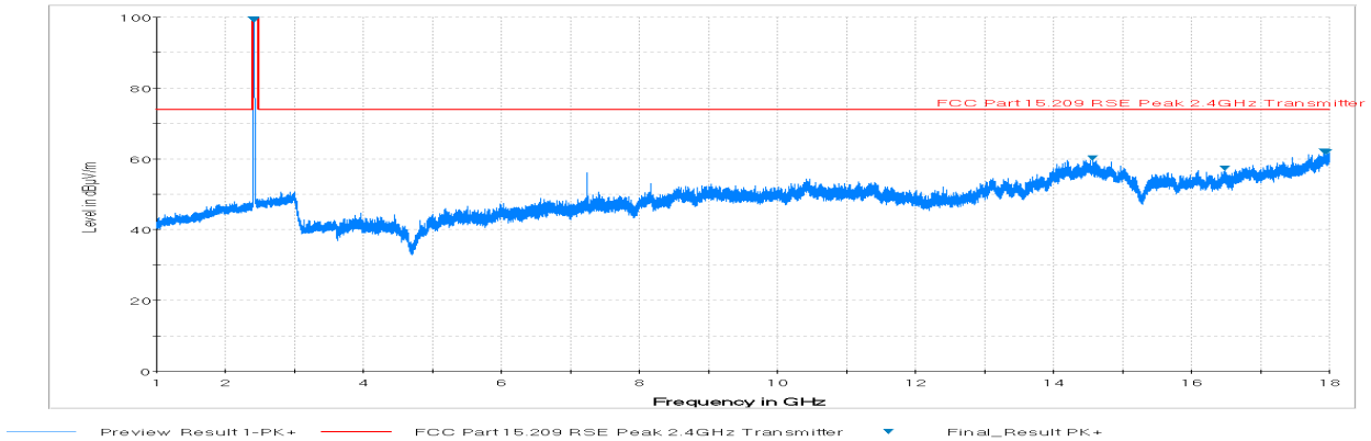
Plot 7-31. Radiated Spurious Plot above 1GHz (802.11b – Ch. 1, Ant. Pol. H)
