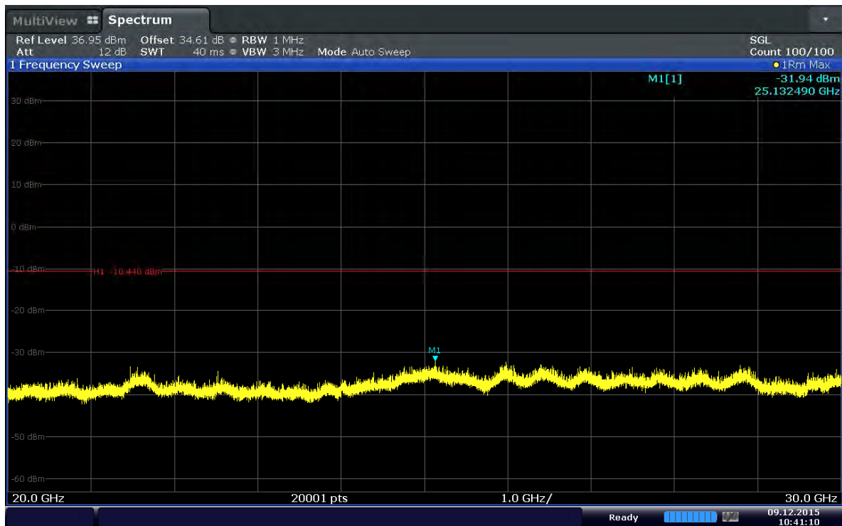
Plot 6-29. Conducted Spurious Plot (Band 41–15MHz–QPSK–RB Size 1–RB Offset 0–Ch.40315)
