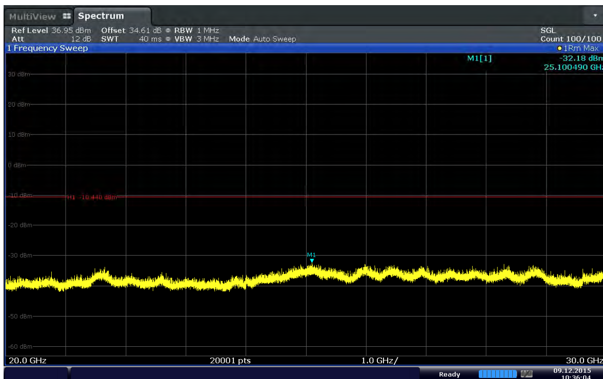
Plot 6-20. Conducted Spurious Plot (Band 41–10MHz–QPSK– RB Size 1–RB Offset 0–Ch.40290)
