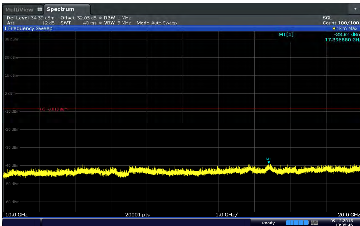
Plot 6-19. Conducted Spurious Plot (Band 41–10MHz–QPSK– RB Size 1–RB Offset 0–Ch.40290)
