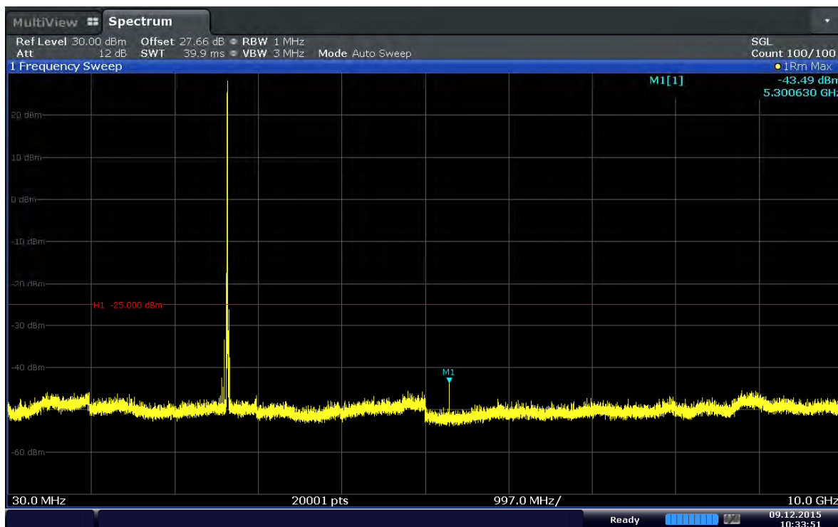
Plot 6-15. Conducted Spurious Plot (Band 41–5MHz–QPSK–RB Size 1–RB Offset 0–Ch.41215)
