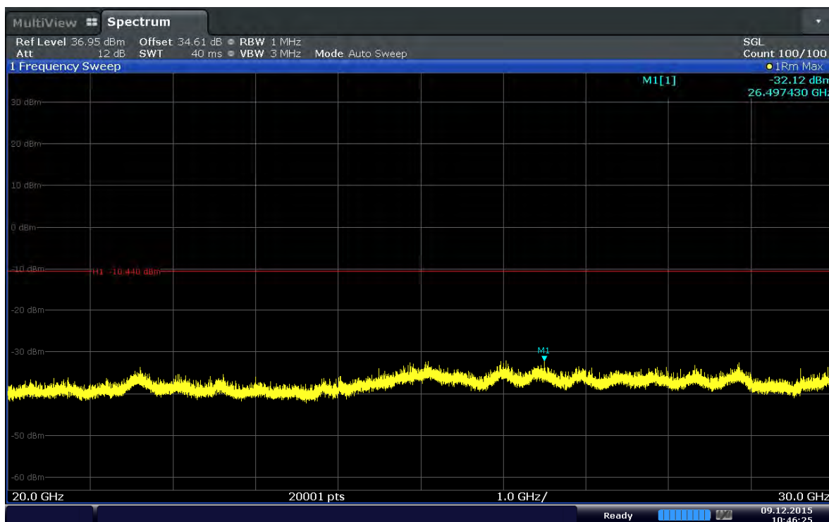
Plot 6-38. Conducted Spurious Plot (Band 41–20MHz–QPSK–RB Size 1–RB Offset 0–Ch.40340)
