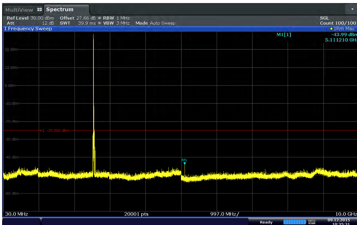
Plot 6-18. Conducted Spurious Plot (Band 41–10MHz–QPSK–RB Size 1–RB Offset 0–Ch.40290)
