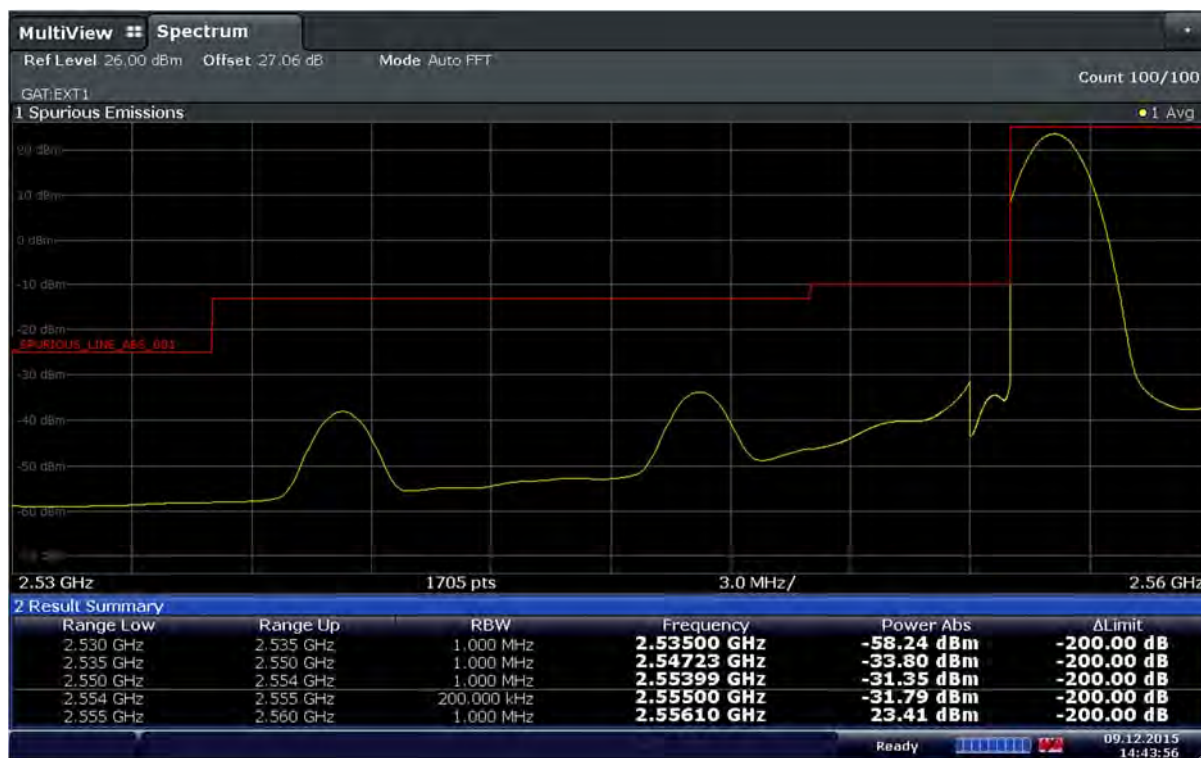
Plot 6-53. Lower Band Edge Plot (Band41 – 20MHz – QPSK – RB Size 1 – RB Offset 0 – Ch.40340)
