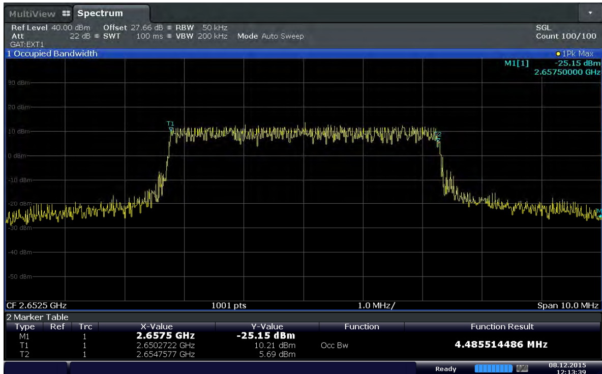
Plot 6-1. Occupied Bandwidth Plot (Band 41 – 5MHz QPSK - RB Size 25)
