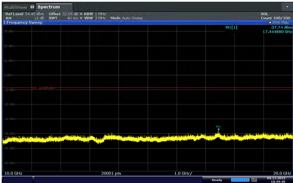
Plot 6-43. Conducted Spurious Plot (Band 41–20MHz–QPSK–RB Size 1–RB Offset 0–Ch.41140)
