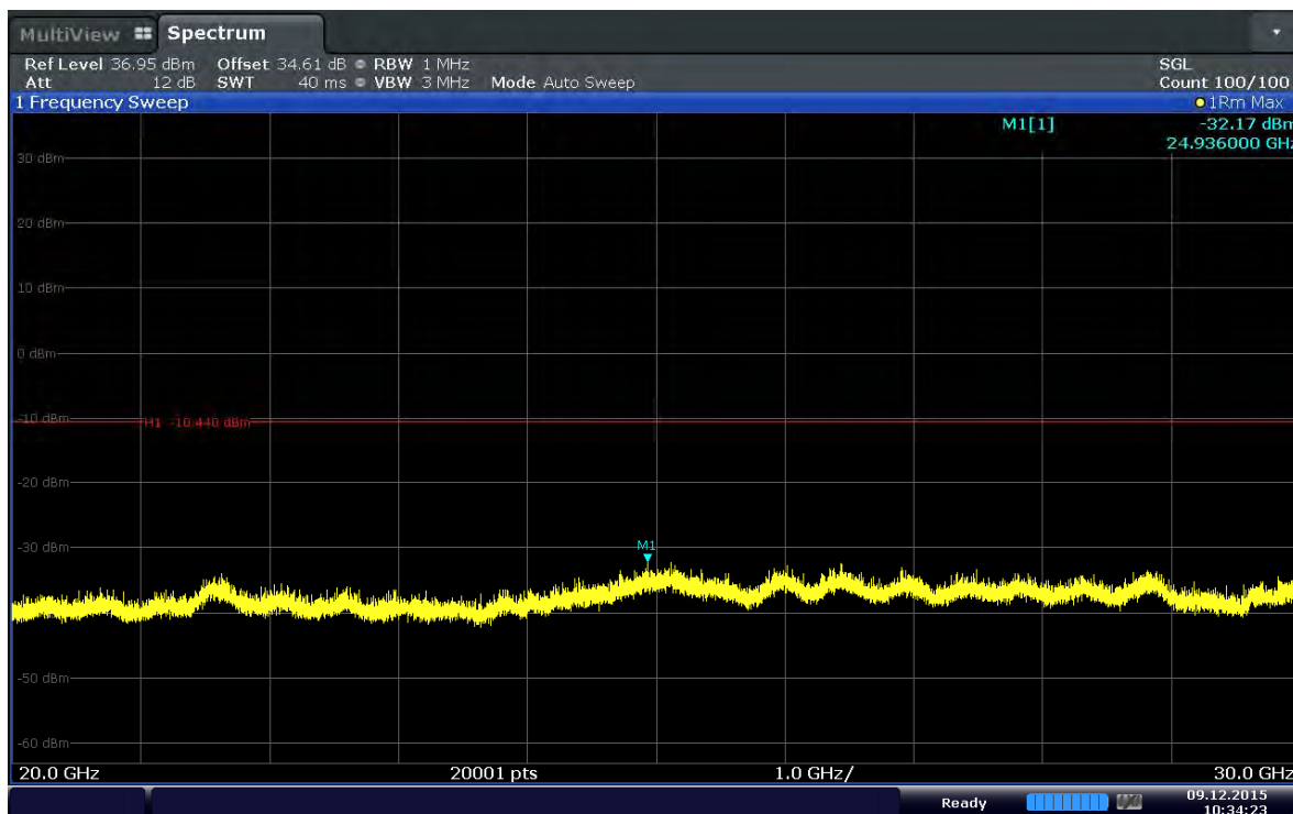
Plot 6-17. Conducted Spurious Plot (Band 41–5MHz–QPSK– RB Size 1–RB Offset 0–Ch.41215)
