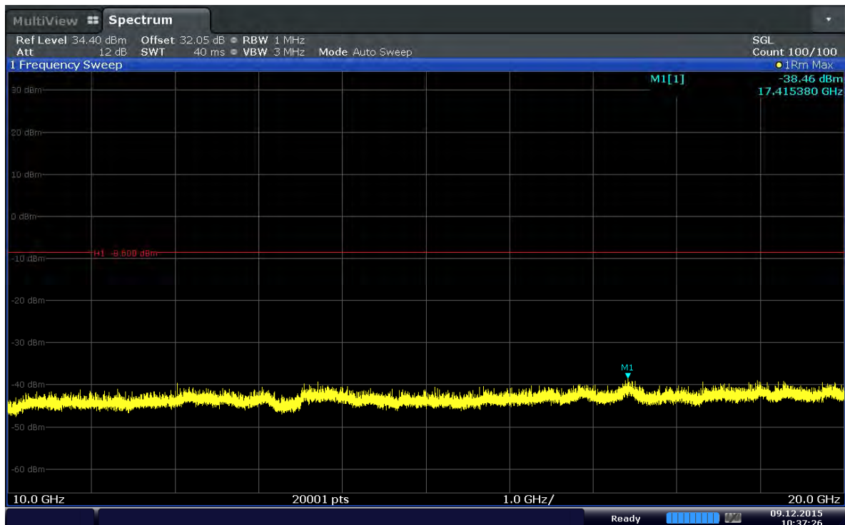
Plot 6-22. Conducted Spurious Plot (Band 41–10MHz–QPSK–RB Size 1–RB Offset 0–Ch.40740)
