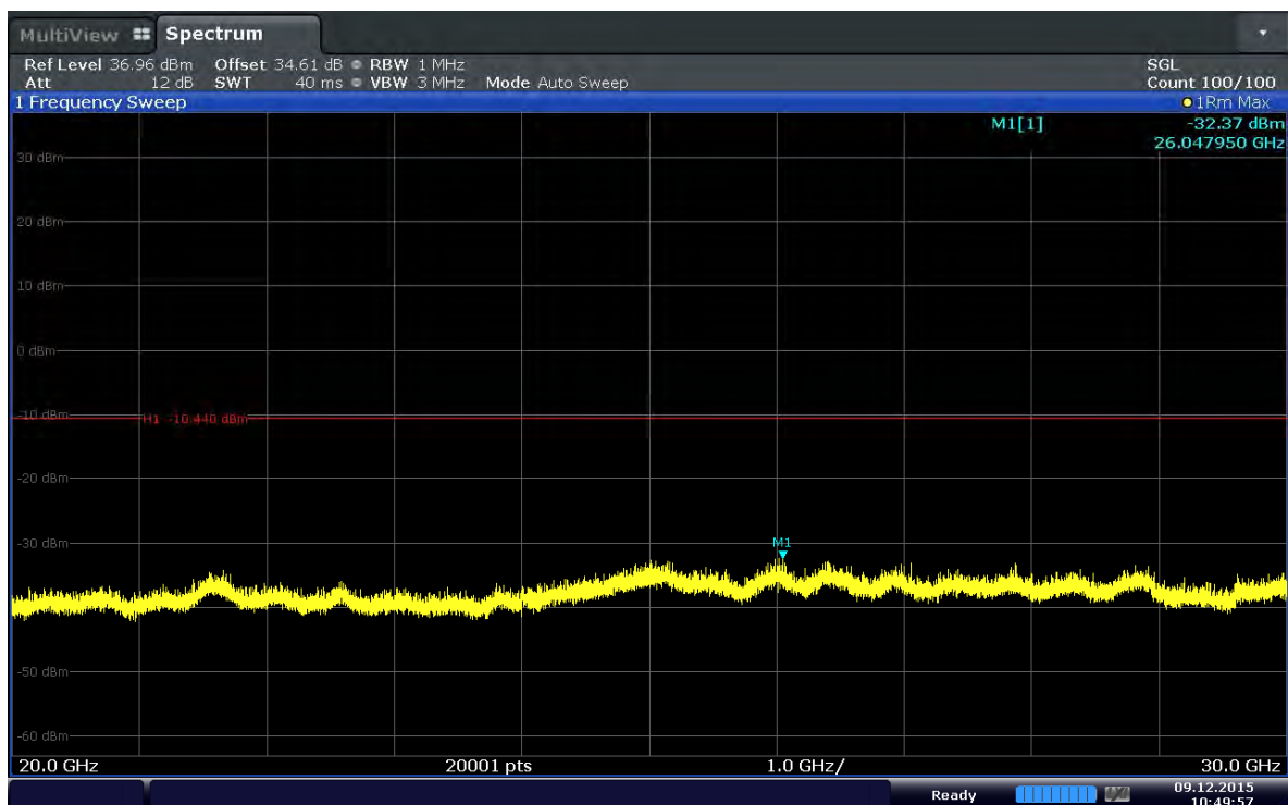
Plot 6-44. Conducted Spurious Plot (Band 41–20MHz–QPSK–RB Size 1–RB Offset 0–Ch.41140)
