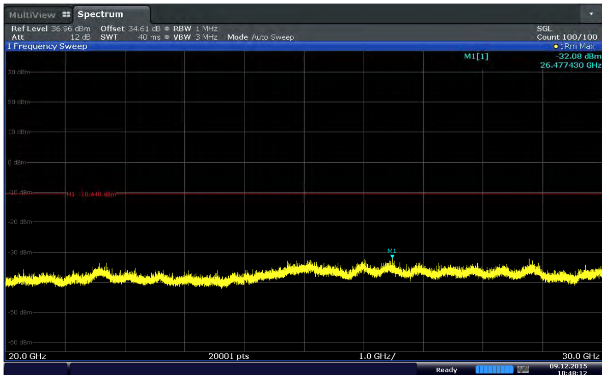
Plot 6-41. Conducted Spurious Plot (Band 41–20MHz–QPSK–RB Size 1–RB Offset 49–Ch.40740)
