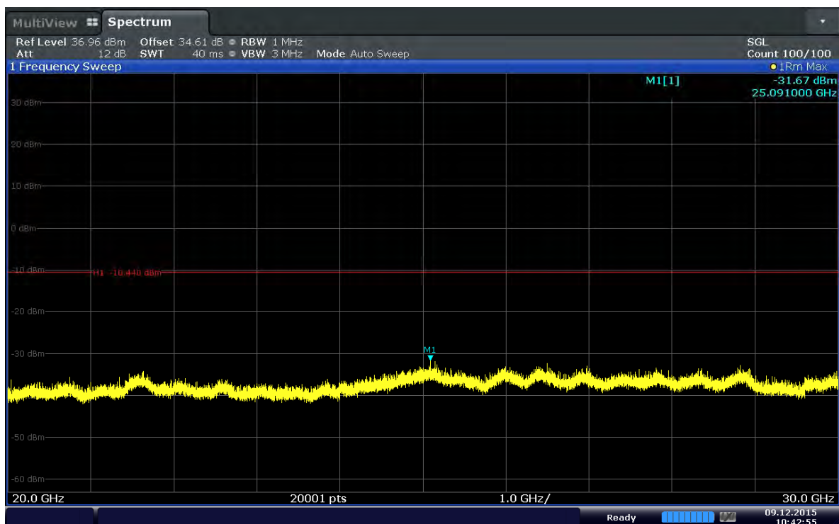
Plot 6-32. Conducted Spurious Plot (Band 41–15MHz–QPSK–RB Size 1–RB Offset 36–Ch.40740)
