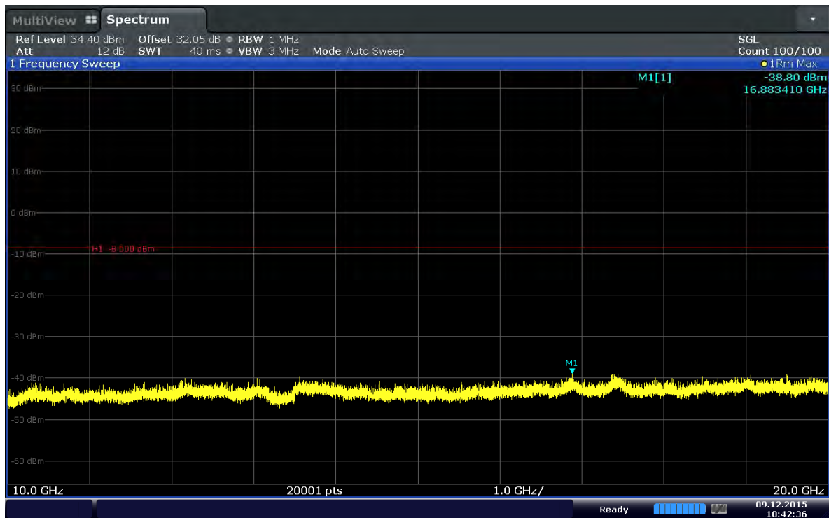
Plot 6-31. Conducted Spurious Plot (Band 41–15MHz–QPSK–RB Size 1–RB Offset 36–Ch.40740)
