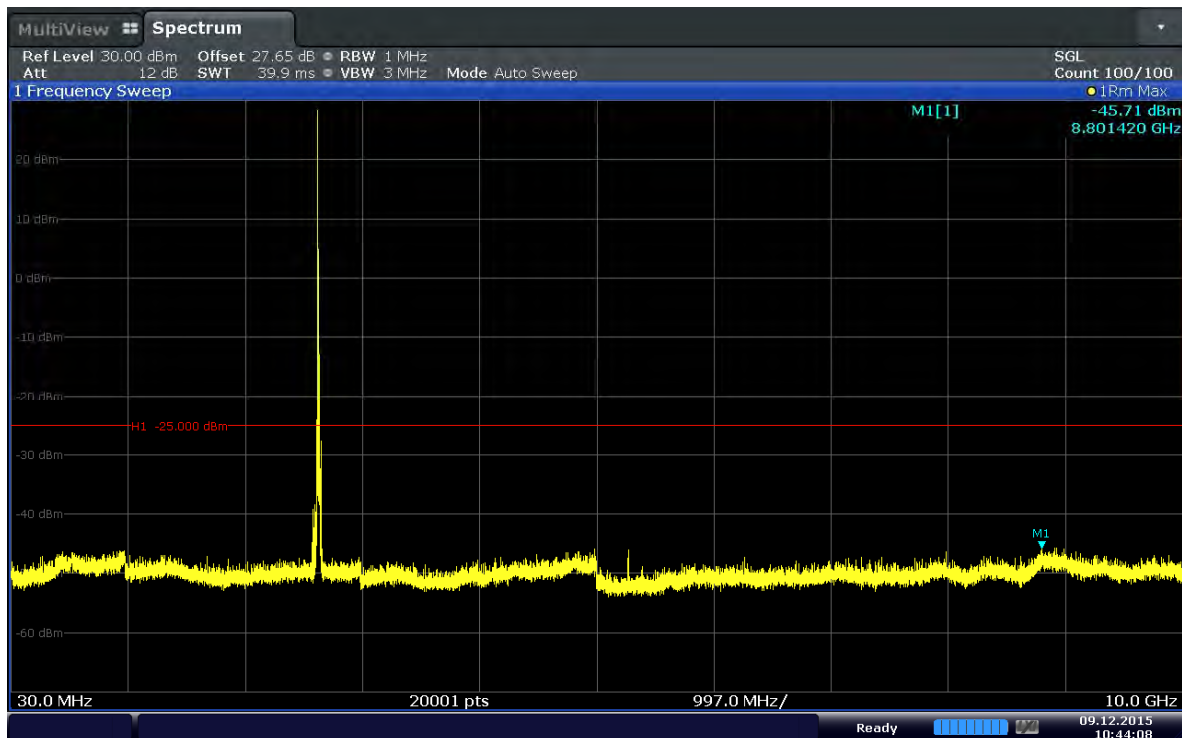
Plot 6-33. Conducted Spurious Plot (Band 41–15MHz–QPSK–RB Size 1–RB Offset 0–Ch.41165)
