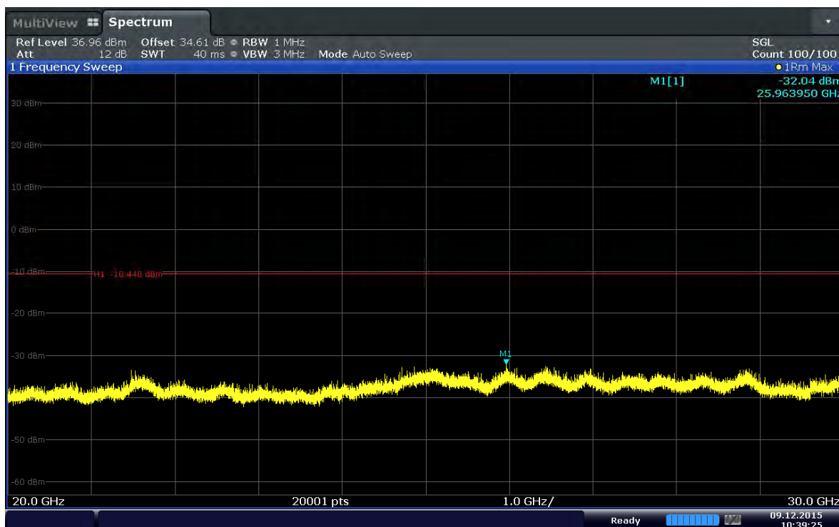
Plot 6-26. Conducted Spurious Plot (Band 41–10MHz–QPSK– RB Size 1–RB Offset 0–Ch.41190)
