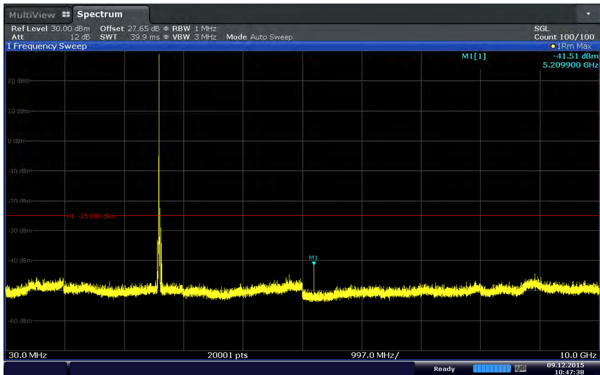
Plot 6-39. Conducted Spurious Plot (Band 41–20MHz–QPSK–RB Size 1–RB Offset 49–Ch.40740)
