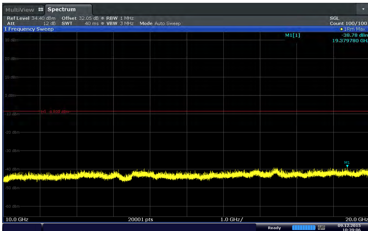
Plot 6-25. Conducted Spurious Plot (Band 41–10MHz–QPSK– RB Size 1–RB Offset 0–Ch.41190)
