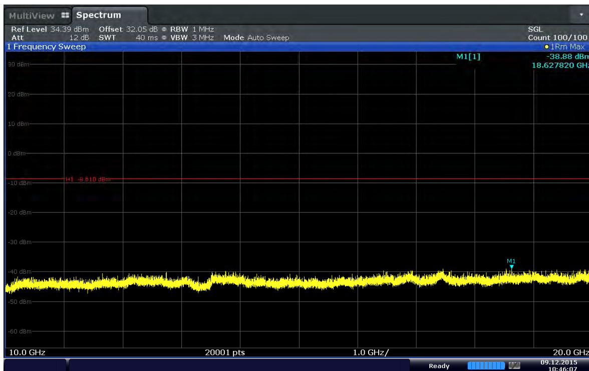
Plot 6-37. Conducted Spurious Plot (Band 41–20MHz–QPSK–RB Size 1–RB Offset 0–Ch.40340)
