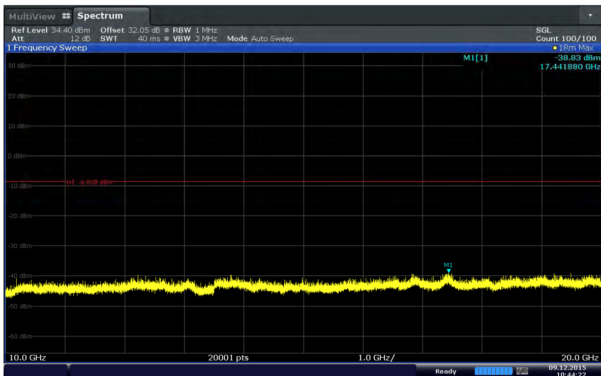
Plot 6-34. Conducted Spurious Plot (Band 41–15MHz–QPSK–RB Size 1–RB Offset 0–Ch.41165)
