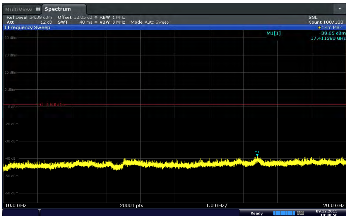
Plot 6-9. Conducted Spurious Plot (Band 41–5MHz–QPSK–RB Size 1–RB Offset 0–Ch.40265)
