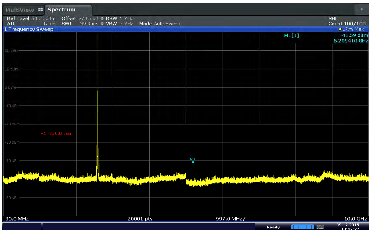
Plot 6-30. Conducted Spurious Plot (Band 41–15MHz–QPSK–RB Size 1–RB Offset 36–Ch.40740)
