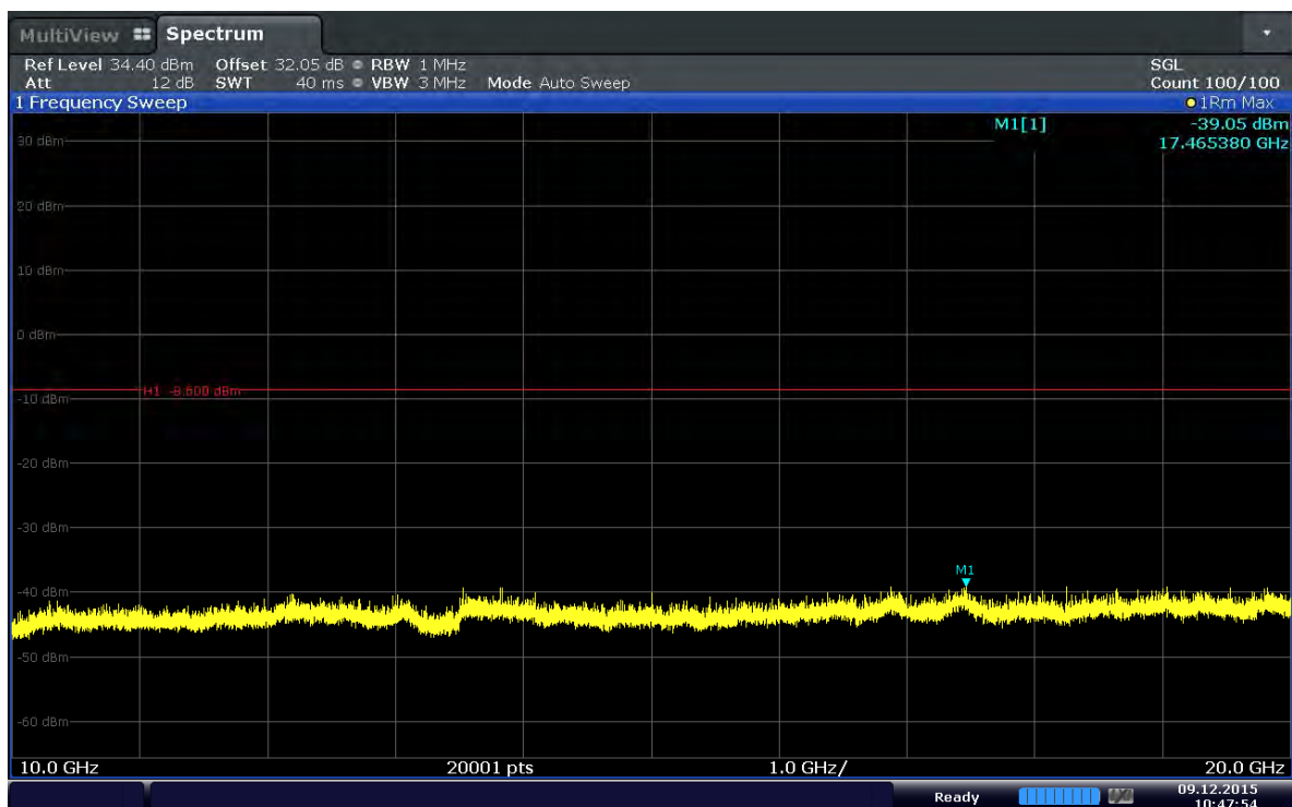
Plot 6-40. Conducted Spurious Plot (Band 41–20MHz–QPSK–RB Size 1–RB Offset 49–Ch.40740)
