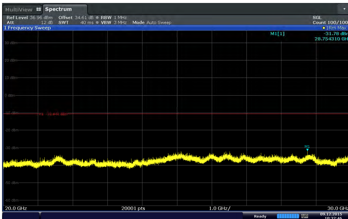
Plot 6-14. Conducted Spurious Plot (Band 41–5MHz–QPSK–RB Size 1–RB Offset 12–Ch.40740)
