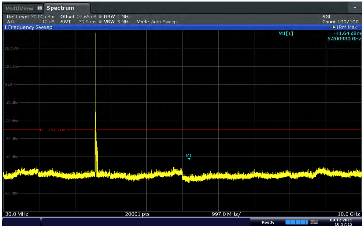
Plot 6-21. Conducted Spurious Plot (Band 41–10MHz–QPSK–RB Size 1–RB Offset 0–Ch.40740)
