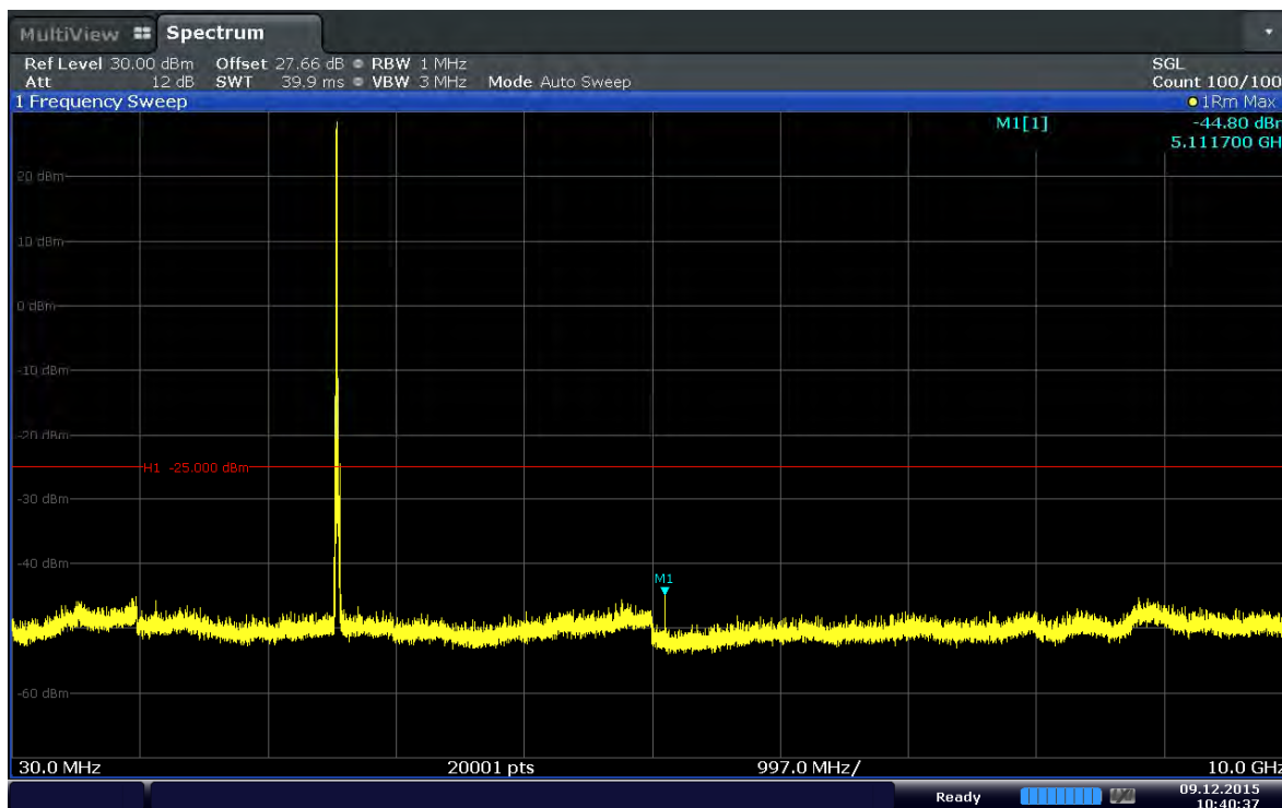
Plot 6-27. Conducted Spurious Plot (Band 41–15MHz–QPSK–RB Size 1–RB Offset 0–Ch.40315)
