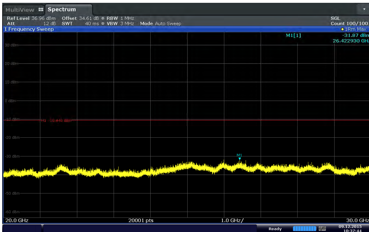
Plot 6-23. Conducted Spurious Plot (Band 41–10MHz–QPSK– RB Size 1–RB Offset 0–Ch.40740)
