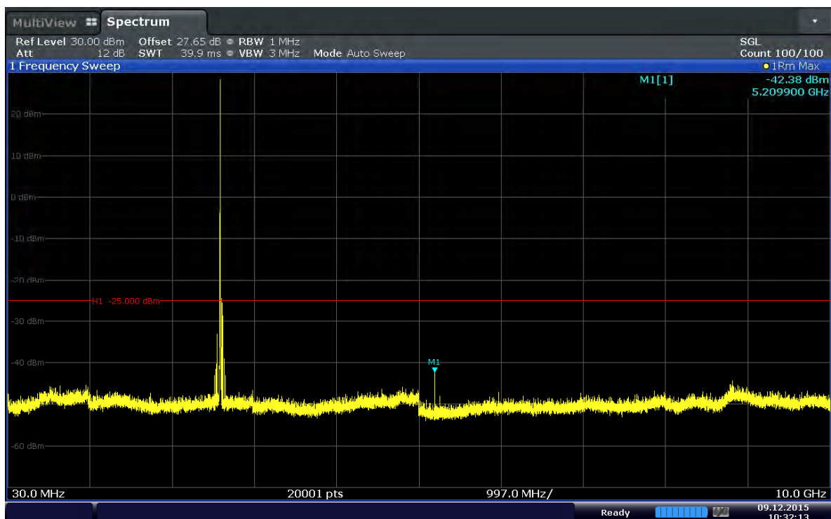
Plot 6-12. Conducted Spurious Plot (Band 41–5MHz–QPSK–RB Size 1–RB Offset 12–Ch.40740)
