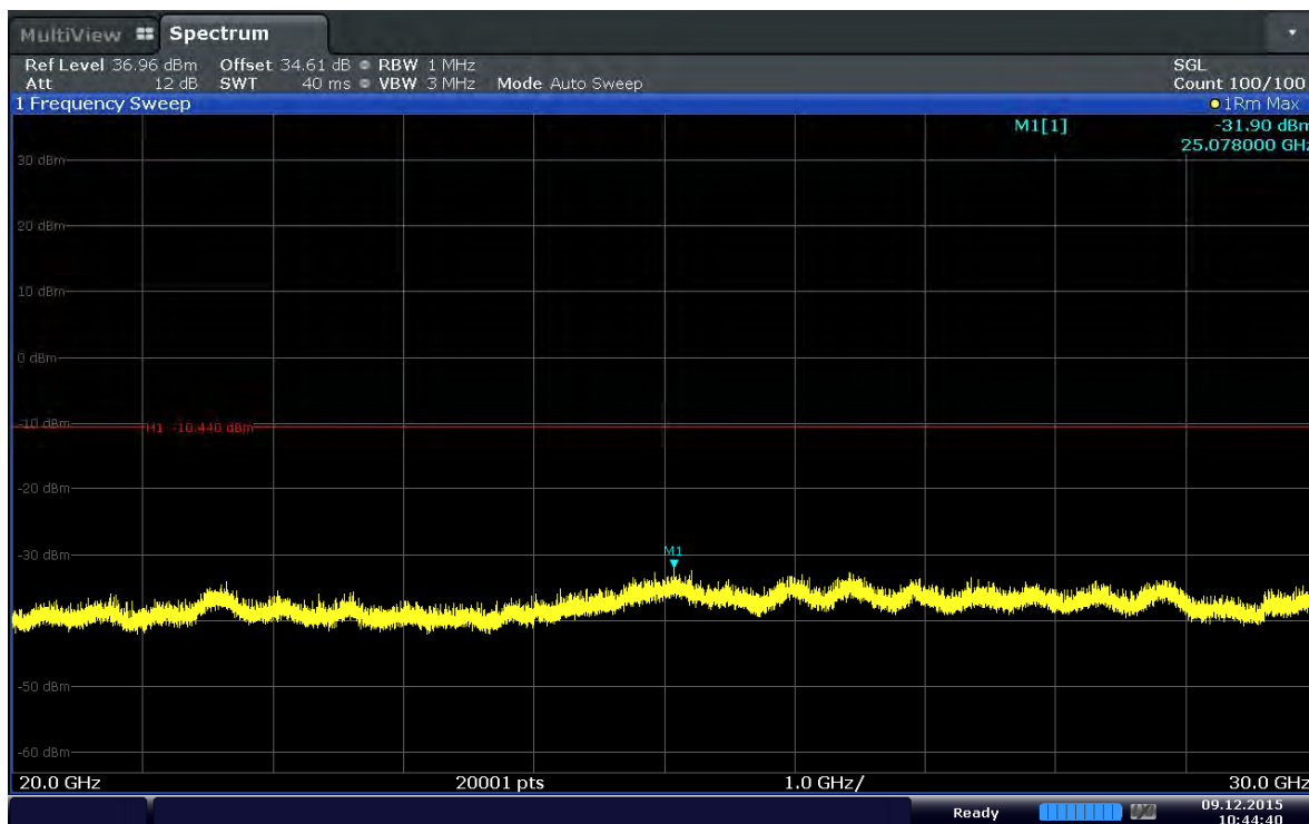
Plot 6-35. Conducted Spurious Plot (Band 41–15MHz–QPSK–RB Size 1–RB Offset 0–Ch.41165)
