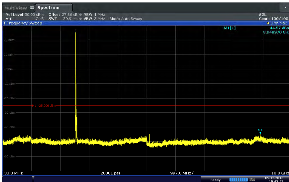
Plot 6-36. Conducted Spurious Plot (Band 41–20MHz–QPSK–RB Size 1–RB Offset 0–Ch.40340)
