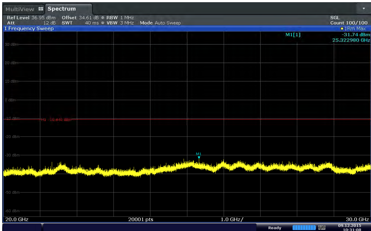
Plot 6-11. Conducted Spurious Plot (Band 41–5MHz–QPSK–RB Size 1–RB Offset 0–Ch.40265)
