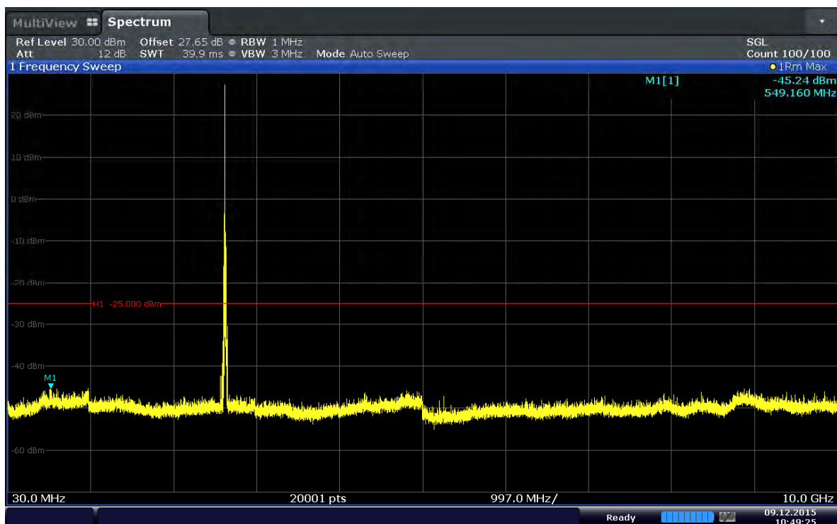
Plot 6-42. Conducted Spurious Plot (Band 41–20MHz–QPSK–RB Size 1–RB Offset 0–Ch.41140)
