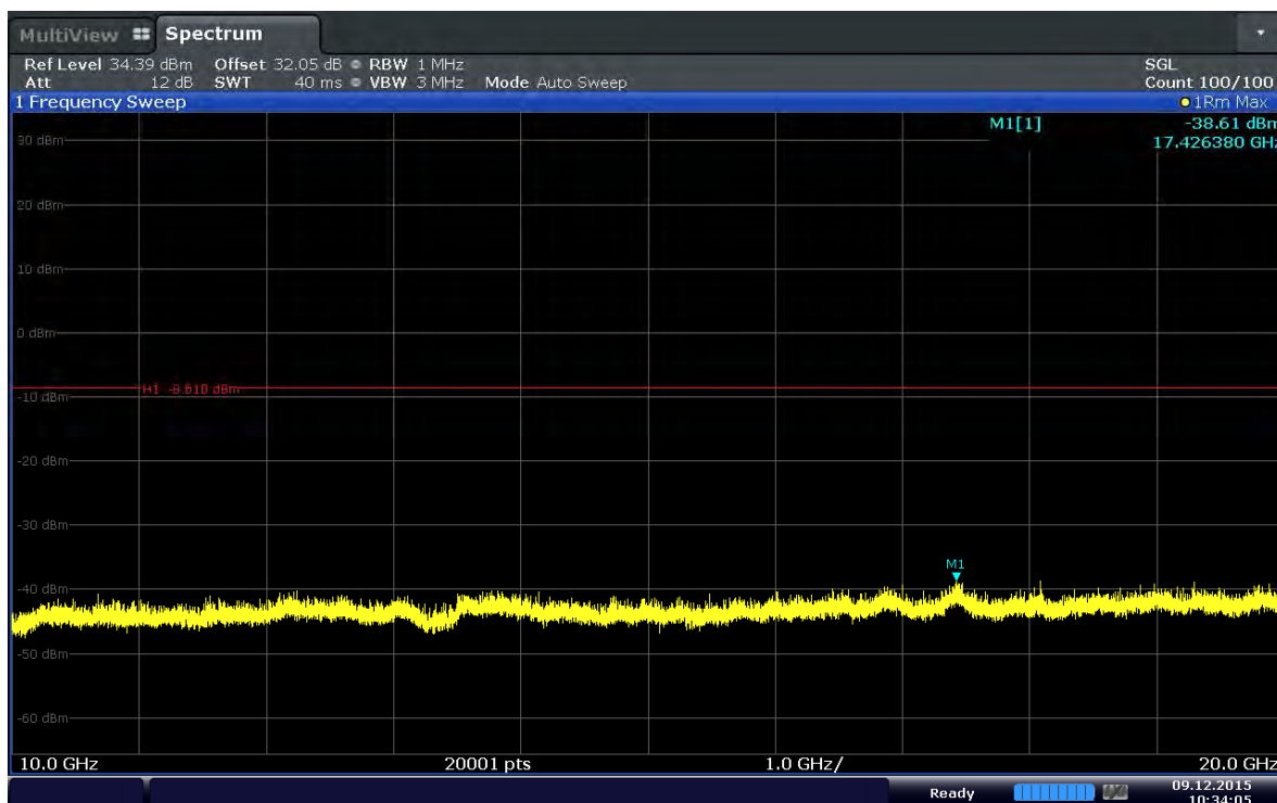
Plot 6-16. Conducted Spurious Plot (Band 41–5MHz–QPSK– RB Size 1–RB Offset 0–Ch.41215)
