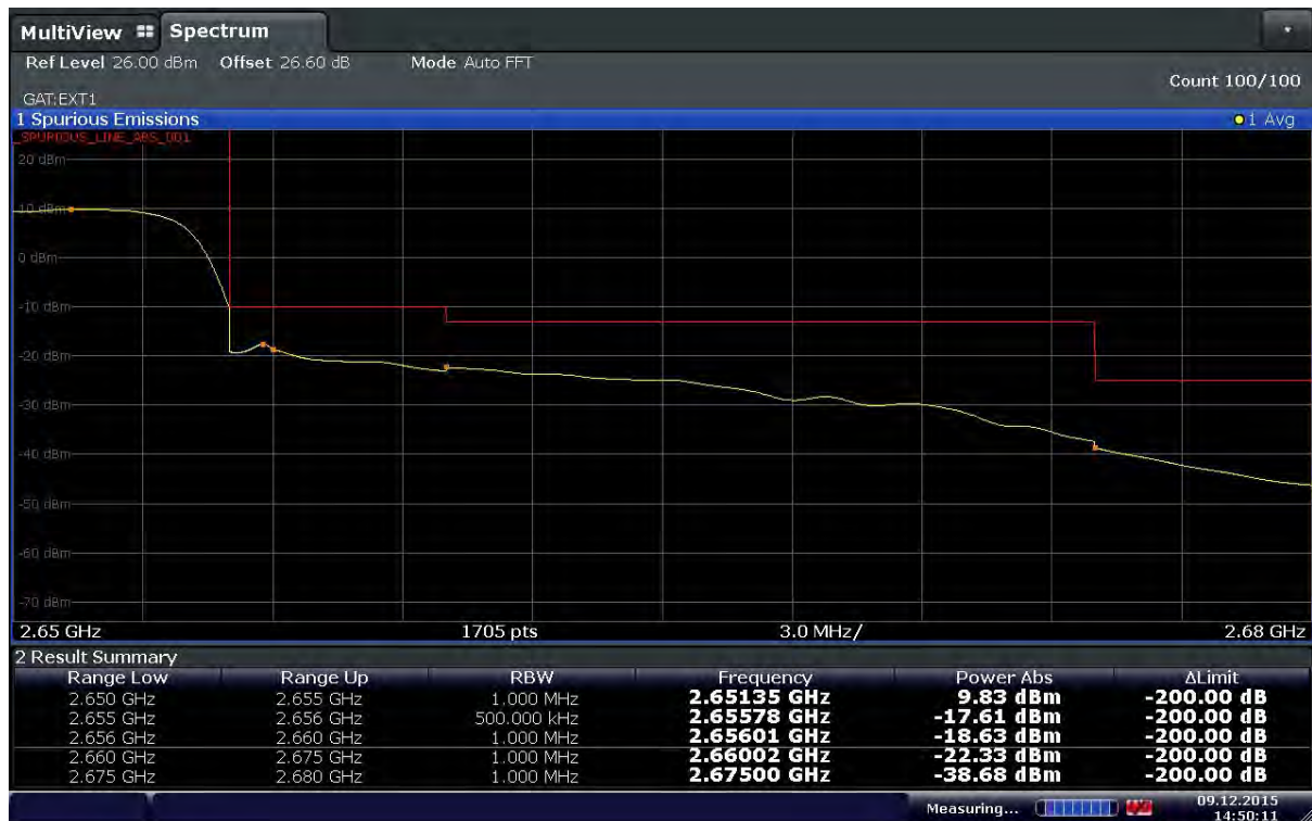
Plot 6-52. Upper Band Edge Plot (Band41 – 20MHz – QPSK – RB Size 100 – Ch.41140)
