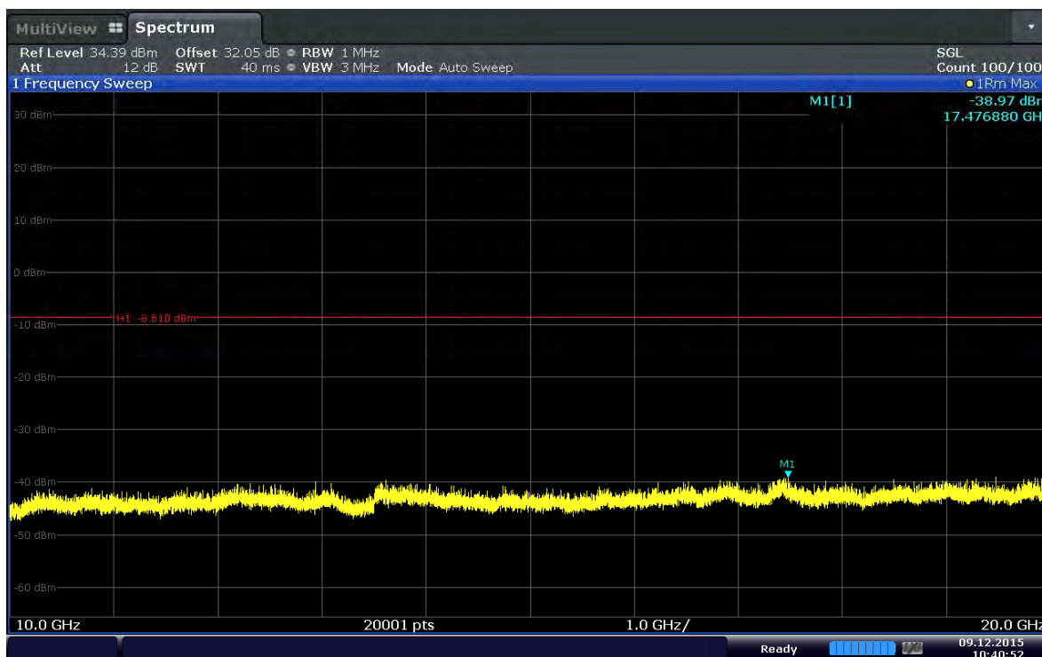
Plot 6-28. Conducted Spurious Plot (Band 41–15MHz–QPSK–RB Size 1–RB Offset 0–Ch.40315)
