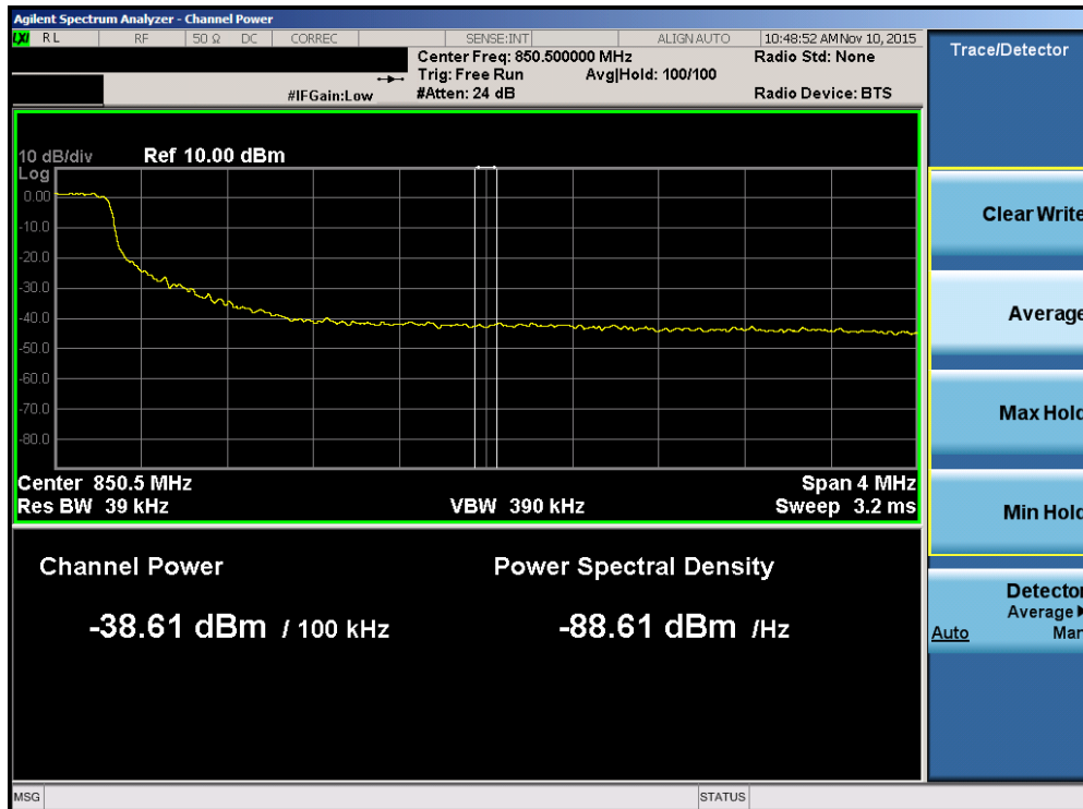
Plot 7-90. Upper Extended Band Edge Plot (Band 5 – 5.0MHz QPSK – RB Size 25)
