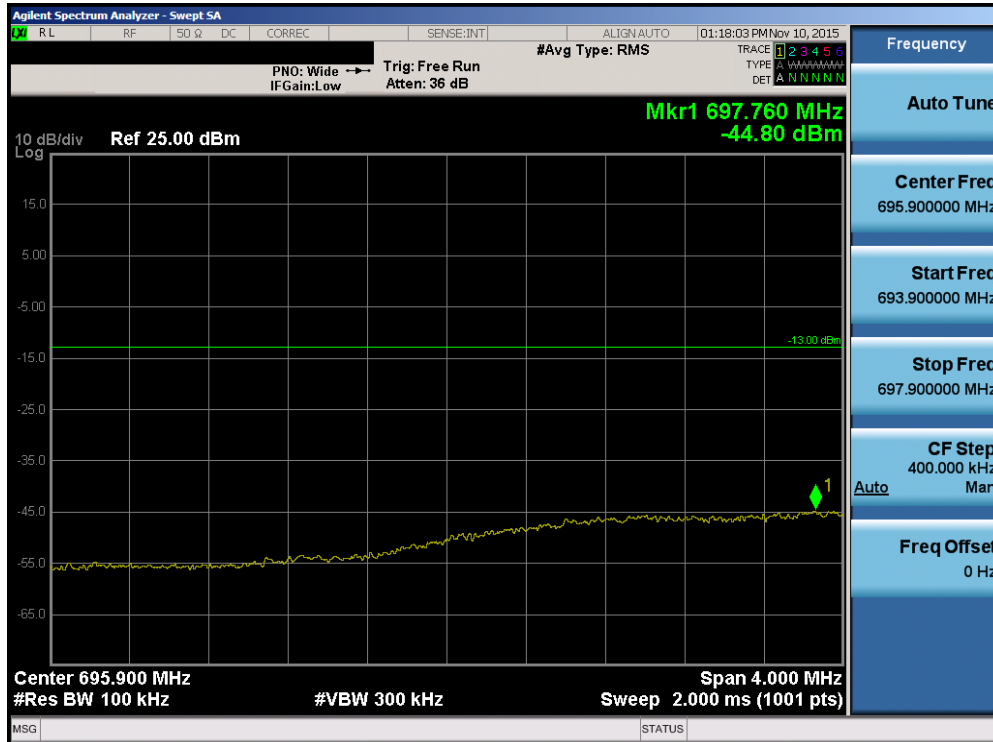
Plot 7-74. Lower Extended Band Edge Plot (Band 17 – 5.0MHz QPSK – RB Size 25)
