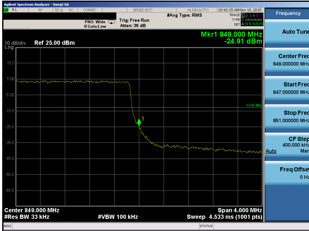
Plot 7-85. Upper Band Edge Plot (Band 5 – 3.0MHz QPSK – RB Size 15)
