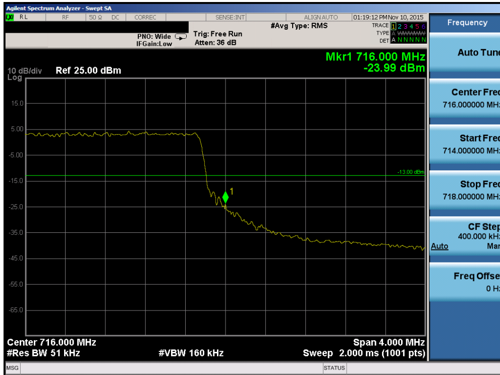
Plot 7-75. Upper Band Edge Plot (Band 17 – 5.0MHz QPSK – RB Size 25)
