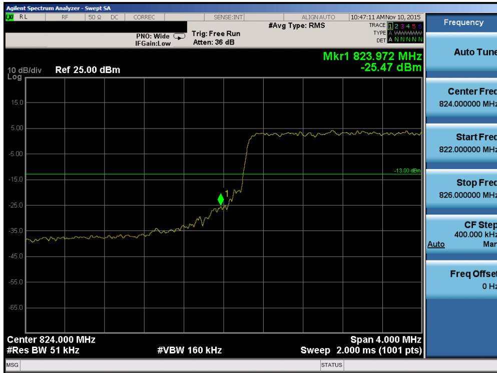
Plot 7-87. Lower Band Edge Plot (Band 5 – 5.0MHz QPSK – RB Size 25)
