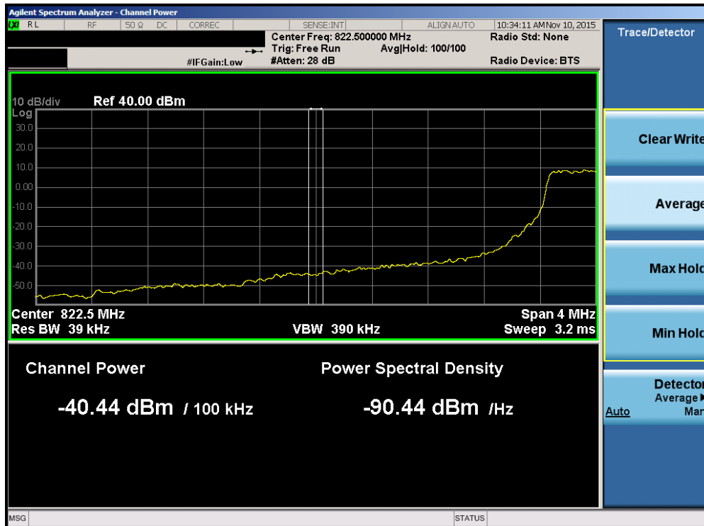
Plot 7-80. Lower Extended Band Edge Plot (Band 5 – 1.4MHz QPSK – RB Size 6)
