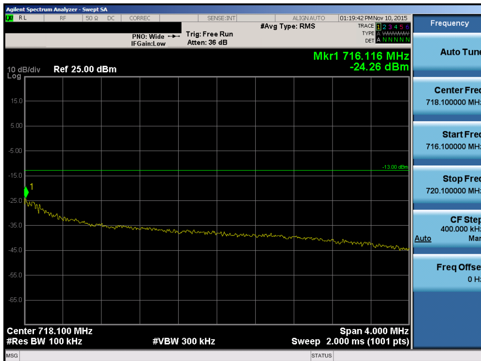
Plot 7-76. Upper Extended Band Edge Plot (Band 17 – 5.0MHz QPSK – RB Size 25)
