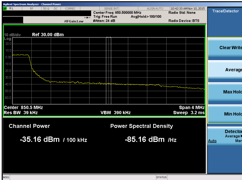
Plot 7-86. Upper Extended Band Edge Plot (Band 5 – 3.0MHz QPSK – RB Size 15)
