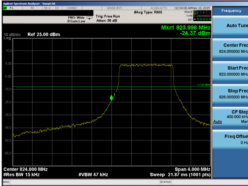
Plot 7-79. Lower Band Edge Plot (Band 5 – 1.4MHz QPSK – RB Size 6)
