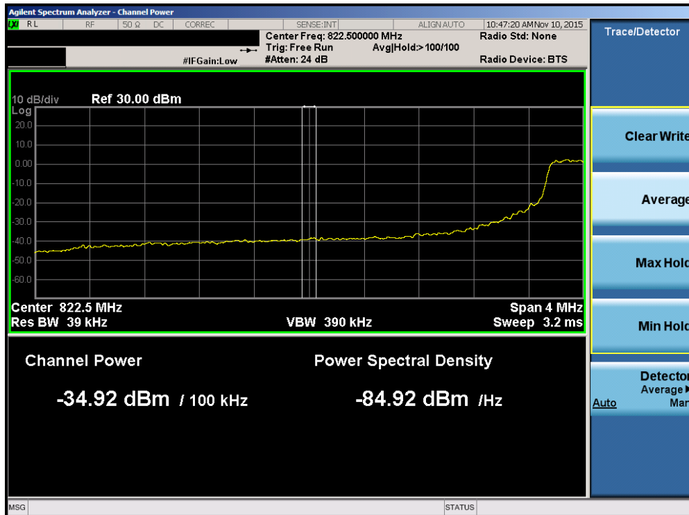
Plot 7-88. Lower Extended Band Edge Plot (Band 5 – 5.0MHz QPSK – RB Size 25)
