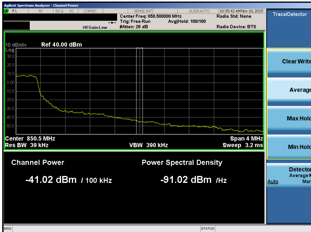
Plot 7-82. Upper Extended Band Edge Plot (Band 5 – 1.4MHz QPSK – RB Size 6)
