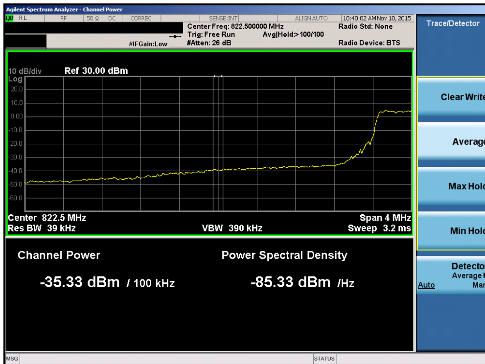
Plot 7-84. Lower Extended Band Edge Plot (Band 5 – 3.0MHz QPSK – RB Size 15)
