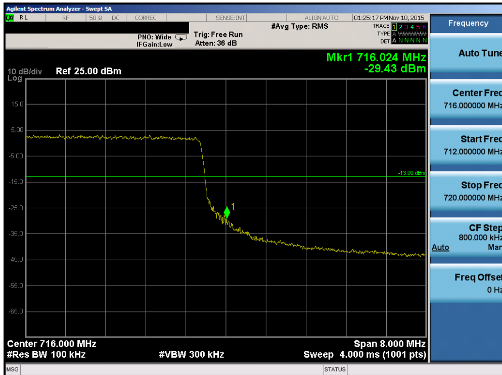
Plot 7-78. Upper Band Edge Plot (Band 17 – 10.0MHz QPSK – RB Size 50)
