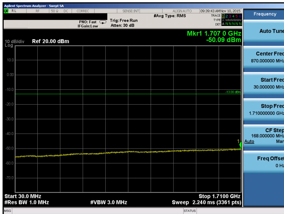
Plot 7-38. Conducted Spurious Plot (AWS WCDMA Mode – Ch. 1762)
