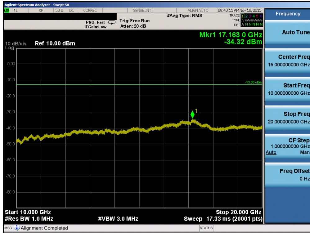
Plot 7-40. Conducted Spurious Plot (AWS WCDMA Mode – Ch. 1762)
