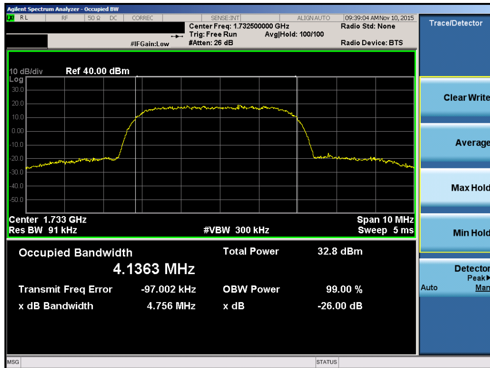
Plot 7-6. Occupied Bandwidth Plot (AWS WCDMA Mode – Ch. 1762)
