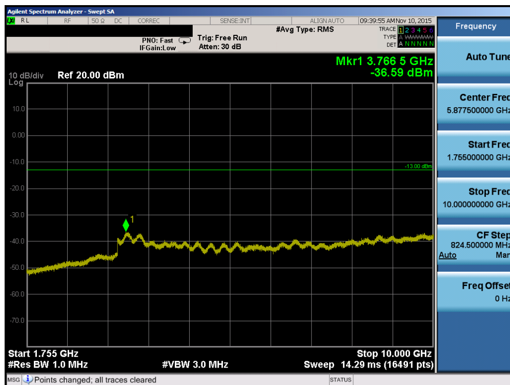
Plot 7-39. Conducted Spurious Plot (AWS WCDMA Mode – Ch. 1762)
