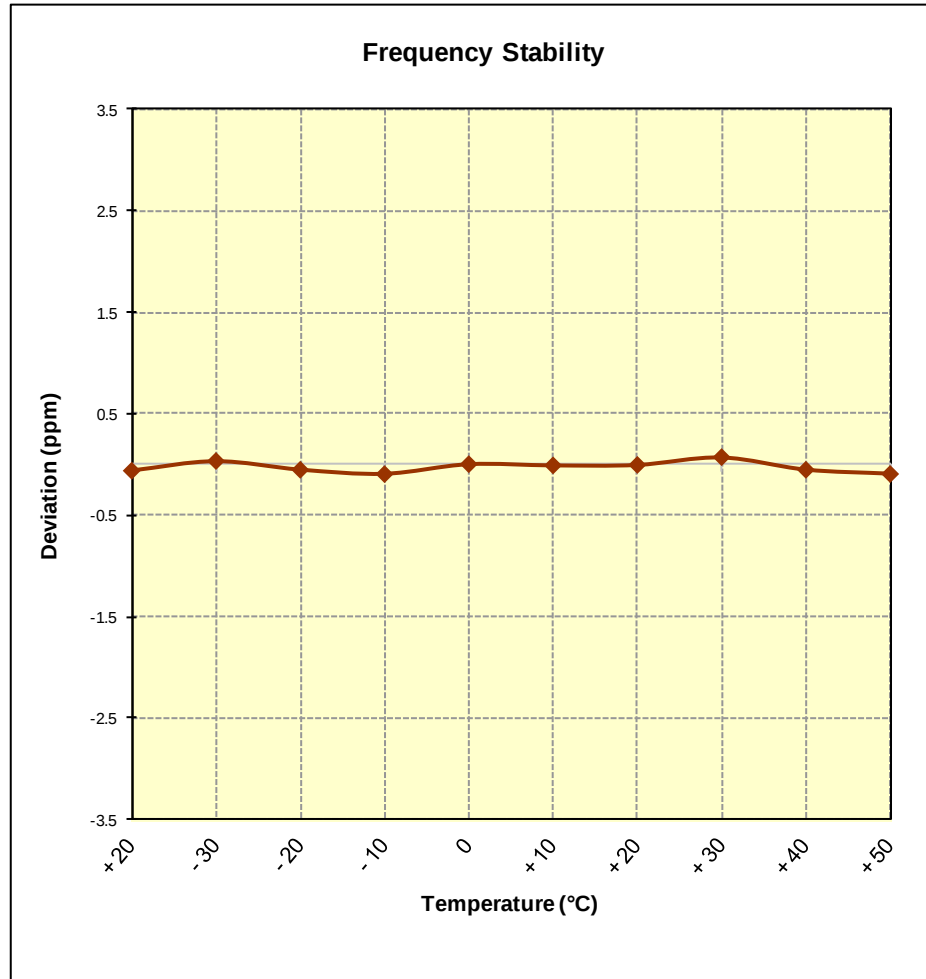
Figure 7-10. Frequency Stability Graph (AWS WCDMA Mode – Ch. 1762)
